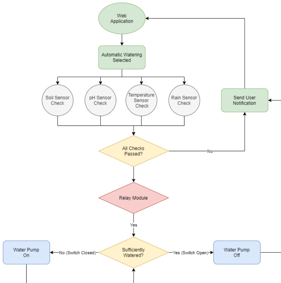
Figure 19: Automatic Watering Structure
