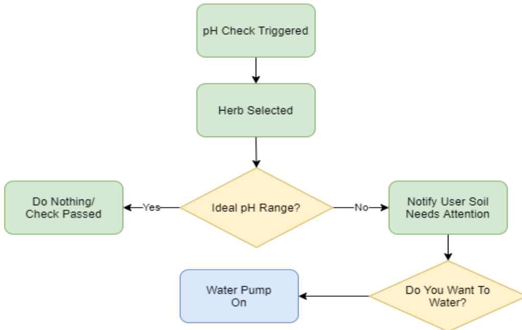
Figure 24: pH Sensor Check
