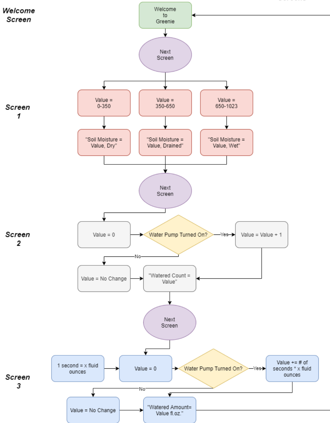
Figure 25: LCD Software to Hardware Configuration
