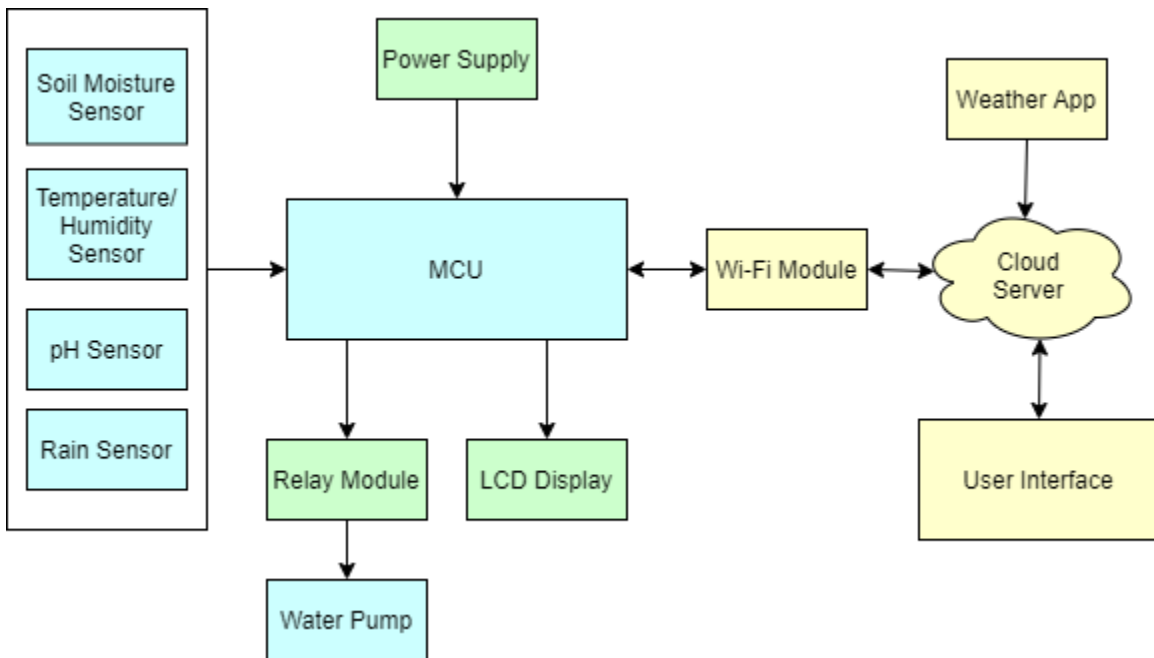
Figure 5: Hardware and Software Communication
