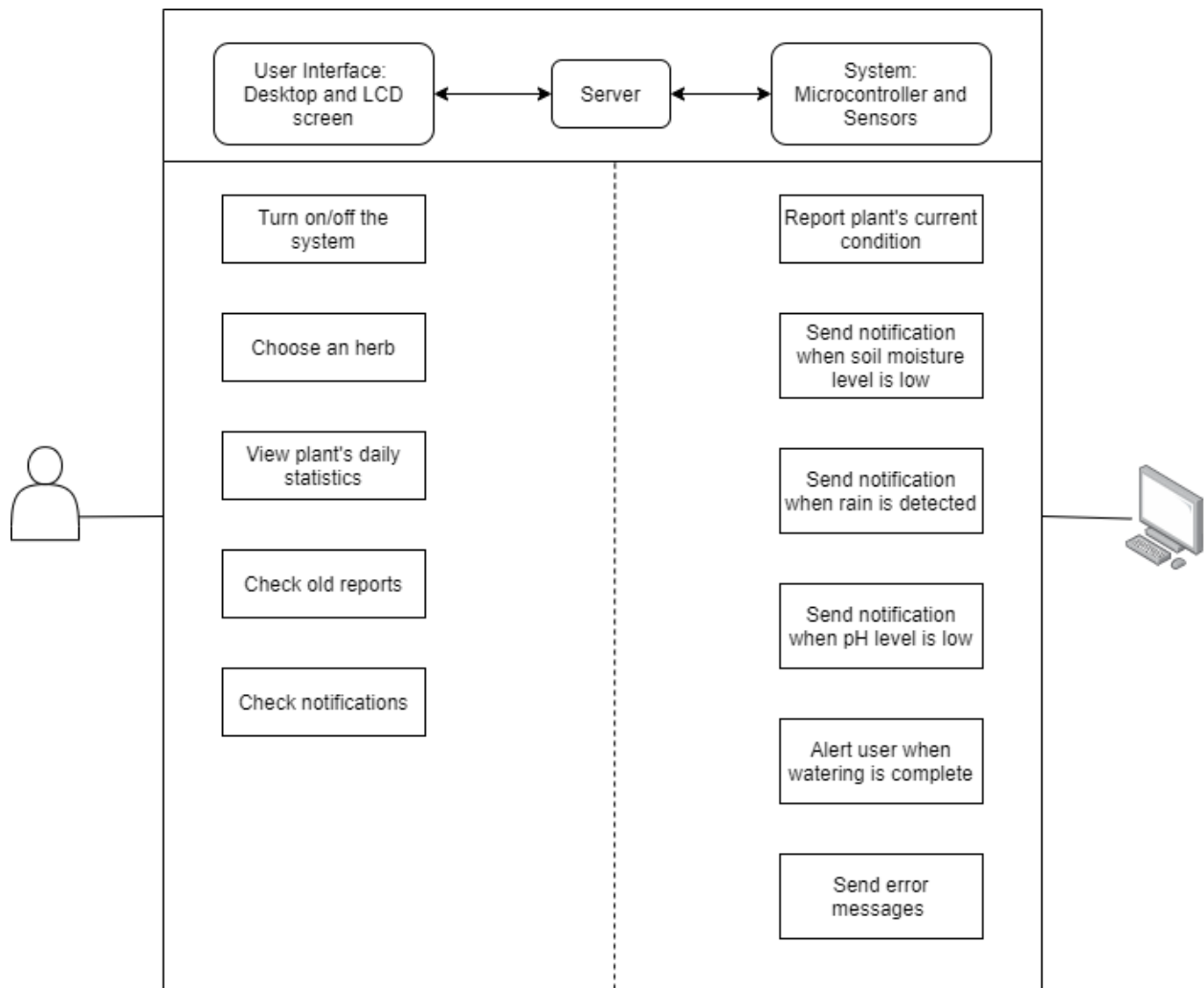
Figure 6: Communication between the user and the system
