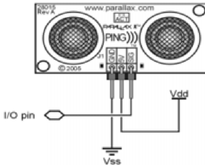
Figure 14: Parallax Ping Sensor
