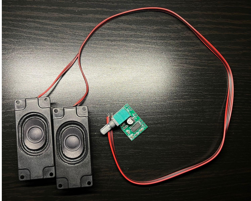
Figure 49: Speakers along with Amplifier
