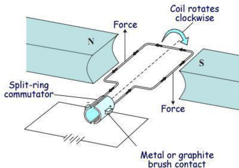
Figure 16: Conceptual diagram of a DC Motor [13]
