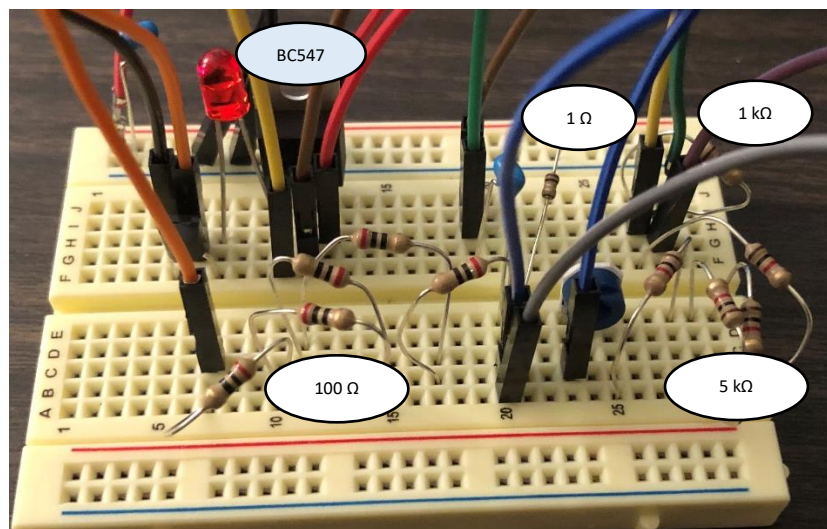
Figure 71: Voltage Regulation from Solar to Battery
