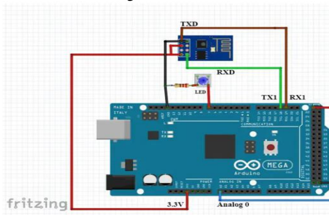
Figure 65: ESP8266-01 and Arduino connection. Reprinted with permission from https://create.arduino.cc
