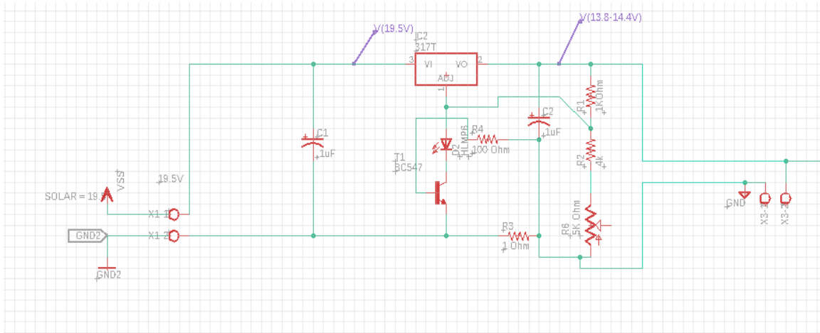
Figure 73: Voltage Regulation Circuitry, Overall Schematic Part 1
