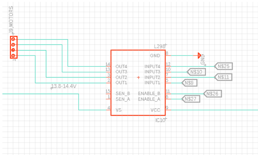
Figure 74: Motor Control, Overall Schematic Part 2
