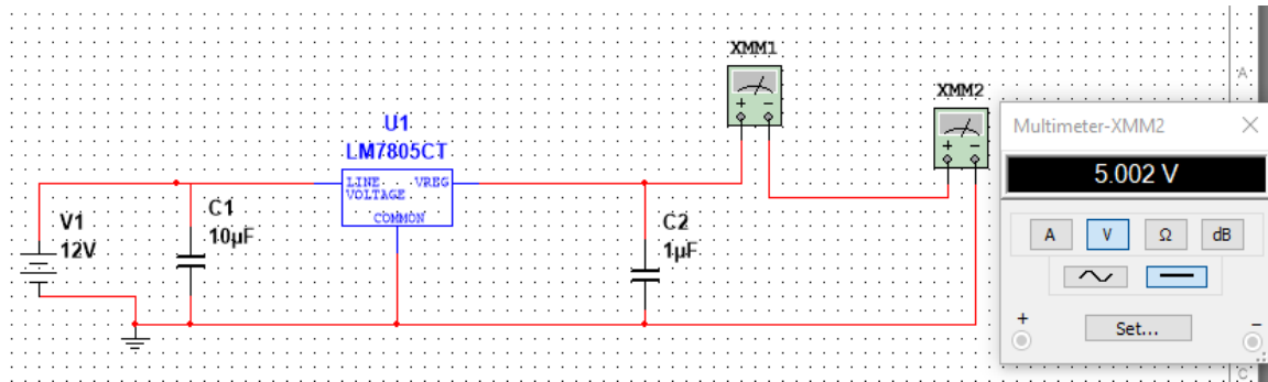
Figure 58: Battery to Microcontroller Schematic
