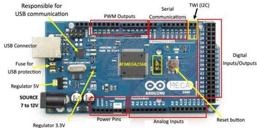
Figure 27: Arduino Mega 2560. Reprinted with permission from www.arduino.cc
