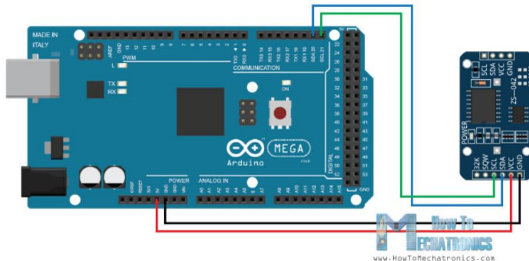
Figure 63: Arduino Mega to DS3231 Connection. Reprinted with permission from HowToMechatronics
