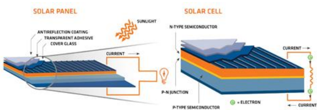
Figure 2: Photovoltaic Functionality
