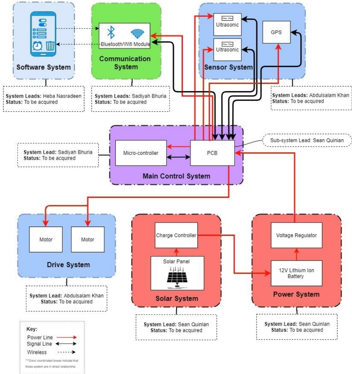
Figure 1: GRAD Bot Block Diagram
