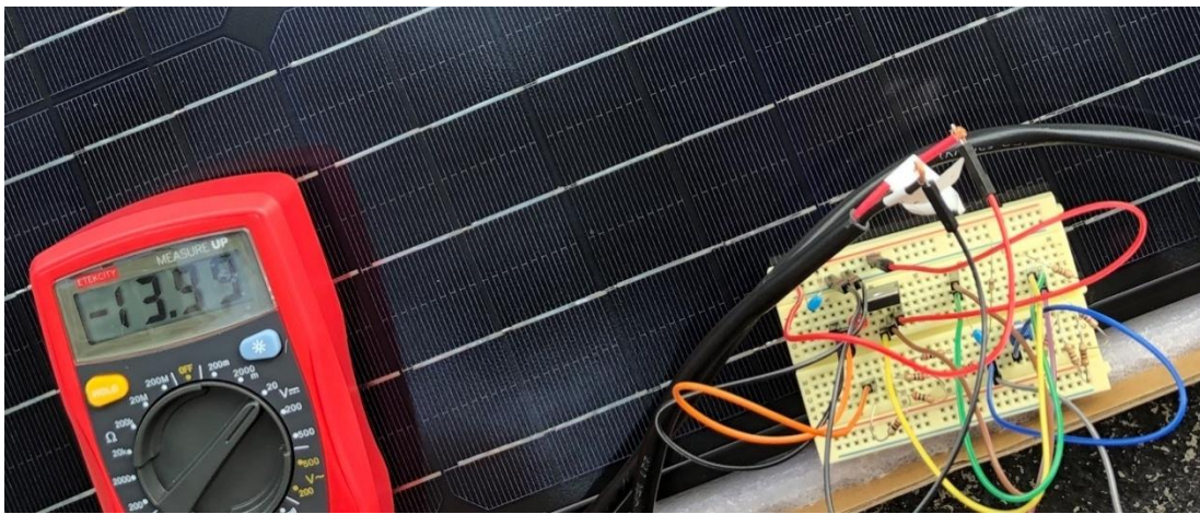
Figure 70: Voltage Testing of the Voltage Regulation Output of Solar Input
