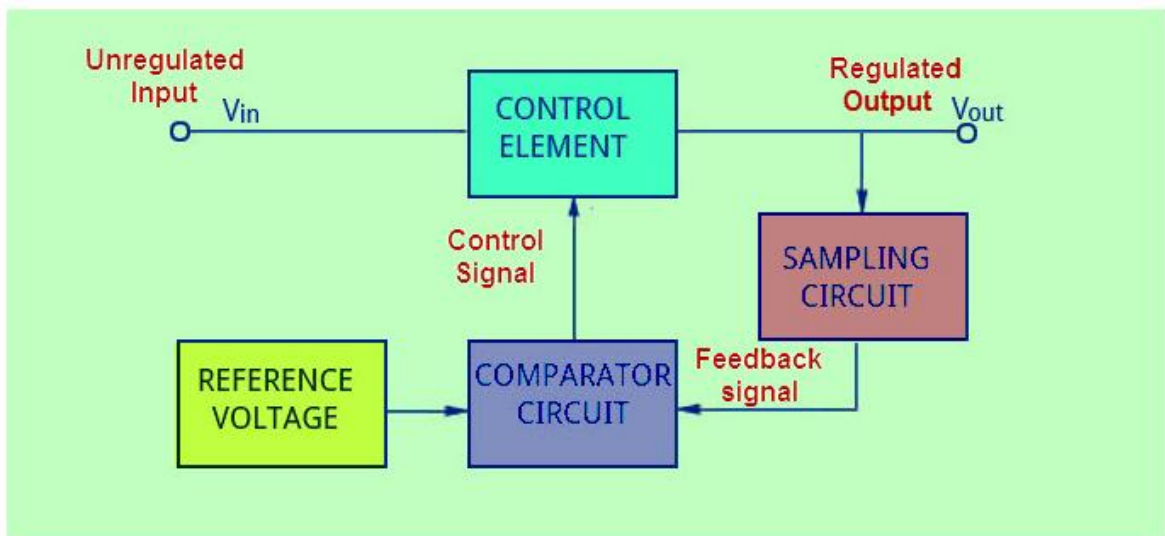
Figure 3: Series Voltage Regulator Topology
