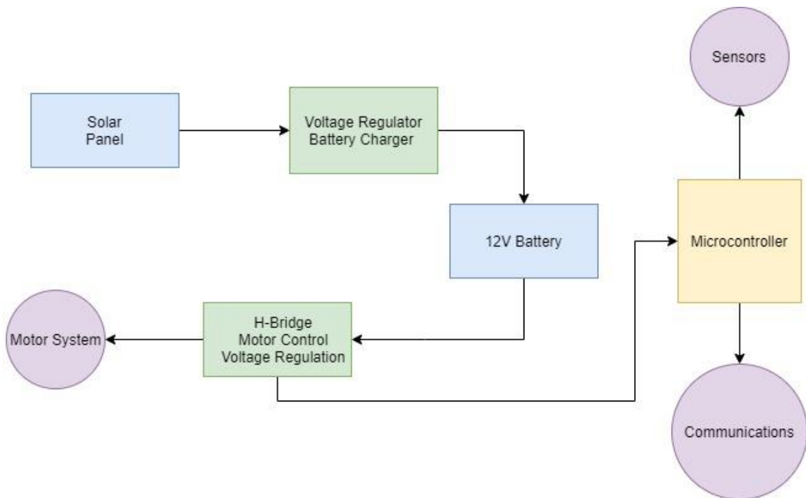
Figure 56: Power Flow Design
