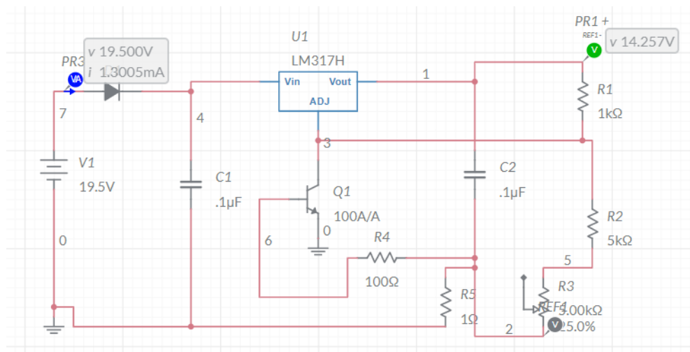
Figure 57: Solar Panel and Battery Voltage Regulator Circuit with LM317
