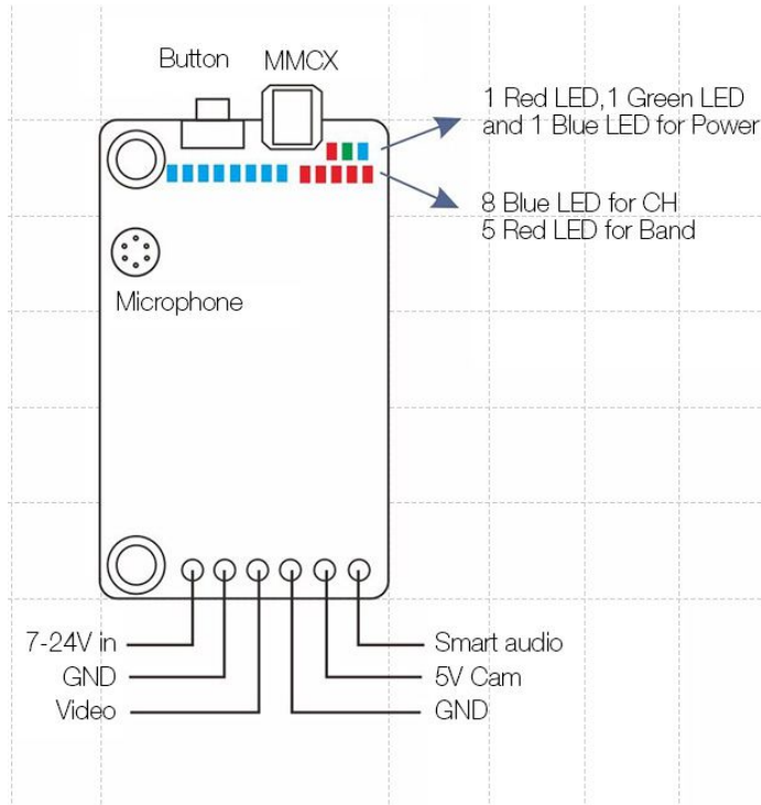
Figure 5.15: Eachine TX805 Schematic (Permission Requested to Reproduce)
