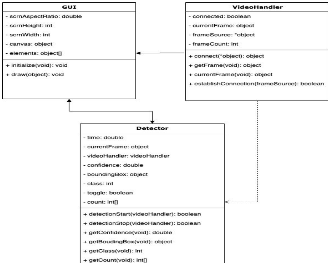
Figure 6.2: Pilot Companion App Class Diagram
