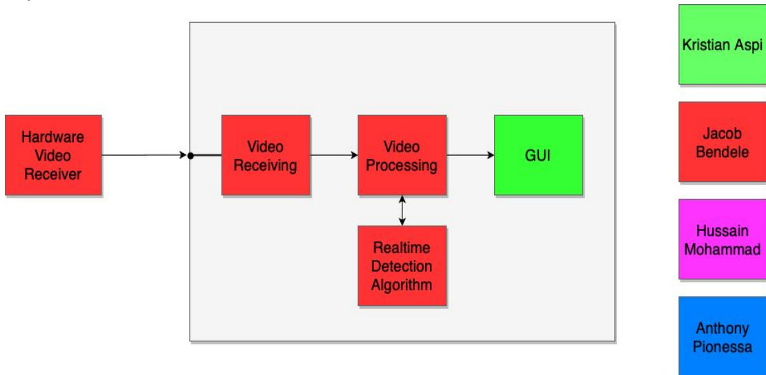
Figure 2.3: Pilot App Software Block Diagram
