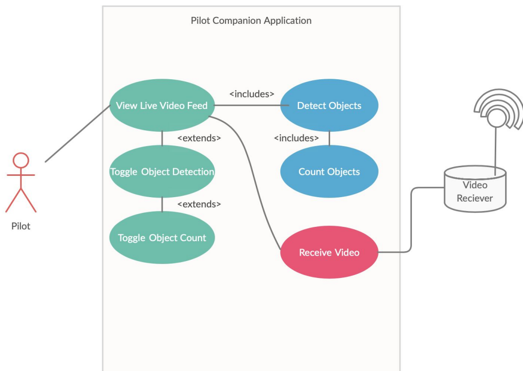
Figure 6.1: Pilot Companion App Use Case
