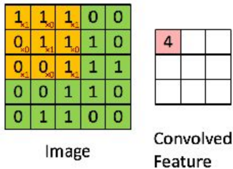
Figure 3.25: Image and Convolved Feature [77]
