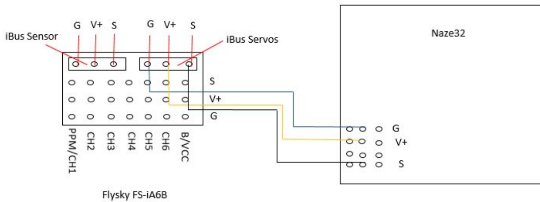
Figure 5.18: Drone Controller Receiver Connection Design
