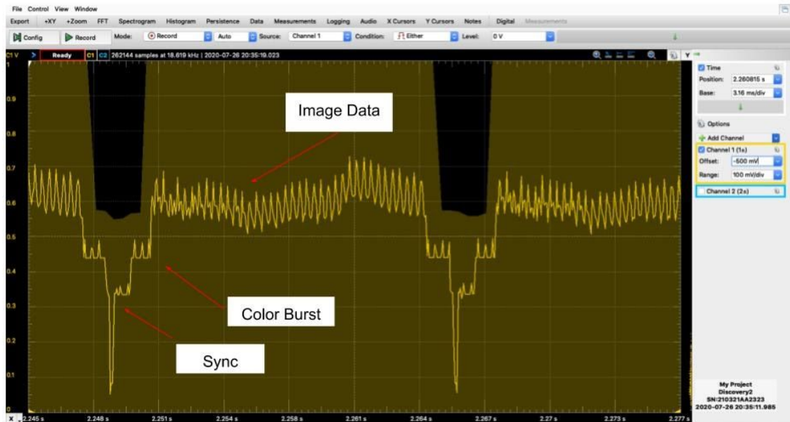
Figure 7.6: Camera Video Signal Test Result
