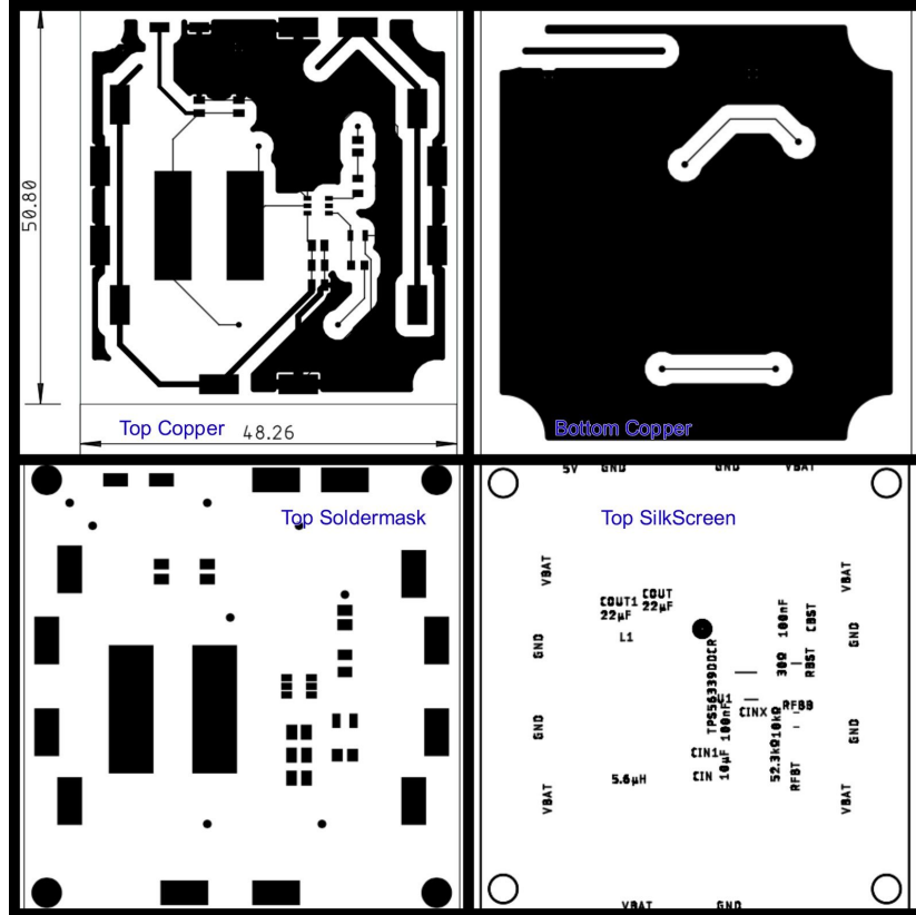
Figure 7.3: Gerber Files Returned from Manufacturer
