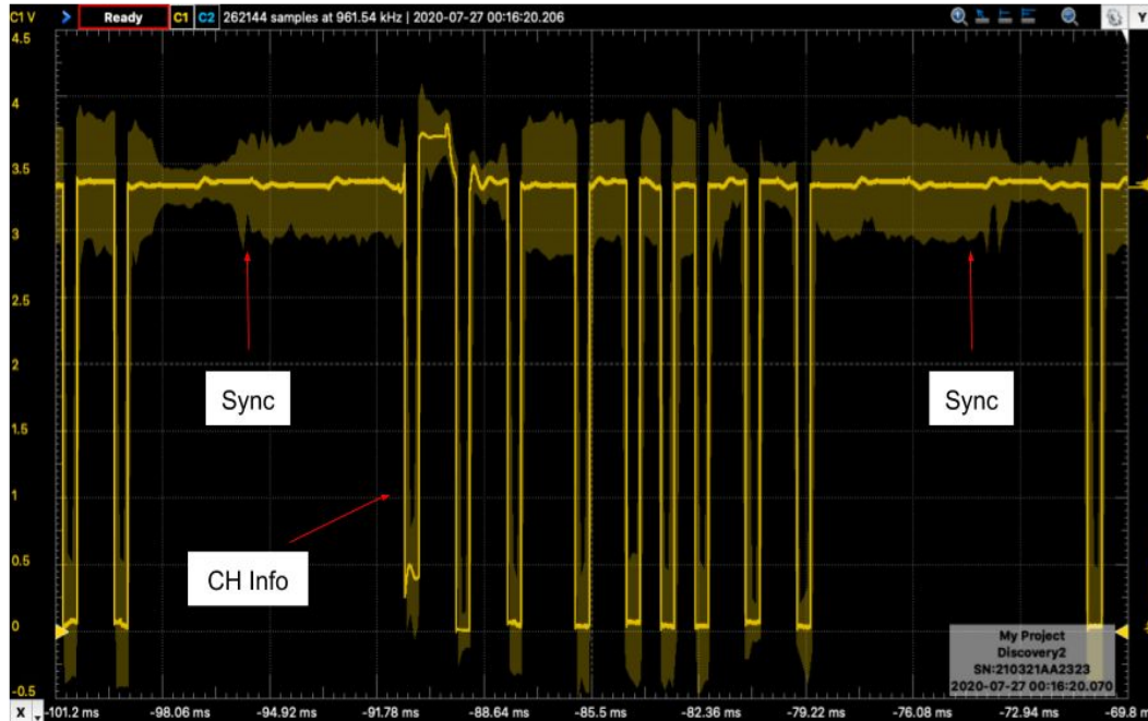
Figure 7.8: CPM Signal Test Result
