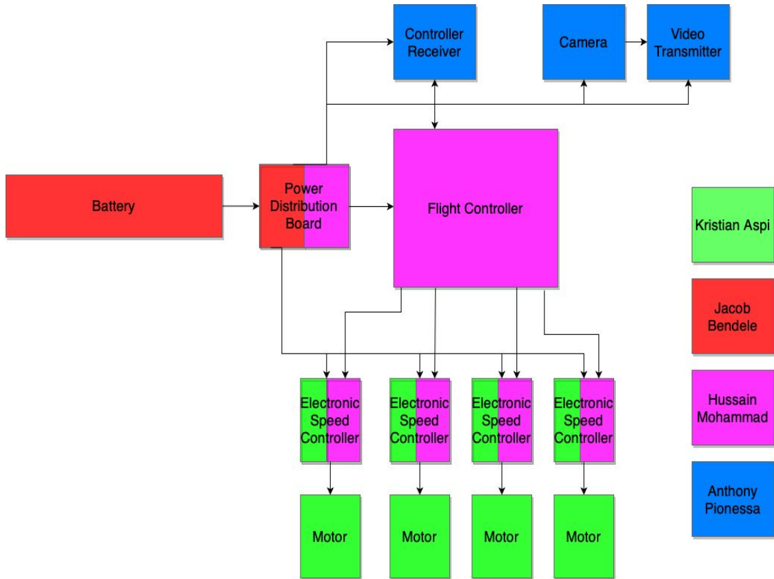
Figure 2.2: Hardware Block Diagram
