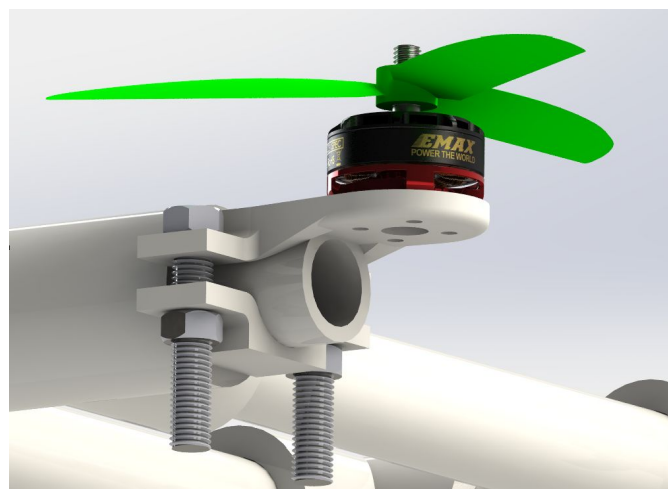
Figure 5.4: Motor Mount CAD
