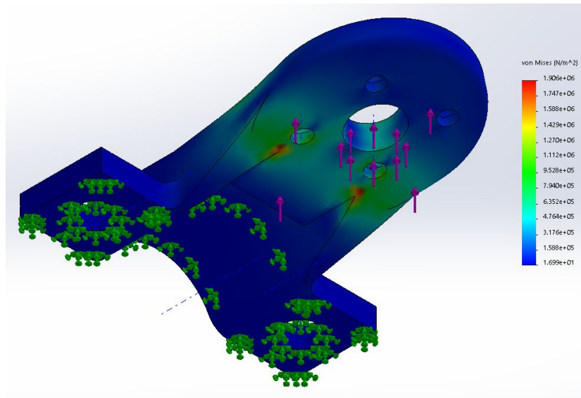
Figure 5.5: Stress Test Analysis
