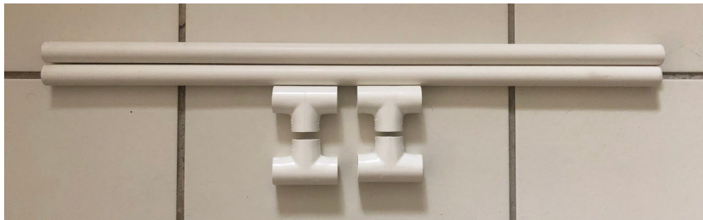
Figure 5.2: Two 2 Feet 1/2" Inch Sch 40 Pipes and 4 1/2"x1/2"x1/2" Tees
