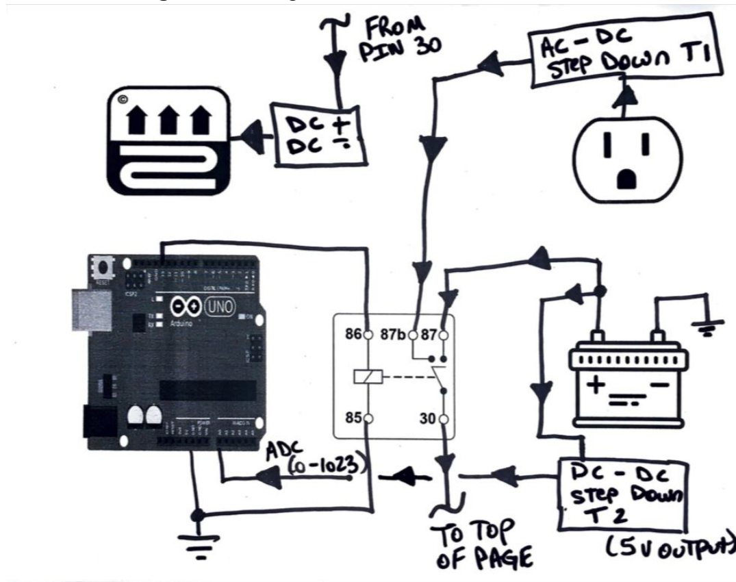
Figure 16 - Diagram of Power Outlet Connection
