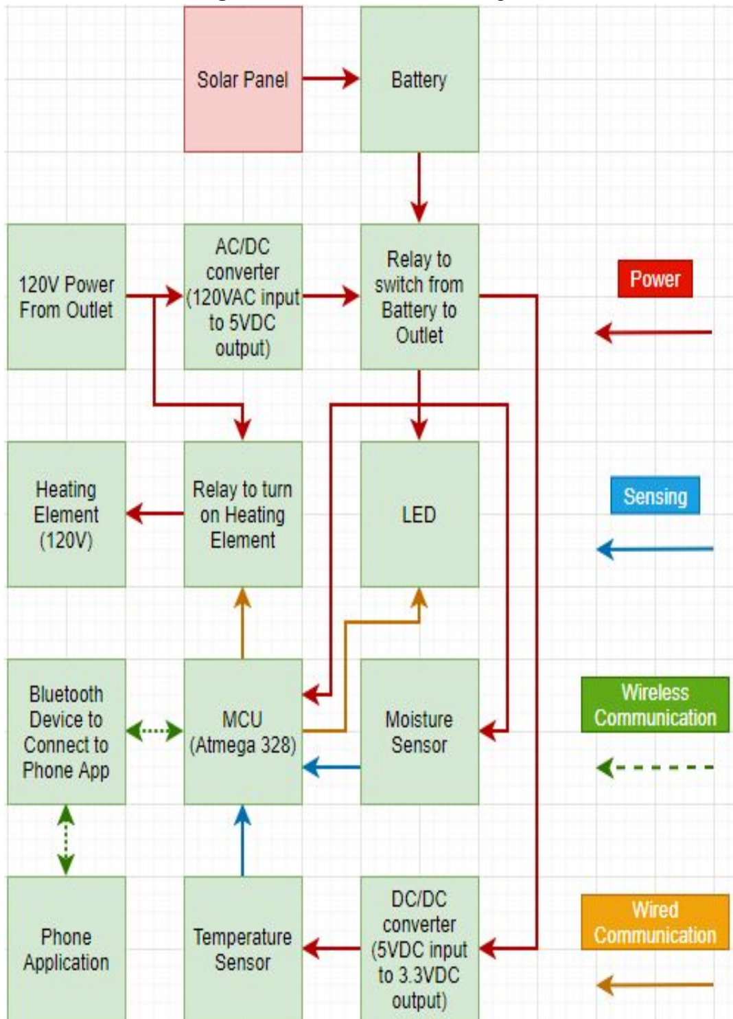
Figure 8 - Hardware Block Diagram
