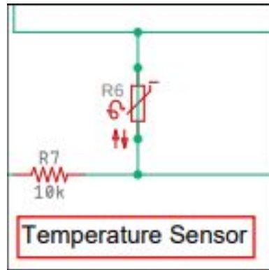
Figure 38 - Temperature Sensor Schematic Snip
