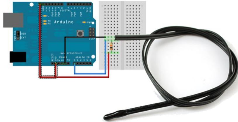
Figure 51 - Initial Temperature Sensor Testing Plan
