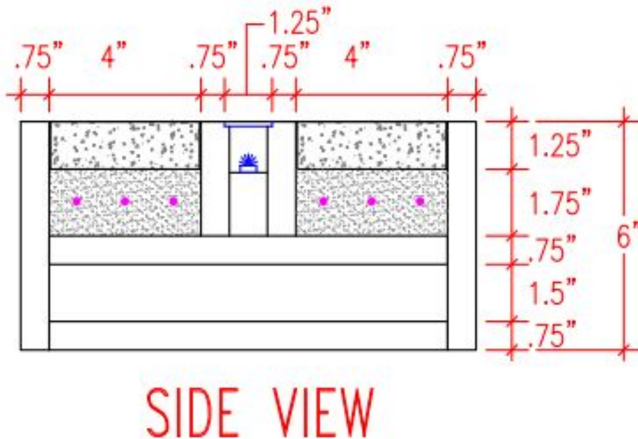
Figure 44 - Side View of Structure with Dimensions
