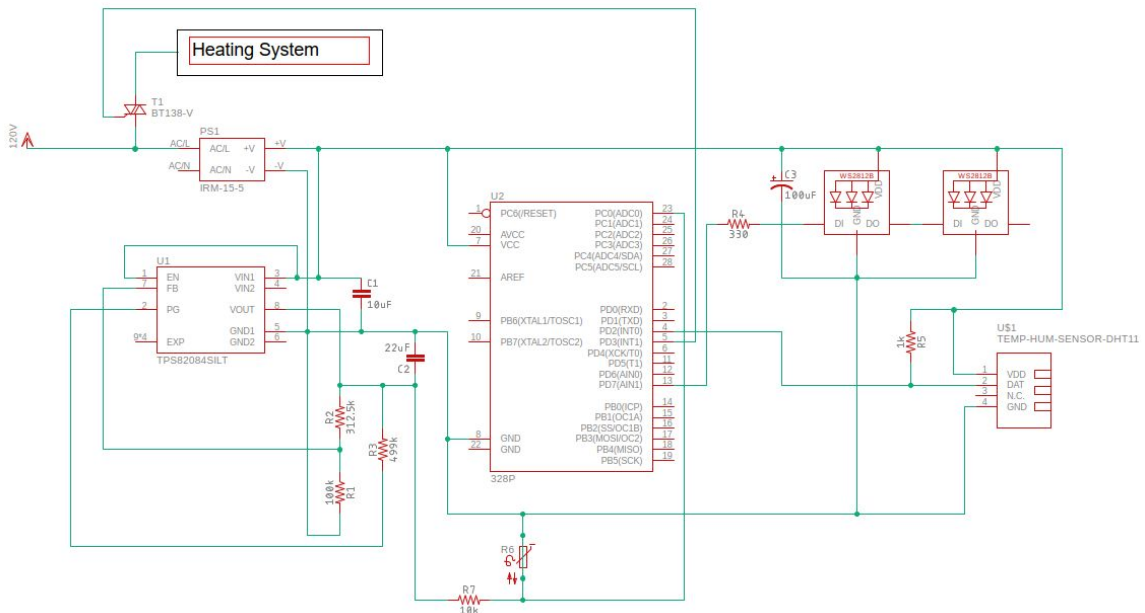
Figure 35 - Design Schematic
