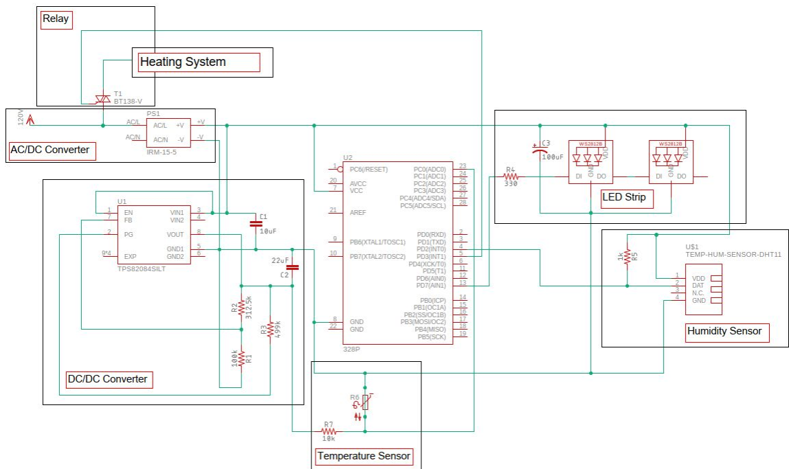
Figure 36 - Design Schematic with labels of areas
