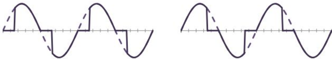
Figure 25 - Forward Phase dimming waveform (left) vs. Reverse Phase dimming waveform (right)
