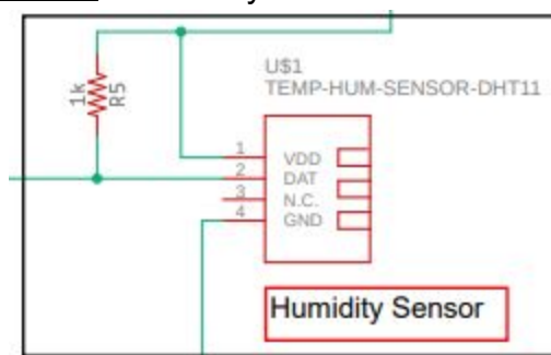
Figure 39 - Humidity Sensor Schematic Snip
