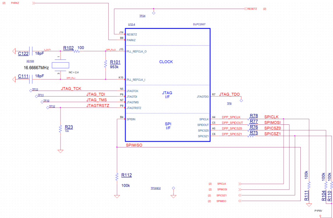
Figure 65 - DLPC2607 Serial Flash Interface
