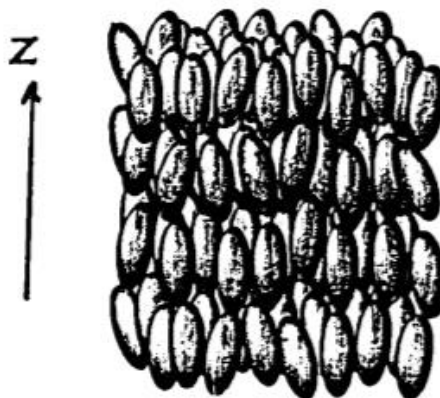
Figure 22 - Liquid crystal molecules aligned in the z-direction
