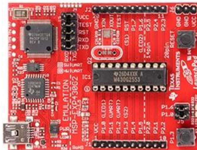
Figure 34 - MSP430G2553
