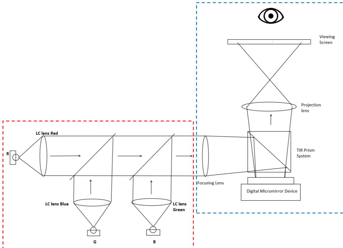
Figure 68 - Finalized Optical Setup Schematic. Pictured: Planned Illumination Setup (boxed in red) and simplified projection setup (boxed in blue)
