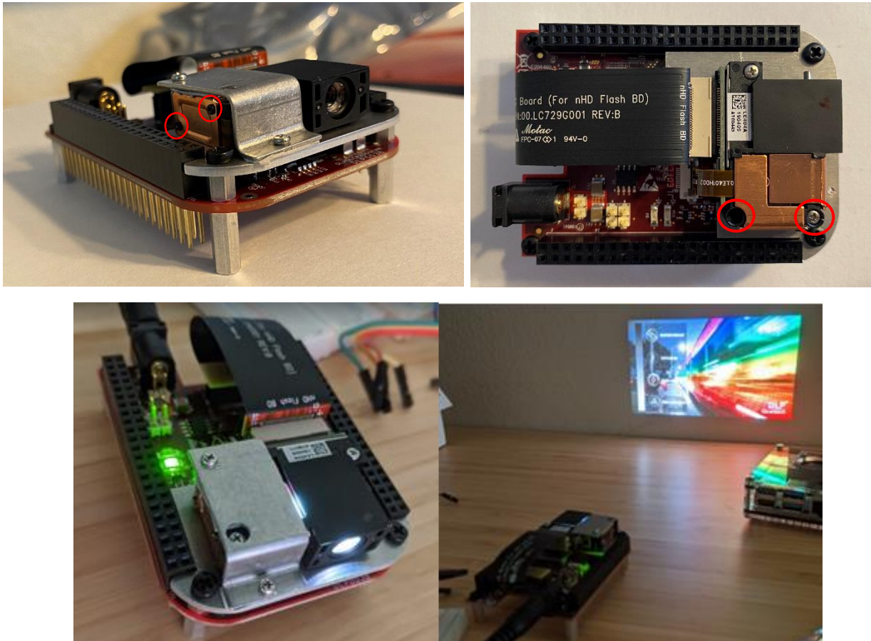
Figure 80 - Unboxed DLP2000 Optical engine and PCB. The top left image shows the module still having the silver heat sink on it; the top right image show the heat sink removed. Circled in red are the screws that need to be removed in order to expose the optics inside the engine. The bottom left and right images show the device plugged in and the EVM performing exactly as expected and promised by Texas Instruments.
