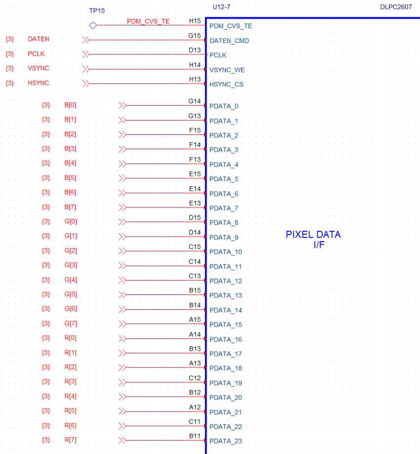
Figure 64 - DLPC2607 Data Interface
