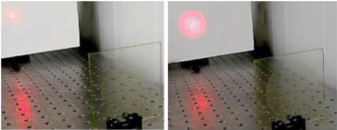
Figure 69 - Example of a LC diffractive lens. Both images are of the same laser and the same lens, but with different circular polarizations running through. It is easy, but critical to get the proper polarization passing through the system [51].
