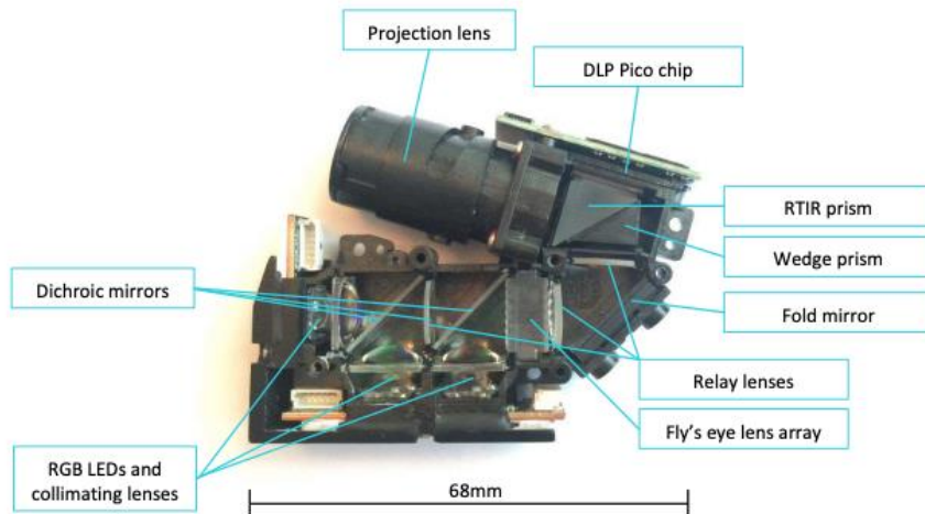
Figure 67 - Optical Components in an Example Pico Projection Optical Module taken from Texas Instruments [121].
