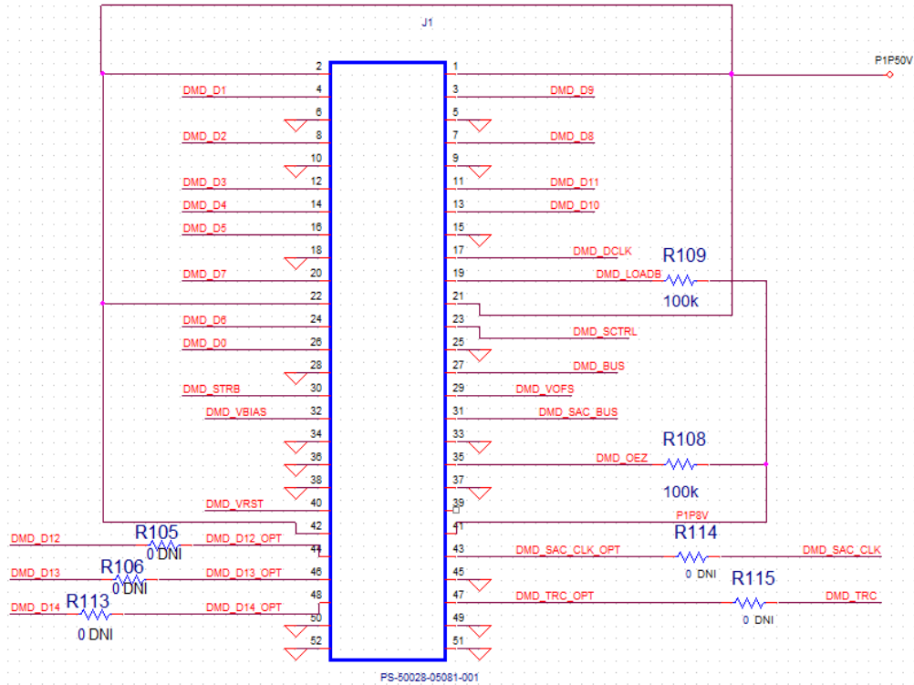
Figure 66 - DMD Flex Cable Connector.
