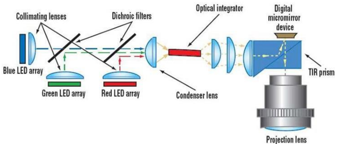
Figure 27: Generic Schematic for a DLP projector taken from ViewSonic. Note the system for combining Red, Green, and Blue light sources into one homogenized beam [58]
