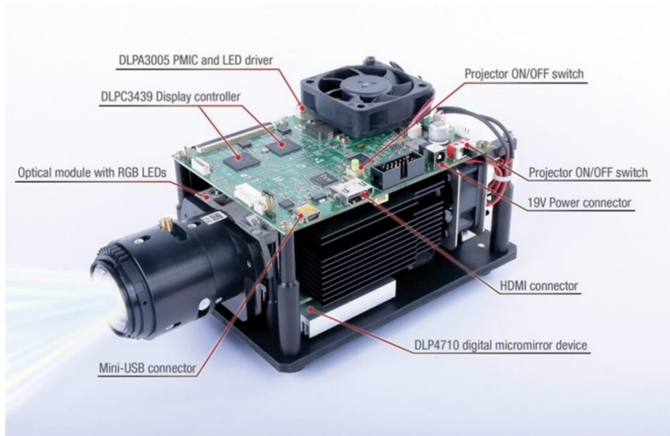
Figure 32 Texas instruments DLP4710 Evaluation Module
