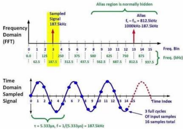
Figure 50 - FFT – Different Input Frequency
