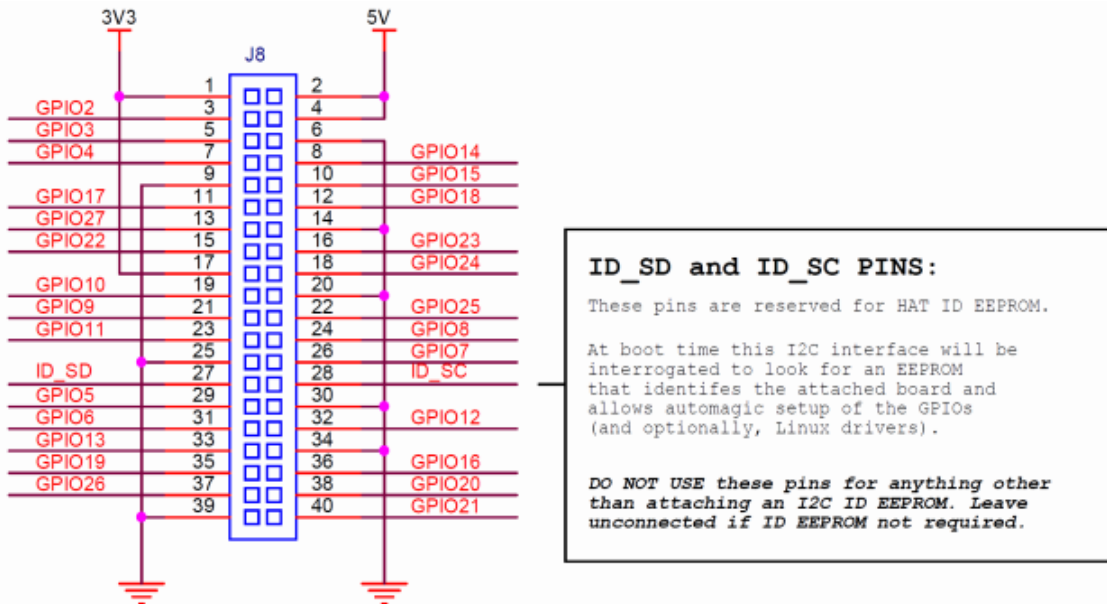
Figure 39 - GPIO Connector Pinout for Raspberry Pi 4
