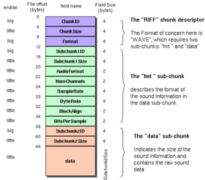
Figure 49 - The Canonical WAVE File Format
