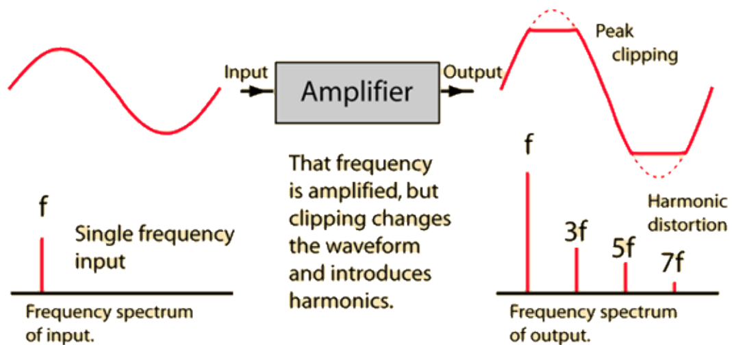
Figure 70: Harmonic Distortion is when the waveforms are clipped, having the sound be off tone
