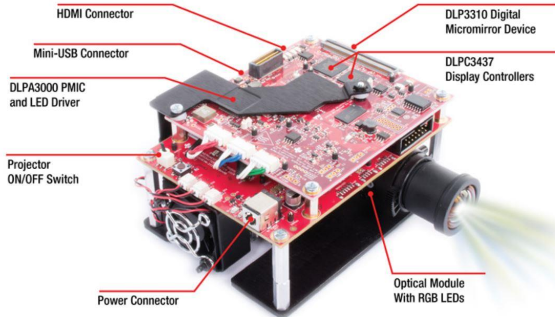
Figure 31 Texas Instruments DLP3310 Evaluation Module
