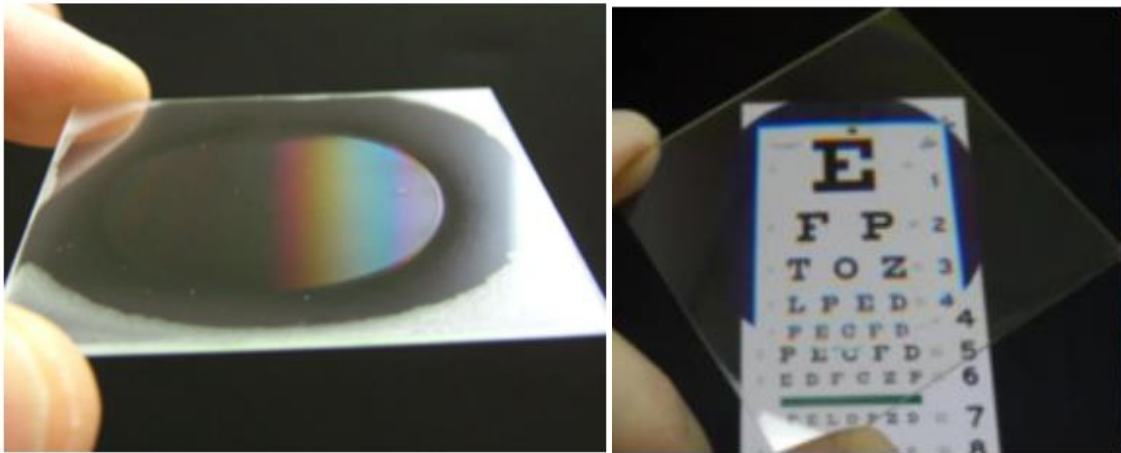
Figure 23 - Actual diffractive waveplate lens made from liquid crystal polymer, produced locally by BEAM Engineering Co. in Orlando, FL [51]
