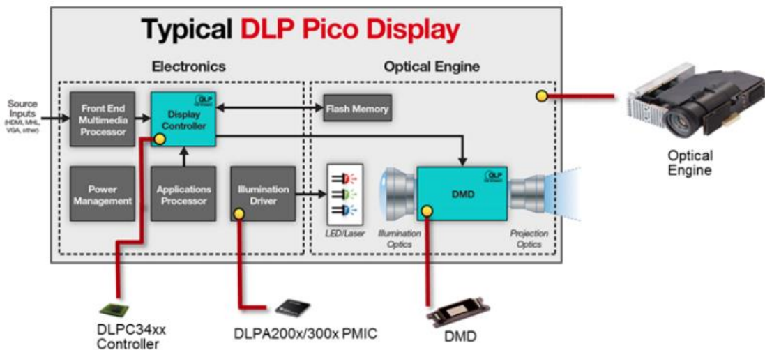
Figure 62 - Typical DLP™ Pico System Block Diagram
