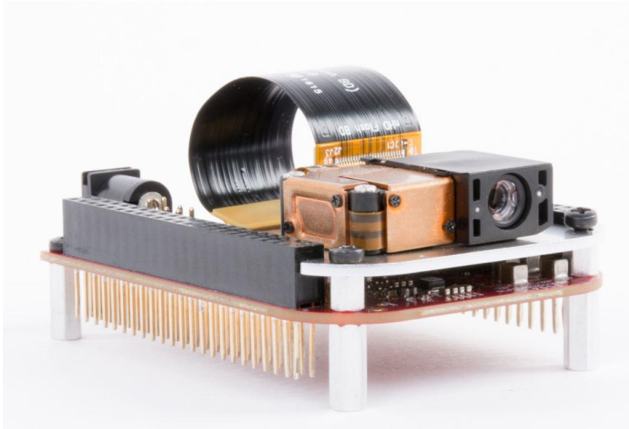
Figure 29 Texas instruments DLP2000 Evaluation Module
