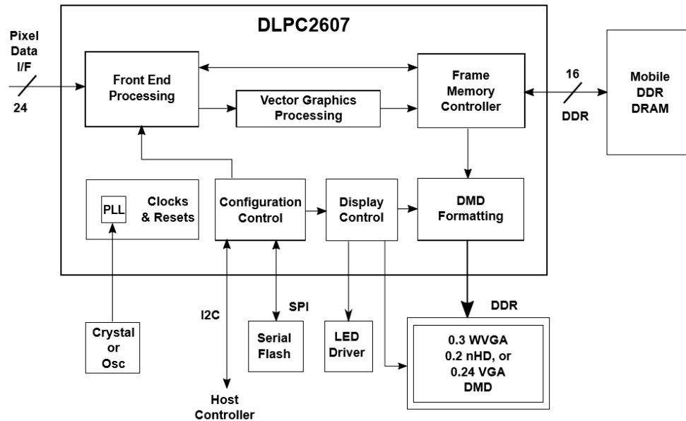
Figure 63: DLPC2607 Block Diagram showing internal processing and input and output functionality
