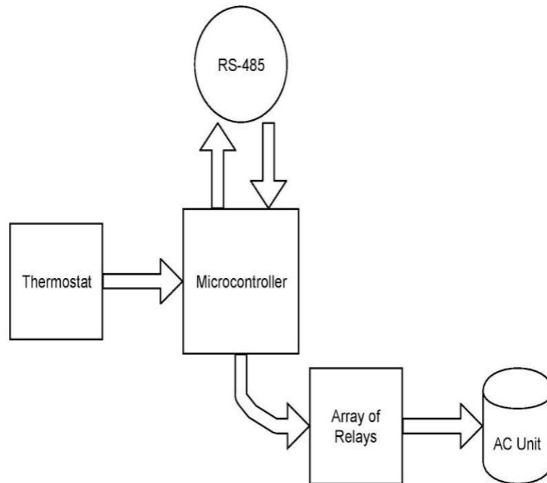
Figure 61 Third Subsystem (Thermostat Board) Block Diagram
