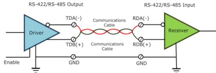
Figure 27 RS-485 Protocol (Courtesy of BB SmartWorks)
