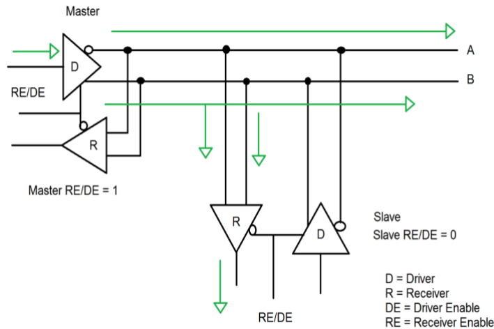
Figure 29 RS-485 Driver and Receiver Data Flow Diagram 2 (Courtesy of BB SmartWorks)
