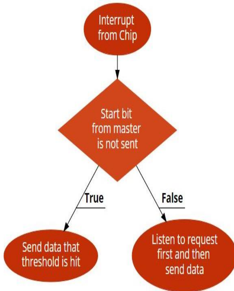
Figure 41 Interrupt Diagram
