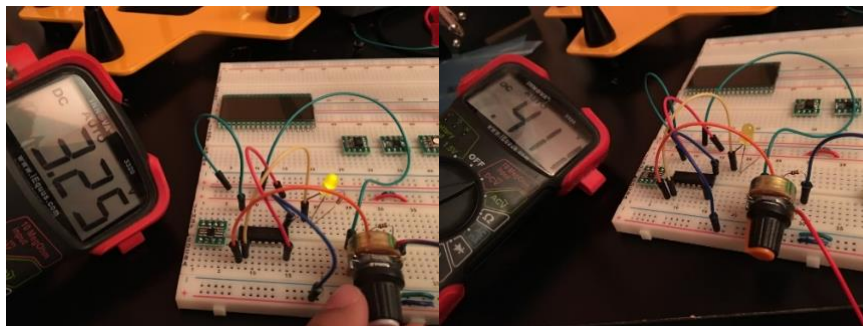
Figure 78 Potentiometer Testing
