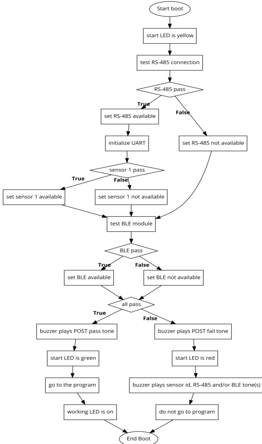
Figure 69 POST Sequence Flow Diagram
