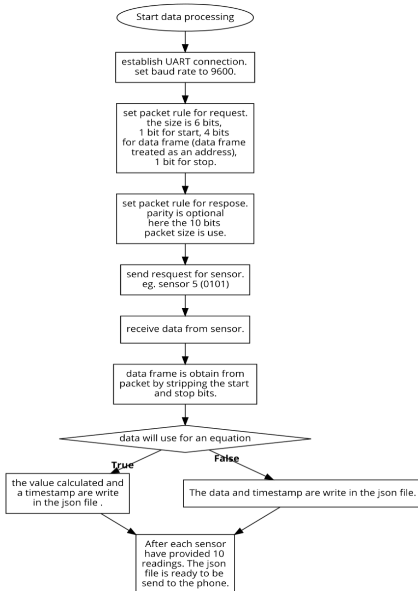
Figure 67 Main MCU Flow Chart Part 1
