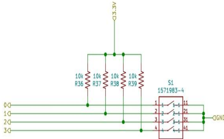
Figure 63 Third Subsystem (Thermostat Board) Schematic Part 2
