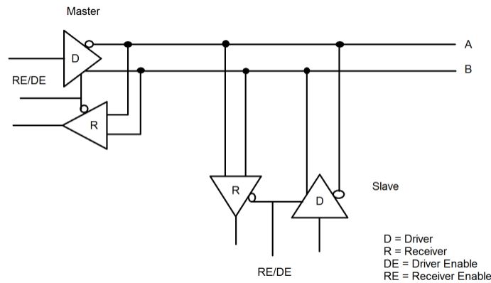
Figure 28 RS-485 Driver and Receiver Data Flow Diagram 1 (Courtesy of BB SmartWorks)
