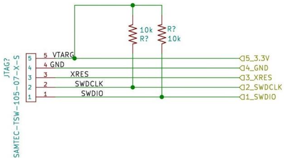
Figure 53 First Subsystem (Main Board) Schematic Part 4
