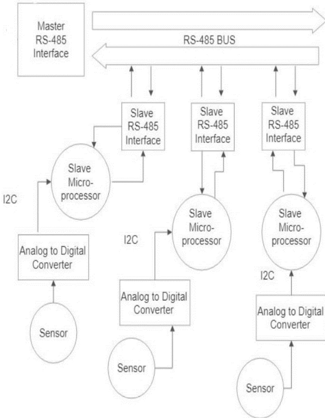
Figure 55 Second Subsystem (Sensors Board) Block Diagram
