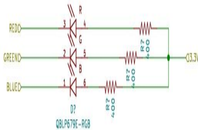
Figure 64 Third Subsystem (Thermostat Board) Schematic Part 3
