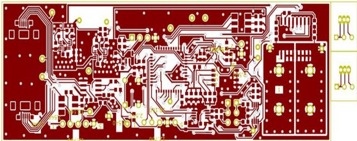
Figure 72 Main Board PCB
