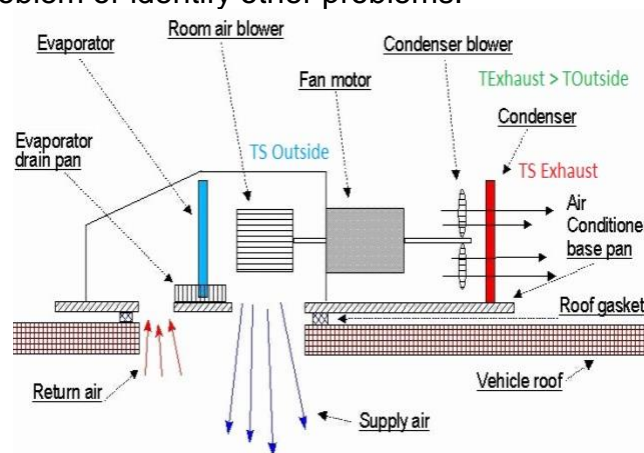
Figure 17 Other Points of AC Compressor Airflow (Courtesy of Bryant RV Services)
