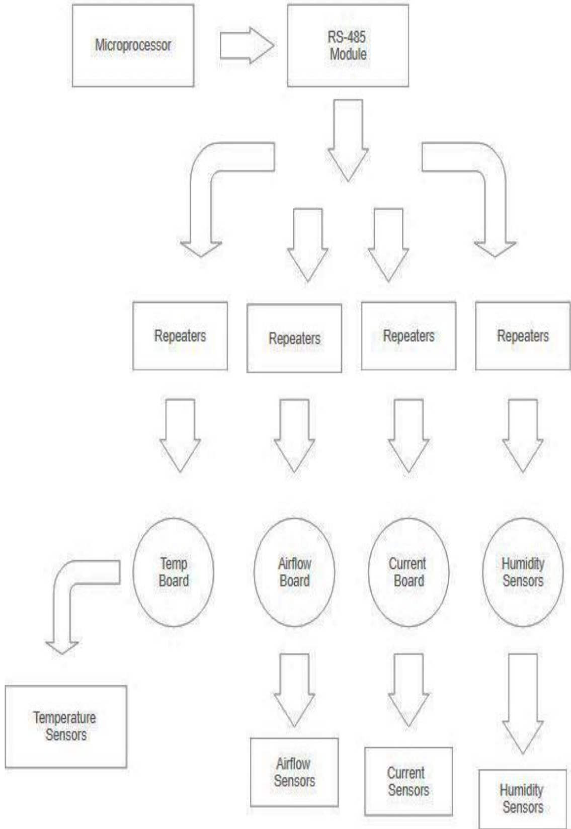
Figure 34 Sensors Flow Diagram
