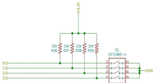
Figure 58 Second Subsystem (Sensor Board) Schematic Part 3
