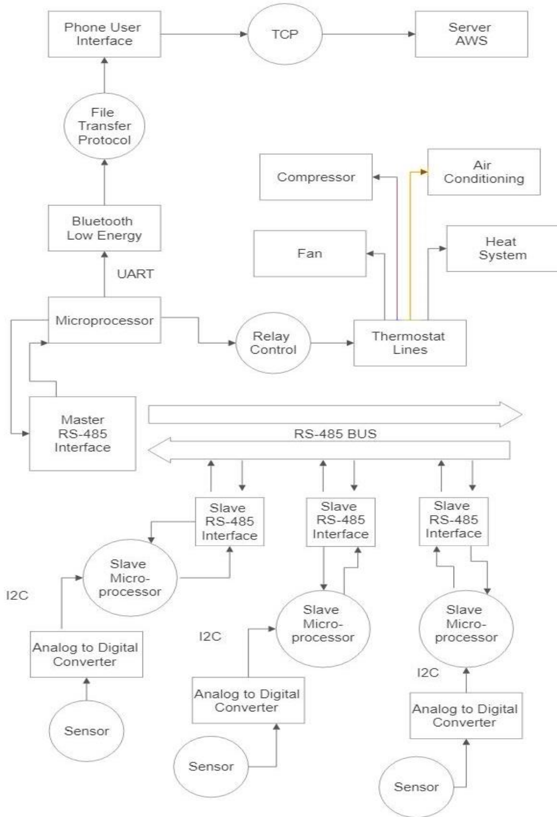
Figure 39 System Data Flow Diagram
