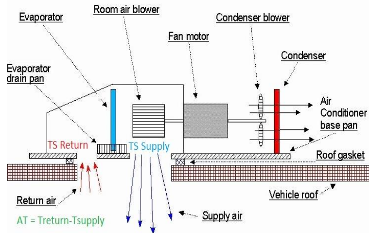
Figure 16 AC Compressor Airflow (Courtesy of Bryant RV Services)
