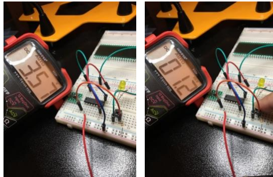
Figure 77 Hex Voltage Level Shifter Test
