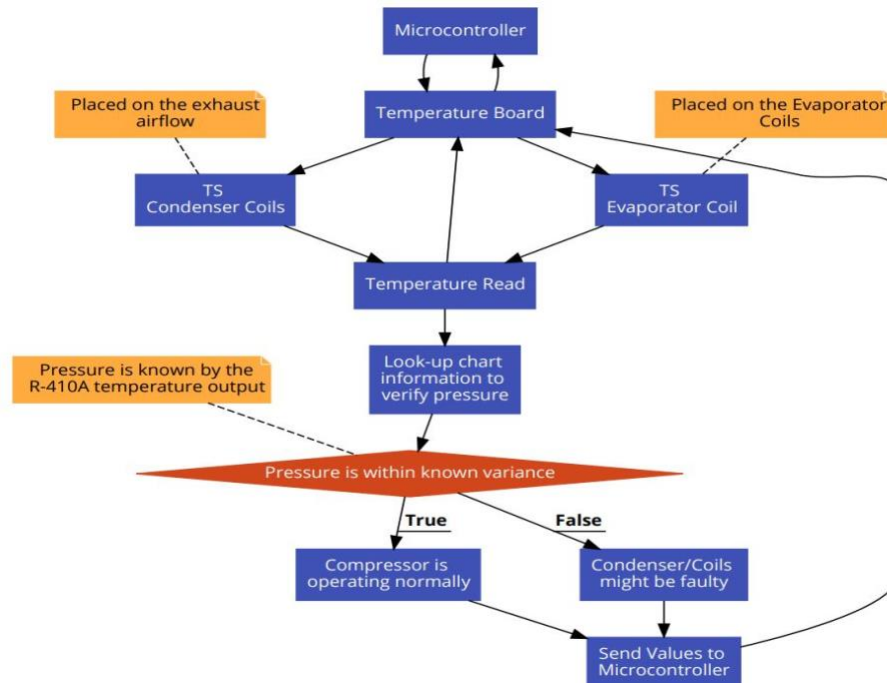
Figure 20 MCU Lookup Flow Diagram
