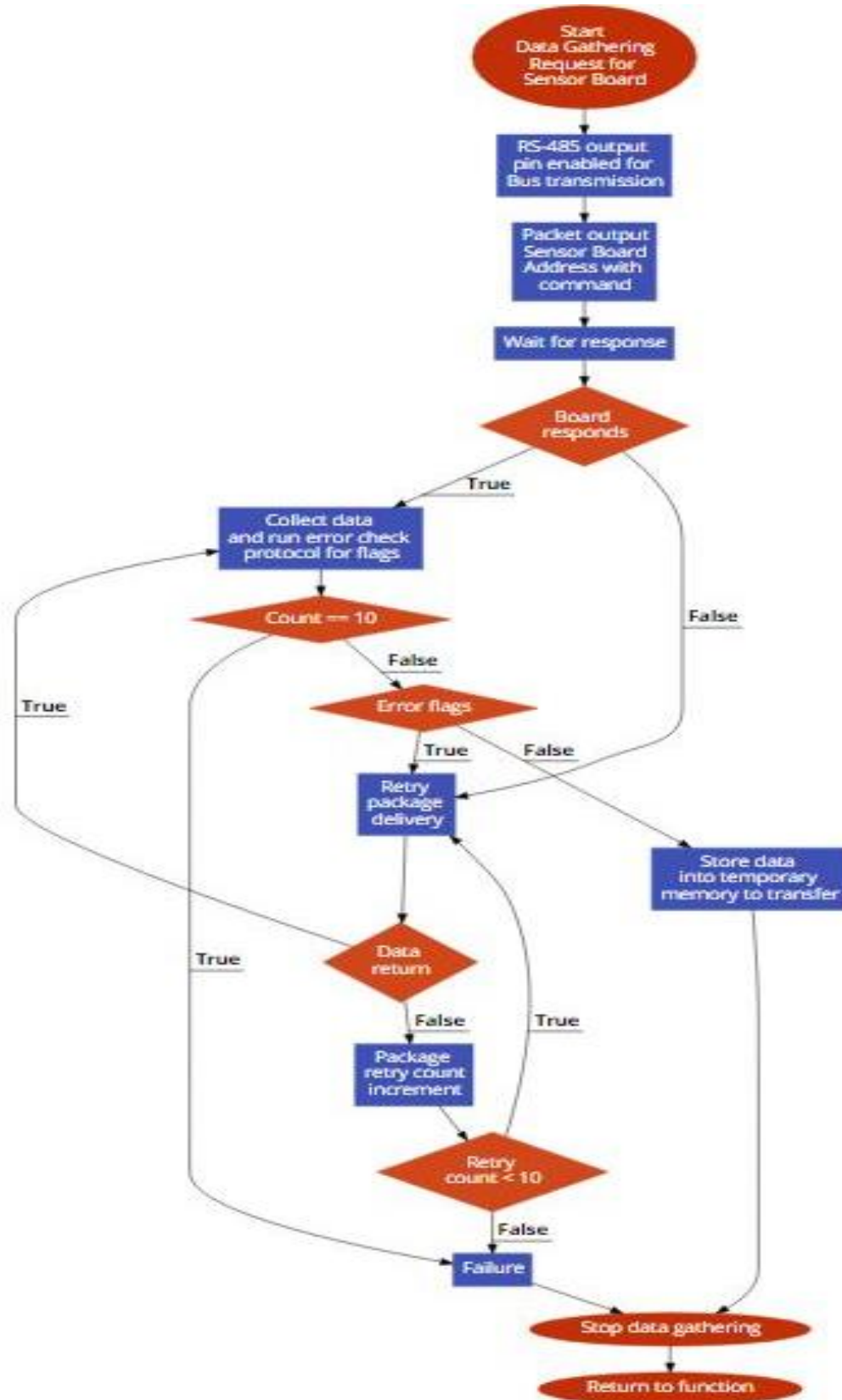
Figure 42 Sensor Data Bits Flow Diagram
