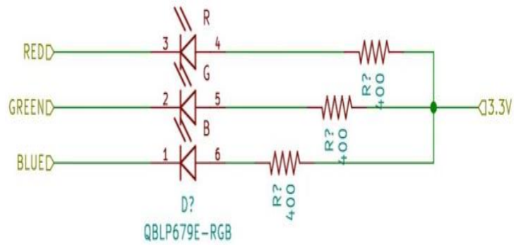
Figure 51 First Subsystem (Main Board) Schematic Part 2
