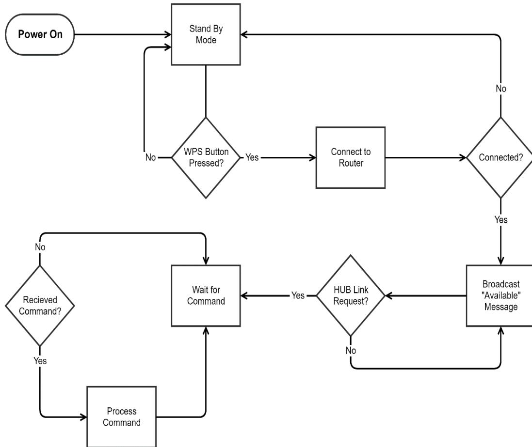
Figure 30. Software Process
