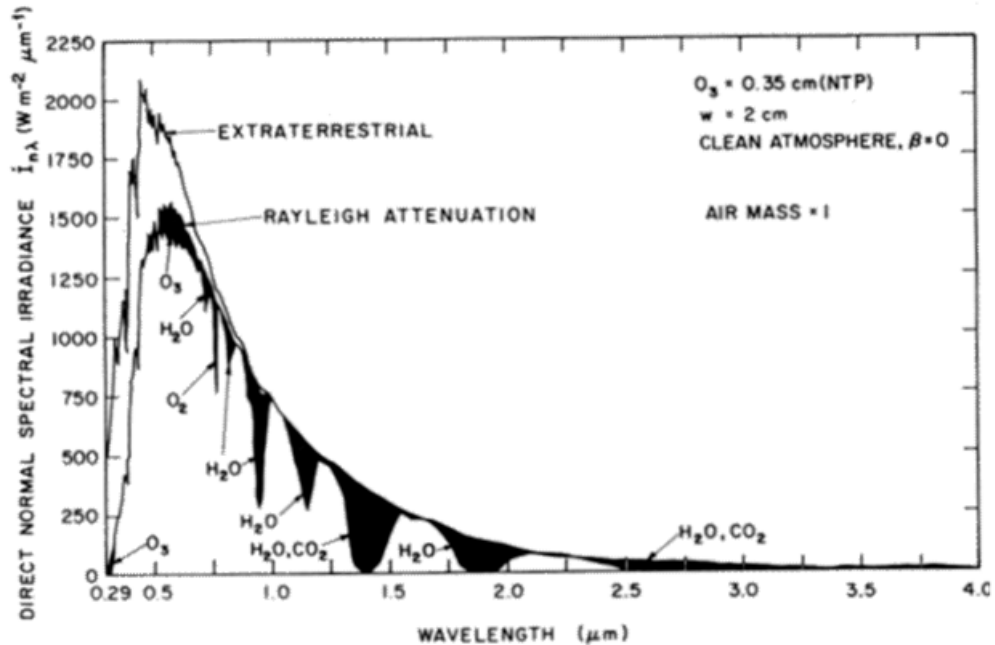
Figure 14. Transmission Spectrum of the Sun
