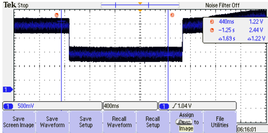
Figure 83. AC Response to Light source
