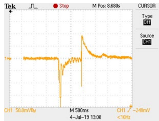
Figure 78. NIR Sensor AC Response at 60 Inches
