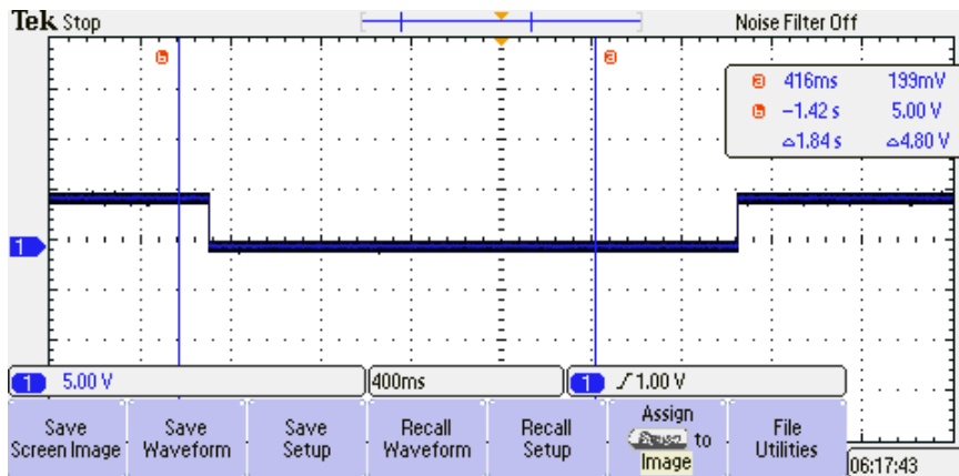
Figure 84. DC Response of NIR Sensor with Tuned Potentiometer
