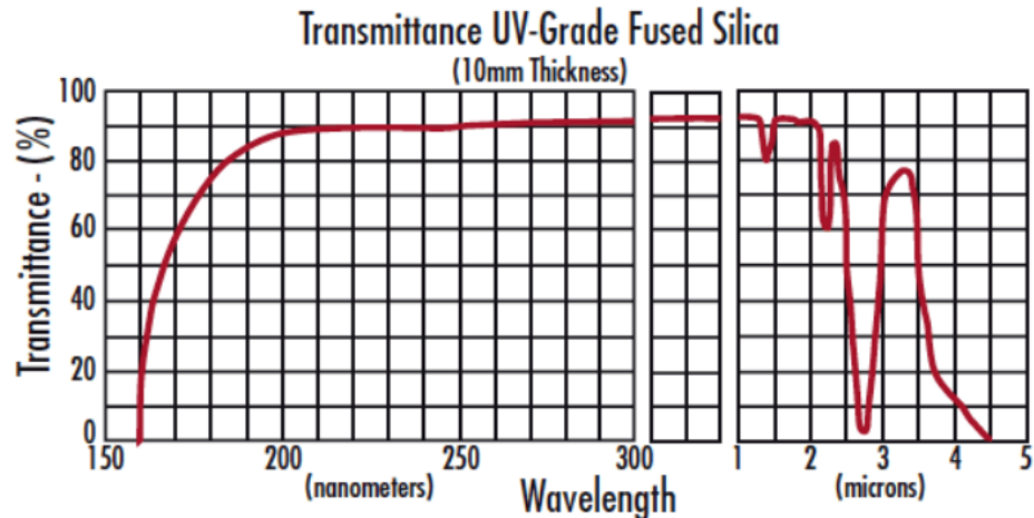
Figure 90. Transmission Spectrum of Fused Silica
