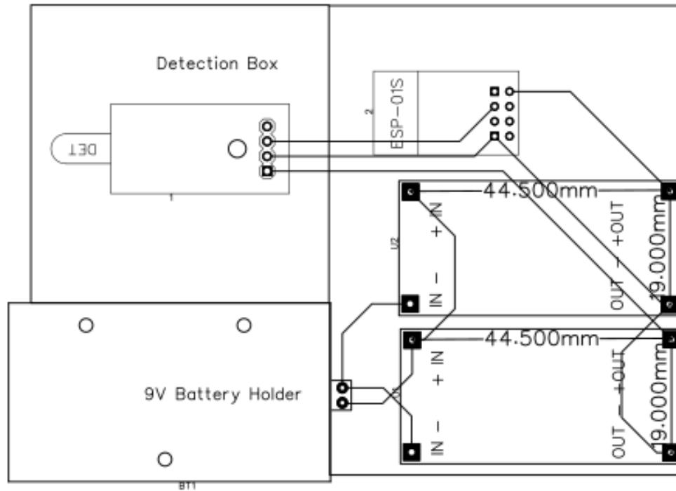
Figure 28. Fire Detector PCB Mockup
