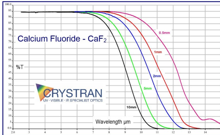
Figure 10. Transmission Spectrum of Calcium Fluoride
