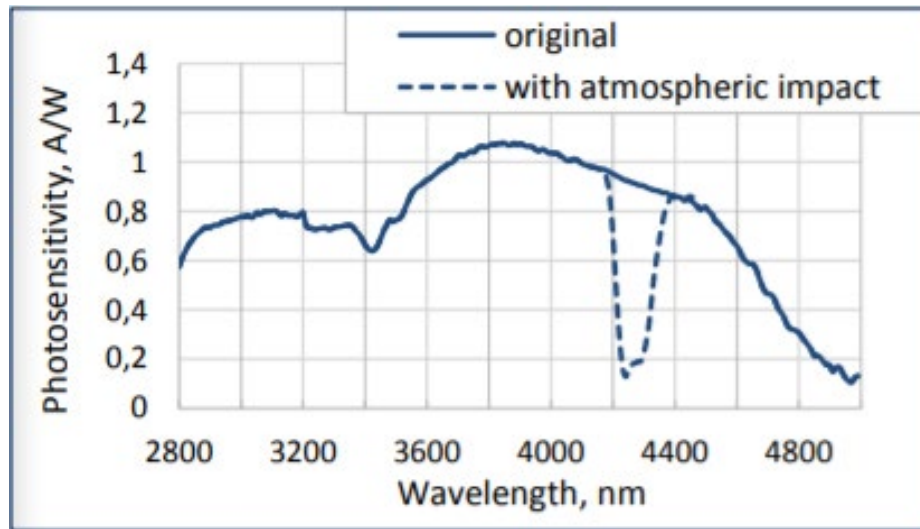
Figure 91. Lms49PD-05 Series Spectral Response of Operational Bandwidth
