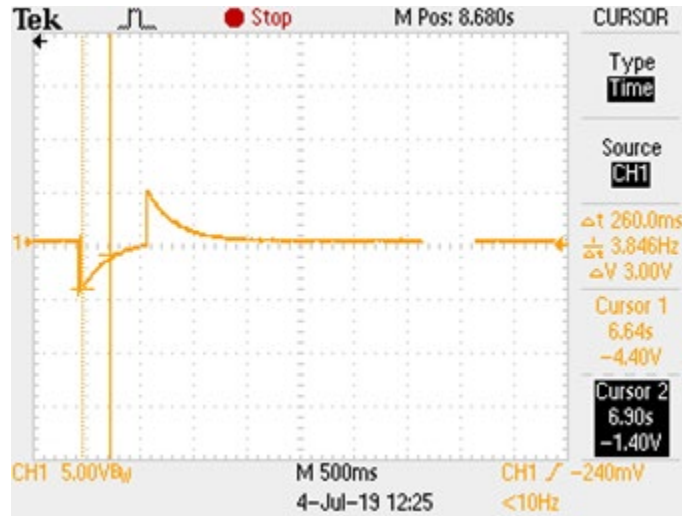
Figure 75. NIR Sensor DC Response Rise/Fall Time
