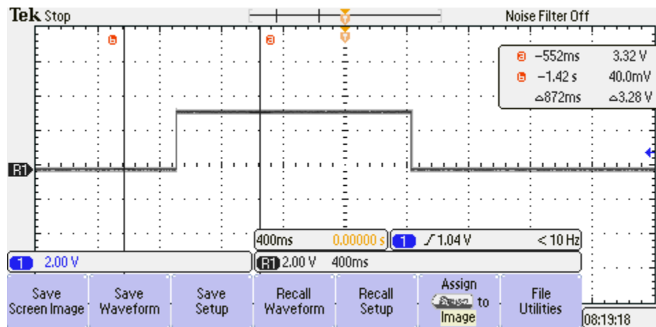
Figure 87. PIR Sensor Output Voltage with Adjusted Potentiometer
