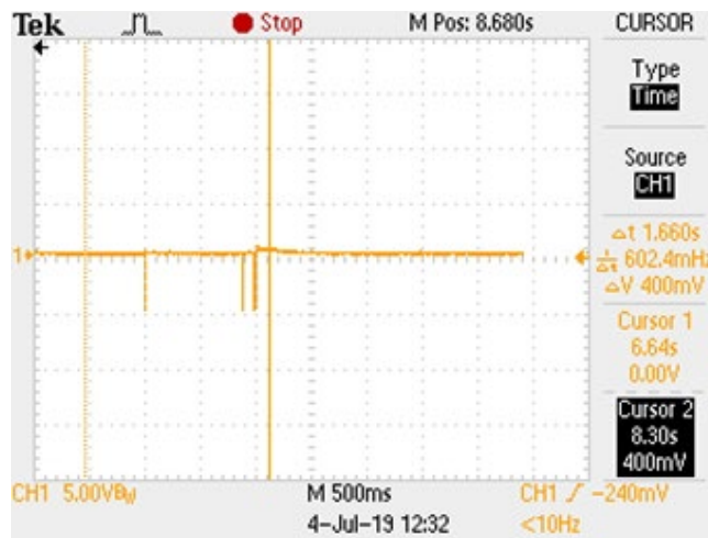
Figure 76. NIR Sensor DC Response for FOV Edge Detection
