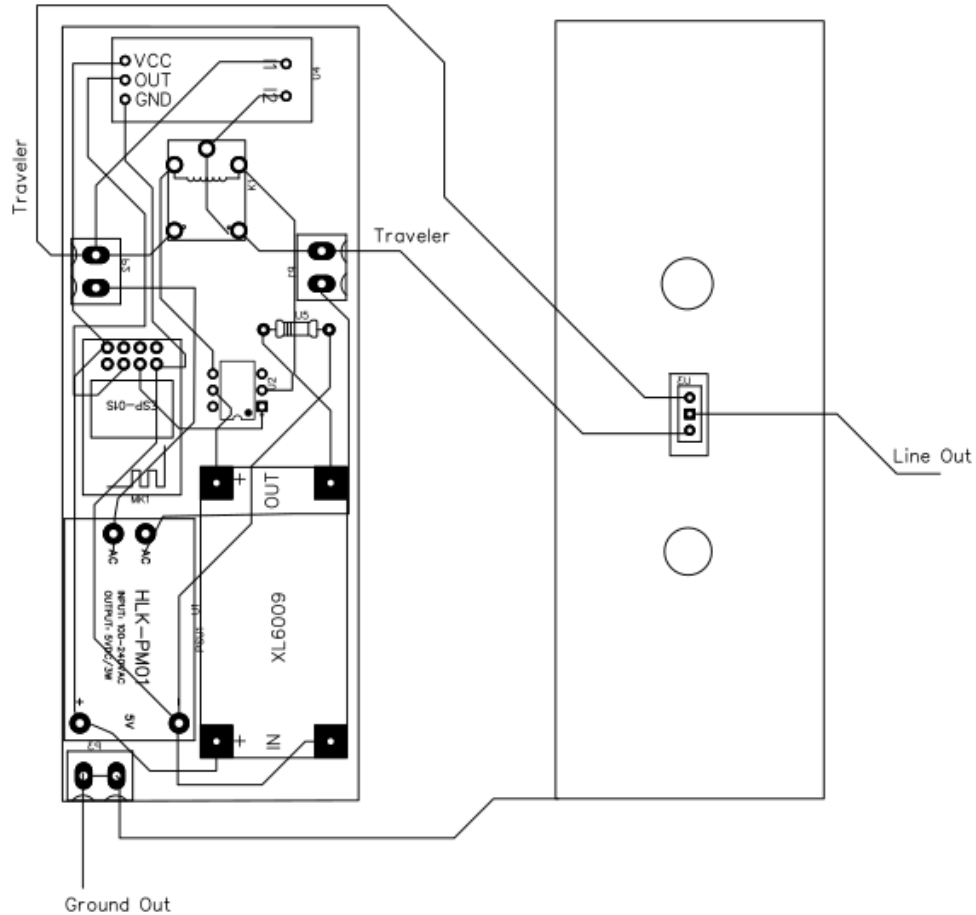
Figure 25. Smart Switch PCB Mock Layout
