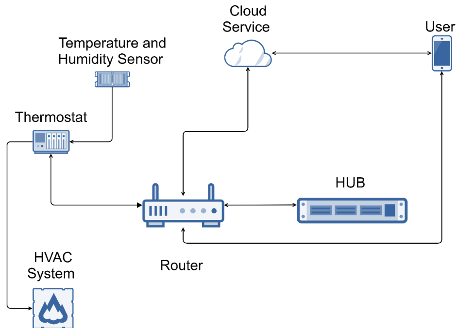
Figure 32. System Diagram
