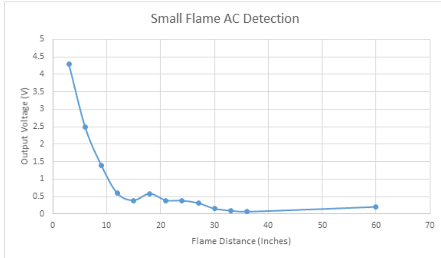
Figure 73. Small Flame Detection AC Output Without Lens Present
