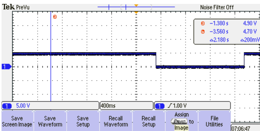
Figure 86. DC Output Response of NIR Sensor for Heated Quartz
