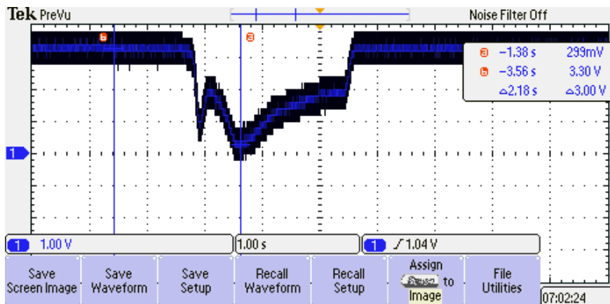
Figure 85. AC Output Response of NIR Sensor for Heated Quartz
