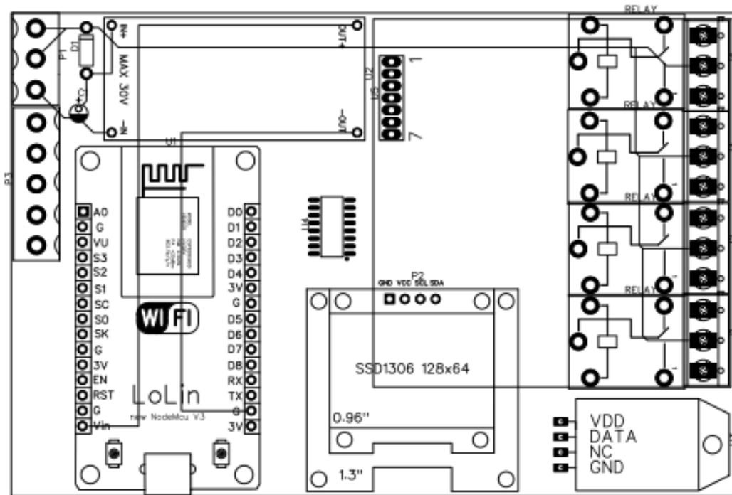
Figure 21. Smart Thermostat PCB Layout Mockup
