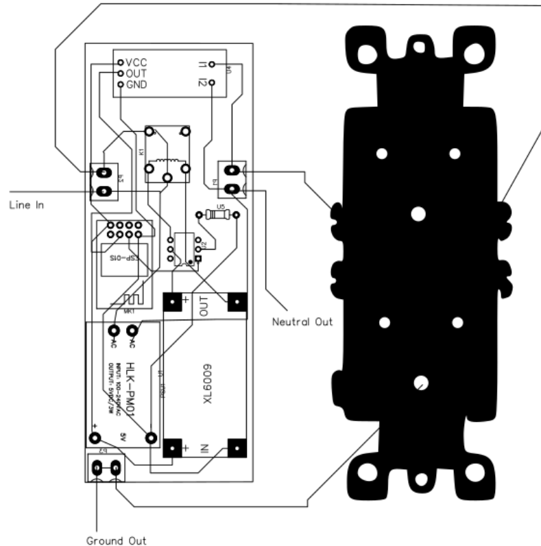
Figure 23. Smart Outlet PCB Layout Mockup
