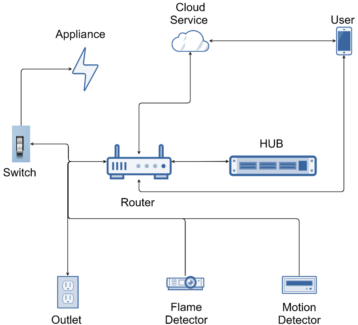
Figure 29. Function Diagram
