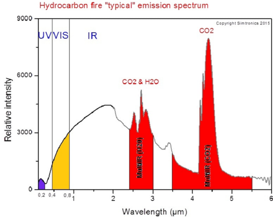
Figure 13. Blackbody Emission Spectrum of “Typical” Hydrocarbon Fire
