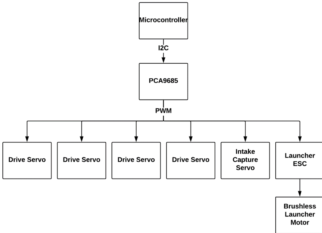
Figure 19 Control signal block diagram
