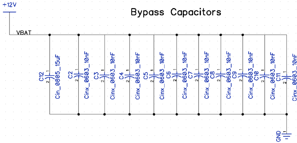
Figure 22: Bypass Capacitors for 6.8V-6A DC-DC Converter
