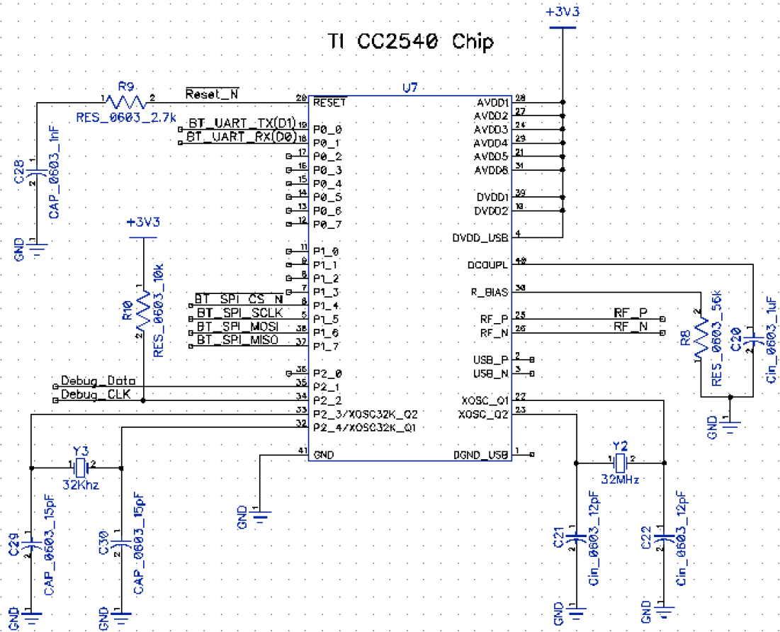
Figure 29 Bluetooth IC and Schematic
