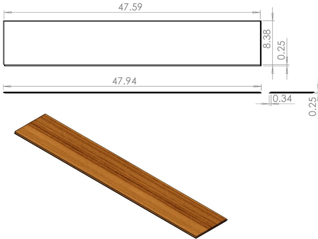
Figure 44 Plank drawing
