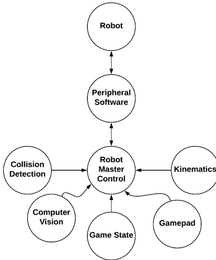
Figure 61 Robot master control data flow
