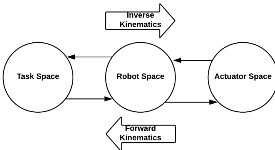
Figure 60 Kinematic Transforms
