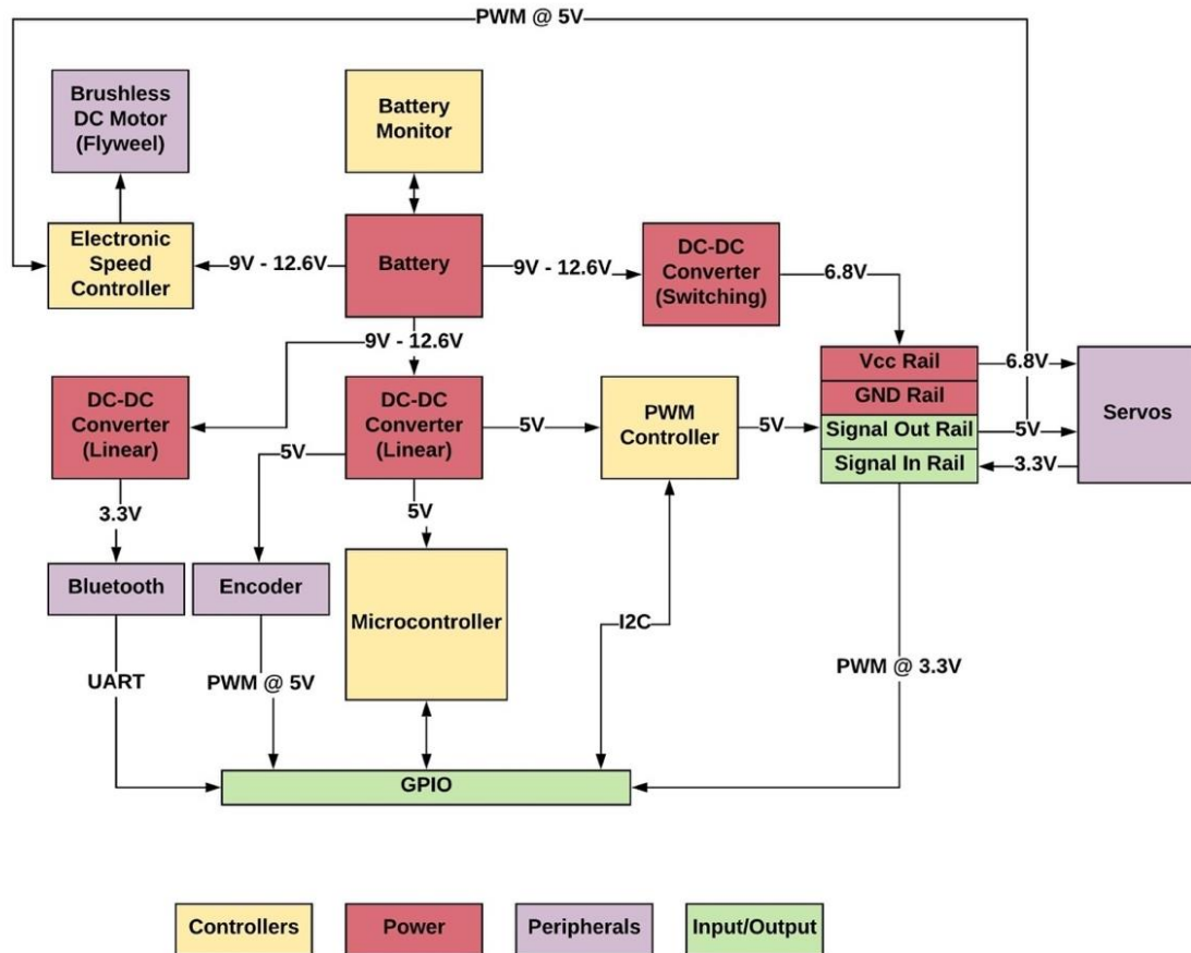
Figure 25 Robot Electrical Network Block Diagram
