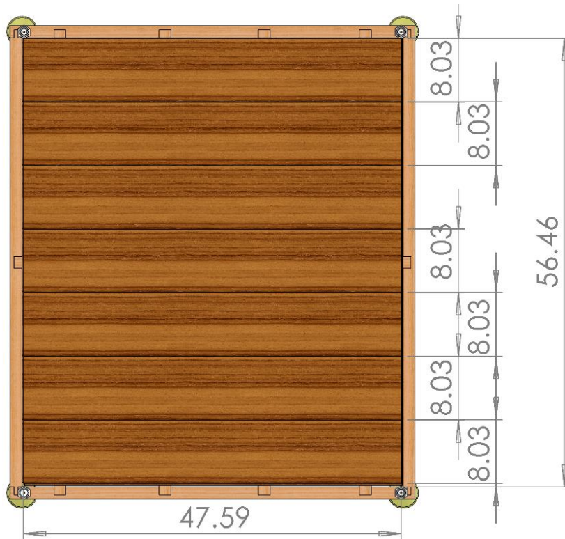
Figure 45 Court Floor panels
