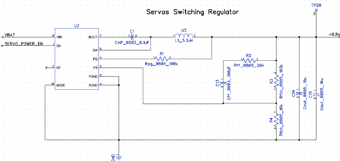
Figure 23: Schematic for 6.8V-6A DC-DC Converter IC
