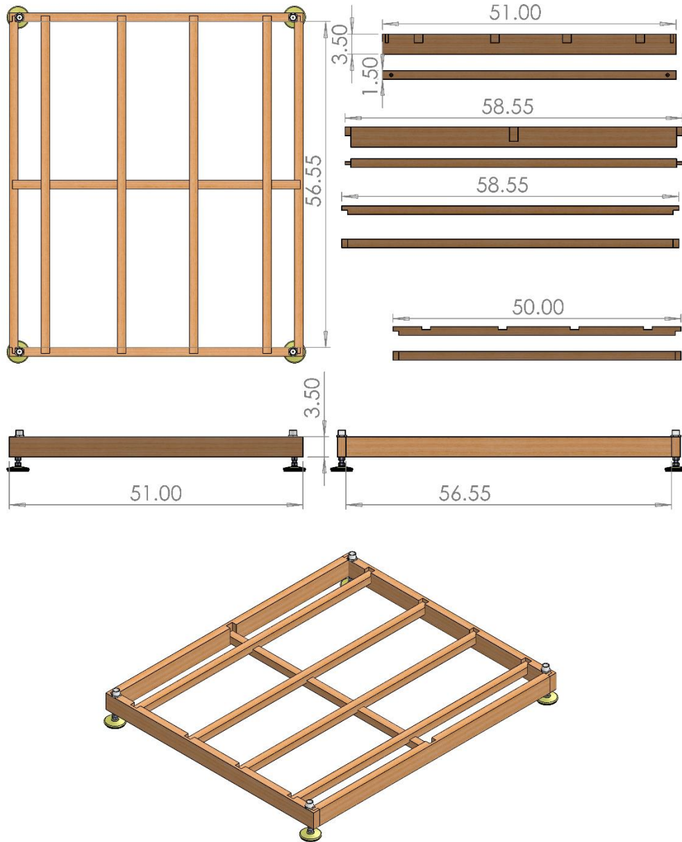
Figure 40 Arena frame drawings
