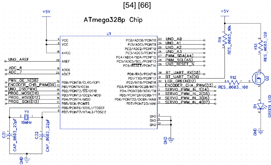
Figure 26: ATmega328P Microcontroller Schematic
