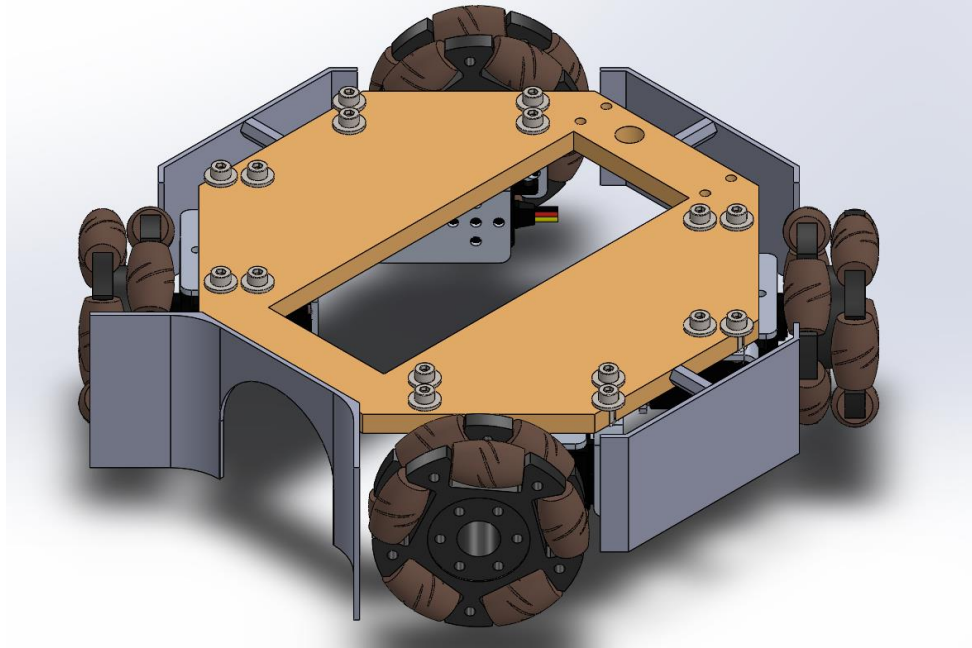
Figure 62 Ball-Prevention plates & cut-outs
