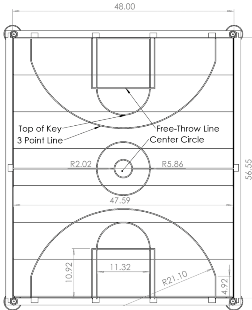
Figure 46 Court markings
