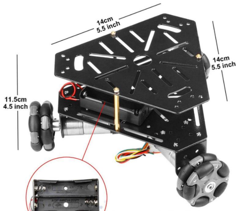
Figure 8 Example Omni-wheel base Permission from Heneng shown in Figure 68
