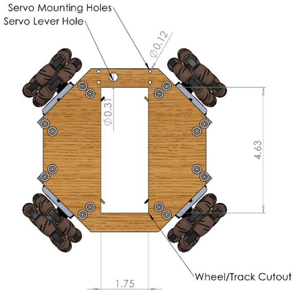
Figure 63 Base-Launcher Integration
