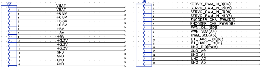
Figure 27: ATmega328P GPIO Connection and additional power rails for testing
