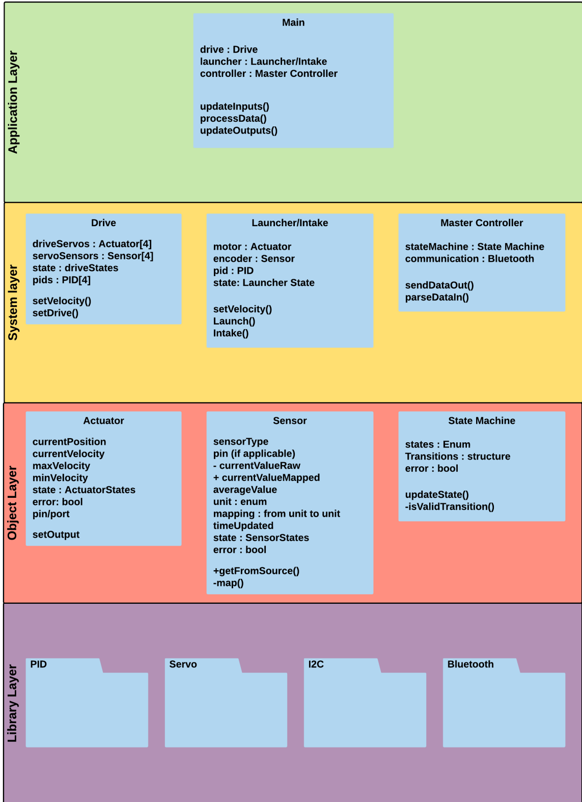
Figure 37 Robot software architecture design and class diagrams
