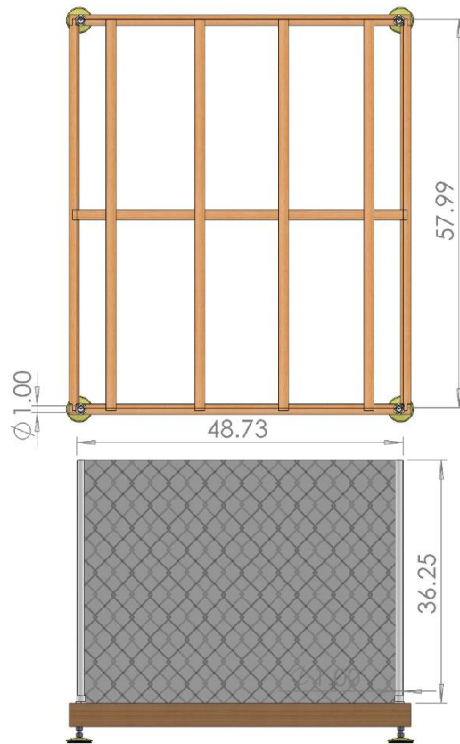
Figure 41 Mesh walls attached to PVC uprights
