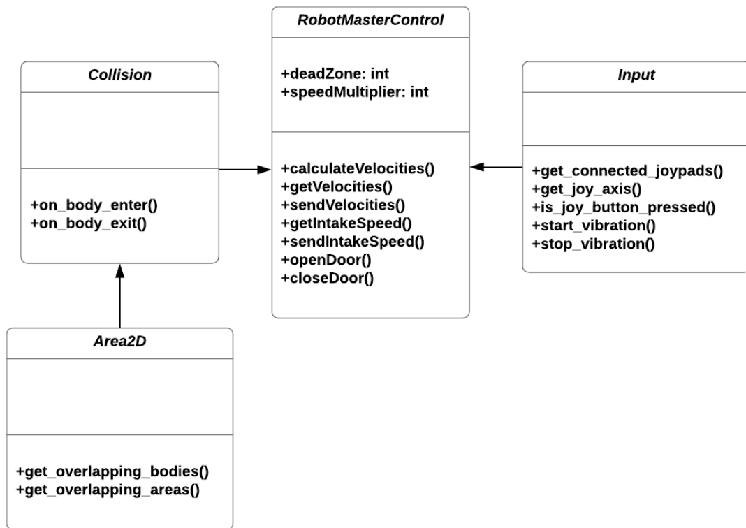
Figure 59 Basic Class Diagram for Movement and Collision Detection
