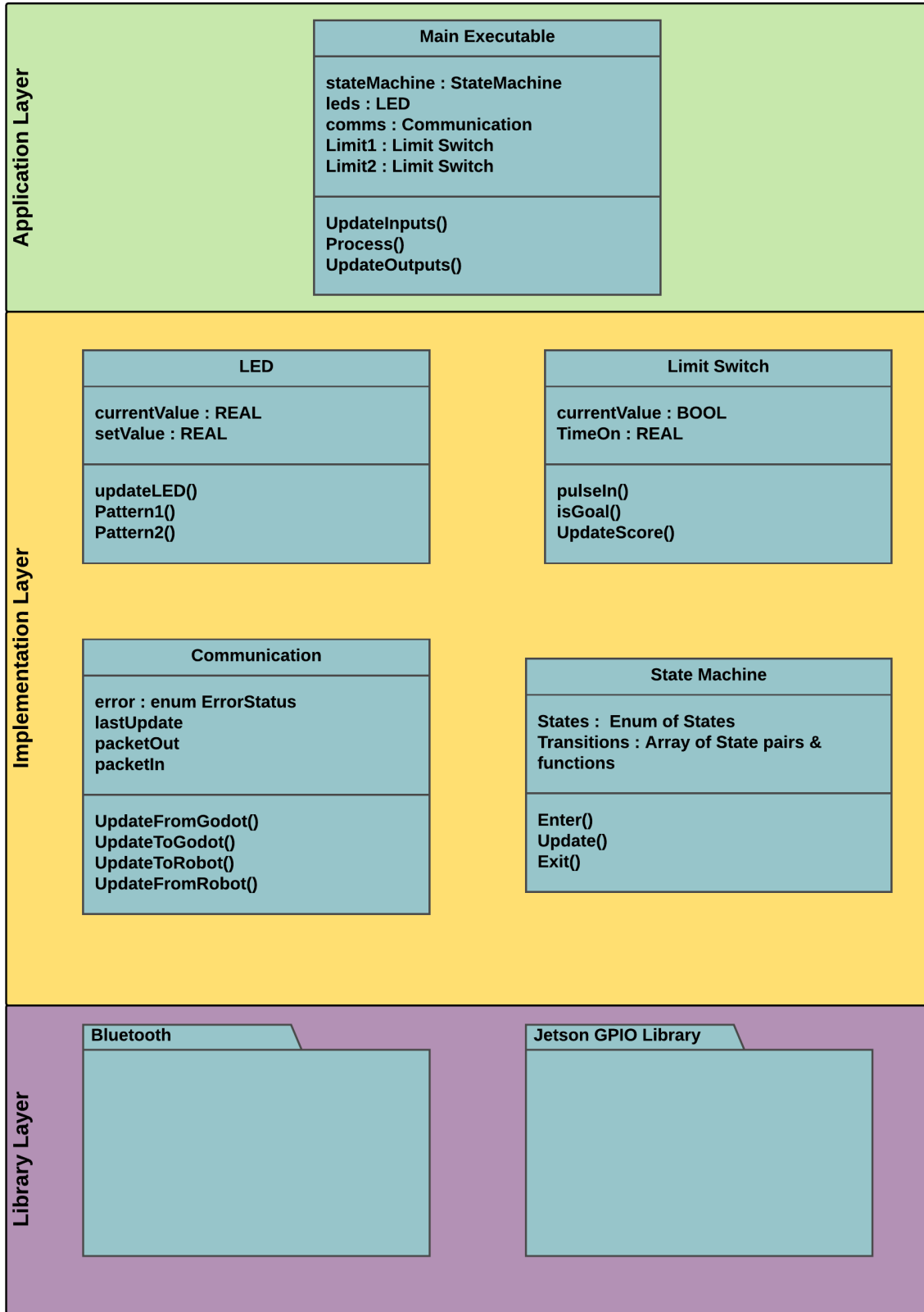
Figure 55 Peripheral software Architecture and class diagram
