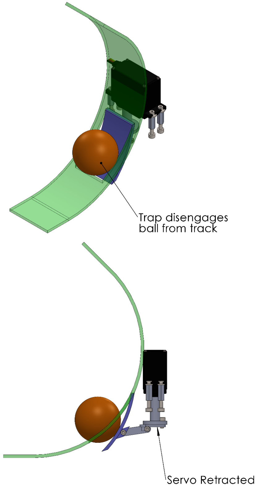
Figure 17 Ball-Trap interaction drawing
