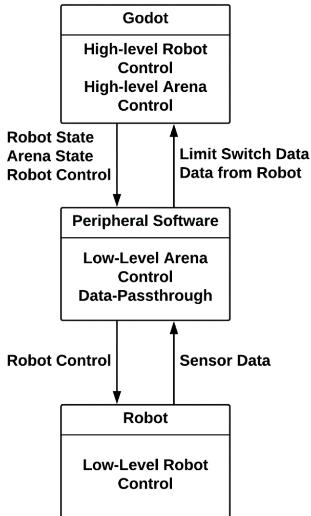
Figure 54 Peripheral Software Communication Diagram
