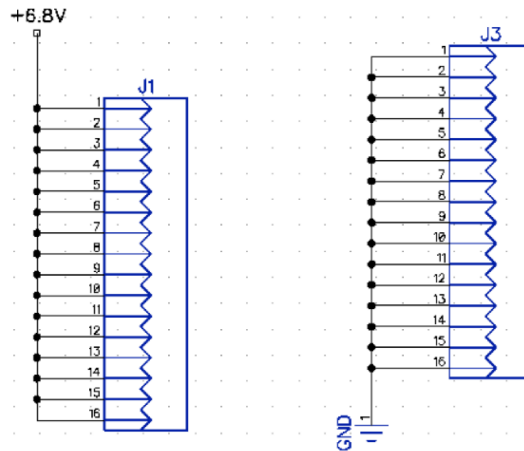
Figure 32 GPIO pins for Servo connections to the PCB
