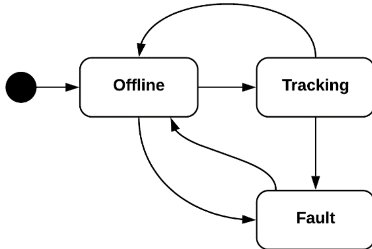
Figure 35 Actuator State Machine
