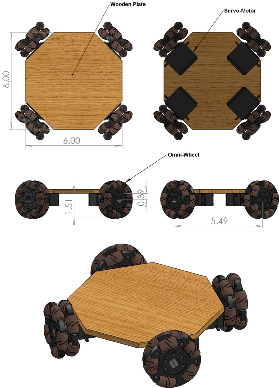
Figure 13 Robot Base Design
