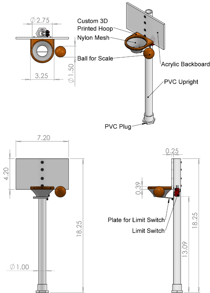
Figure 48 Hoop & Mounting SOLIDWORKS design
