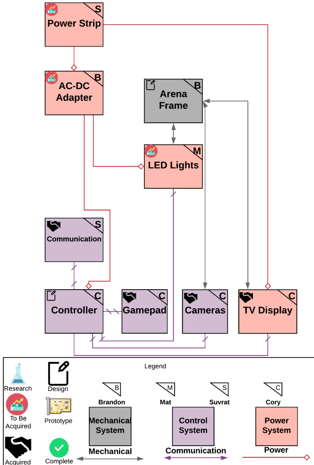
Figure 38 Arena Subsystem Power and Signal Diagram
