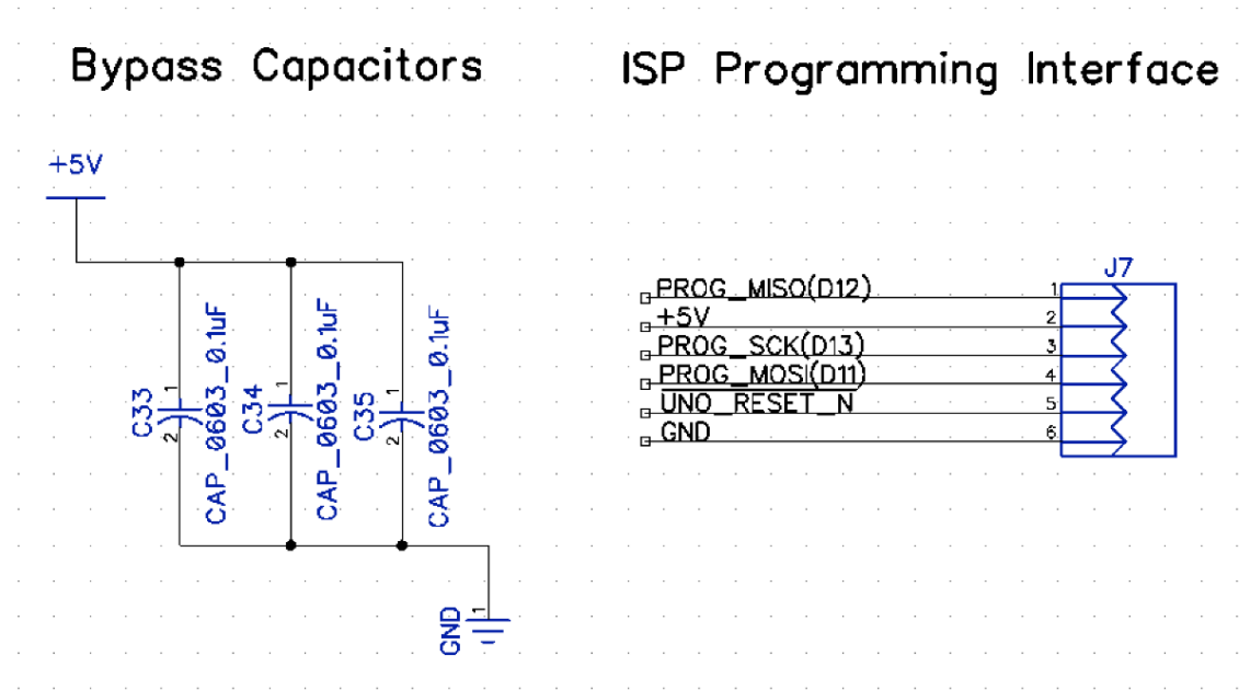
Figure 28: ATmega328P Microcontroller Bypass Capacitors and Programmer Interface
