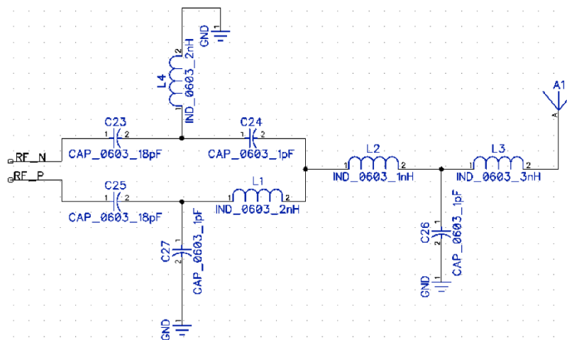
Figure 30 Bluetooth Programmer/Debugger and RF Matching Circuit
