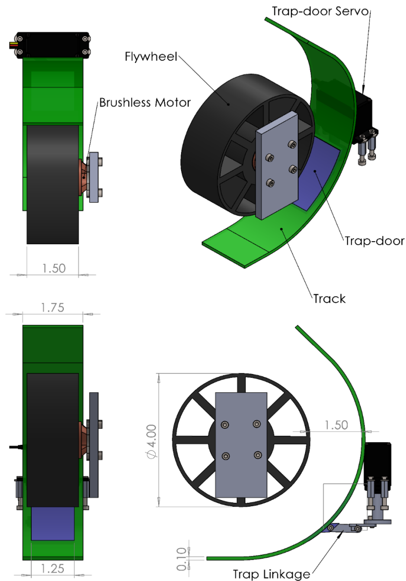
Figure 16 Launcher design drawing
