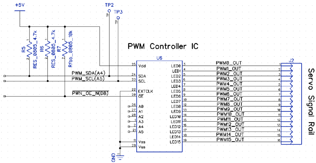
Figure 31 PWM Controller Schematic
