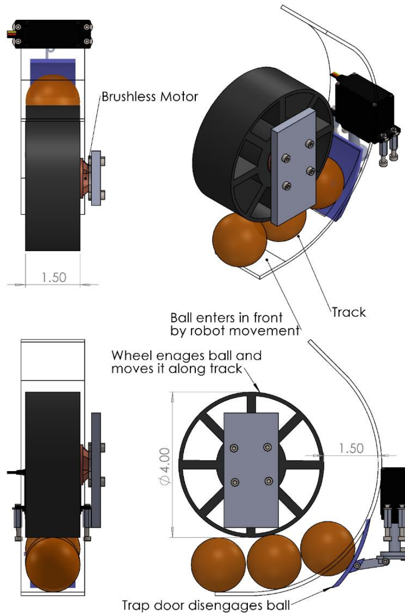
Figure 18 Intake Design
