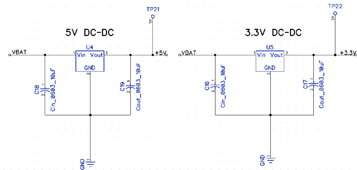
Figure 24: Schematic for 3.3V and 5V DC-DC Converter
