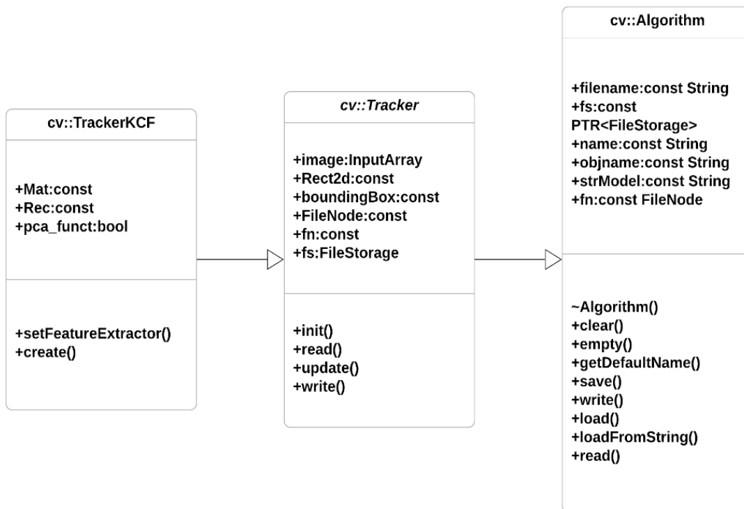
Figure 53 Basic Class Diagram for Computer Vision [82]
