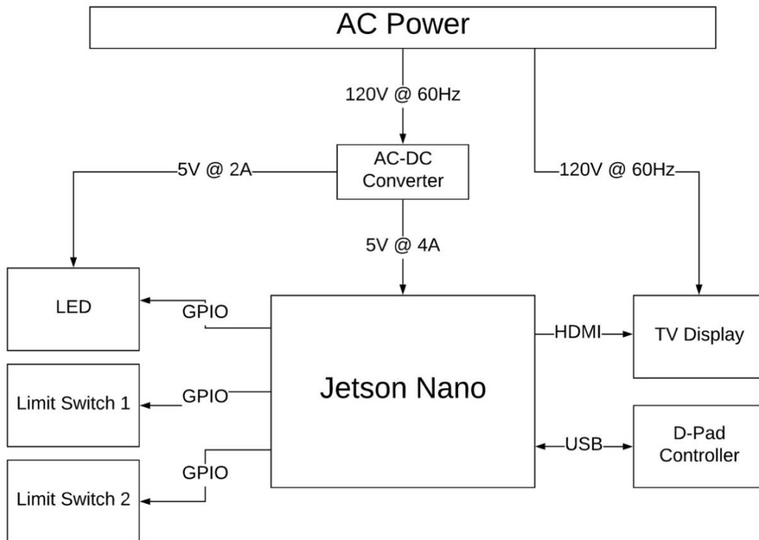
Figure 52 Arena Electrical Network Block Diagram
