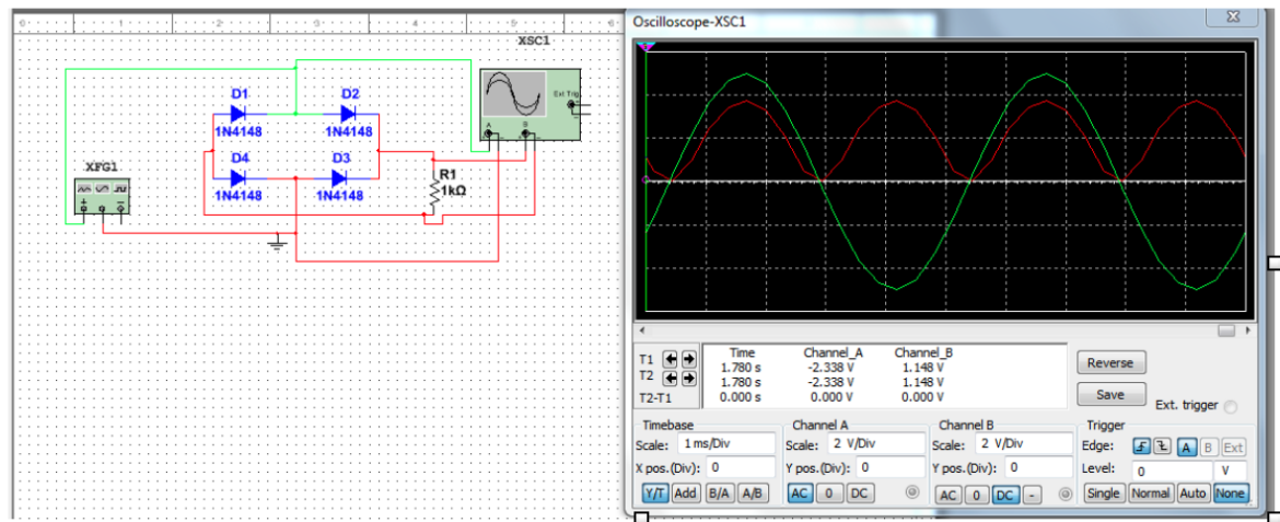
Fig 5.4.3 (2) Rectification Circuit-B
