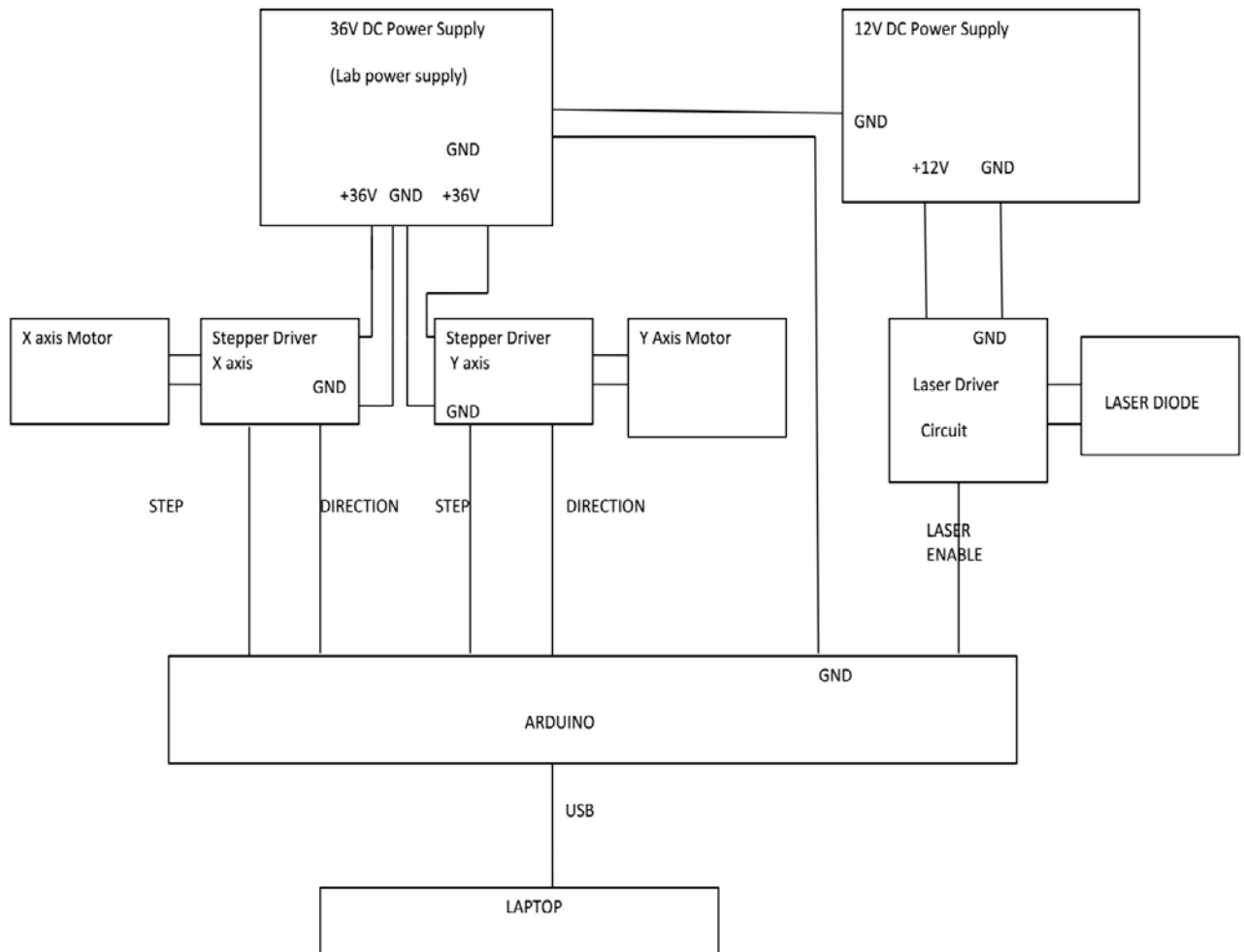
Fig 5.4 Power Delivering Analysis Diagram
