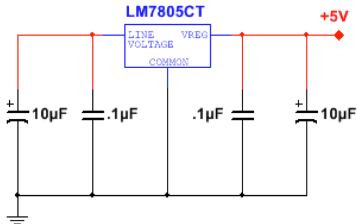
Fig 5.4.2 (1) 5V Power Supply using LM7805.
