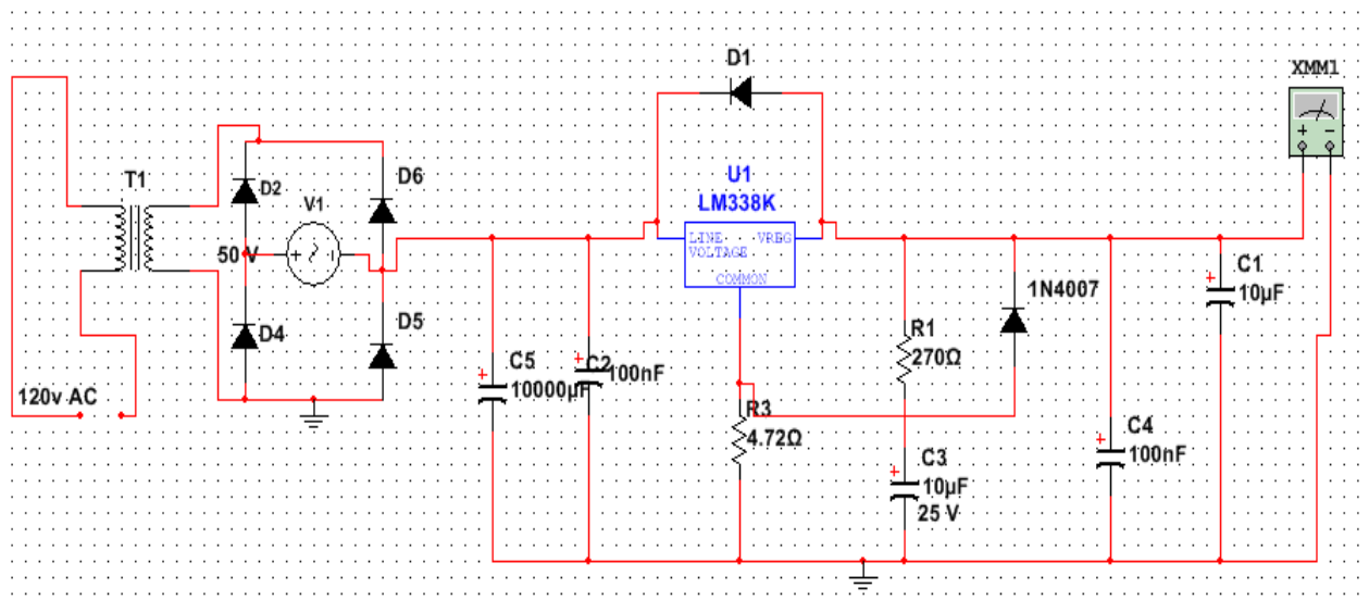
Fig 4.4.4 (1) LM Series Regulator Circuit
