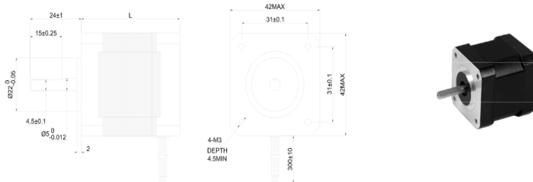
Fig 6.3.2 (1) Datasheet extract of physical specs for the NEMA17 motor (Permission pending from OSM stepper motors)
