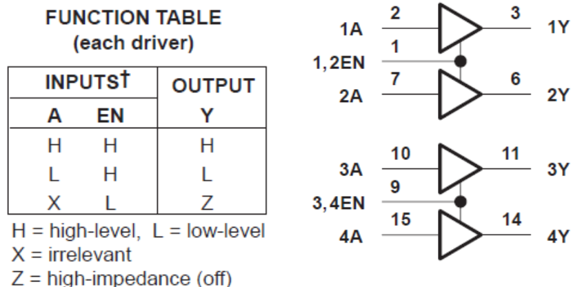
Fig 5.3.2 (2) Function Table (Pending permission from Texas Instruments)
