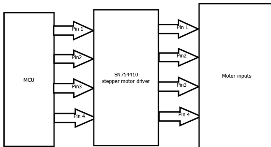
Fig 5.3.4 (1) MCU Stepper Control diagram
