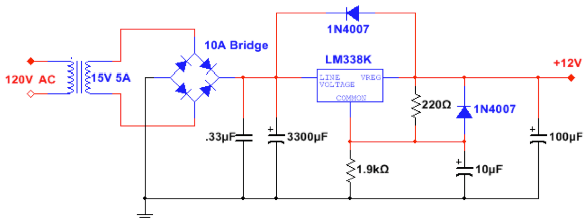
Fig 5.4.1 (1) Circuit Diagram
