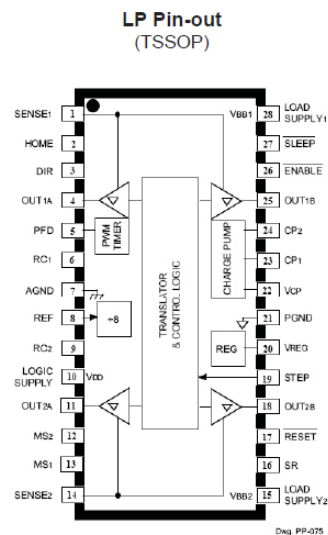
Figure 3.4.2(2) A3977 (Pending permission from allegro)
