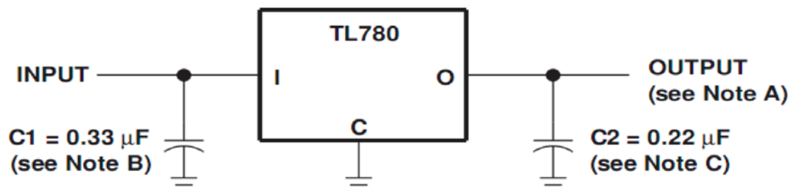
Fig 4.4.5 (1) Parameter Information of TL780 Pending Permission from TEXAS INSTRUMENTS.
