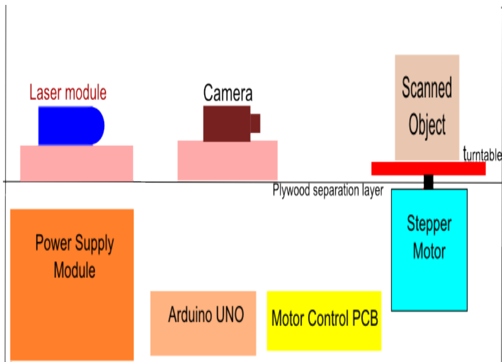
Fig 6.3.3 (1) Vertical cut view of the components diagram
