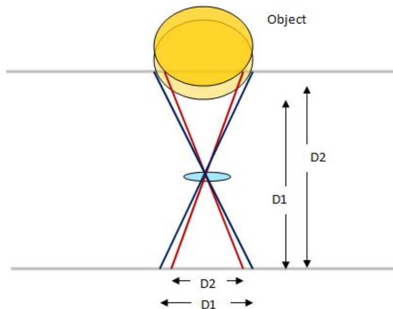
Figure 3.7.4(1) shape from focus (Permission pending)
