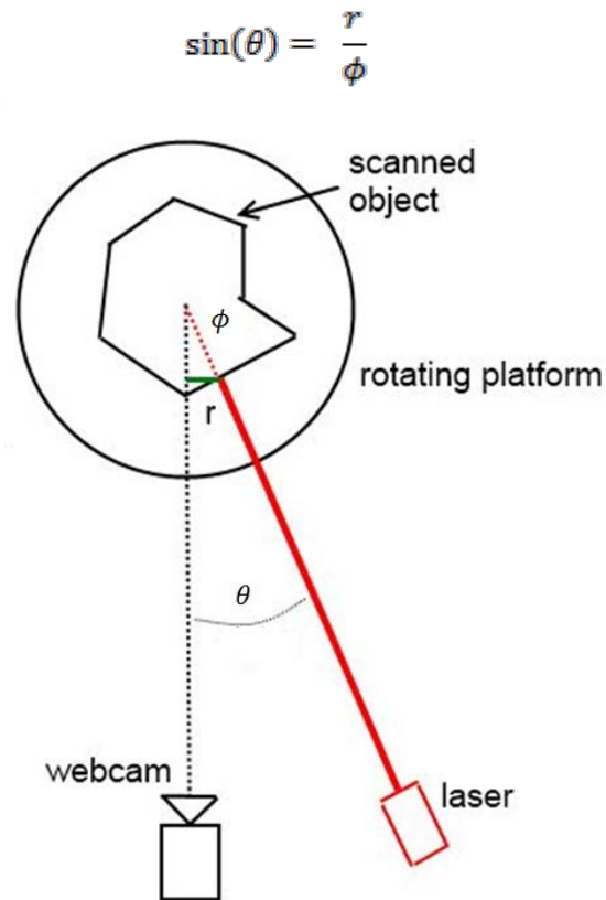
Fig 5.5.7 (1) Laser Triangulation Diagram-A
