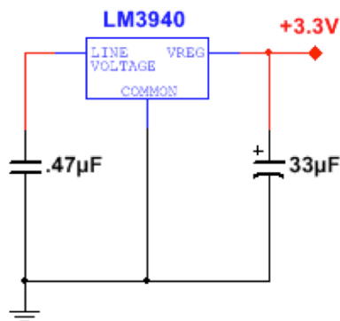
Fig 5.4.2 (2) LM3940 Circuit Diagram
