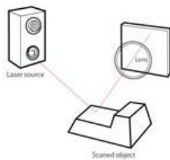
Fig 3.8.7 (1) Laser Triangulation Approach (Pending permission from rapidform.com)
