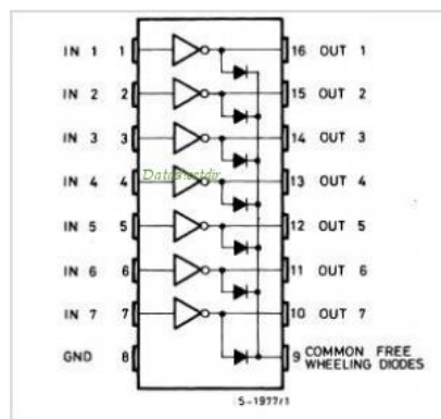
Figure 3.4.2(1) PINout diagram of the ULN2804A (Pending approval from T.I.)
