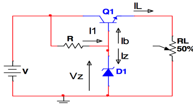
Fig 4.4.2 (2) Emitter Follower
