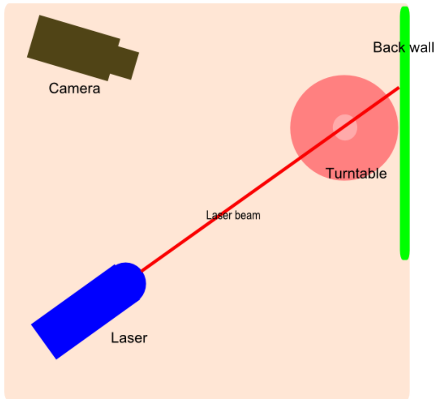
Fig 6.3.3 (2) Top view of the components
