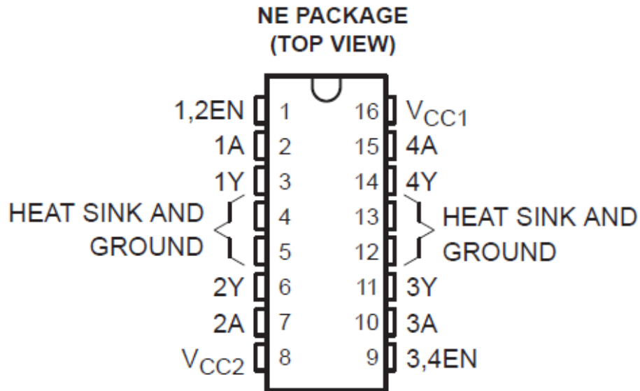
Fig 5.3.2 (1) SN754410 Integrated circuit Pin diagram (Pending permission from Texas Instruments)
