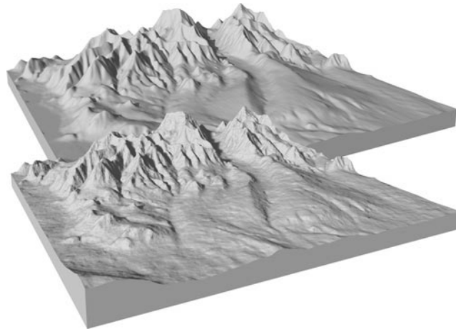
Fig 4.3(8) 3D Surface Model of a Valley (Pending Permission from pubs.usgs.gov)
