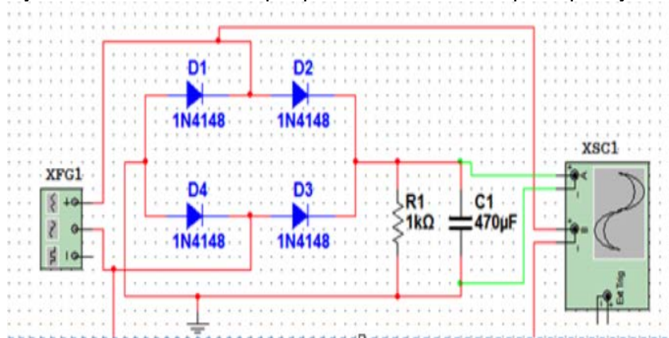
Fig 5.4.3 (1) Rectification Circuit-A
