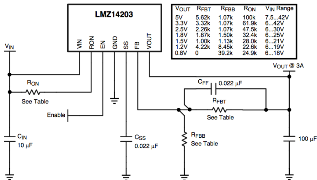
Fig 4.4.7 (2) Schematic of LMZ14203 Pending permission from Texas Instruments.
