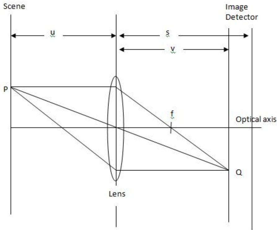
Figure 3.7.4 (2) Shape from focus (Convex Lens) (Permission Pending)
