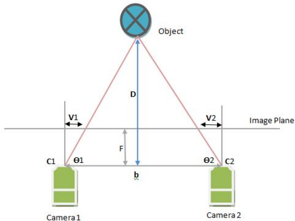
Figure 3.7.3(1) Stereo vision triangulation (Giving credit to ni.com)
