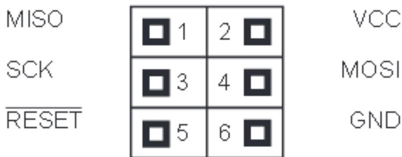
Fig 5.3.3 (1) ISP Diagram
