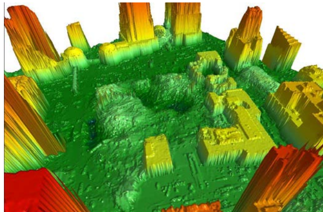
Fig 4.3(9) 3D Surface Model of Aerial New York City (Pending Permission from GIS Community)
