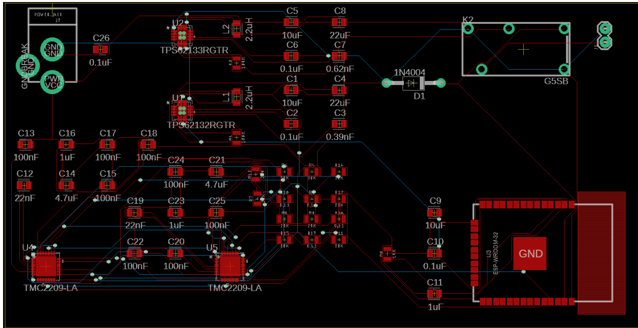
Figure 6-7: PCB Board Prototype
