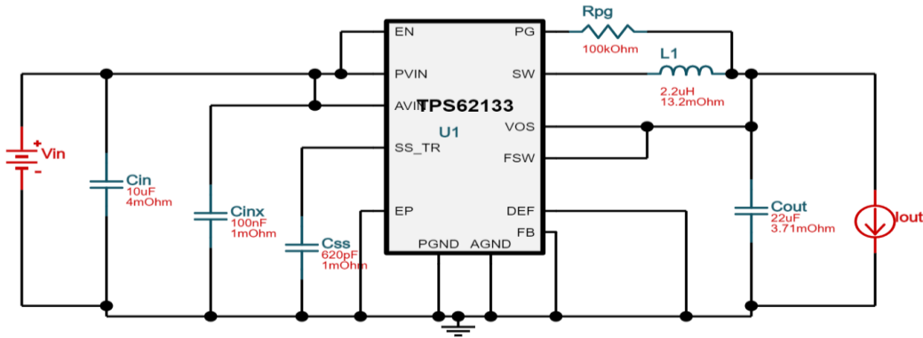
Figure 5-3: 5.0V Voltage Regulator Schematic, Courtesy of Texas Instruments
