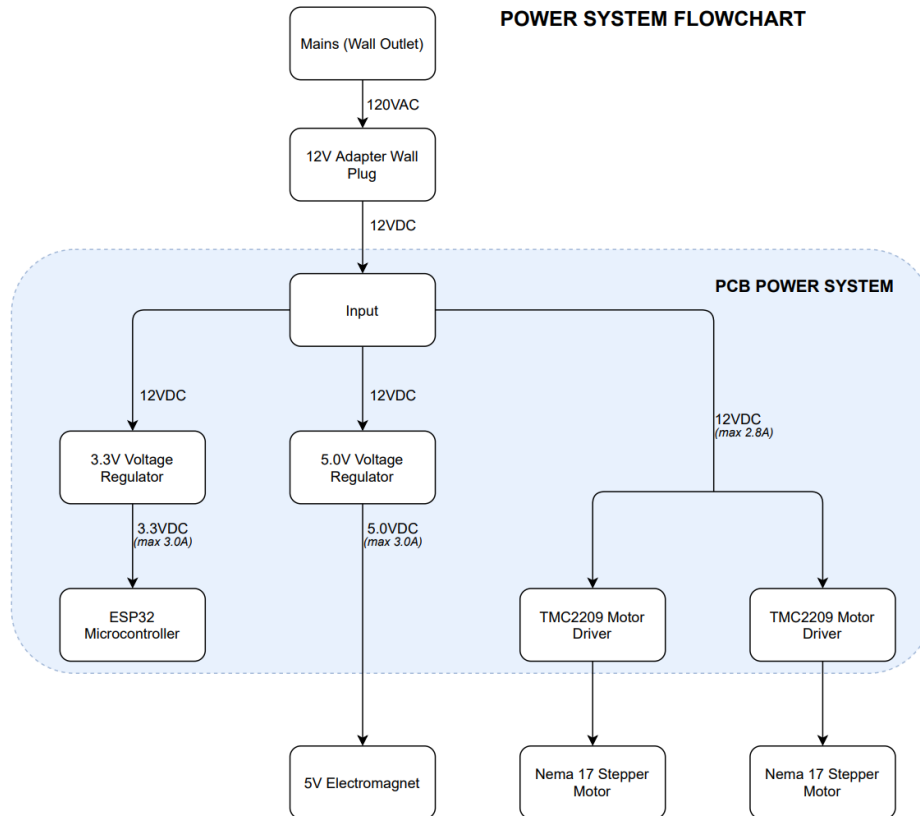
Figure 5-1: Power System Flowchart
