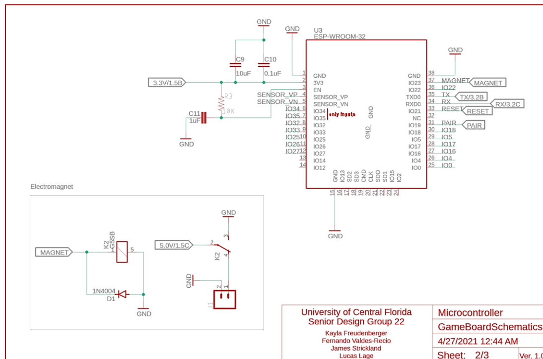
Figure 6-6: Microcontroller and Electromagnet PCB Schematic Prototype
