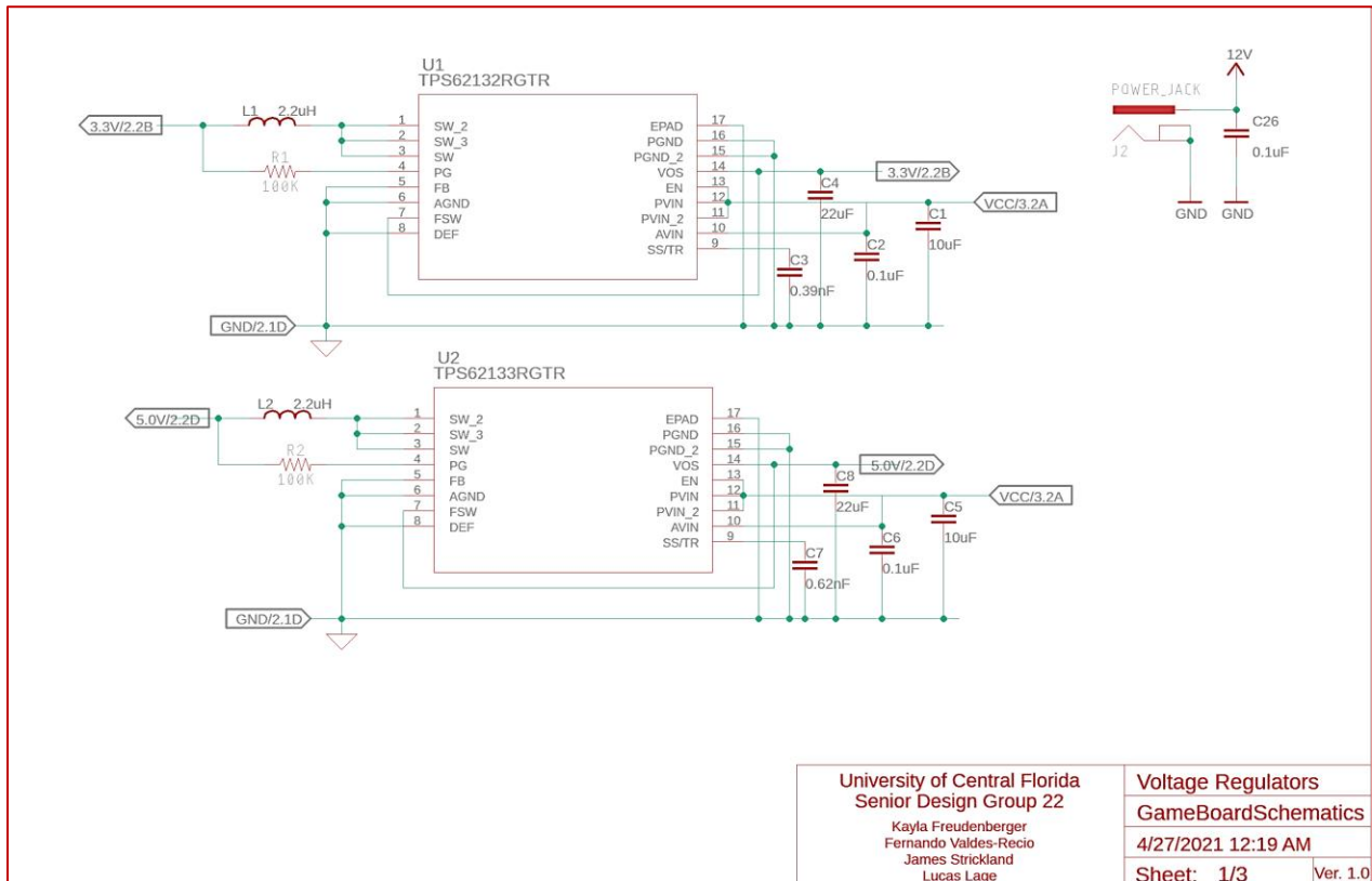
Figure 6-4: Voltage Regulator PCB Schematic Prototype
