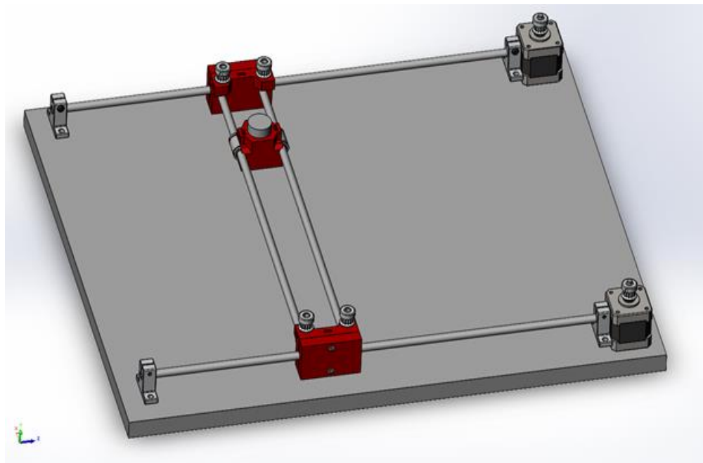
Figure 6-1: Arcane Game Board SolidWorks Design
