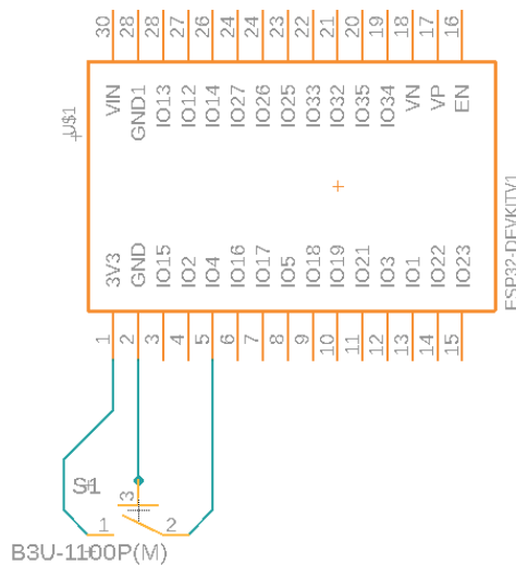
Figure 6-9: Schematic of an ESP32 Development Kit with a push button connecting VCC to GPIO pin 4. This proved troublesome to work with and should be avoided in the final design.
