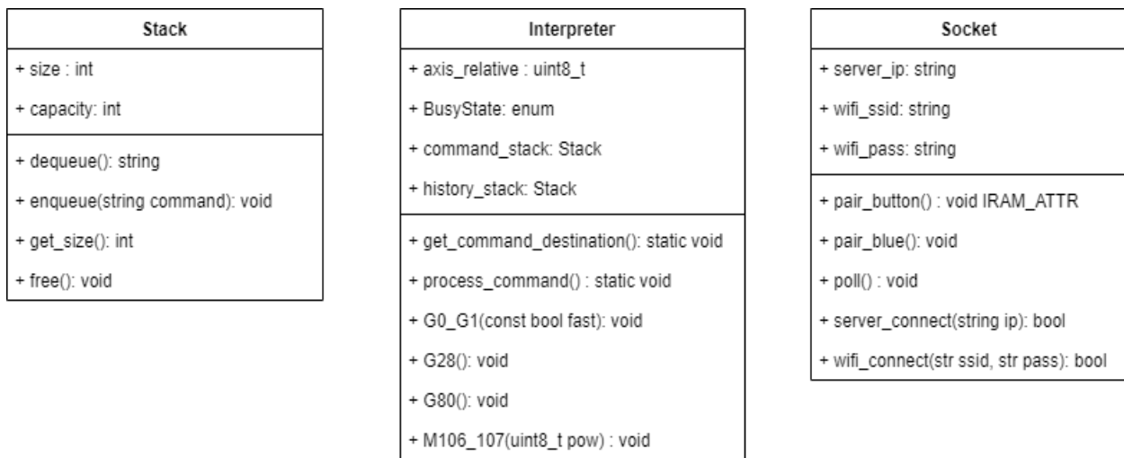
Figure 5-6: Class Diagrams
