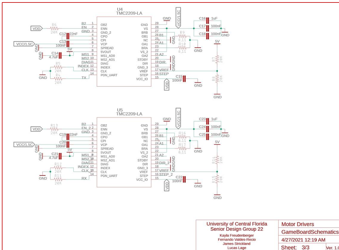
Figure 6-5: Motor Driver PCB Schematic Prototype
