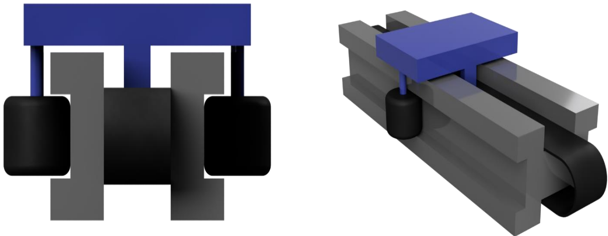
Figure 3-3: Mock-up of Basic Belt Linear Stage Assembly
