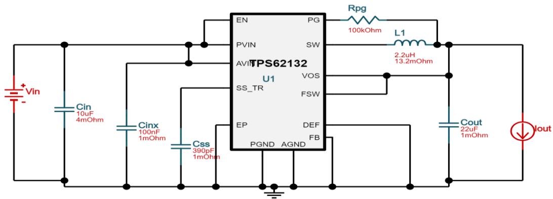
Figure 5-2: 3.3V Voltage Regulator Schematic, Courtesy of Texas Instruments
