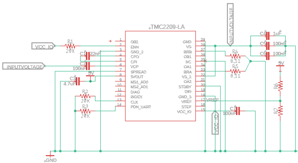
Figure 5-4: TMC2209-LA Schematic
