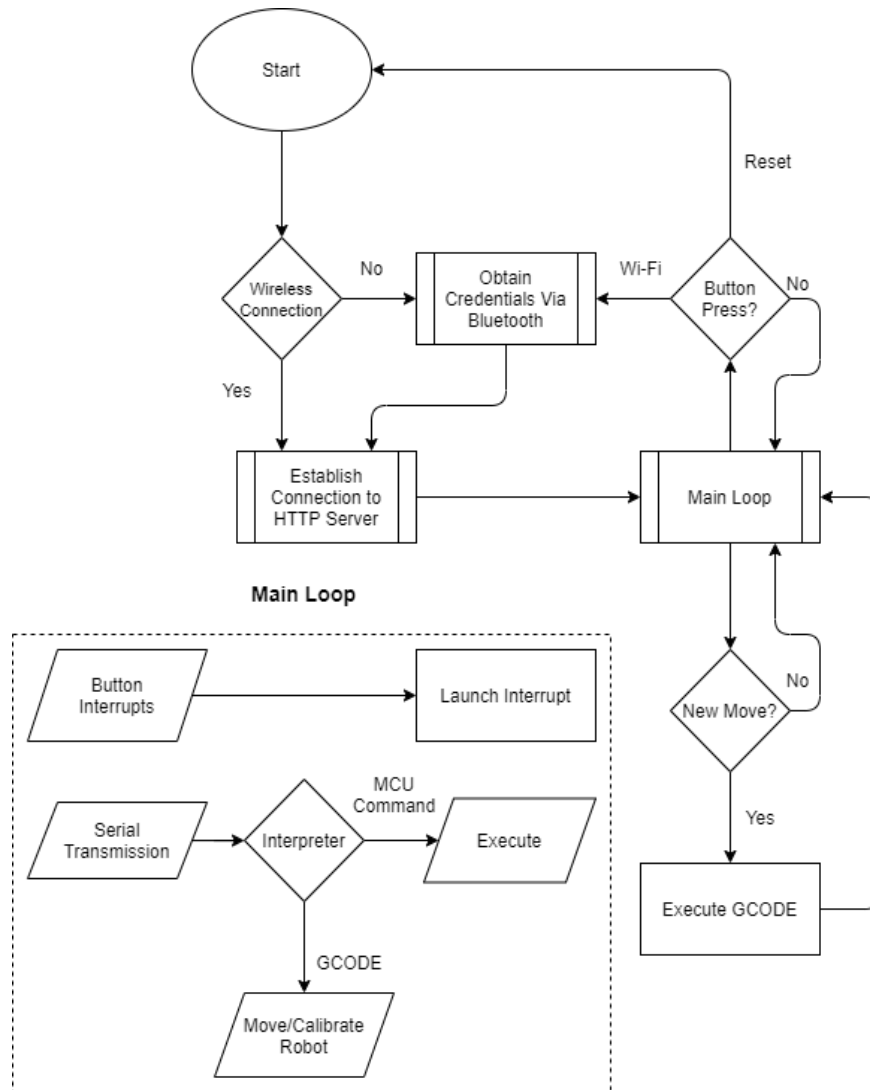
Figure 5-5: Flow Diagram of MCU Firmware Operation
