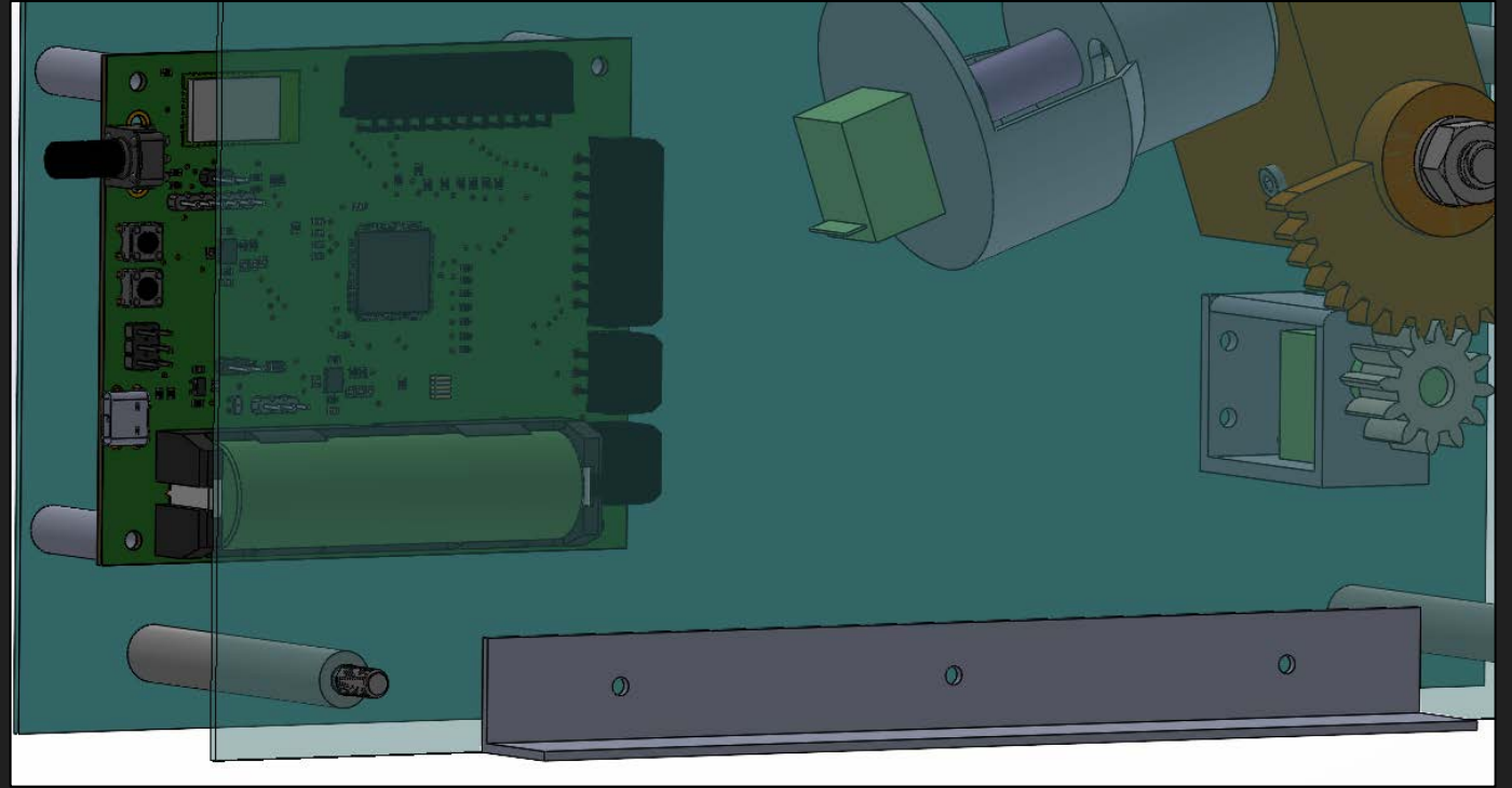
PCB positioning and unit mounting brackets
