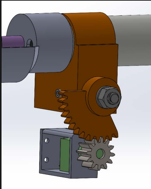
Lever angle gear reduction and encoder mount
