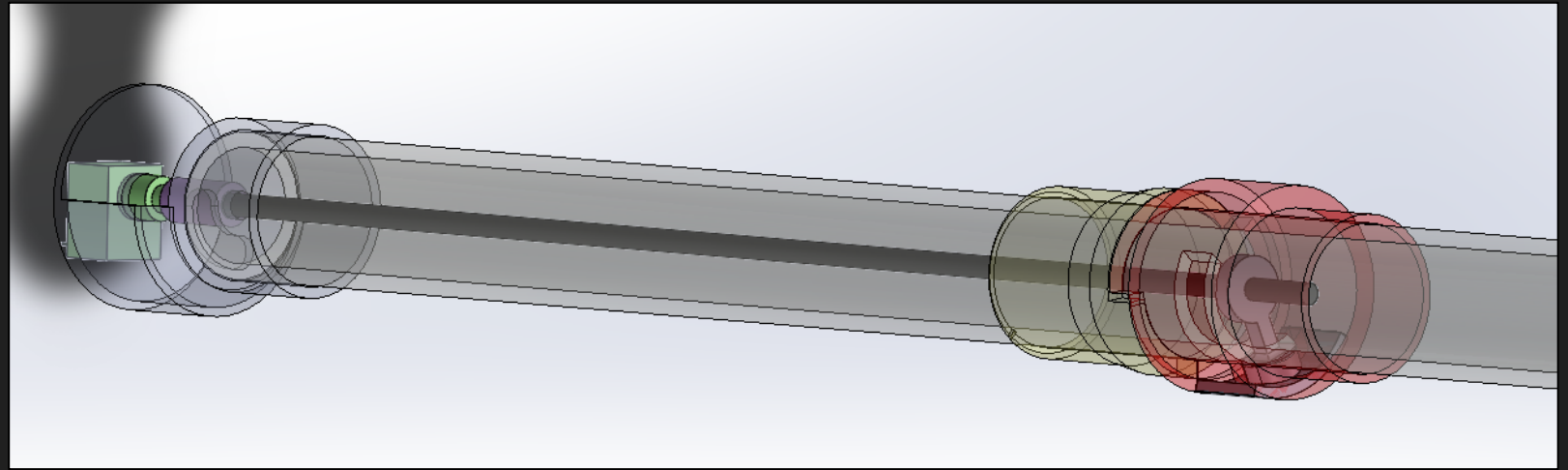
Throttle and connecting rod complete assembly
