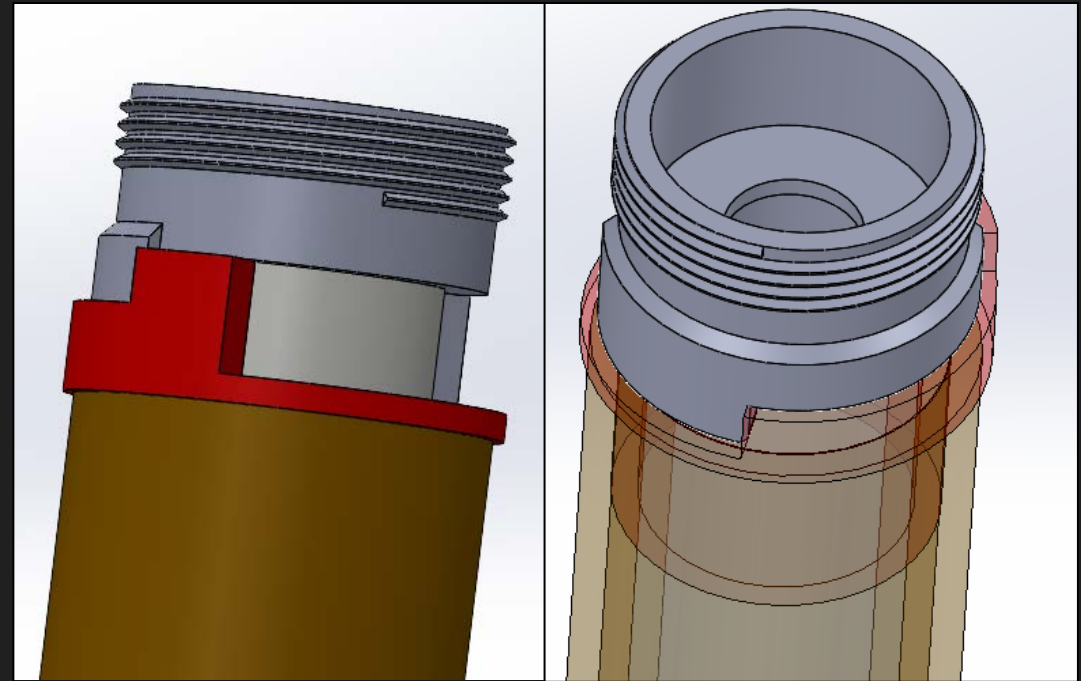
Collective lever endcap and 17-pin Molex interface
