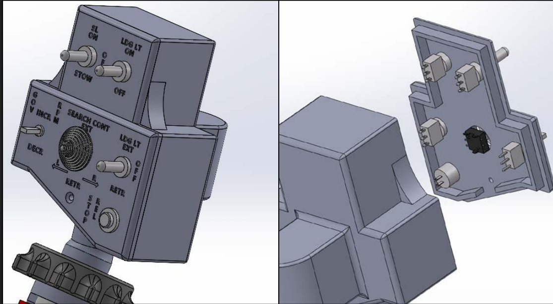
Huey collective head assembly and faceplate
