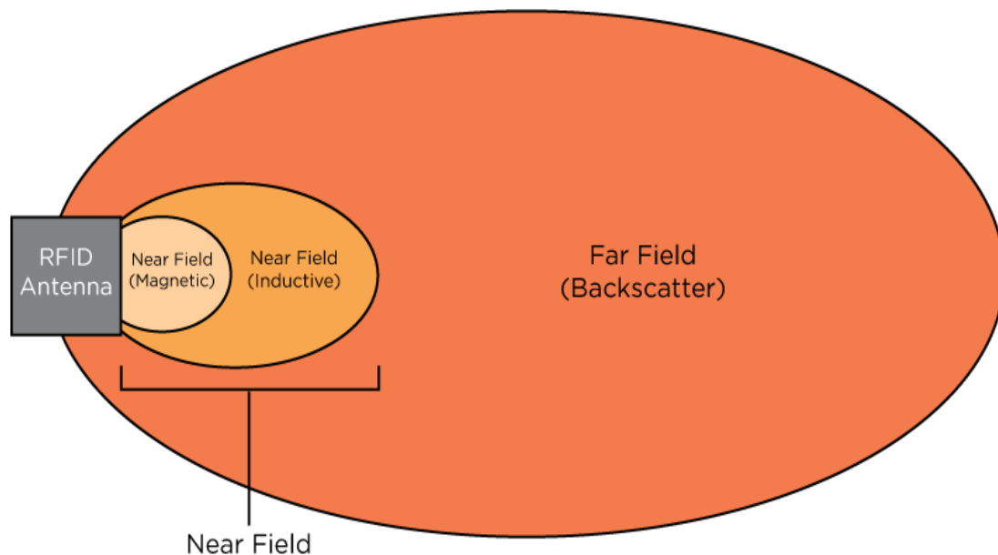
Figure 8: Near Field vs Far Field
