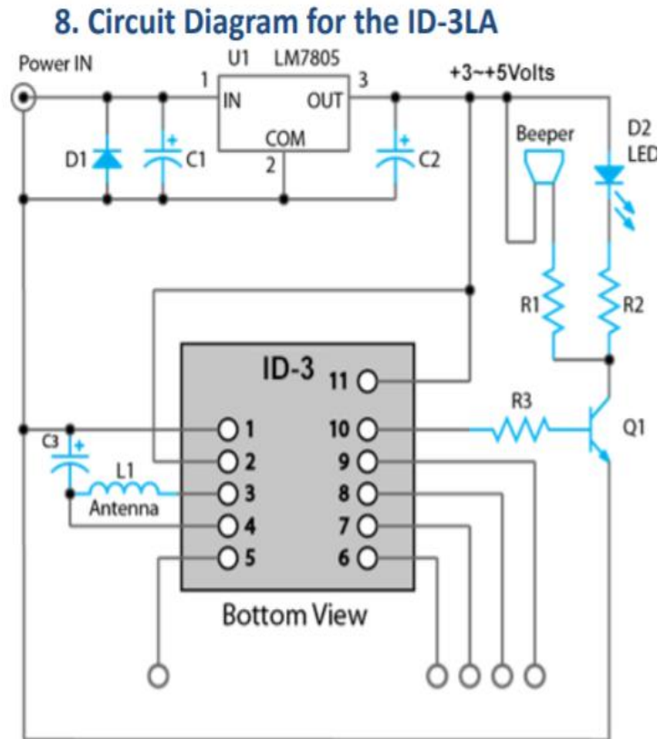
Figure 33: ID-3LA Schematic (Copyright permission granted)
