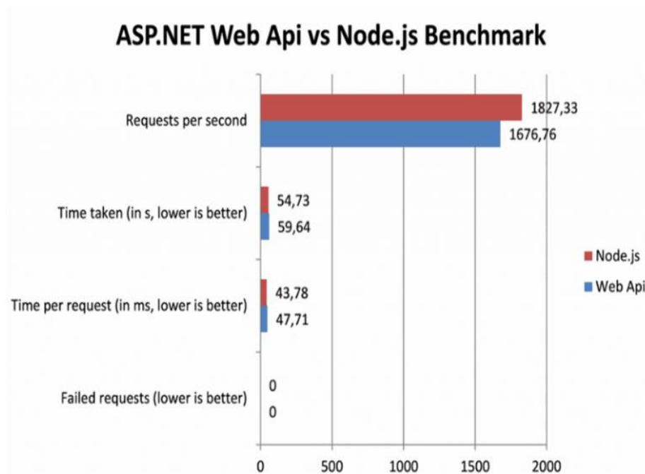
Figure 53: ASP and Node benchmark comparisons
