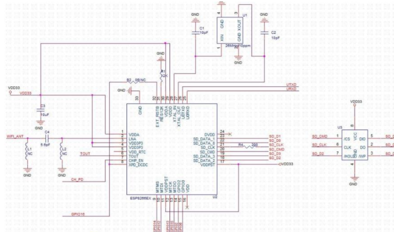
Figure 41: ESP8266 Schematic (Copyright permission pending)
