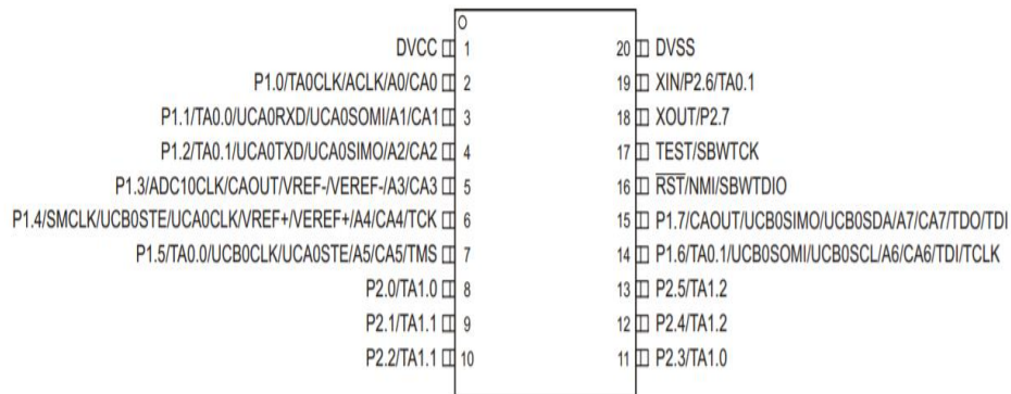
Figure 43: MSP430 layout
