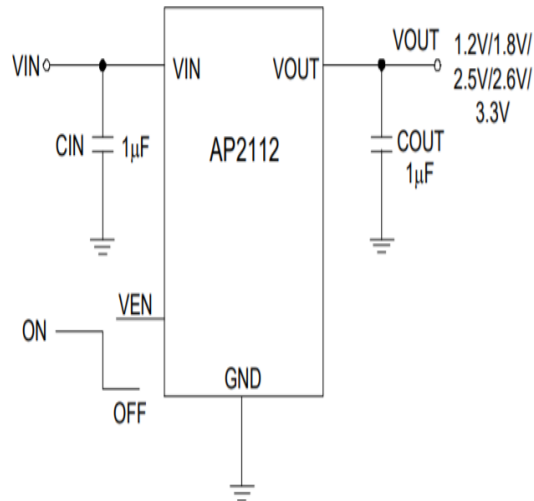
Figure 37: AP2112K schematic
