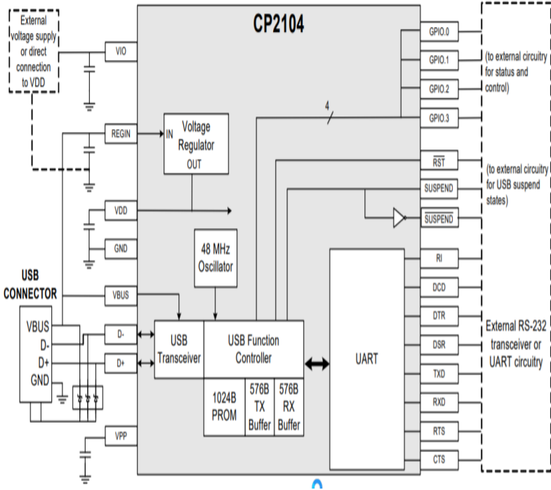
Figure 39: CP2104 Schematic
