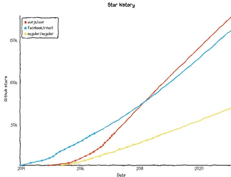
Figure 58: Popularity Vue vs React vs Angular
