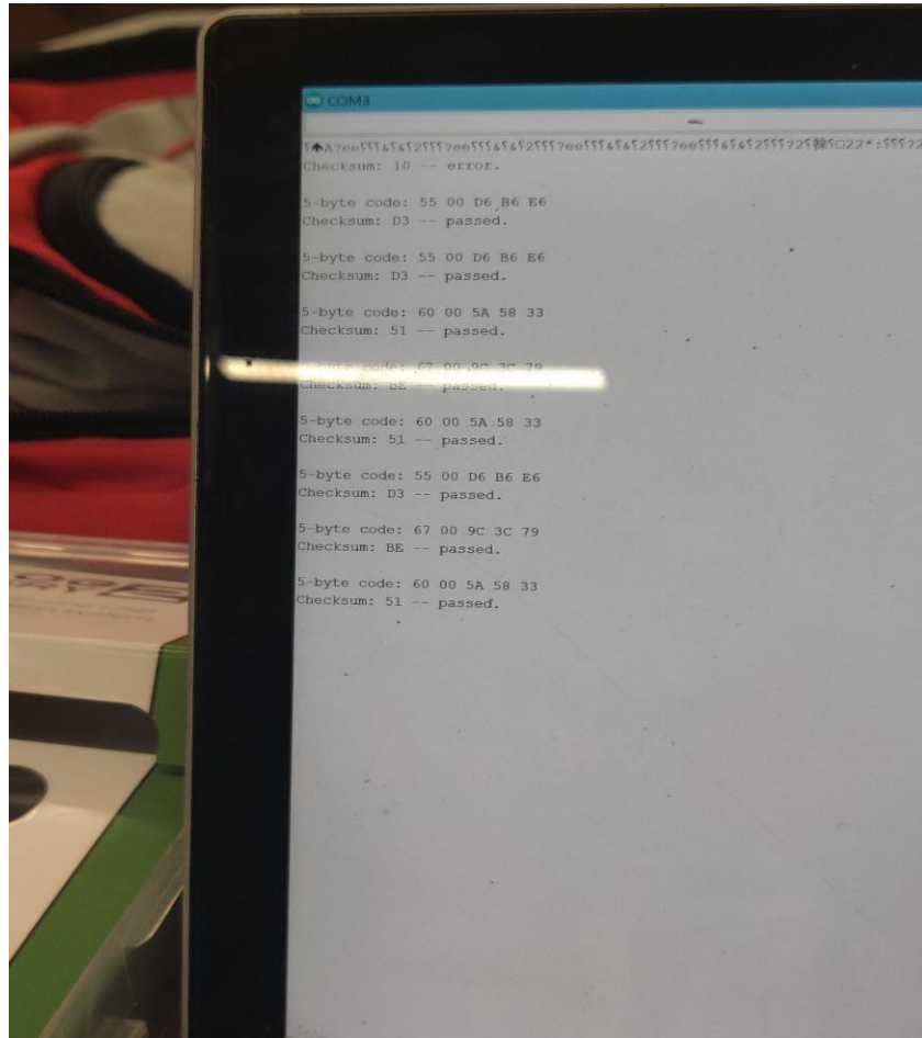
Figure 82: Serial Output of ID-12LA test
