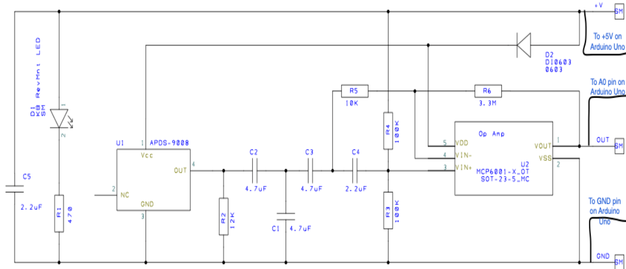
Pulse Sensor Amplified Designed by Joel Murphy Licensed under the TAPR Open Hardware License ( www.tapr.org/OHL ) Spring 2012
