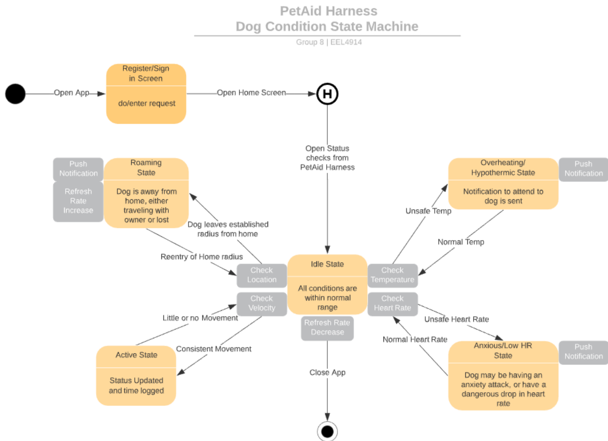
Figure 14: PetAid pet condition state machine
