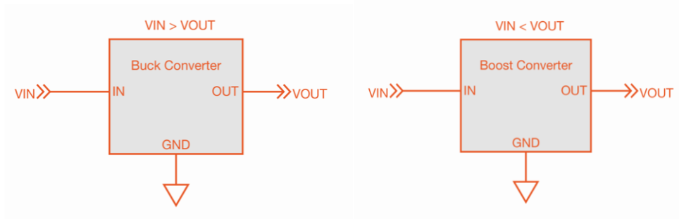
Figure 17: Buck Converter and Boost Converter.
