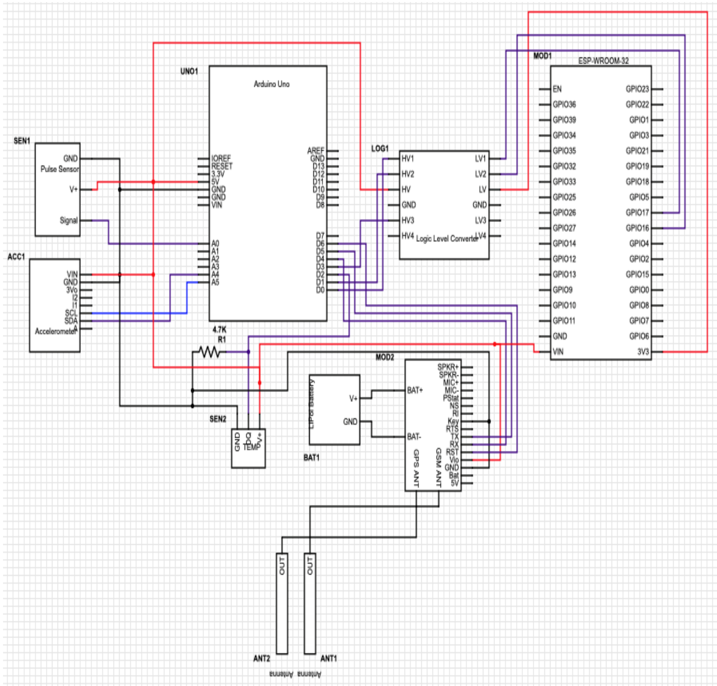
Figure 20: Final Schematic made in Scheme-it by Digikey (Data Line, Clock Line, High Voltage Line, Ground Line)
