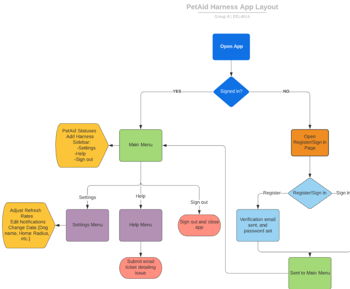
Figure 13: PetAid application layout
