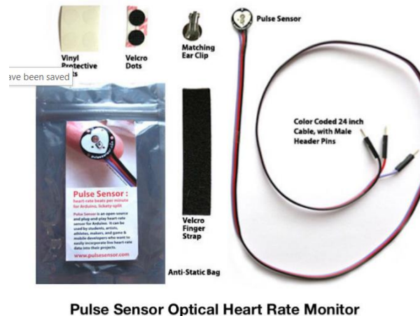
Figure 23: Heart rate pulse sensor kit for testing (courtesy of PulseSensor.com).
