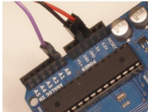
Figure 27: Arduino Uno +V, GND, A0 pin connectors.
