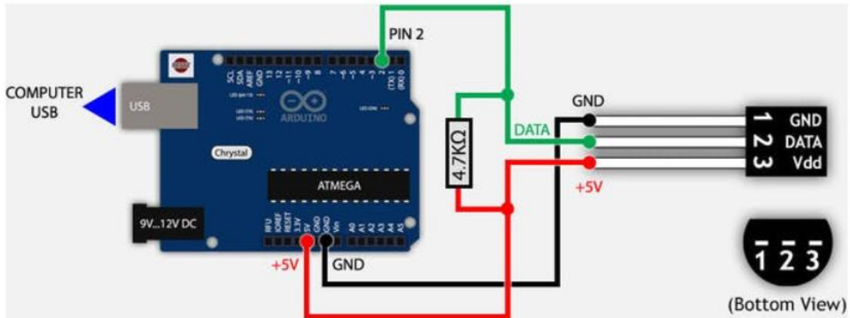
Figure 30. Circuit for the Temperature sensor testing (Courtesy of Arduino.com)
