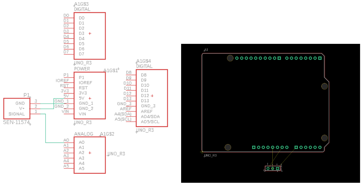
Figure 29: Heart Rate monitor schematic and board layout with Arduino Uno.
