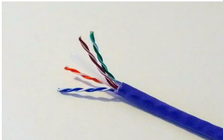
Figure 28: Stranded Cat 6 Ethernet cable
