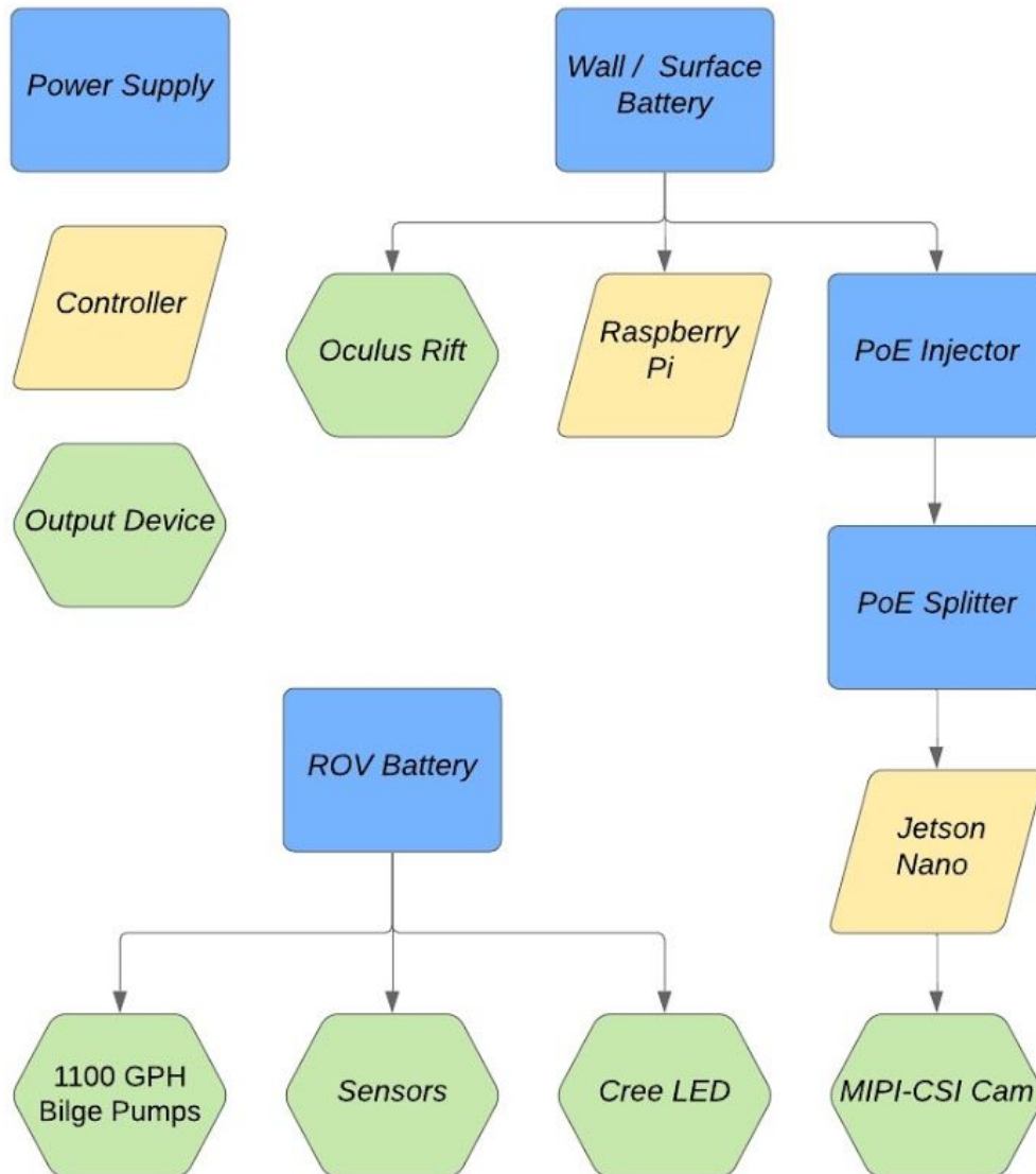
Figure 21: High-Level Power Flow
