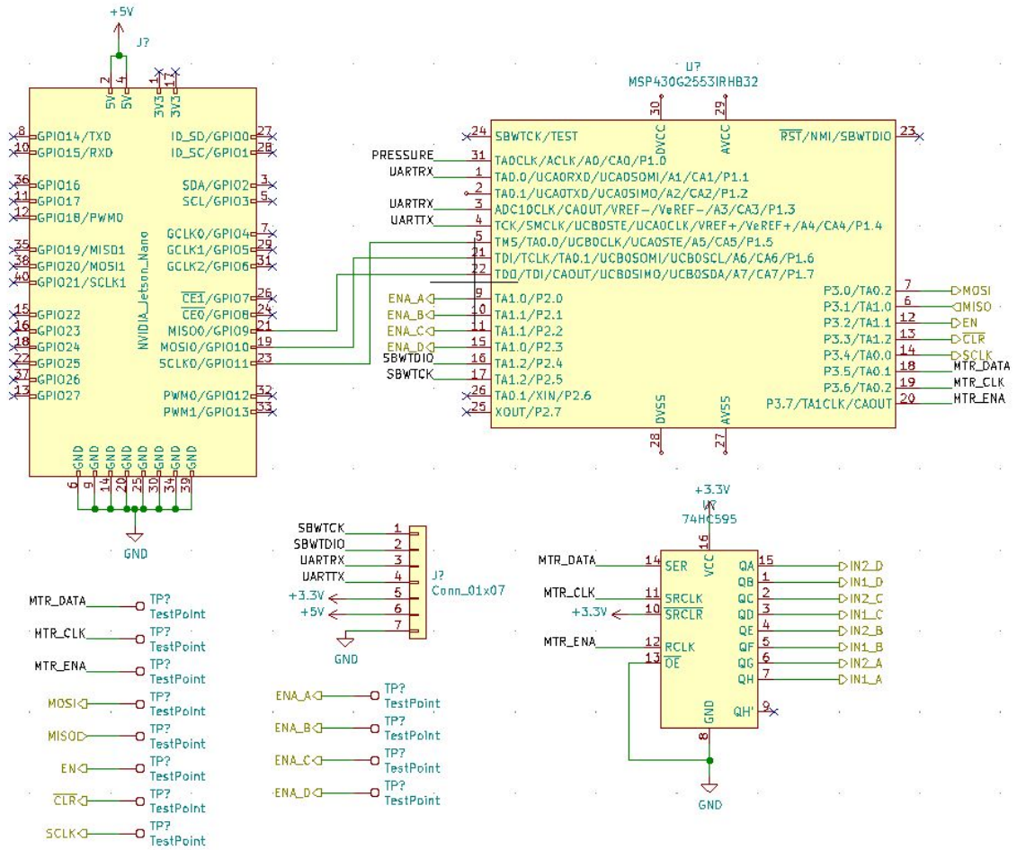
Figure 37: The connections between the Jetson, the MSP430 and discrete components
