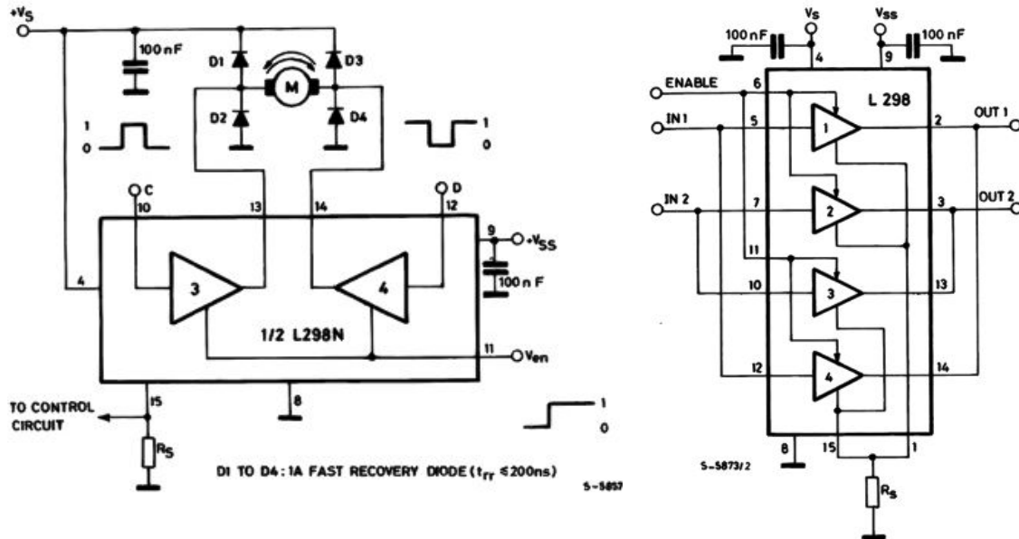
Figure 38: Application schematics from the L298
