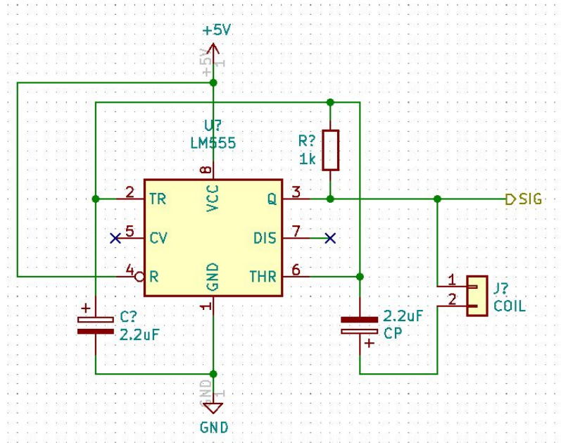
Figure 42: RLC oscillator circuit using the 555 timer
