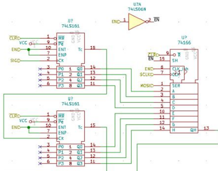
Figure 43: This pulse counting circuit provides a SPI interface to measure frequency
