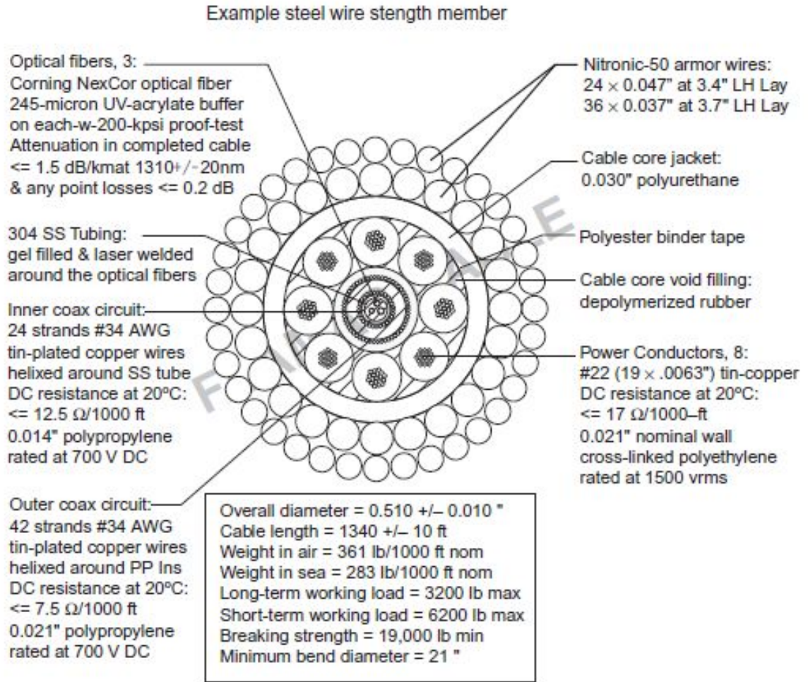
Figure 27: Steel wire strength member Reprinted with permission pending, from [24]
