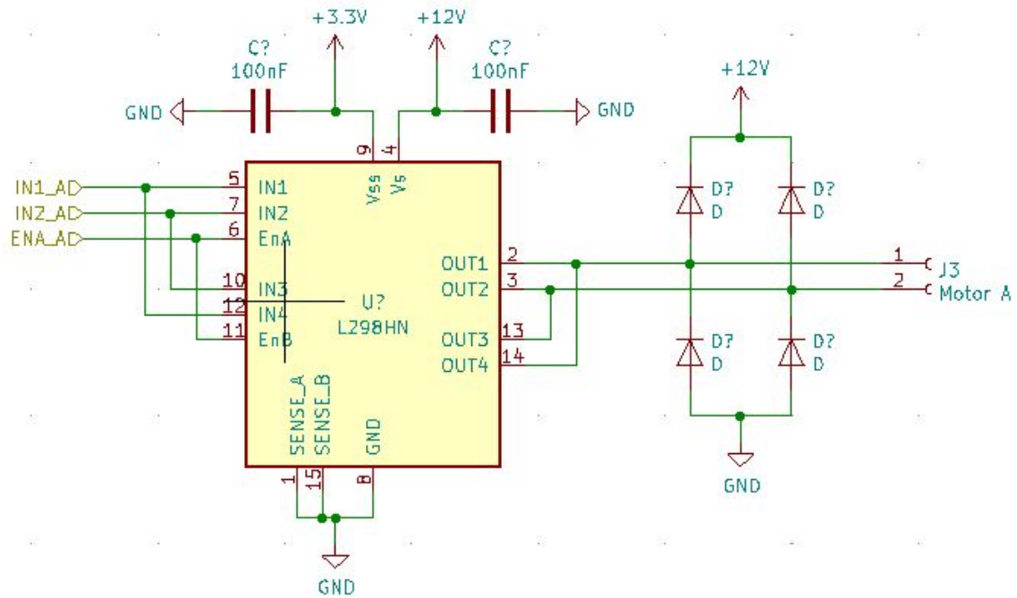
Figure 39: The resultant schematic of the motor driver subassembly.
