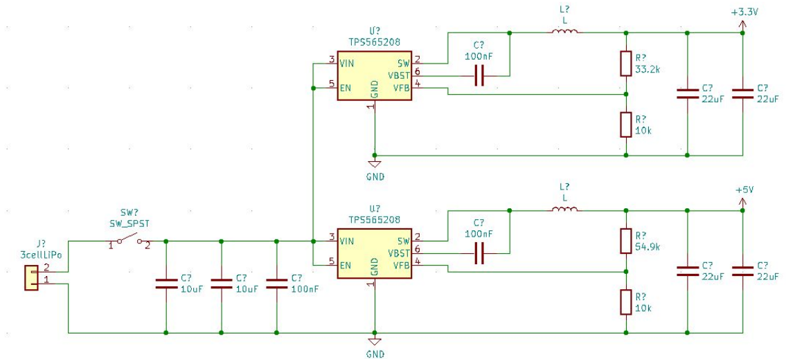
Figure 40: The voltage regulation for the low power electronics systems
