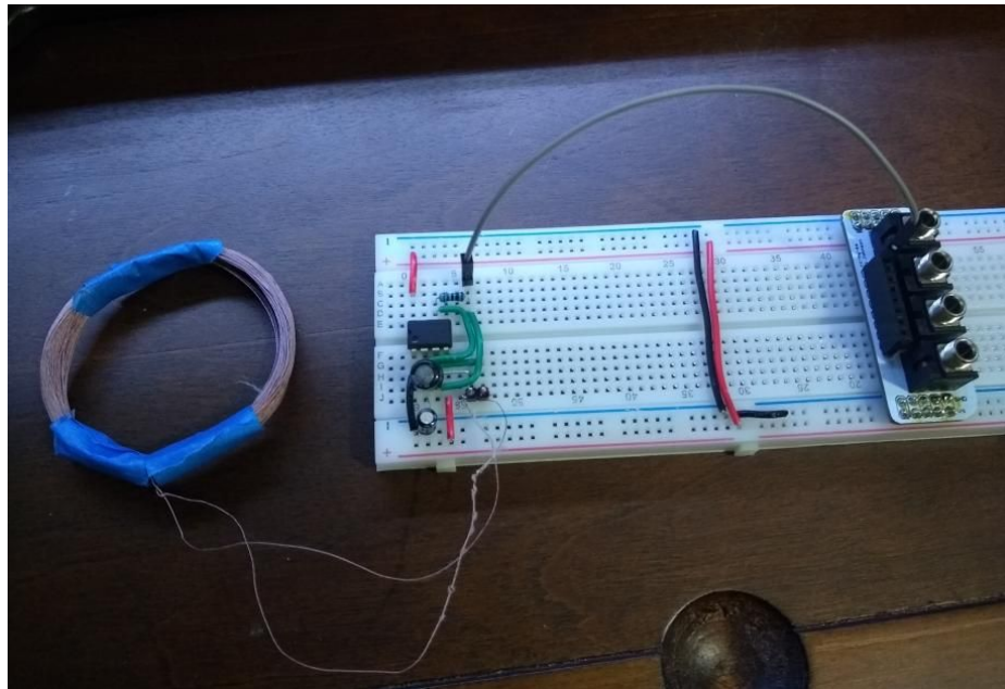
Figure 44: Breadboard prototype of metal detection circuit
