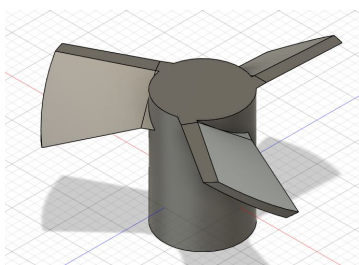
Figure 50: Design 1
