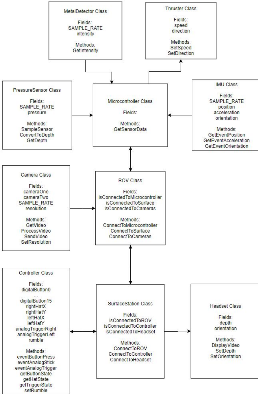
Figure 46: Class Diagram
