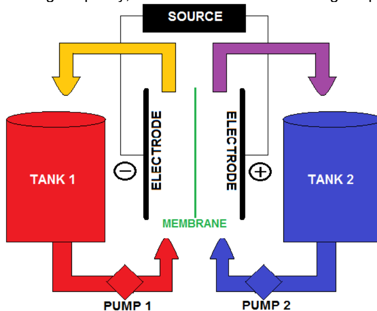
Figure 4.4.3.1: How the Flow battery works
