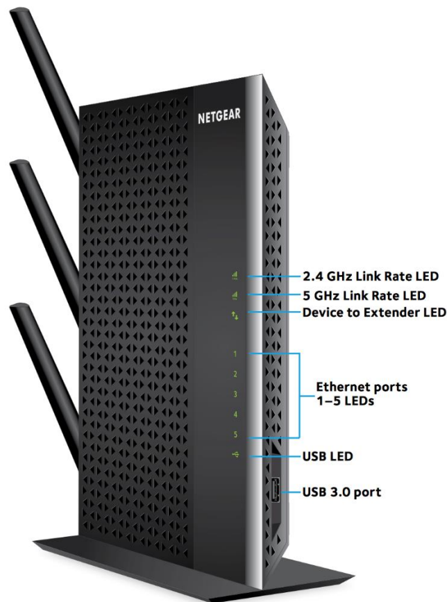
Figure 4.3.7.5.1: Wi-Fi Extender Front Panel and Side Panel [source]
