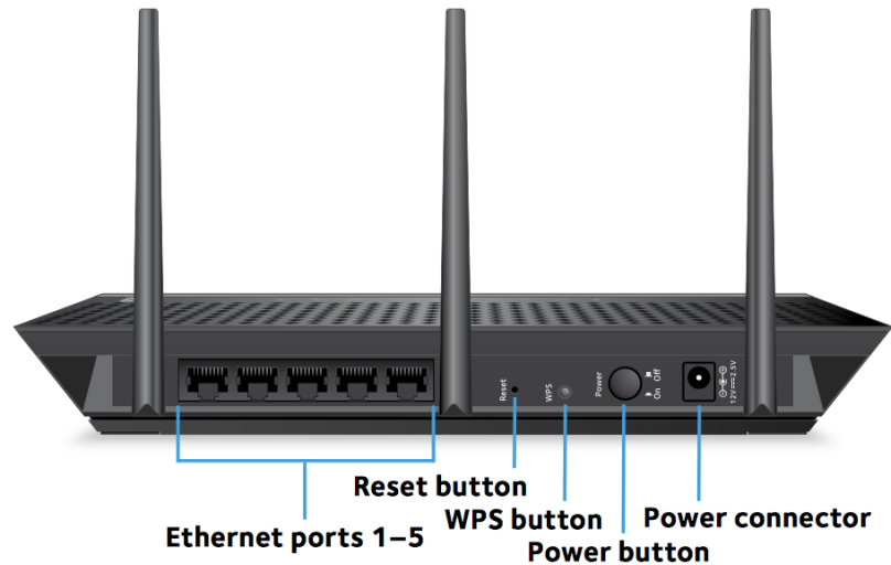
Figure 4.3.7.5.2: Wi-Fi Extender Rear Panel [source]
