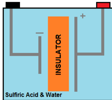
Figure 4.4.3.2: Cell of lead acid battery
