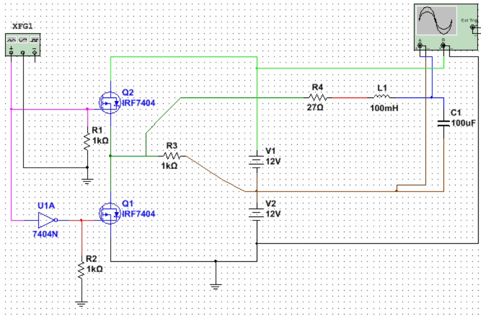
Figure 4.5.4.0a: Inverter Design A
