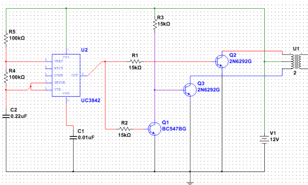
Figure 4.5.4.0b: Inverter Design B
