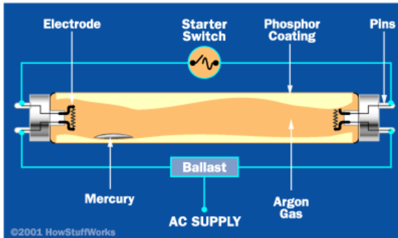
Figure 4.2.1.0c: Fluorescent Light Bulb
