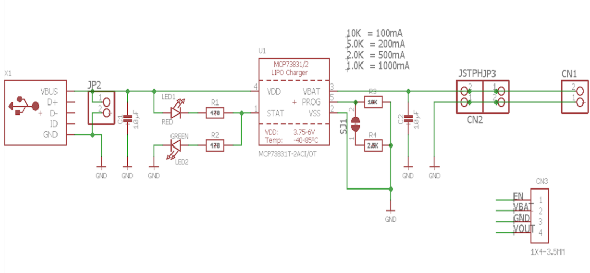
Figure 48: Battery Charging Design Schematic
