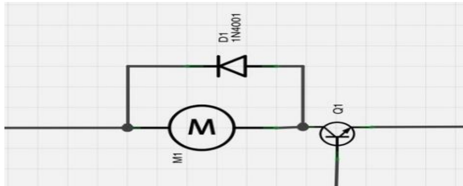
Figure 28: Motor Control Circuit Courtesy of https://learn.adafruit.com
