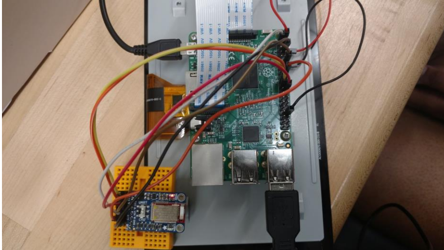
Figure 70: BlueFruit LE UART Wiring for Raspberry Pi
