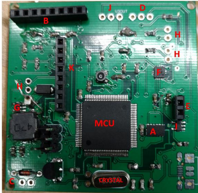
Figure 83: PCB with soldered components
