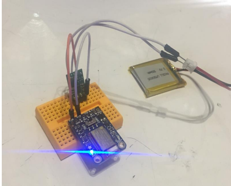
Figure 76: Bluetooth Powered with Battery and Voltage Regulator
