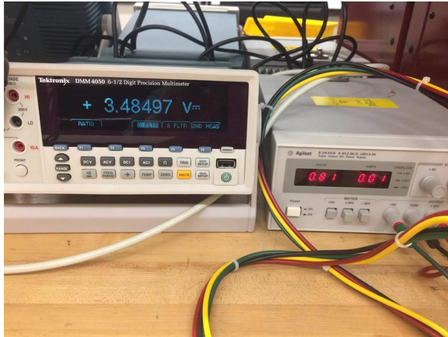
Figure 67: Supply voltage and base voltage of vibrating motor circuit
