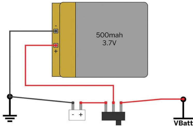
Figure 13: Battery Connection Schematic Example Courtesy of https://learn.adafruit.com/all-about-batteries/
