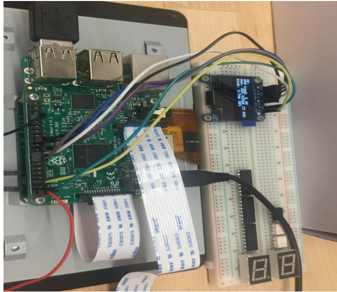
Figure 77: OLED Display Wiring to Raspberry Pi
