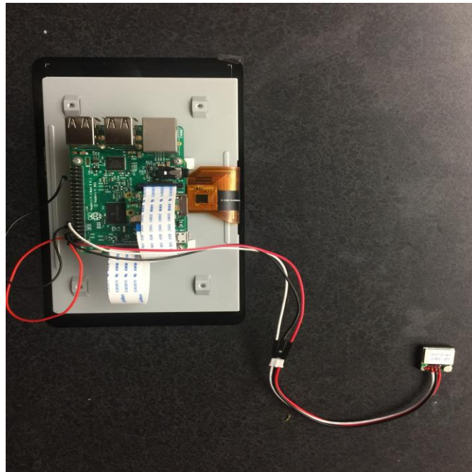
Figure 73: GPS UART Wiring for Raspberry Pi
