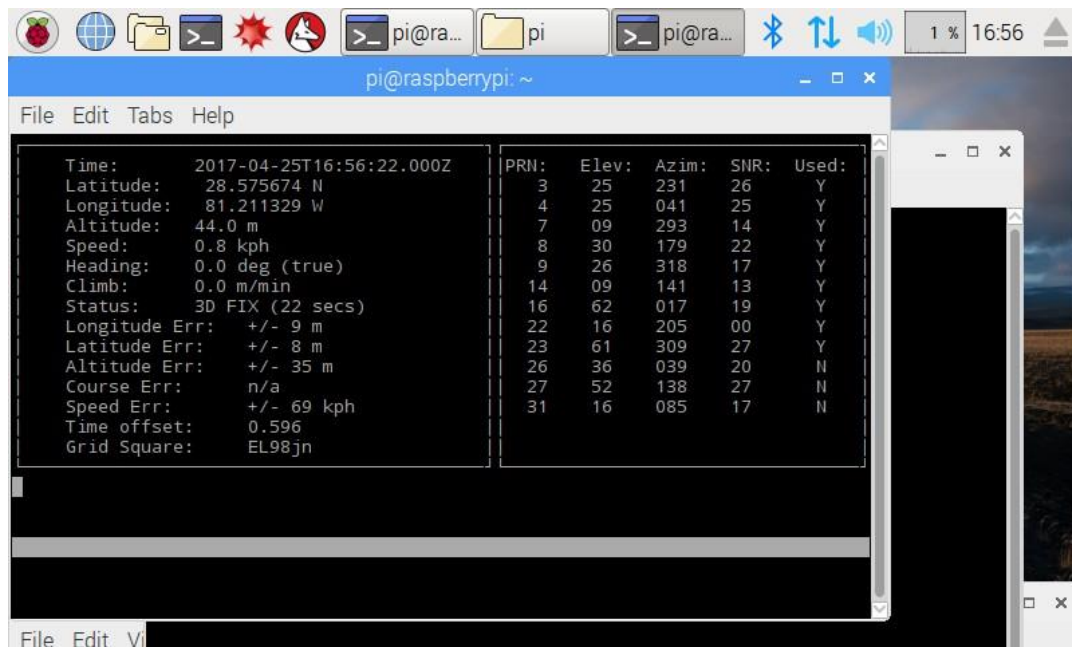
Figure 74: GPS Component Receiving Data
