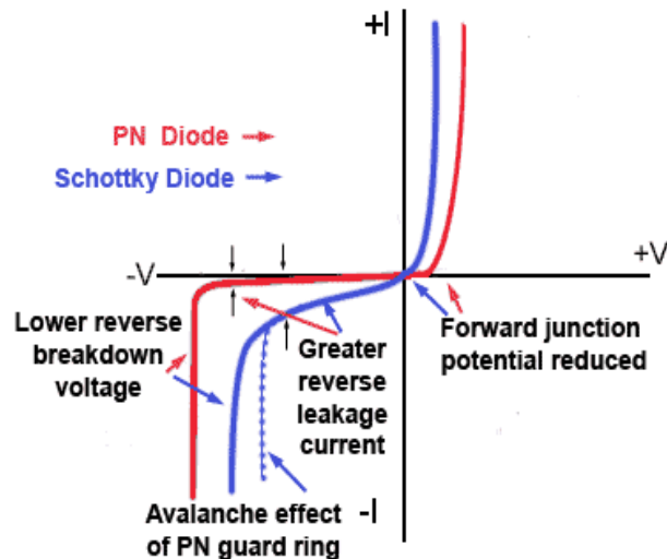
Figure 40: Voltage and Current Relationship of a Schottky Diode Courtesy of http://www.electronics-tutorials.ws
