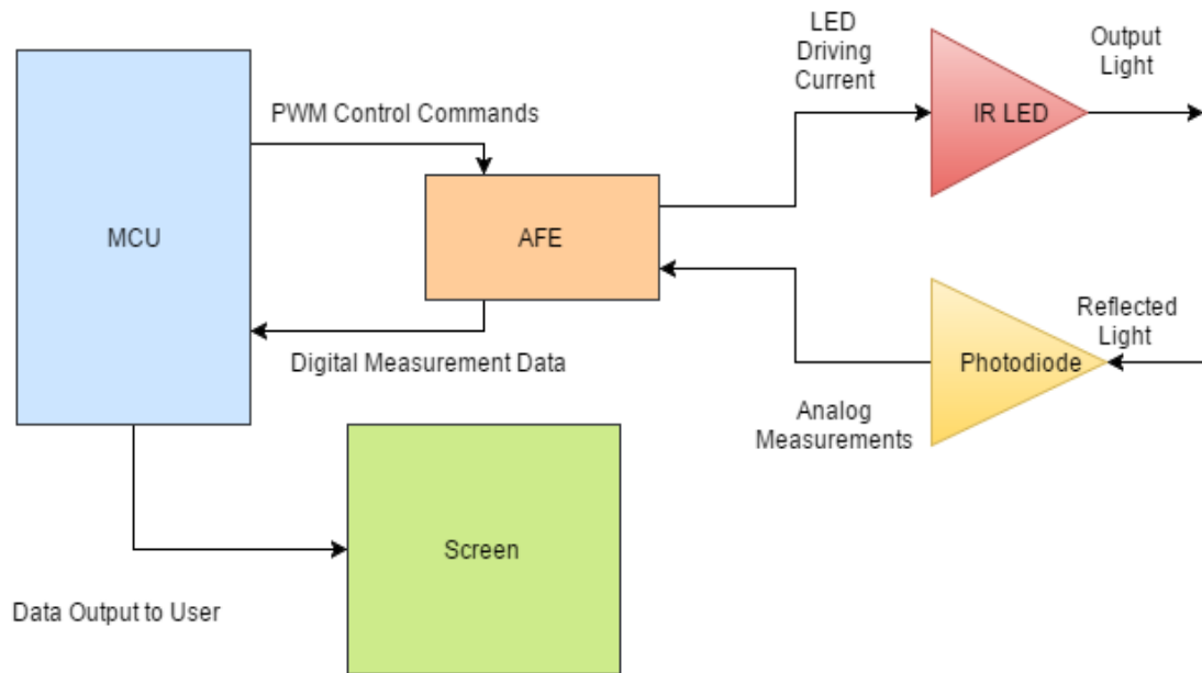
Figure 49: Pulse Sensor Communication Diagram
