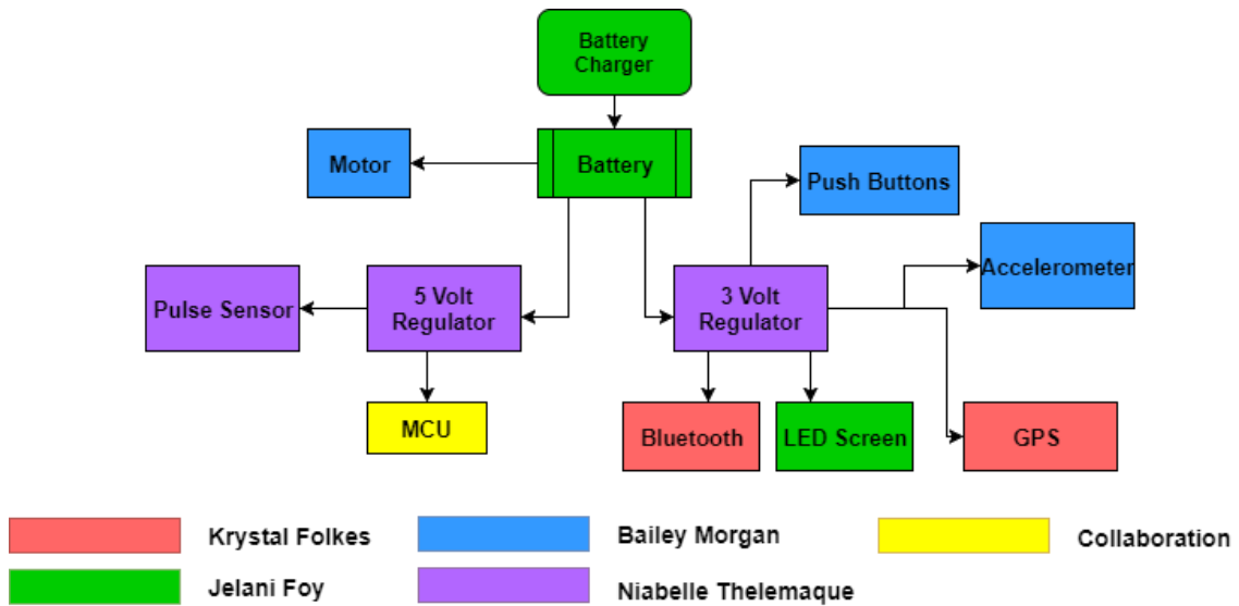
Figure 47: Power Block Diagram
