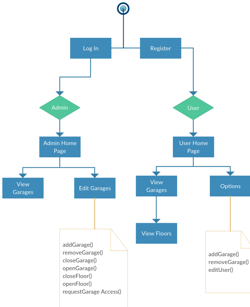
Figure 7.13 - Website Page Flow
