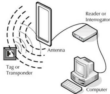
Figure 6.8.2 - An example of data transmission via RFID tag to reader
