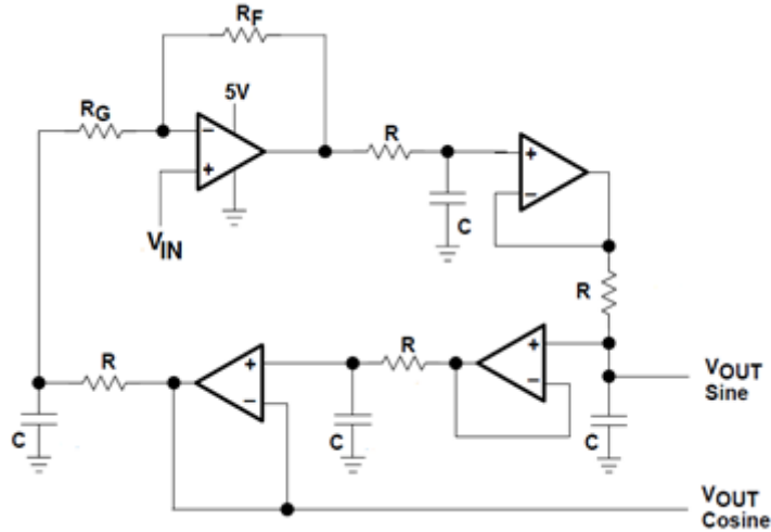
Figure 7.3.2.1 – Bubba Oscillator (Texas Instrument – Sine Wave Oscillator SLOA060)
