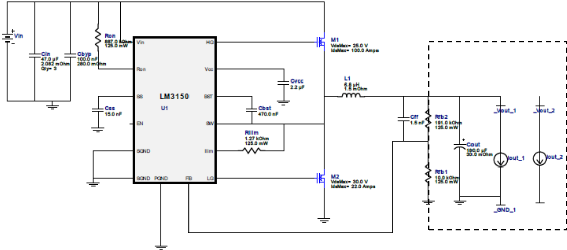
Figure 7.3.1.6 - Schematic Design for the DC-DC 12V 13A output Circuit The Input will be 14V supply from the deep cycle battery to to the LM3150 and the output terminal will be connected to load#1 (the 100W DC-to-AC inverter ) and load #2 (the 24W solenoid #1)
