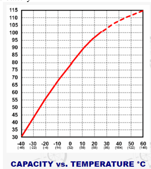
Figure 6.2.1 Battery capacity vs Temperature
