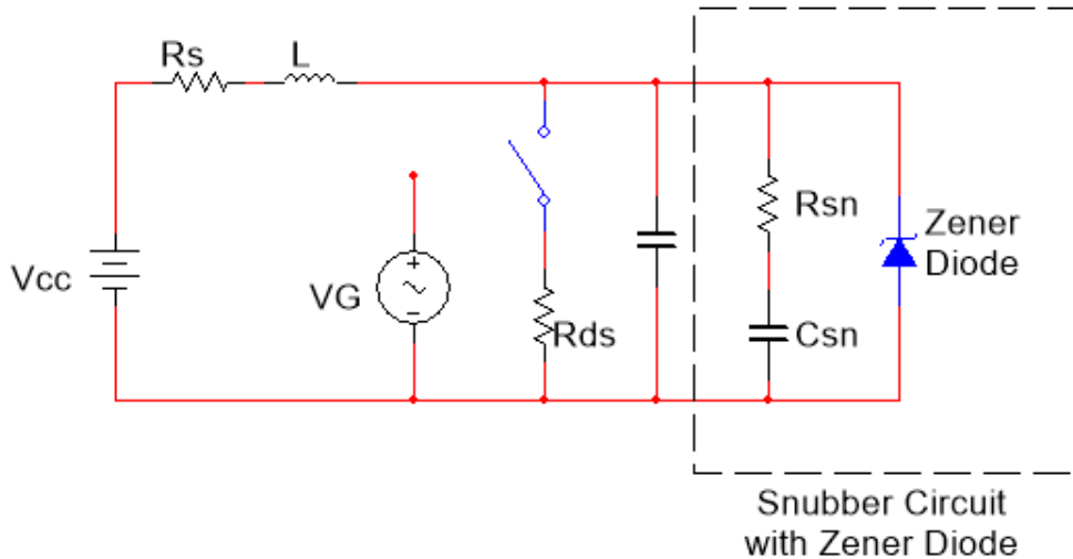
Figure 7.3.3.3 – Inductive Load Circuit with Snubber and Zener Diode
