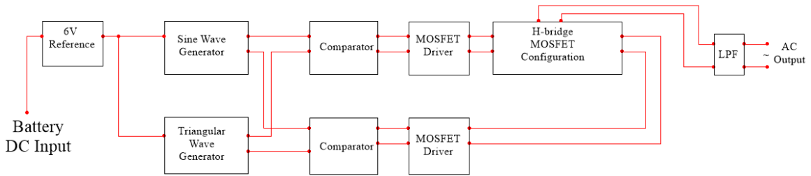
Figure 7.3.3.13 – DC-to-AC Converter Block Diagram
