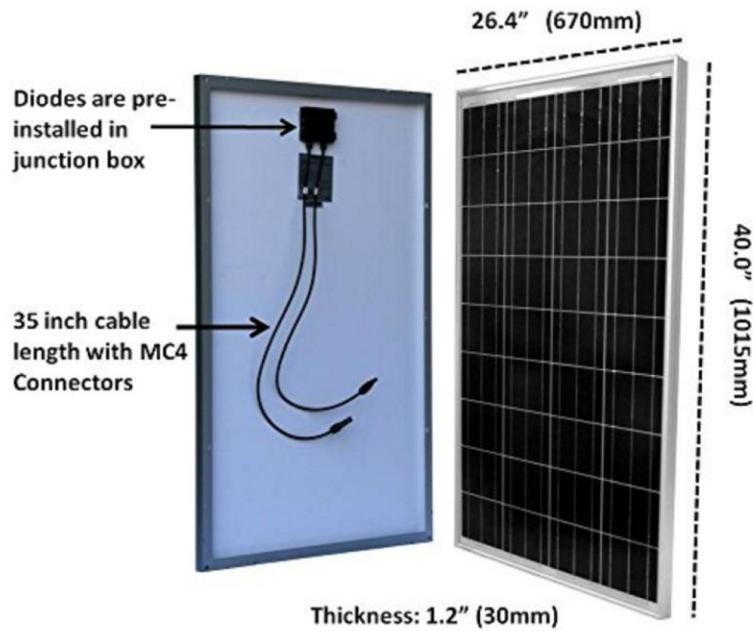
Figure 7.3.2.1 - 100W Polycrystalline Solar Panel from WindyNation (reprint with permission from WindyNation)
