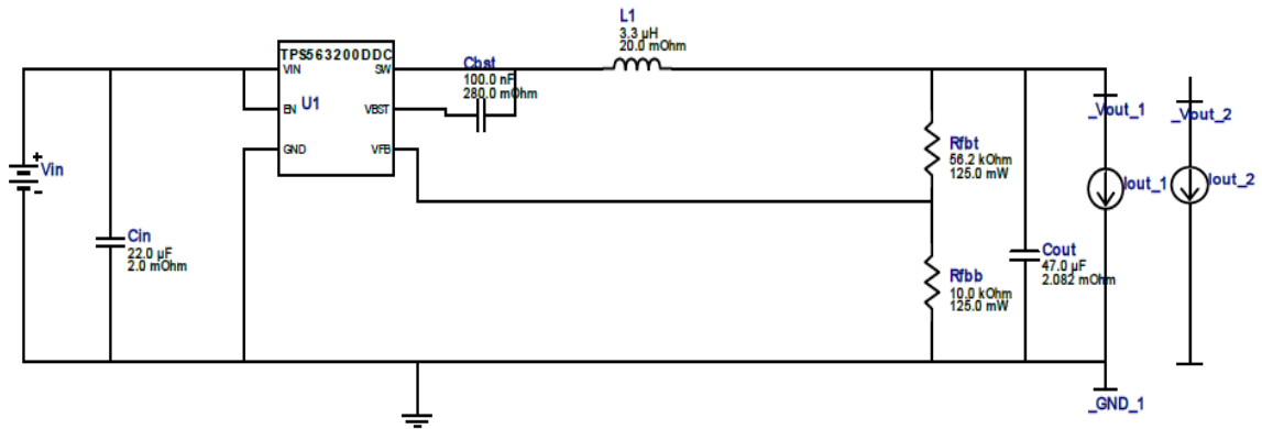
Figure 7.3.1.11 – Schematic design for supply #5
