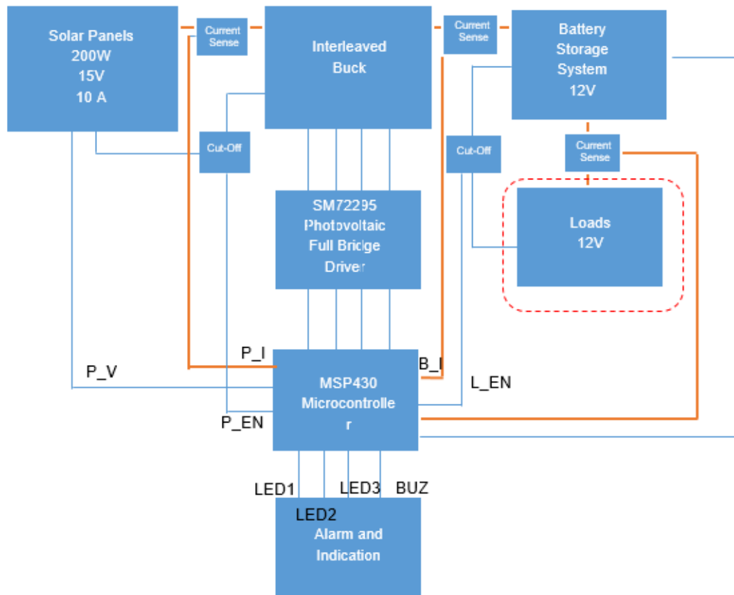
Figure 7.3 - MPPT Charge Controller Block Diagram
