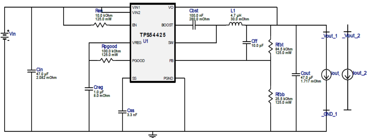
Figure 7.3.1.10 - Schematic Design of the Supply #4 Circuit
