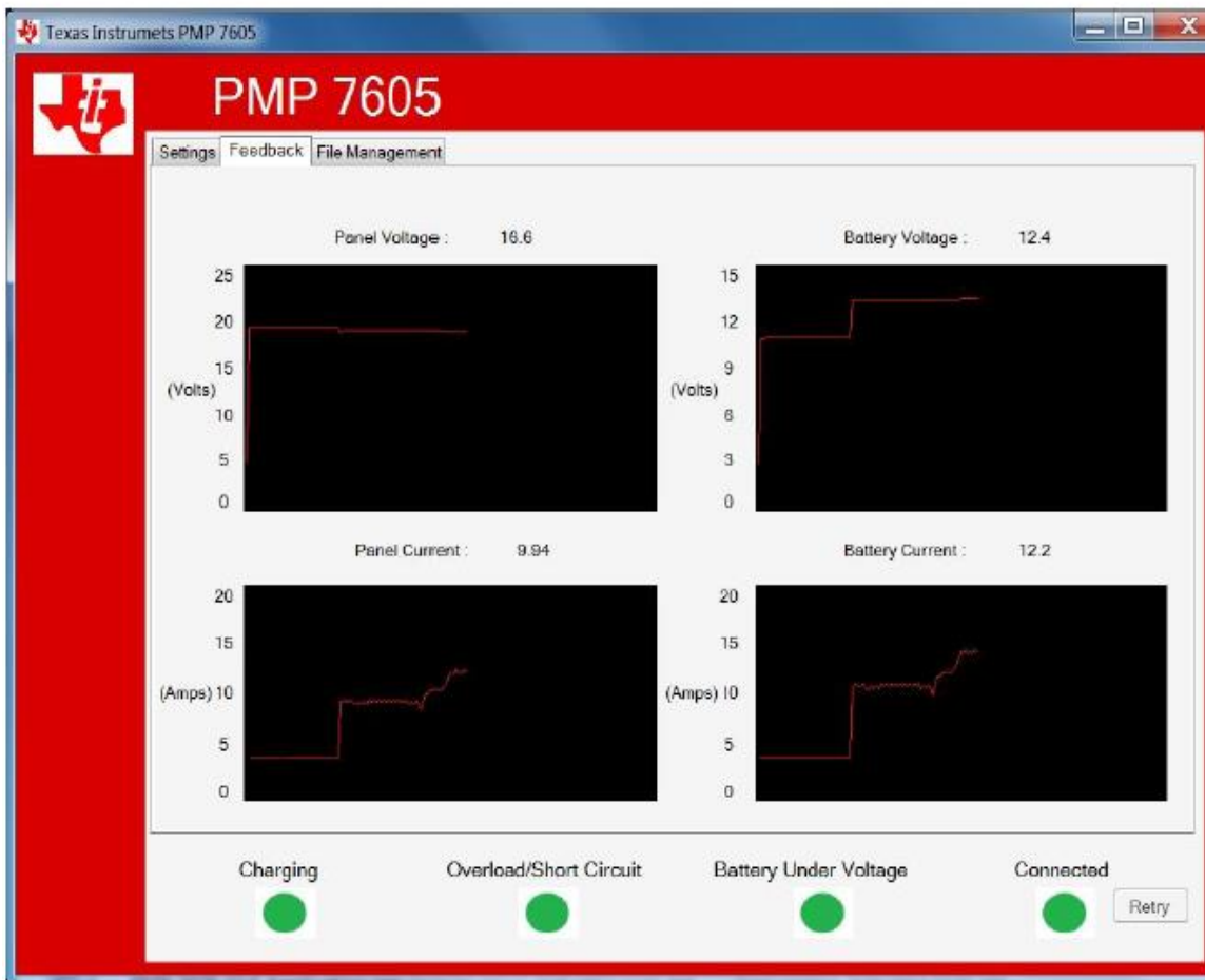
Figure 8.5.1.4 - Graphical Data Reading for PMP7605 Device (Pending Permission from Texas Instrument)
