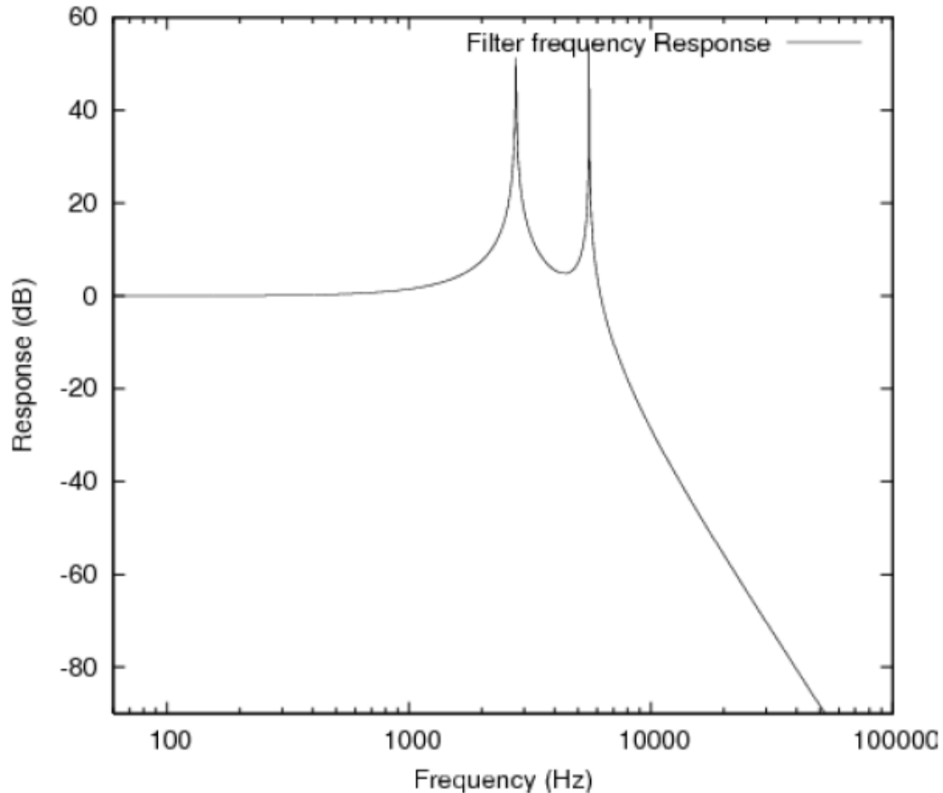
Figure 7.3.2.11 - Filter Frequency Response (Permission is pending from www.wpi.edu )
