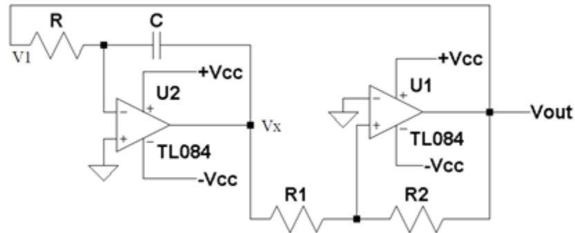
Figure 7.3.2.2 - Triangular-square wave waveform generator (EEL 4309 Lab Manual)
