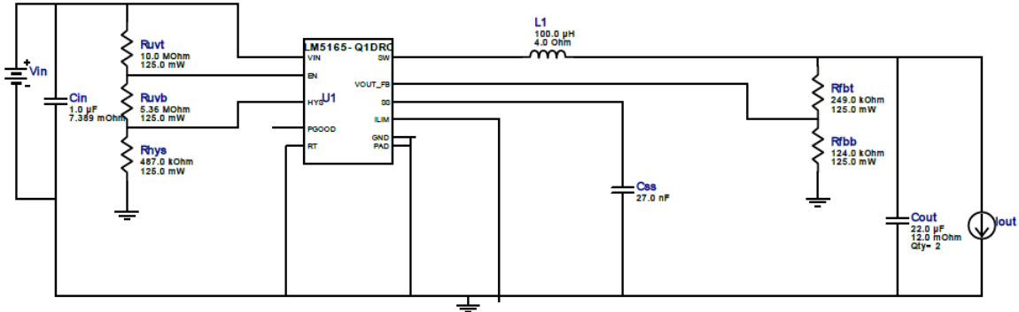
Figure 7.3.1.8 - Schematic Design of the Supply #3 Circuit
