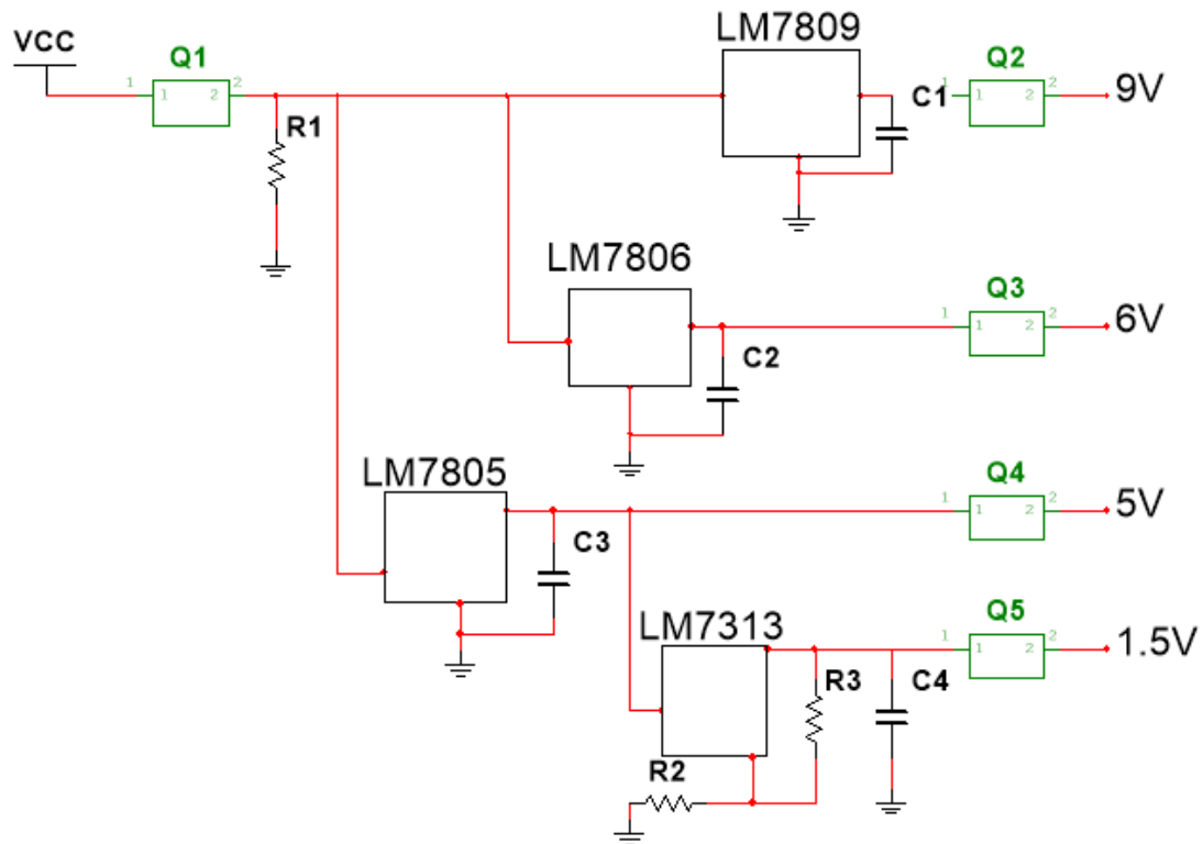
Figure 7.3.3.1 - DC-to-DC Converter with Multiple Outputs
