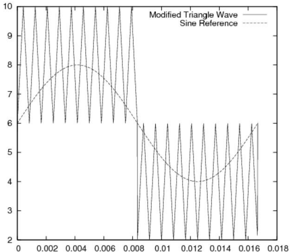
Figure 7.3.2.4 - Modified triangle wave, overlaid with sine reference (Permission is pending from www.wpi.edu)
