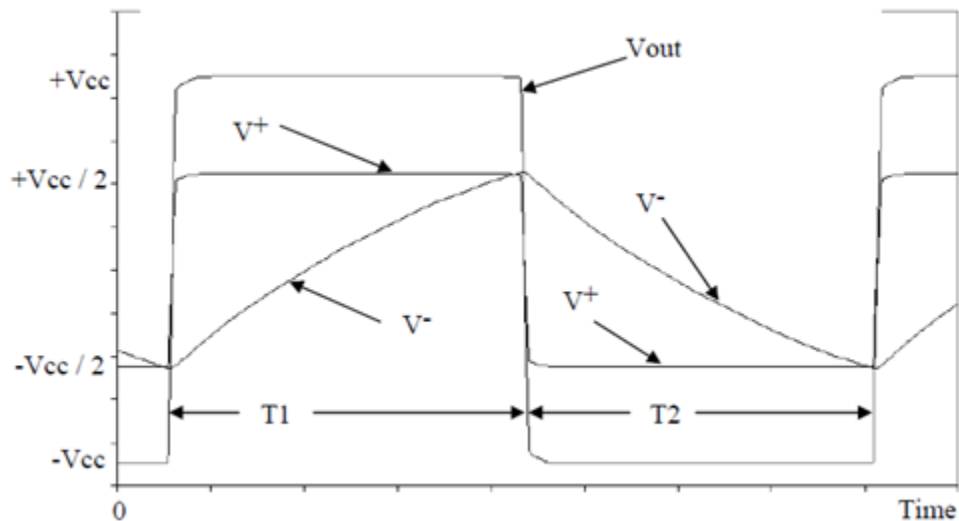
Figure 7.3.2.3 - The Schmitt trigger oscillator waveforms. (EEE4809 – Electronic II Lab Manual)
