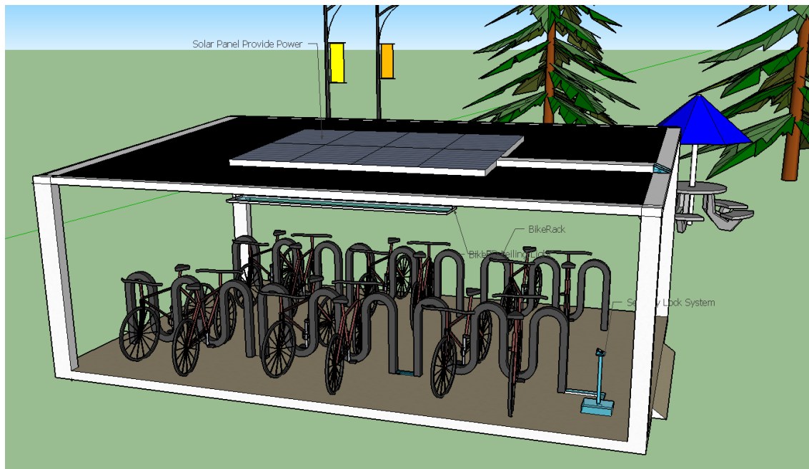
Figure 7.2.1 – Structural Design
