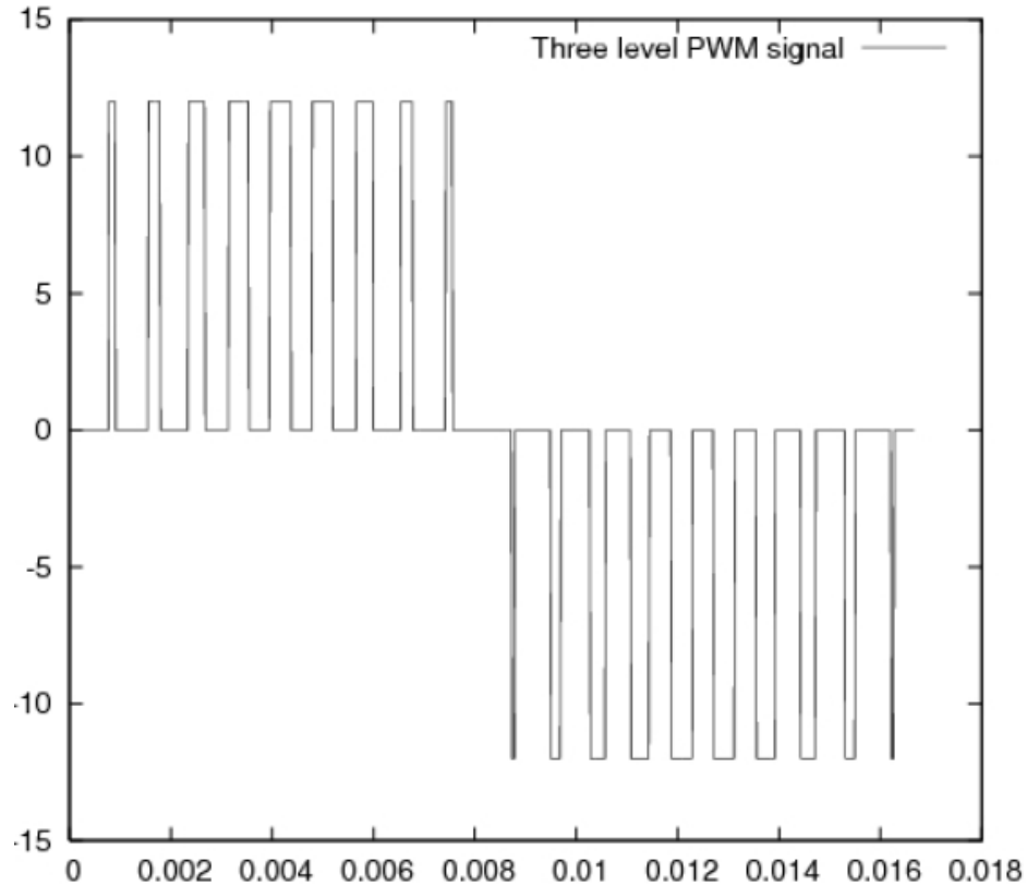
Figure 7.3.2.6 - Trilevel PWM signal (Permission is pending from www.wpi.edu )
