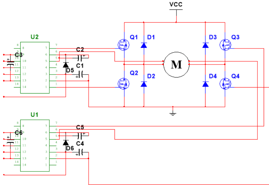
Figure 7.3.2.8 - H-bridge with MOSFET driver
