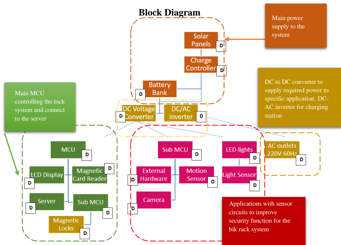
Figure 7.1 - Hardware Block Diagram and Engineering tasks
