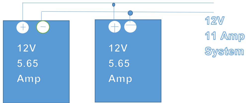
Figure 7.3.2.2 – Solar Panel Connections
