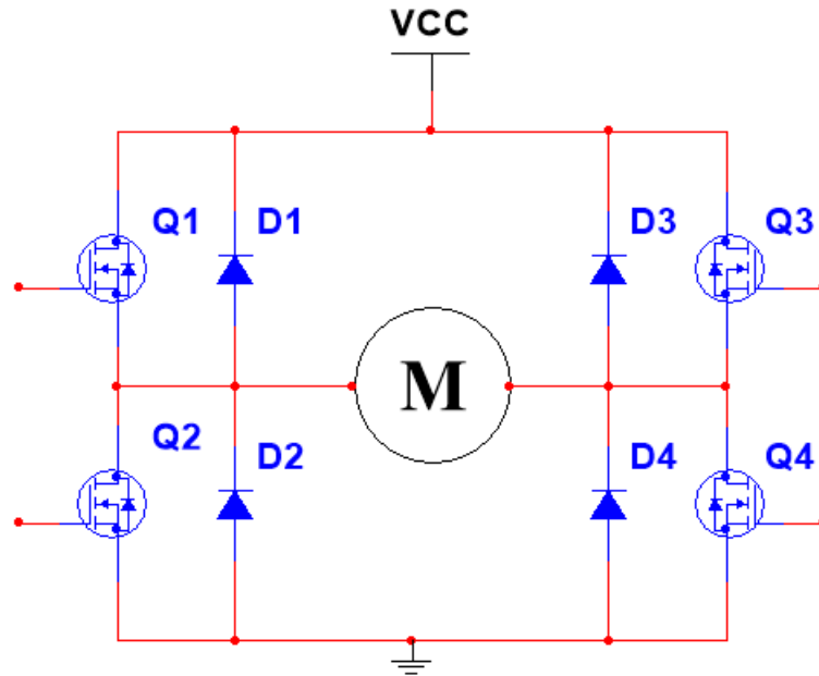
Figure 7.3.2.7 - H-bridge n-channel MOSFET configuration
