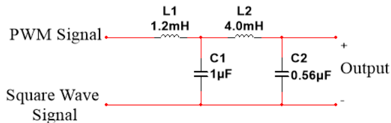
Figure 7.3.2.10 - Two pole LPF
