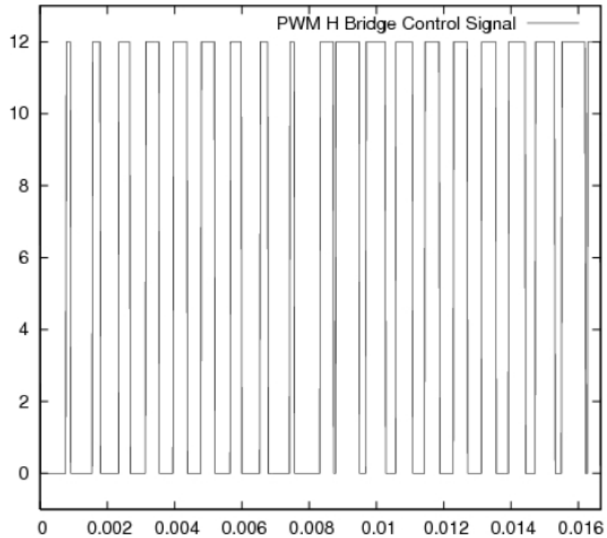
Figure 7.3.2.5 - PWM control signal (Permission is pending from www.wpi.edu)
