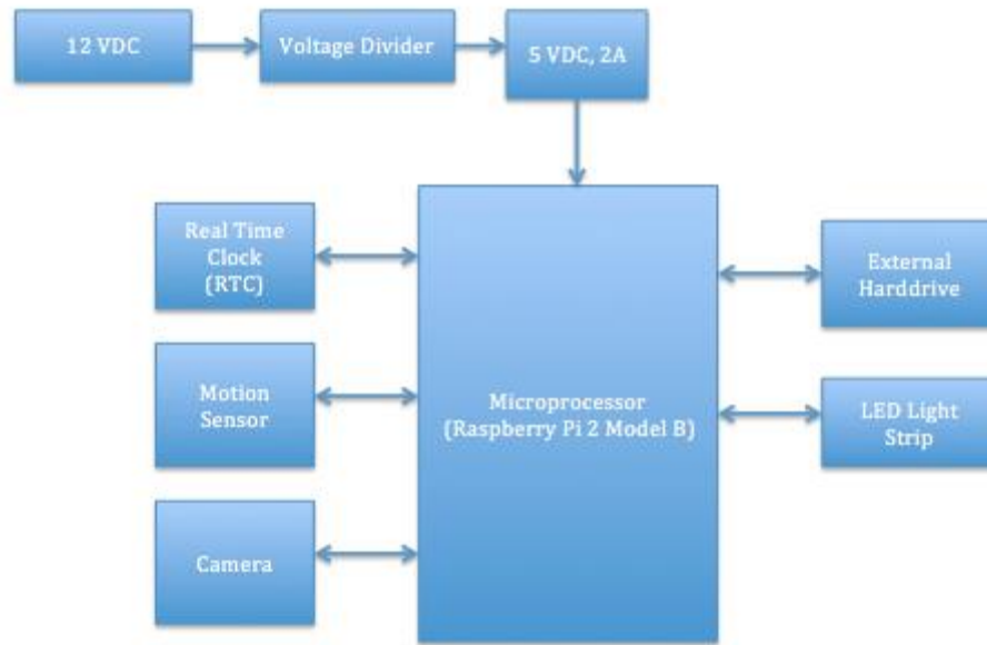
Figure 7.3.3.4 – Block Diagram of Security Camera and Lighting System
