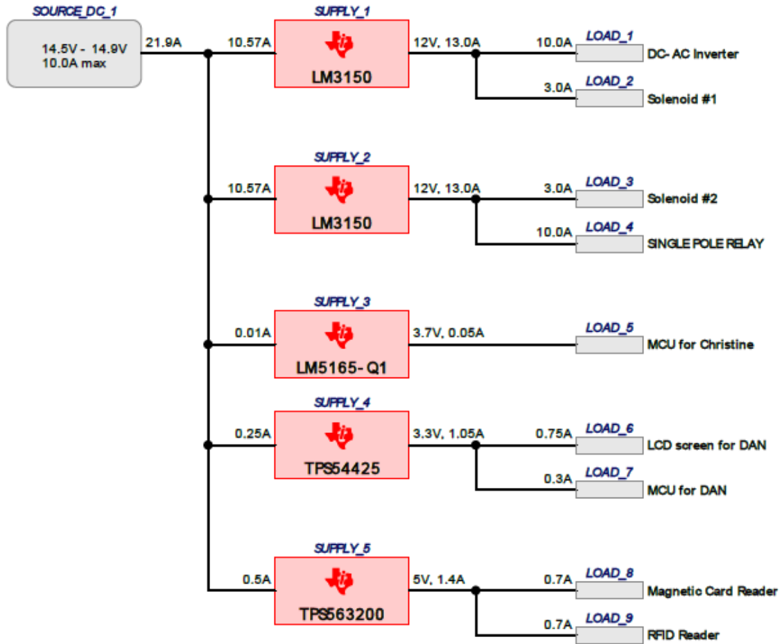
7.3.1.5 - Block Diagram of the Internal Power Distribution System
