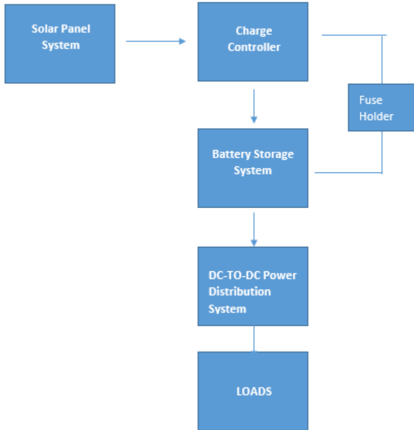
Figure 7.3.1.4 Power Distribution Block Diagram
