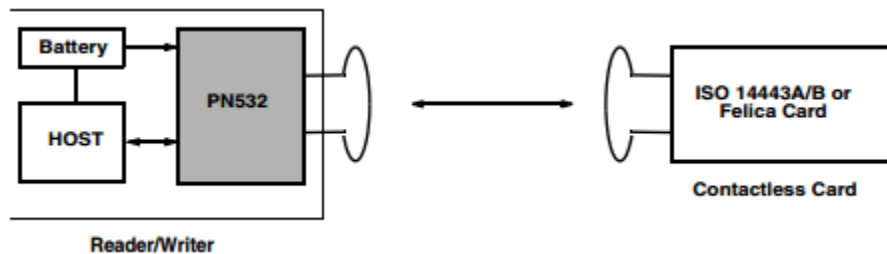
Figure 4.4.4.1 Communication between the RFID reader and an RFID card. Credit to Philips Semiconductors.
