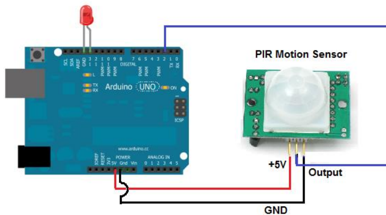
Figure 16 Arduino to PIR Sensor
