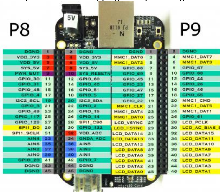
Figure 1 BeagleBone Black With permission from: Let's make robots
