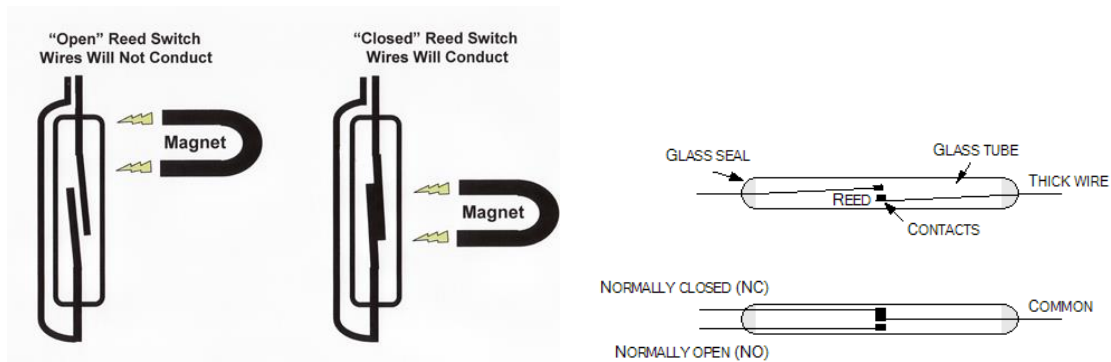
Figure 4a Open vs Closed Reed Switch With permission from: Chicago Sensor
