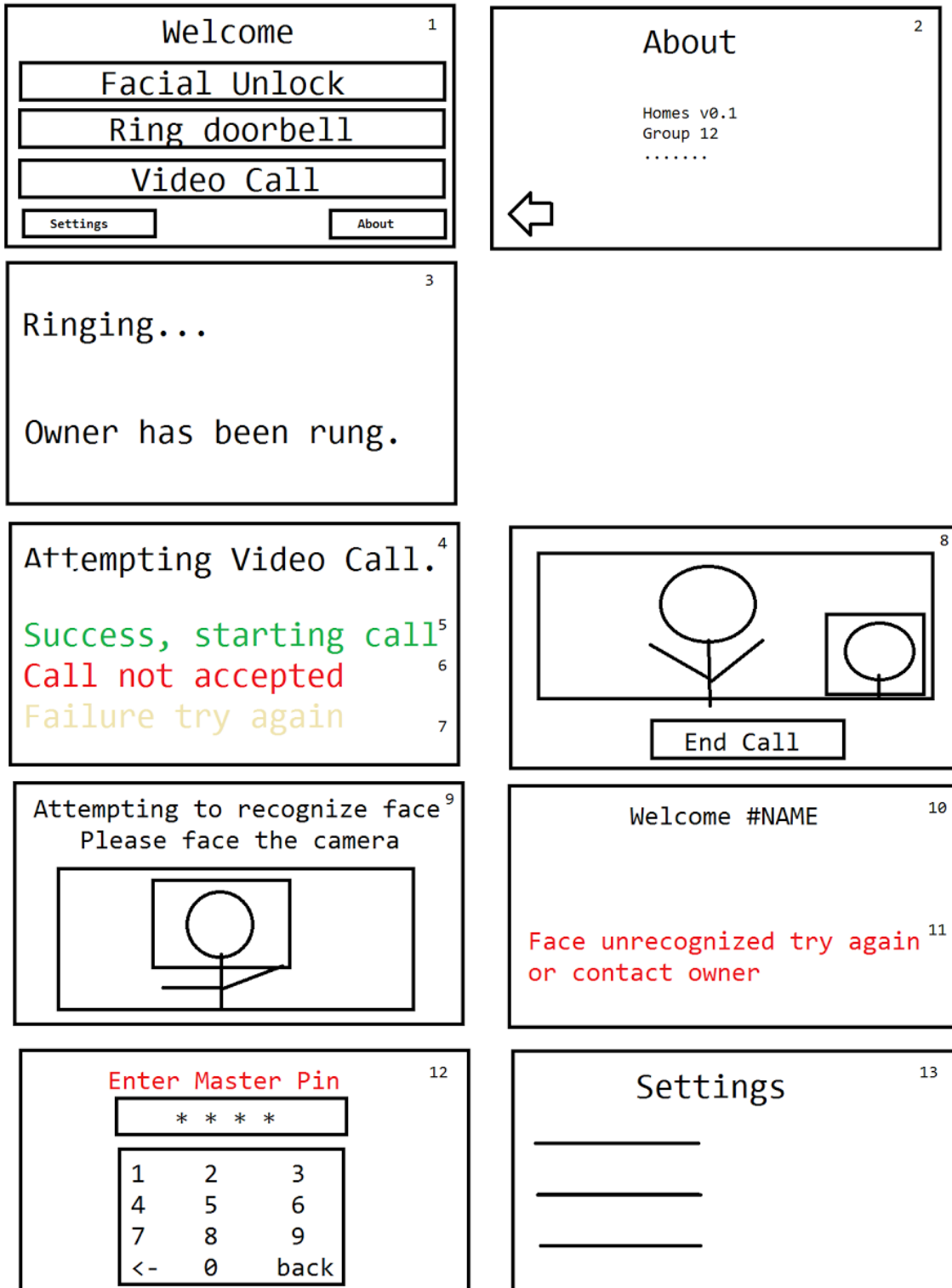
Figure 14 User Interface for LCD
