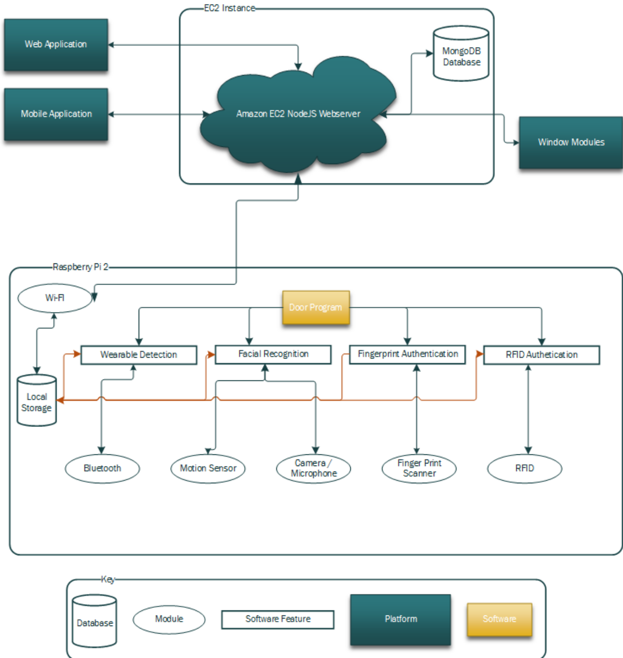
Figure 15 Software Flow Chart
