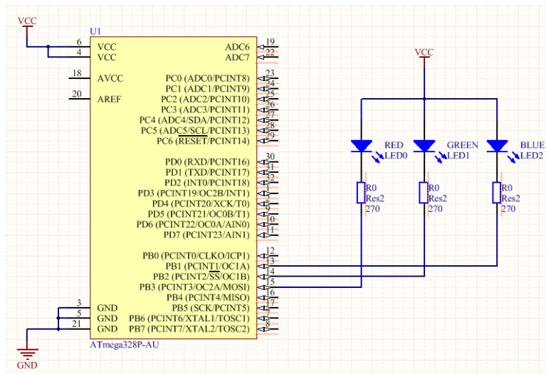
Figure 19 Arduino and RGB LED Pins
