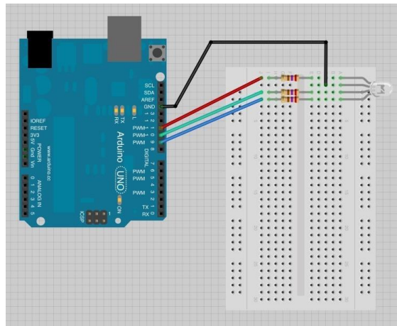
Figure 18 Arduino to RGB LED Circuit Connections
