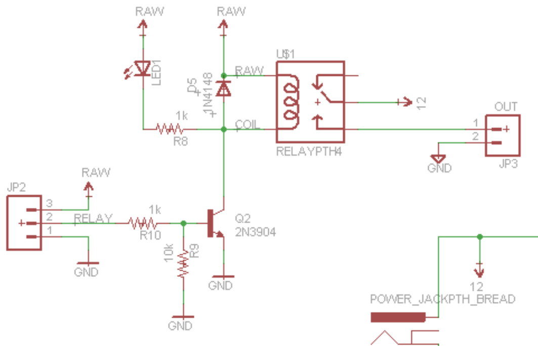
Figure 9 Relay Control Circuit
