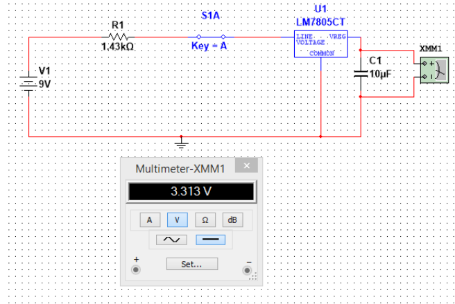
Figure 6b Multisim Schematic
