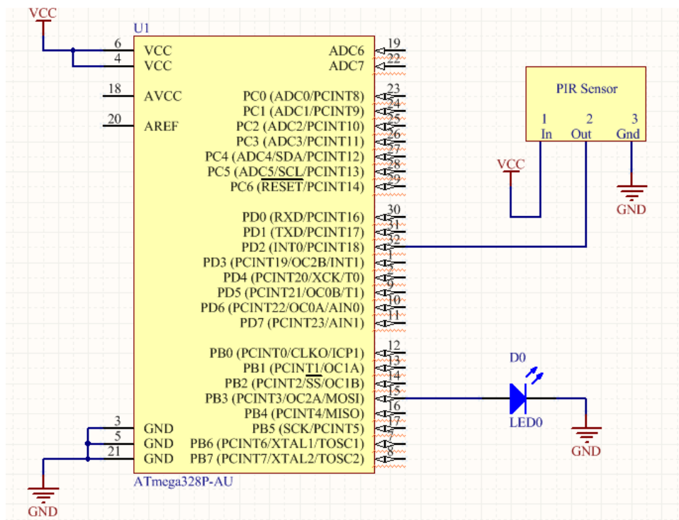
Figure 17 Arduino and PIR Sensor Pins
