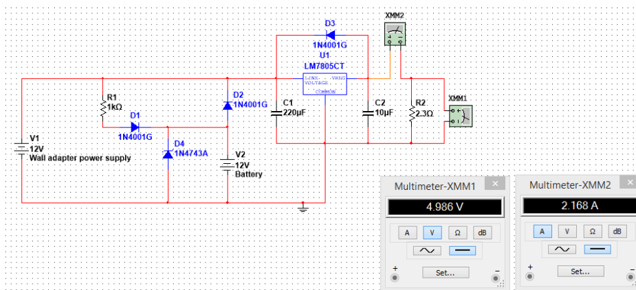
Figure 7 Old Voltage Regulator Circuit with Battery Backup
