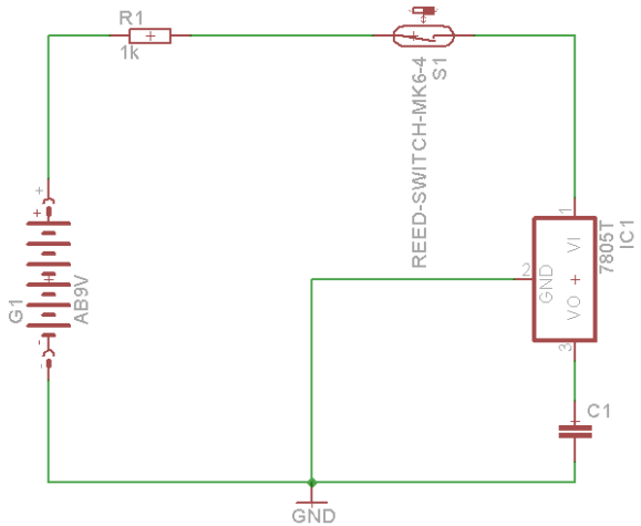
Figure 6a Eagle Schematic
