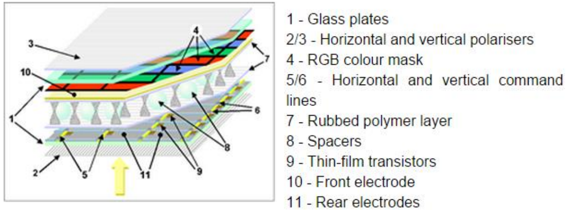
Figure 3 LCD Panel With permission from: Creative Commons
