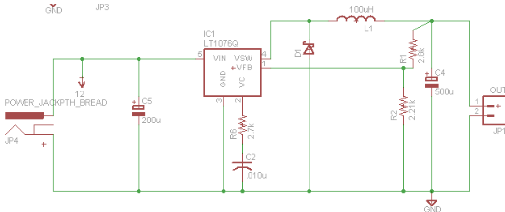
Figure 8 New Voltage Regulator Circuit
