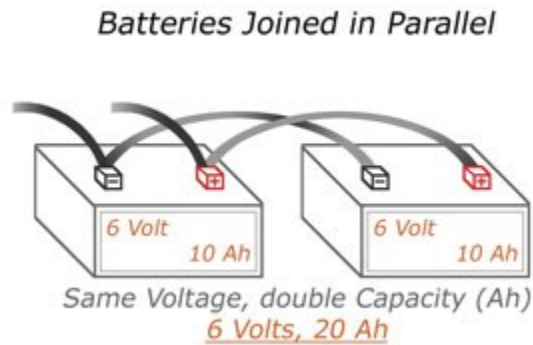
Figure 72: Batteries connected in parallel Source: batterystuff.com
