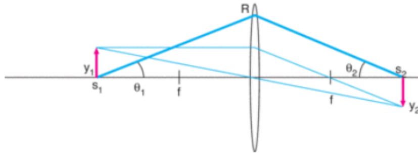
Figure 56: Basic Ray Trace
