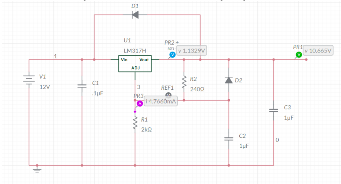
Figure 43: LM317 10V Linear Voltage Regulator
