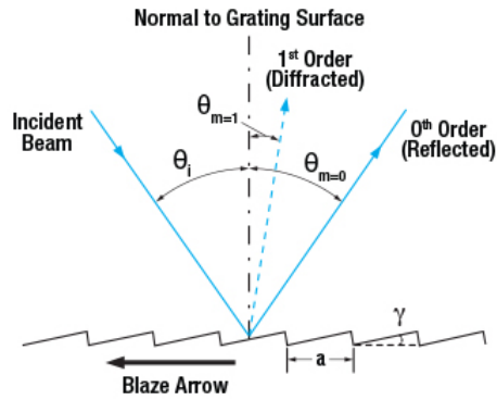
Figure 54: Grating Angular Calculation
