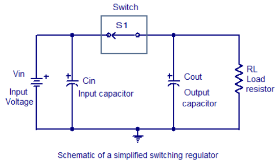
Figure 20: General Switching Voltage Regulator
