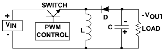
Figure 24: Buck/Boost Converter Circuit Schematic
