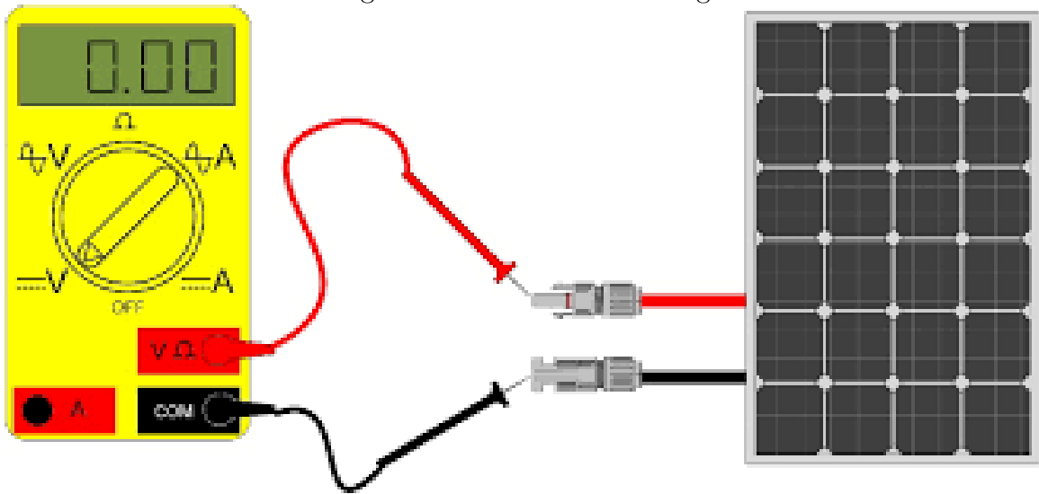
Figure 66: Solar Panel Testing
