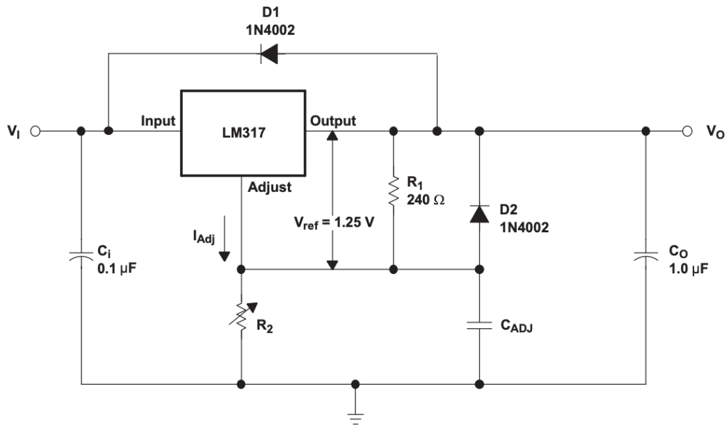
Figure 40: LM317 Linear Voltage Regulator
