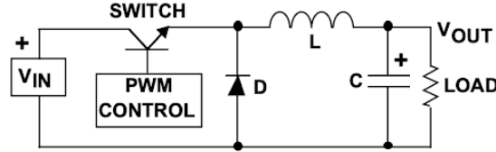
Figure 22: Buck Converter (Step Down) Circuit Schematic
