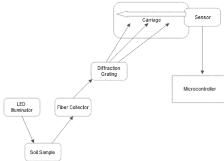
Figure 50: Sensing subsystem block diagram
