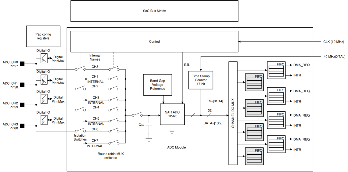
Figure 34: CC3200 ADC module architecture [6]
