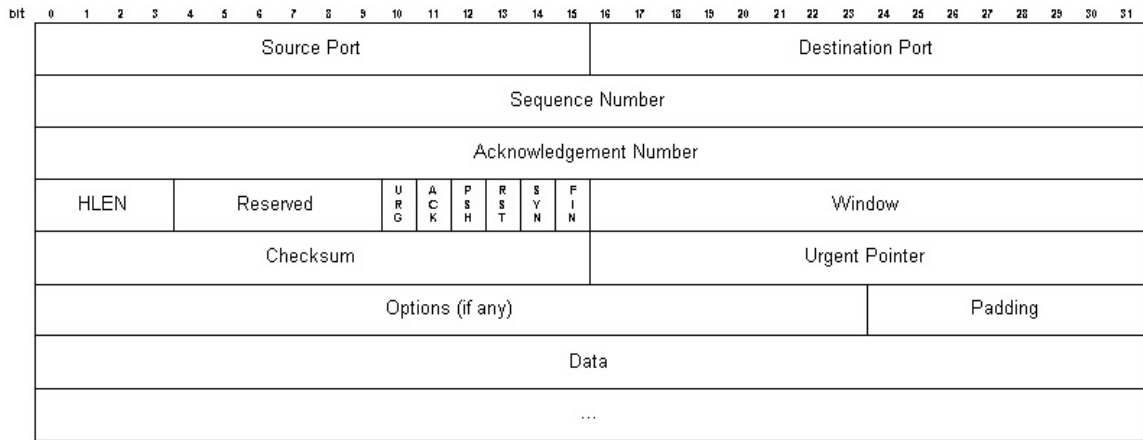
Figure 26: TCP frame [2]
