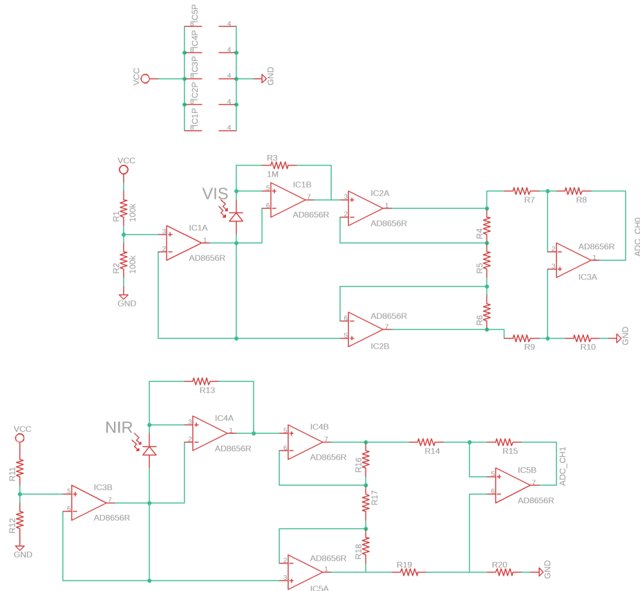
Figure 60: Sensing Schematic
