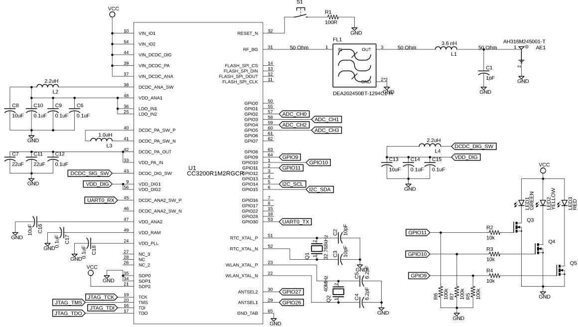
Figure 37: MCU subsystem schematic
