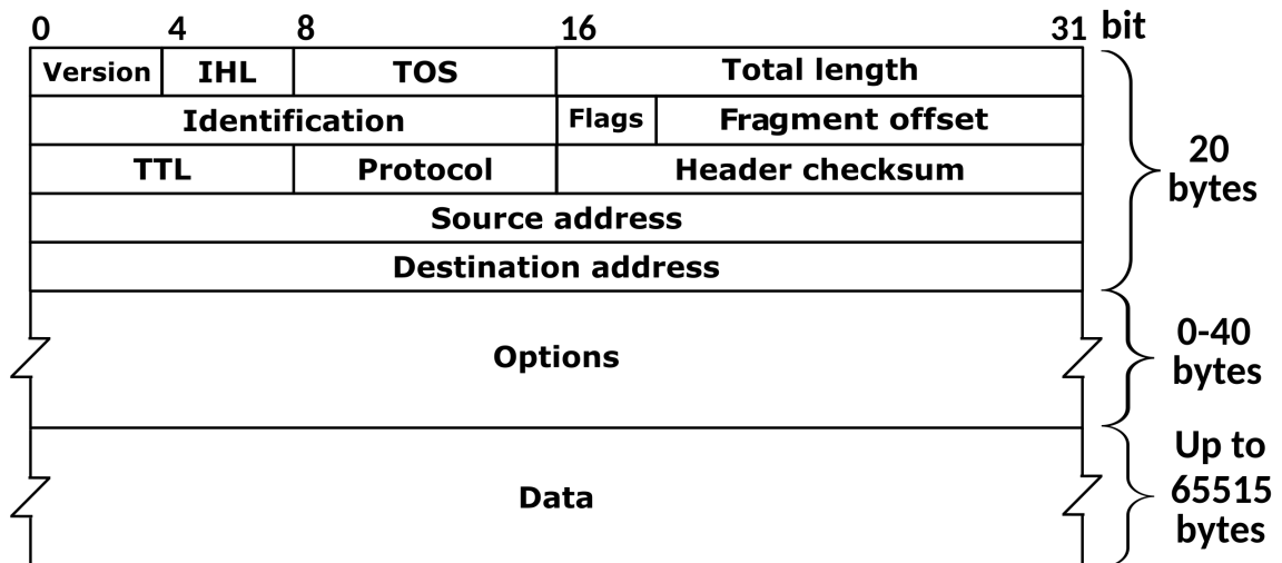
Figure 27: IPv4 frame [3]
