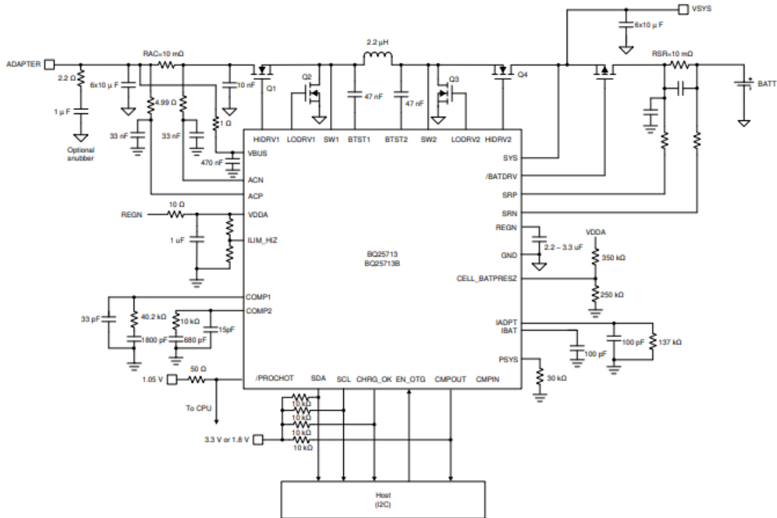
Figure 15: BQ25713 General Application Schematic
