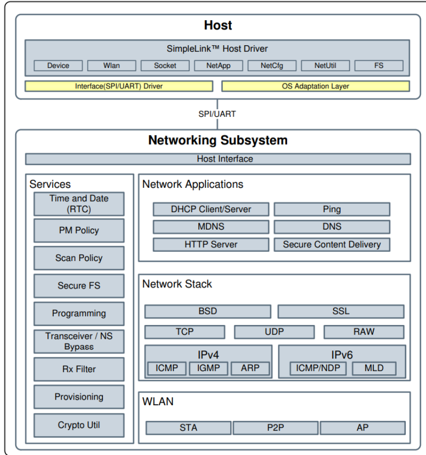
Figure 29: CC3220 networking subsystem [4]
