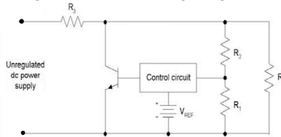
Figure 19: Shunt Voltage Regulator
