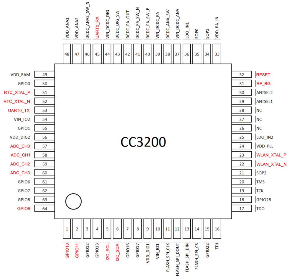
Figure 36: CC3200 pinout diagram
