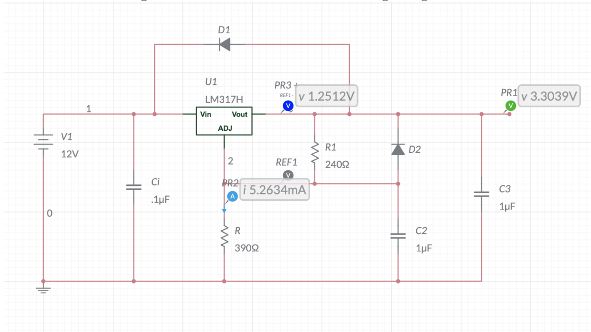
Figure 41: LM317 3.3V Linear Voltage Regulator
