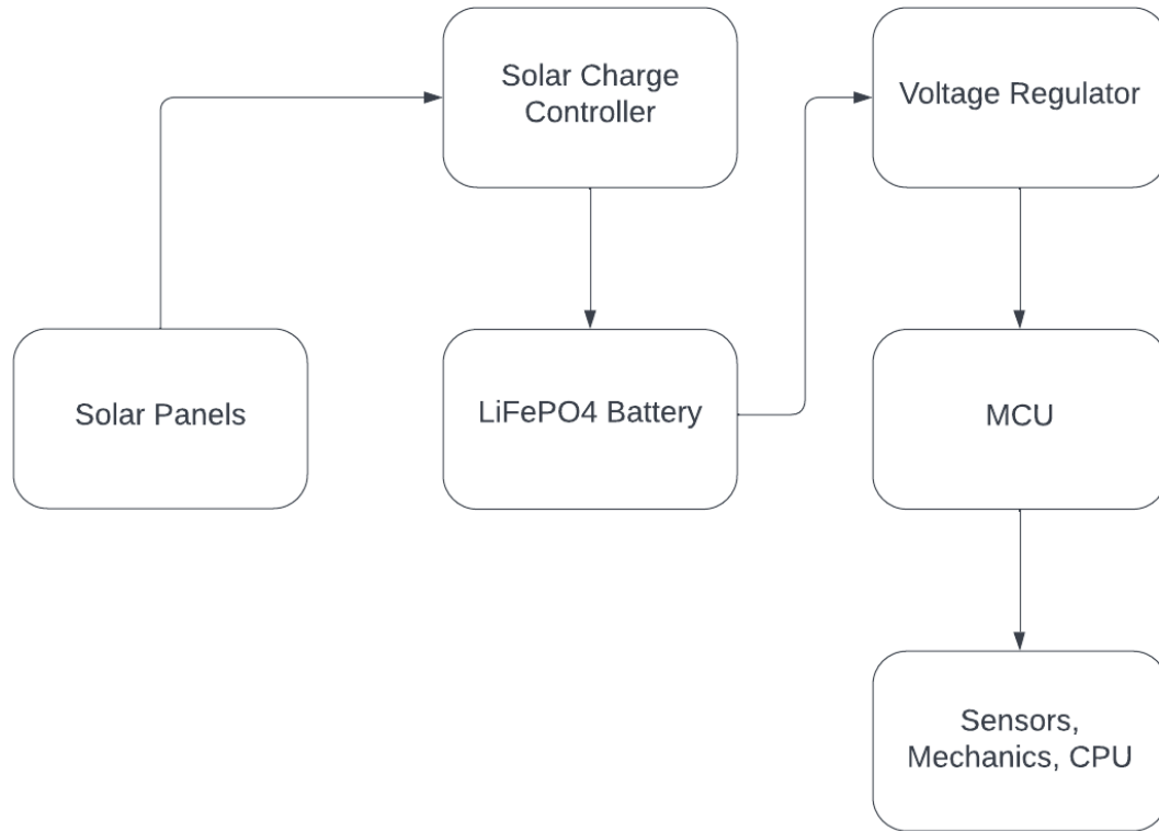
Figure 38: Power subsystem block diagram
