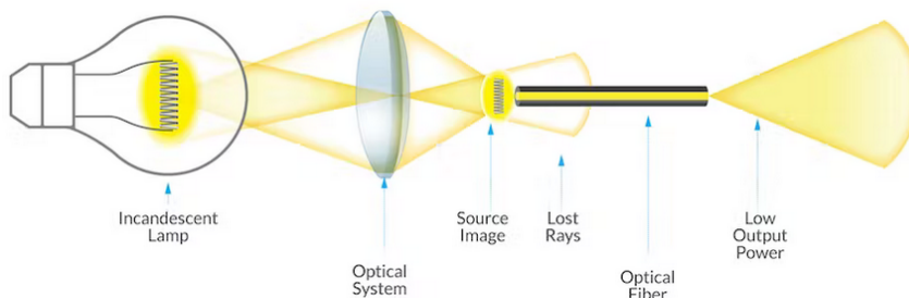
Figure 53: Coupling a diffuse light into a fiber
