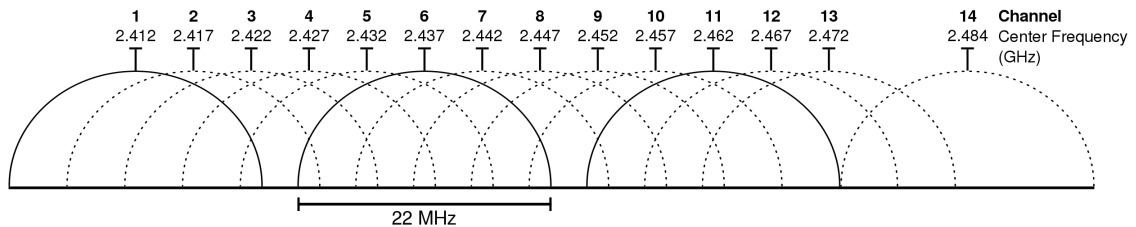
Figure 25: 802.11b/g/n channels [1]
