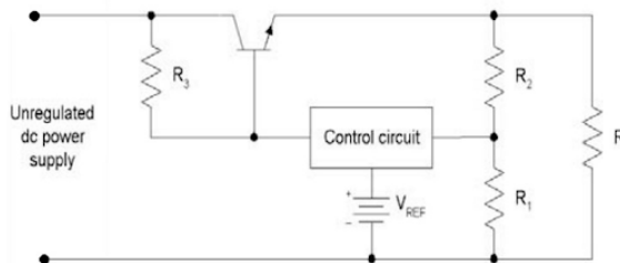
Figure 18: Series Voltage Regulator
