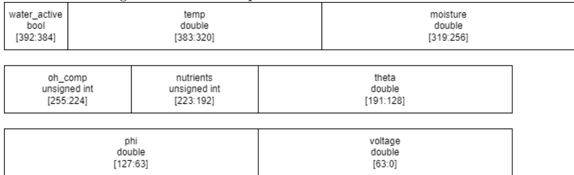
Figure 33: Bitwise representation of data sent to AWS
