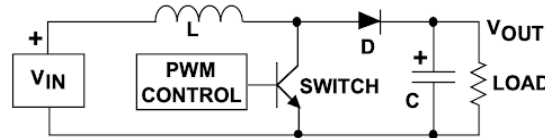
Figure 23: Boost Converter (Step Up) Circuit Schematic
