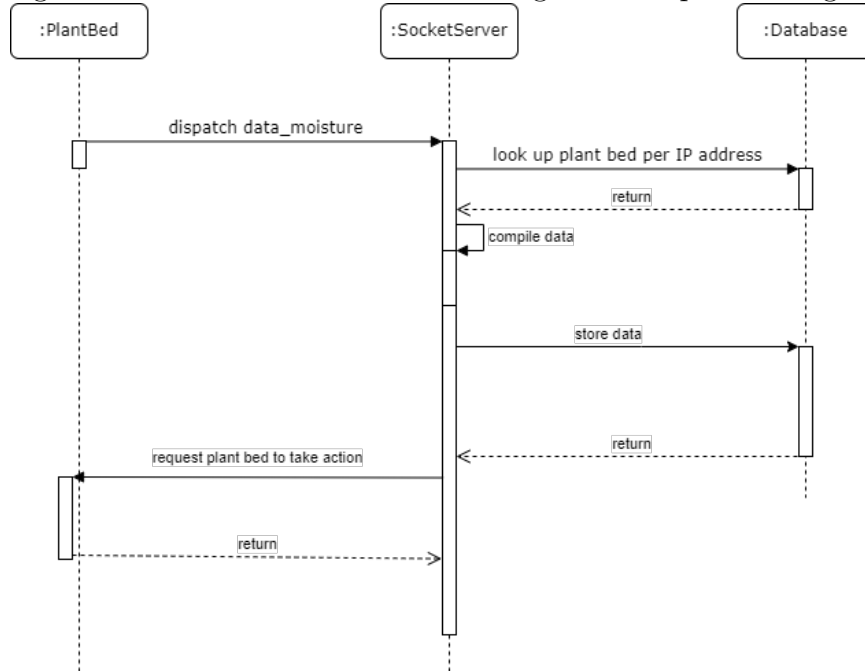
Figure 65: Web-Plant Bed Socket Integration Sequence Diagram
