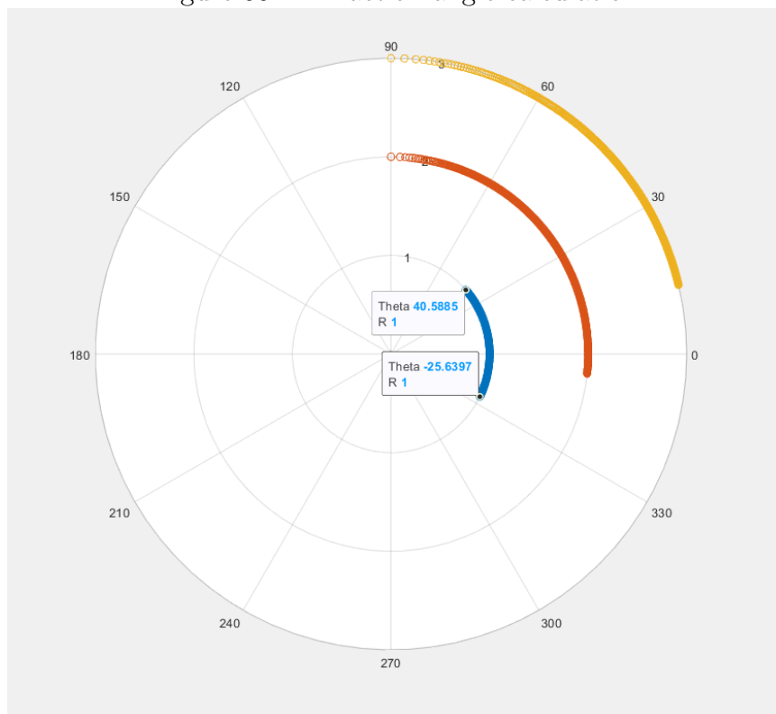
Figure 55: Diffraction angle calculation
