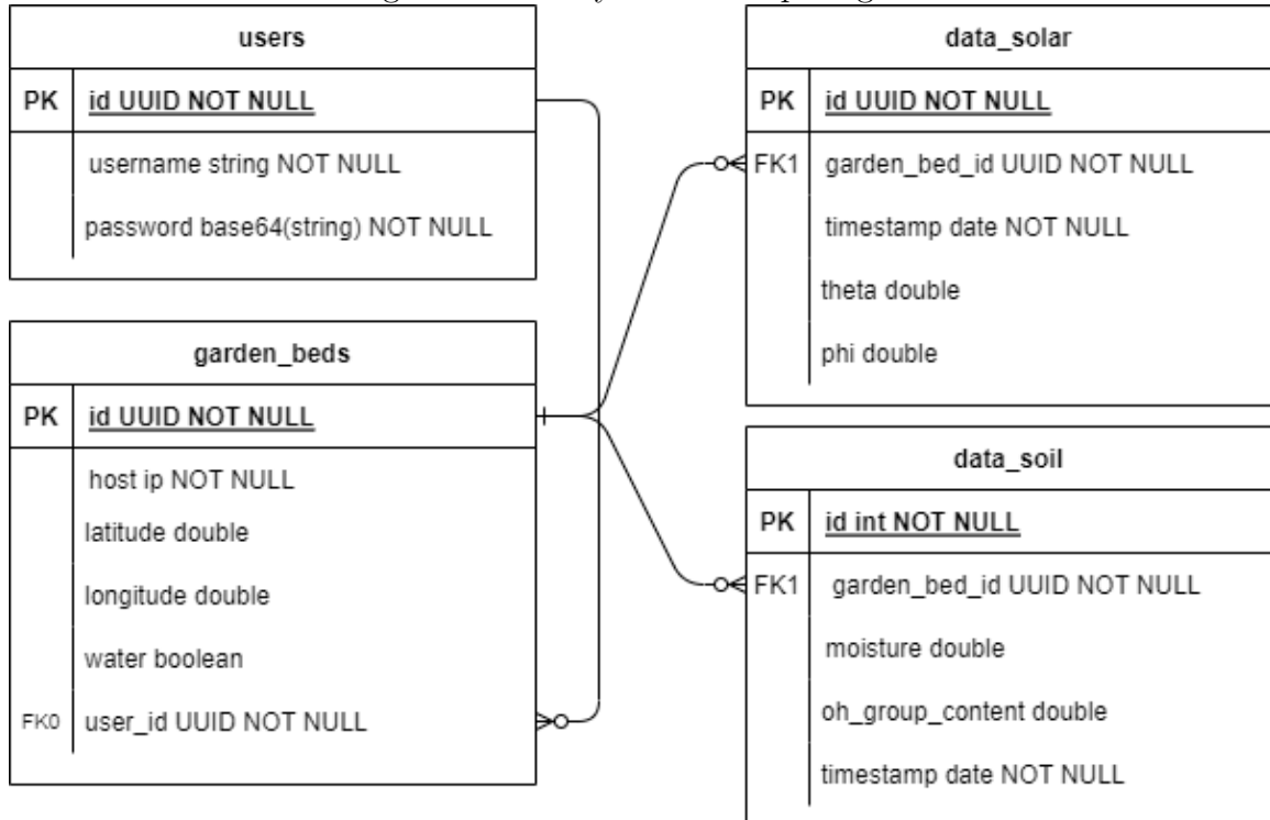
Figure 63: Entity relationship diagram
