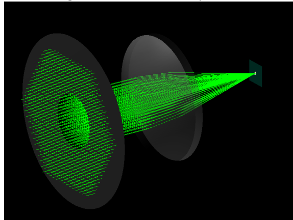
Figure 57: Sensor Ray Trace
