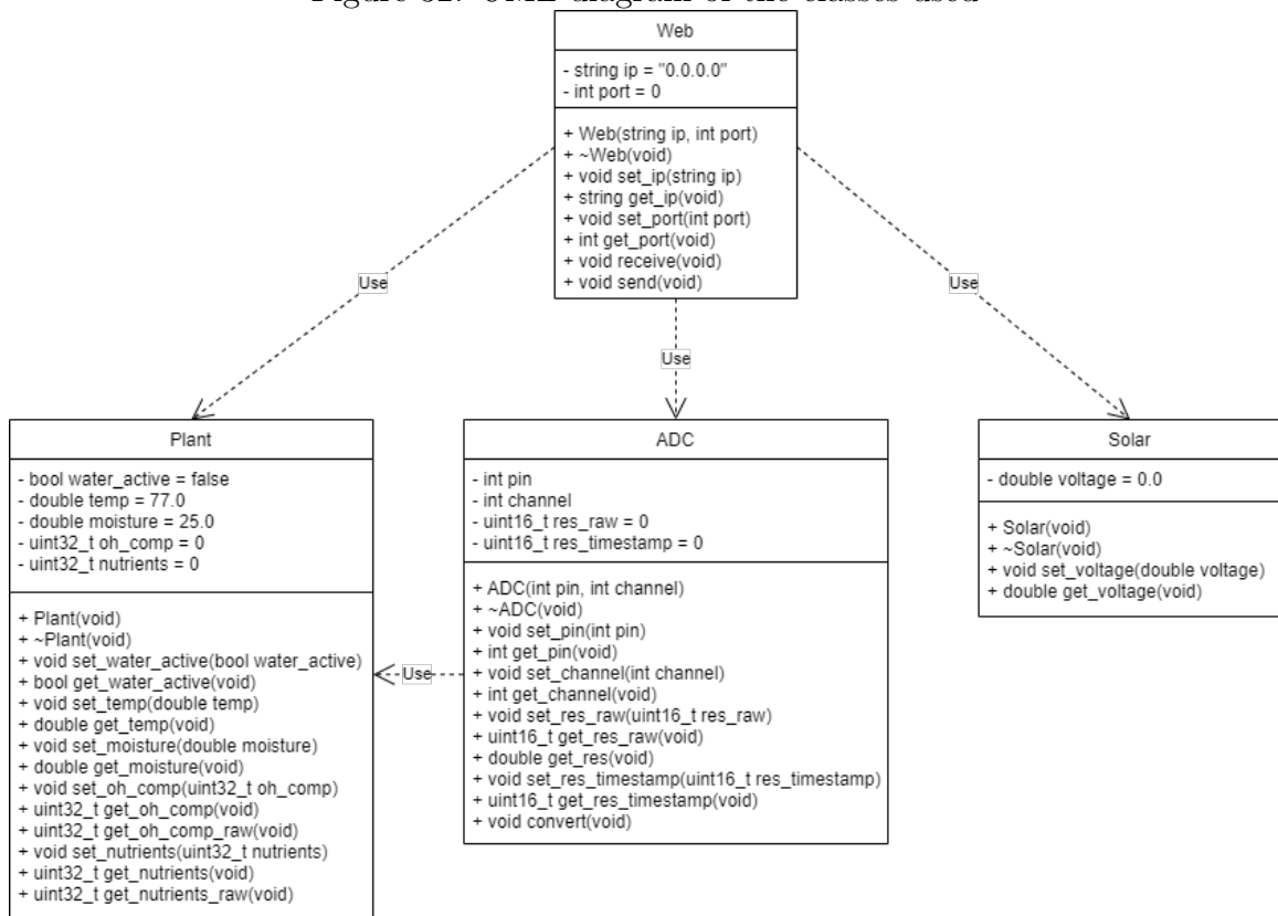
Figure 32: UML diagram of the classes used
