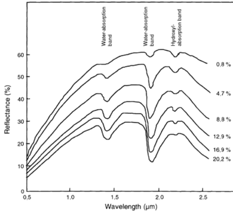
Figure 61: Soil Spectrograph
