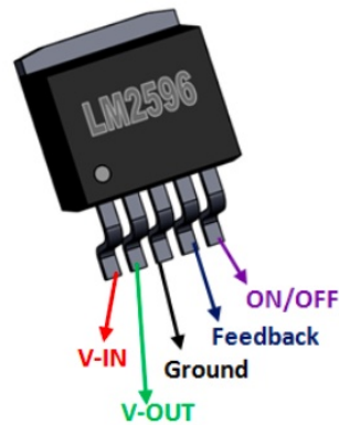
Figure 21: LM2596 Pin Diagram
