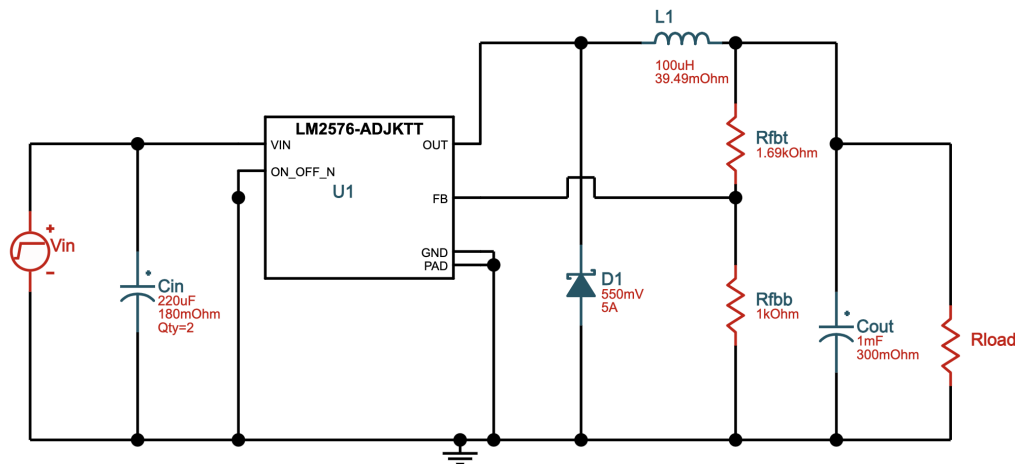
Figure 47: LM2576 WEBENCH Design
