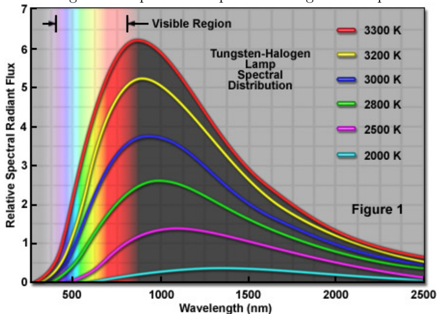
Figure 51: Spectral Output of a Tungsten Lamp
