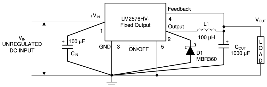
Figure 44: LM2576 Fixed Switching Voltage Regulator
