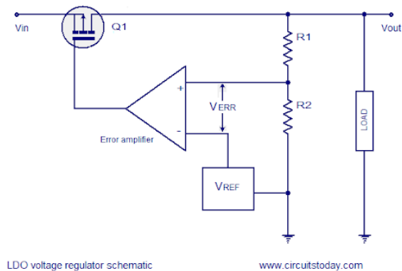
Figure 16: General Linear Voltage Regulator Circuit Schematic
