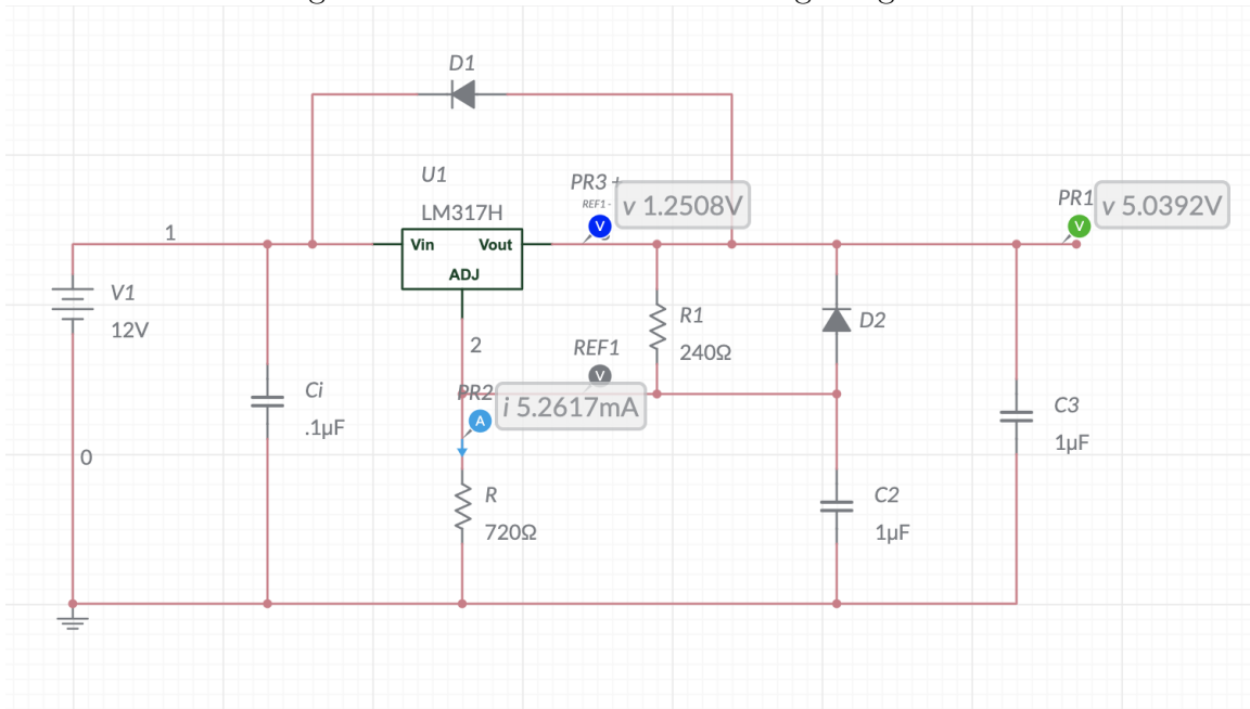
Figure 42: LM317 5V Linear Voltage Regulator
