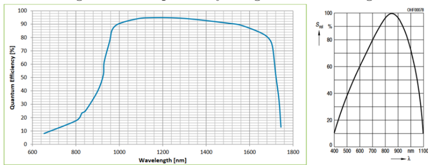
Figure 67: Responsivity Diagrams for Testing
