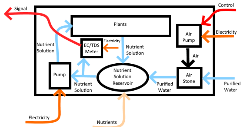
Figure 2.7.5 Hydroponic System
