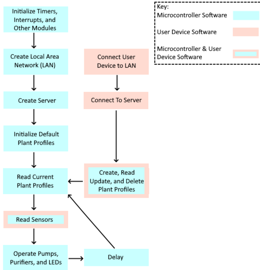
Figure 5.6.5 Block diagram software implementation of our project.
