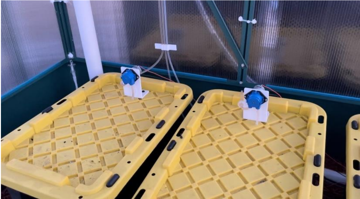
Figure 5.3.1 Nutrient and pH Down deposition system (Missing pH Up)
