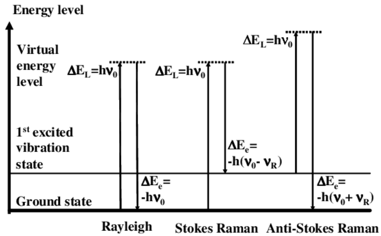
Figure 3.2.2 “Energy diagram for Rayleigh, Stokes Raman, and anti-Stokes Raman scattering.” [52]
