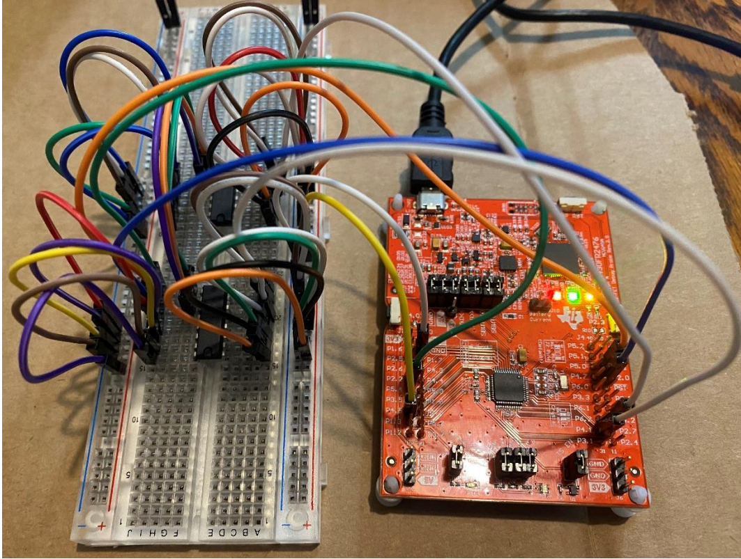
Figure 5.6.7 Liquid level sensing testing environment.
