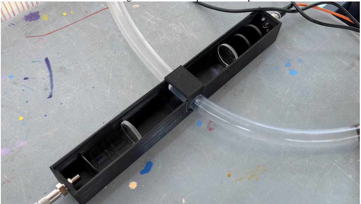
Figure 5.7.2 Final optical setup for spectroscopy analysis through a water sample.
