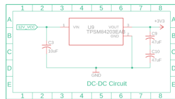
Figure 5.6.3 Final Schematic diagram of our project.
