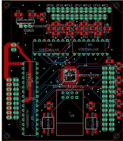
Figure 5.6.4 Image of our final PCB
