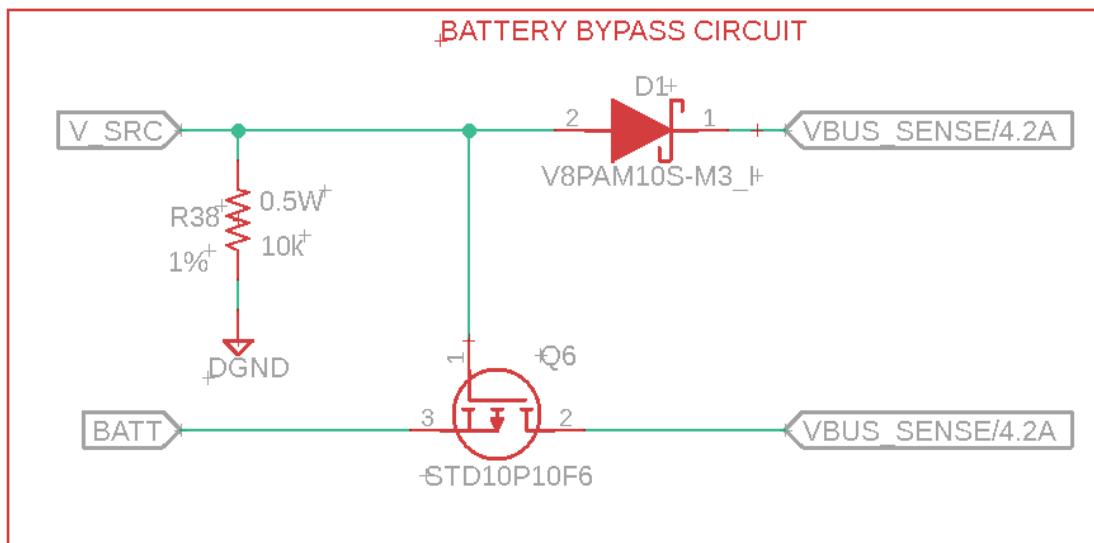
Figure 14:Battery Bypass Circuit
