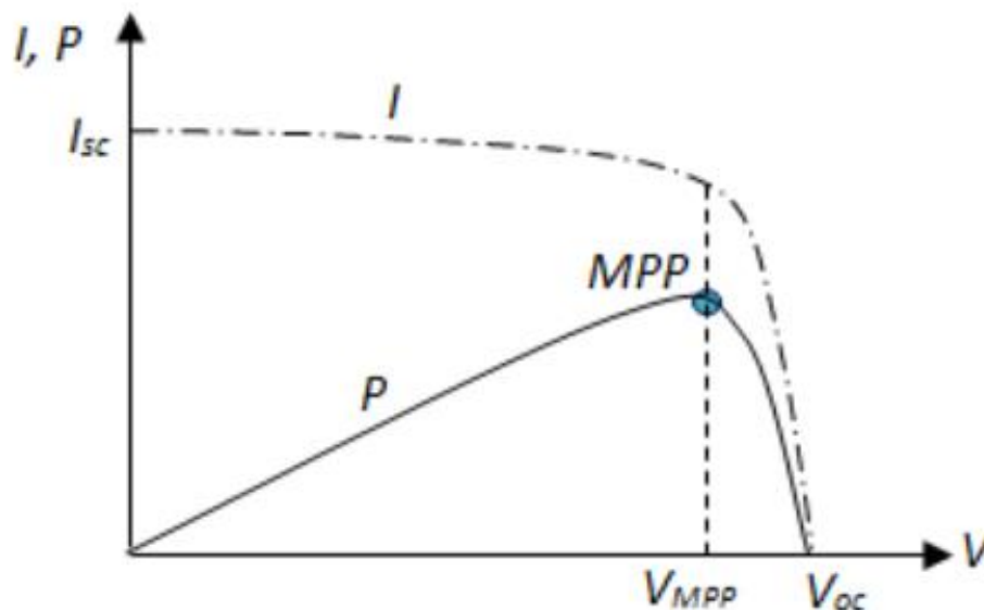
Figure 29: Maximum Power Point Tracking Representation
