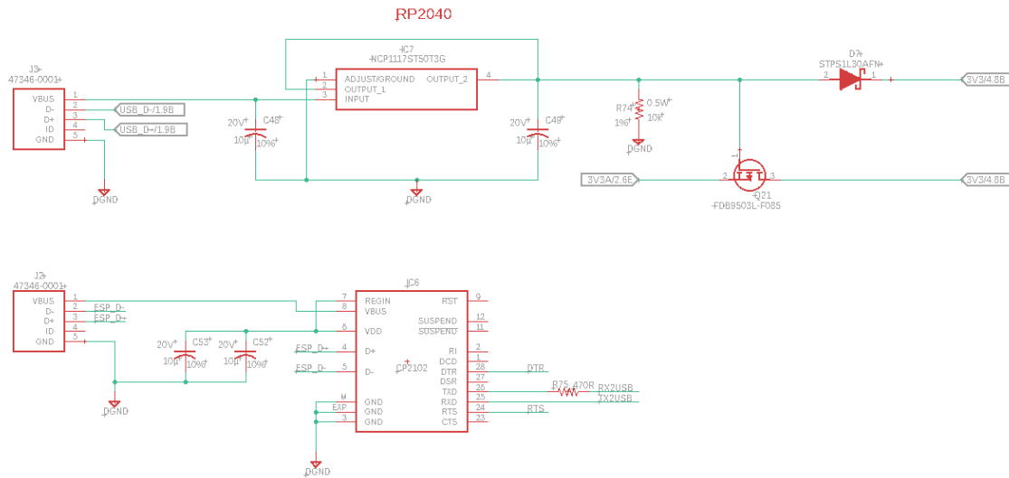
Figure 28: In system Programmability MicroUSB Interfaces
