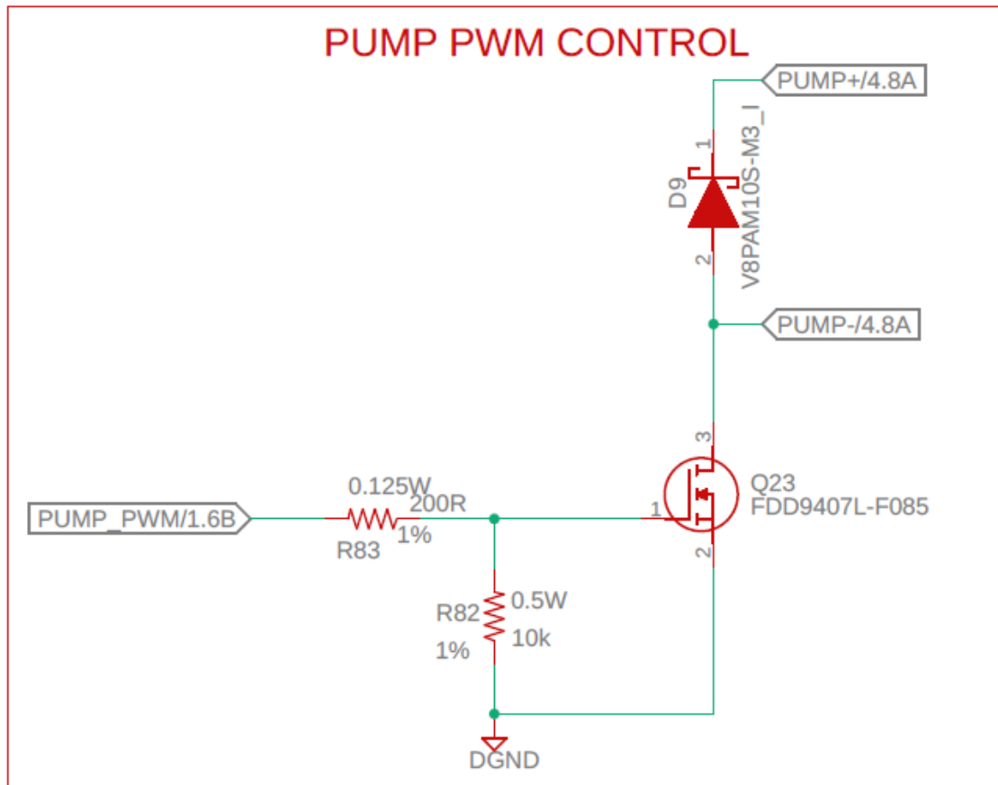
Figure 30: Pump PWM Electronic Speed Controller
