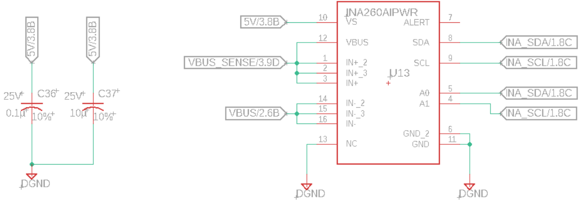
Figure 13: Power Sense Circuit.
