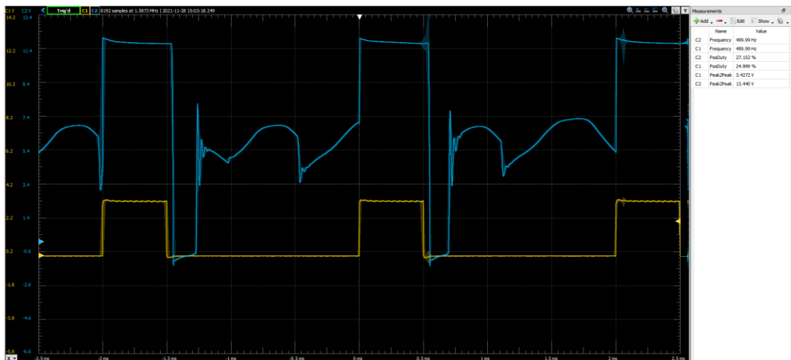
Figure Pump Control PWM signal vs GPIO PWM signal
