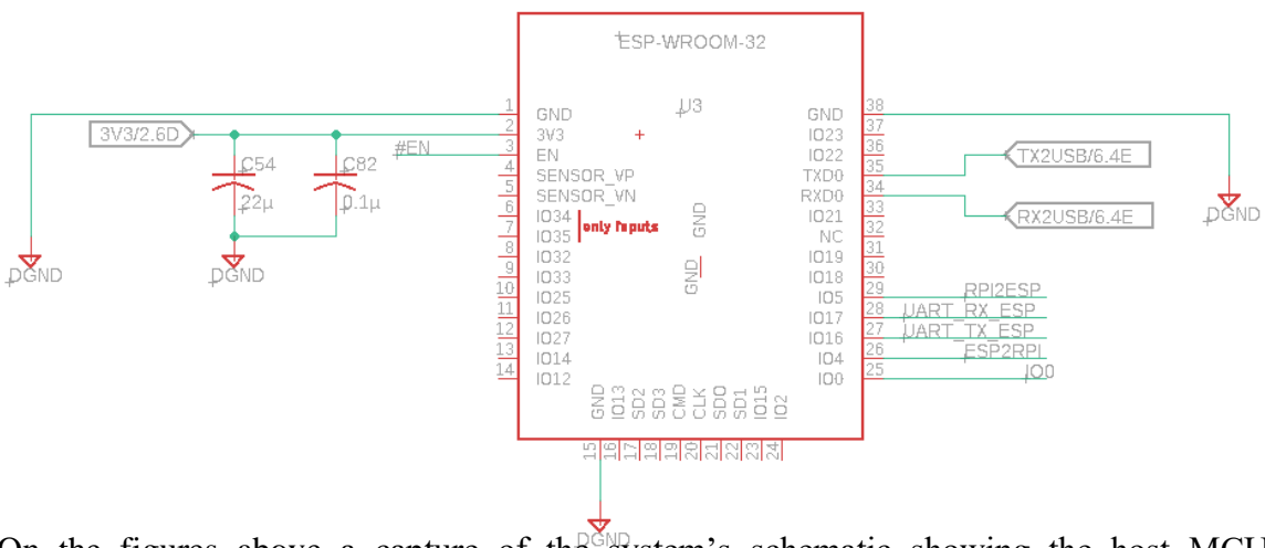
On the figures above a capture of the system's schematic showing the host MCU connection to the peripheral ESP32 and the implementation of the "Chip Select" interrupt interface. Figure 10: Interboard Communication ESP32
