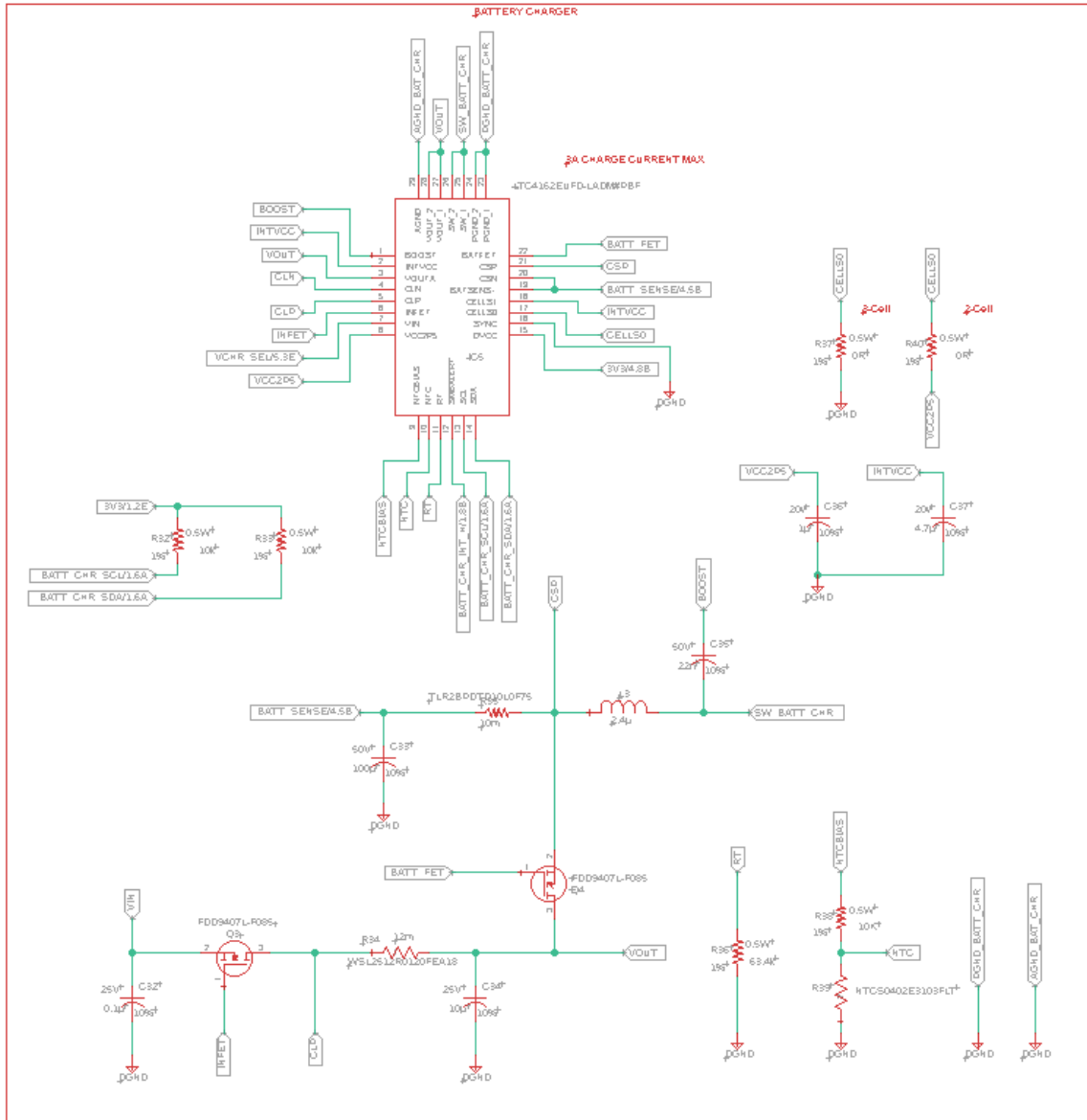
Figure 18: Battery Charger Circuit
