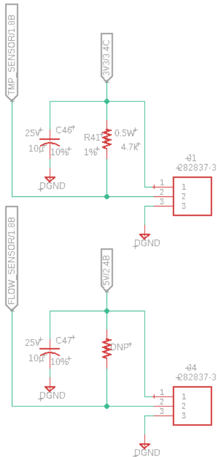
Figure 25: Temperature Sensor and Flow Sensor Peripherals Interface
