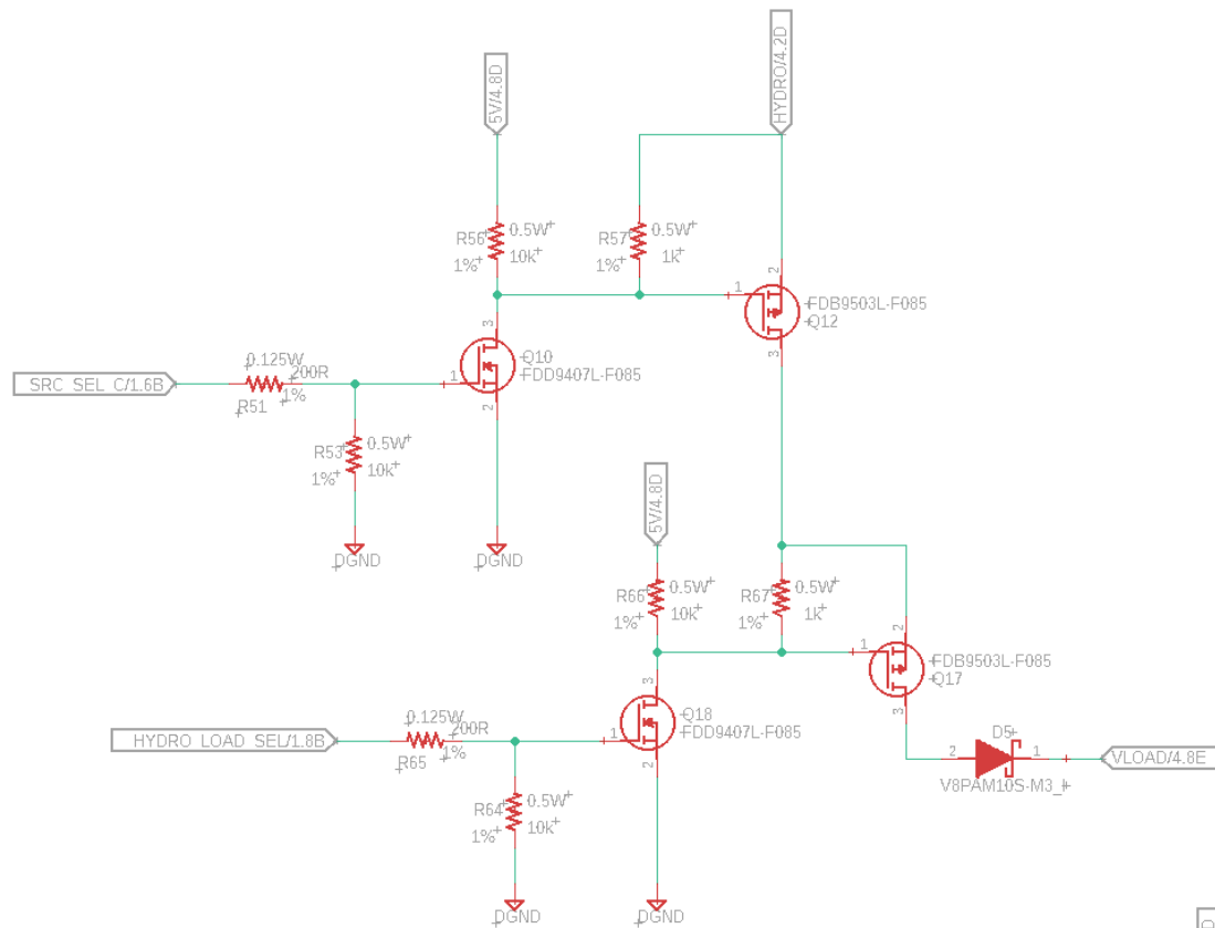
Figure 26:Hydro Generated Power & External Load Select / Enable Logic Circuit
