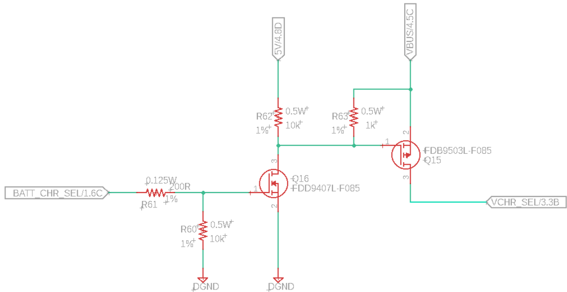
Figure 19: Battery Charger Enable Logic Circuit
