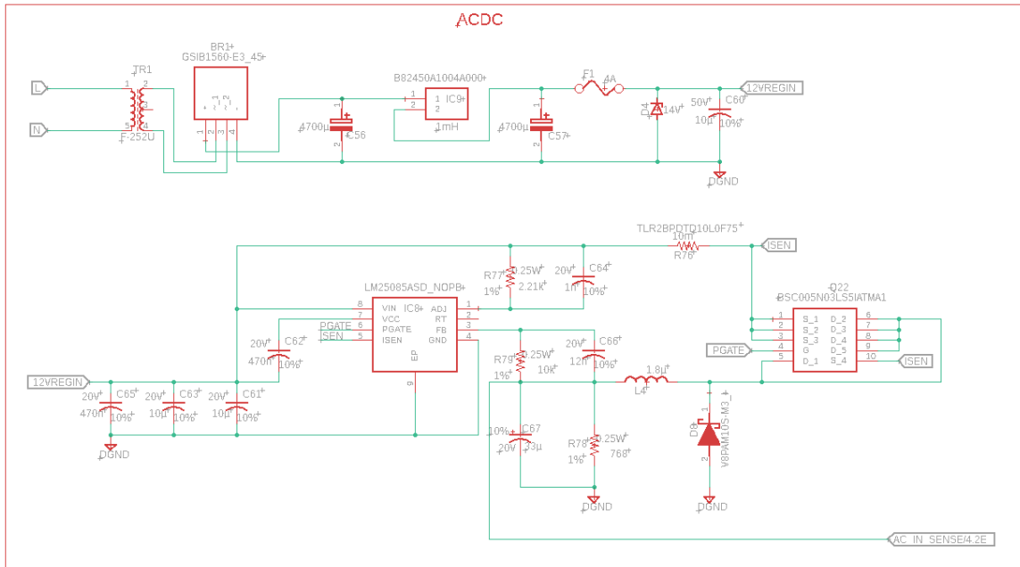
Figure 22:ACDC Circuit with 12V Regulated Output
