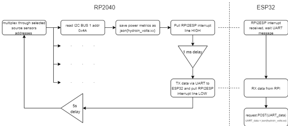
Figure 34: Sensor Reading, Interboard Communication and Server Request Software Flowchart
