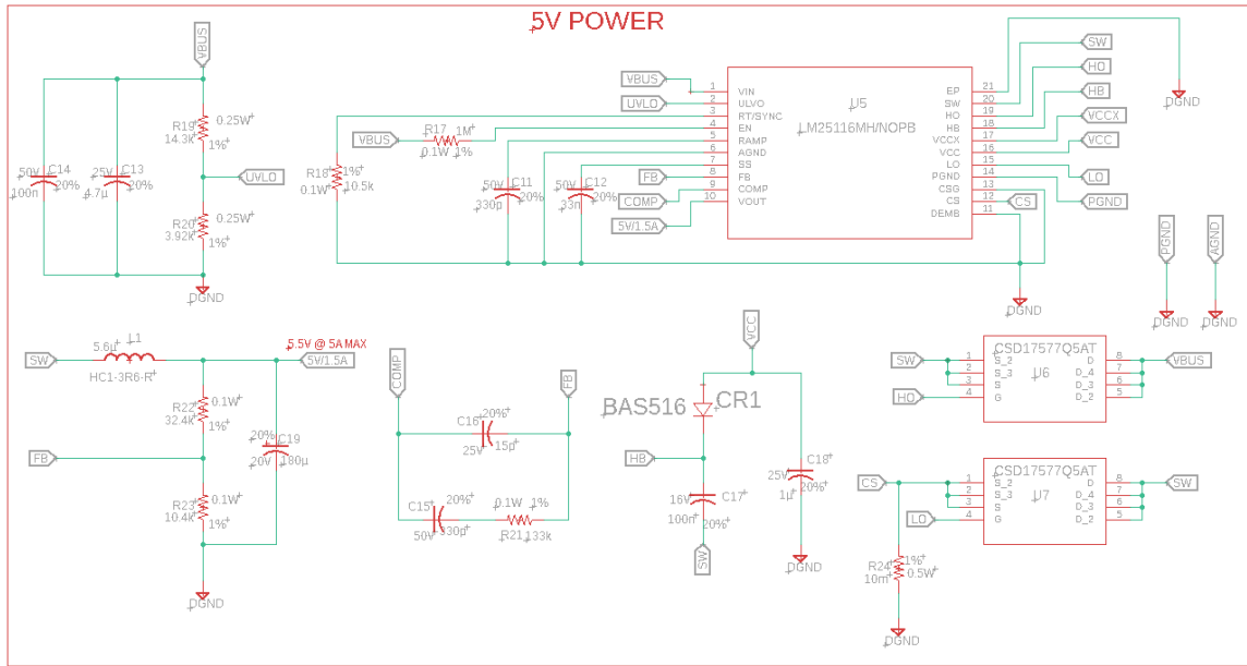
Figure 20:5V Power Rail DCDC Converter Circuit
