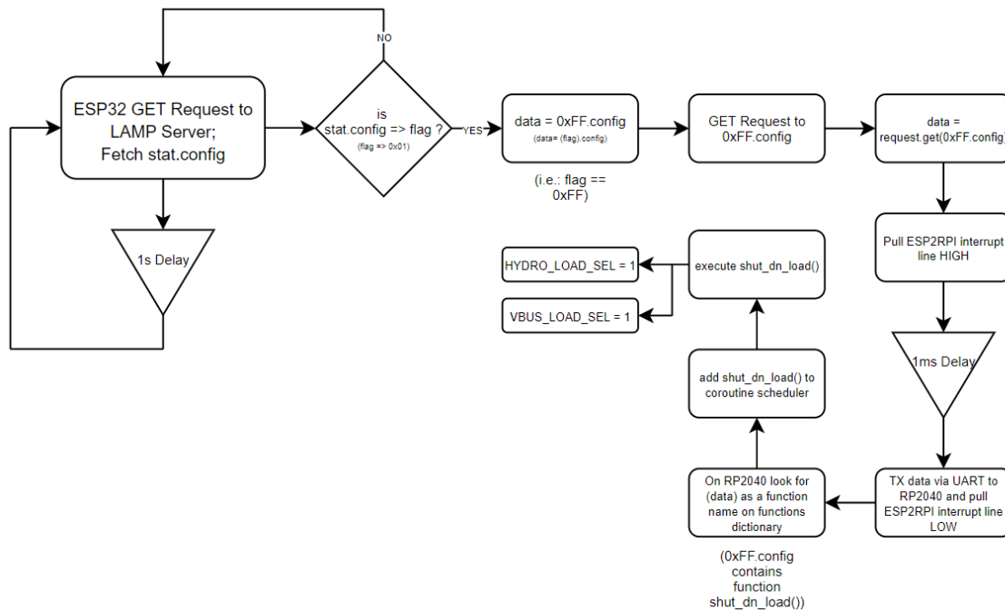
Figure 36: System Command Acknowledge using GET Request
