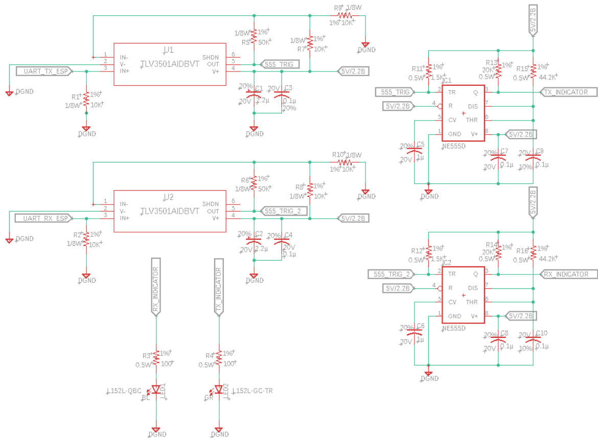
Figure 23: Network Tx/Rx Data Flow Indicator Circuit
