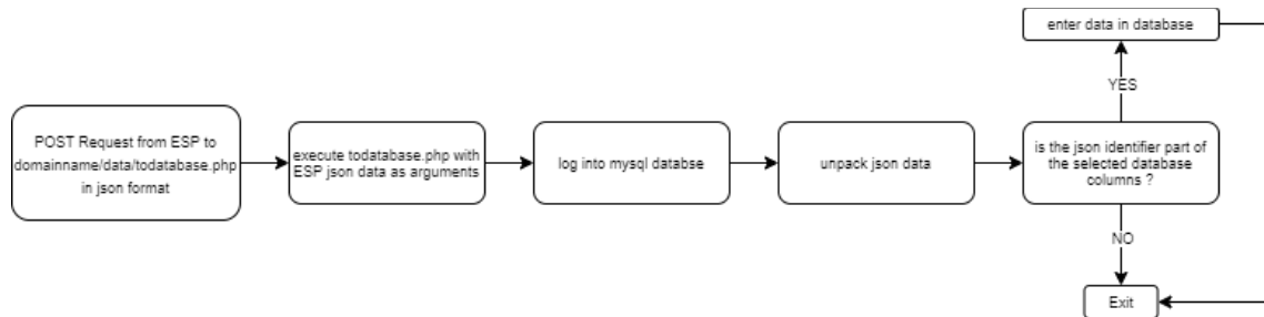
Figure 35: Server Request Handler Flowchart
