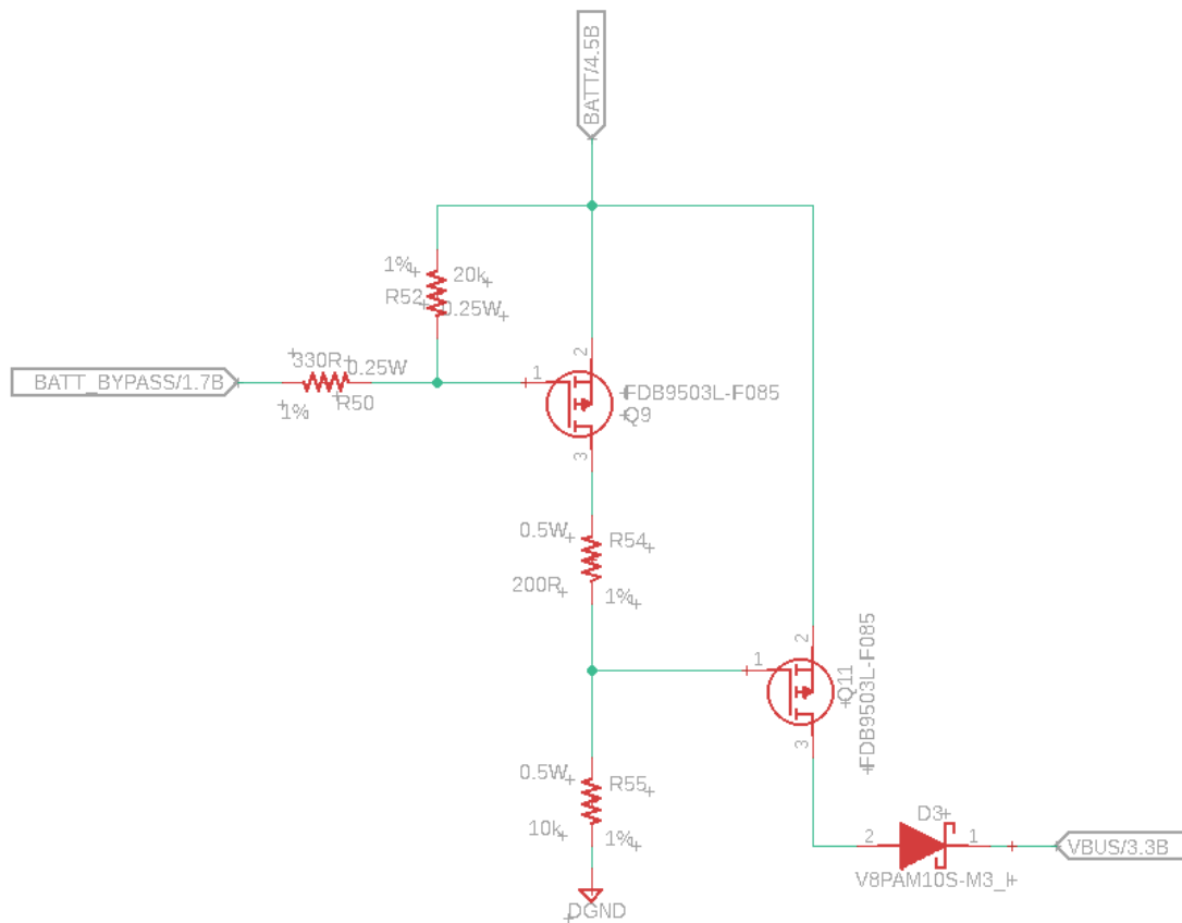
Figure 15: Modified Battery Bypass Logic Circuit
