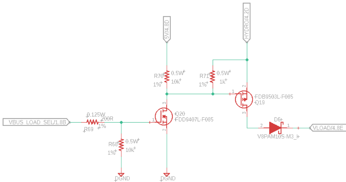
Figure 27: VBUS Rail External Load Enable Logic Circuit
