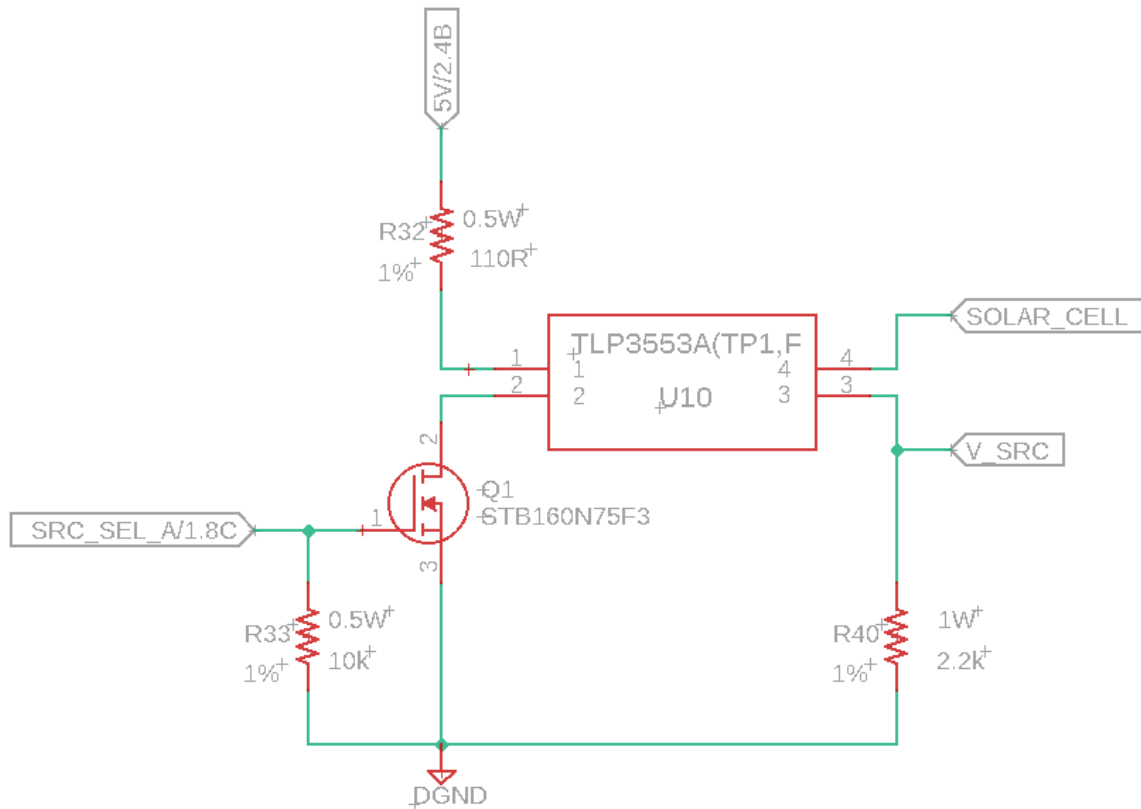
Figure 16: Source Select Logic Circuit
