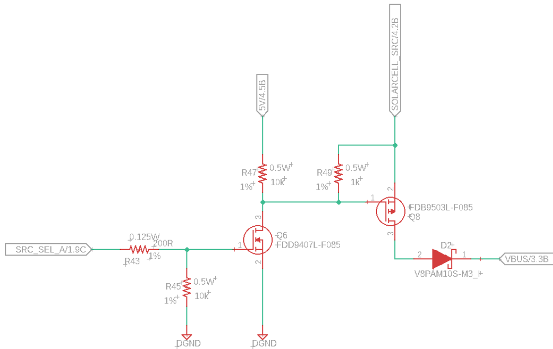
Figure 17: Modified Source Select Logic Circuit
