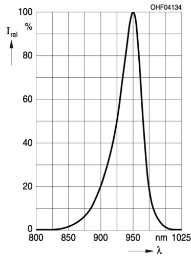
Figure 19 SFH 4546-AWBW Spectrum
