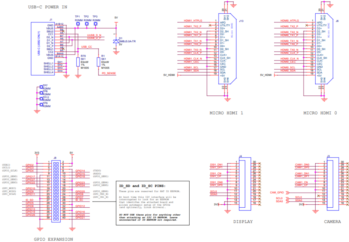
Figure 62 Raspberry Pi 4 Module Schematics (Courtesy of Raspberry Pi)
