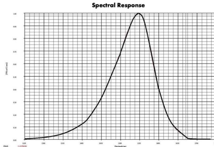
Figure 23 MTE5015-525-IR Spectrum
