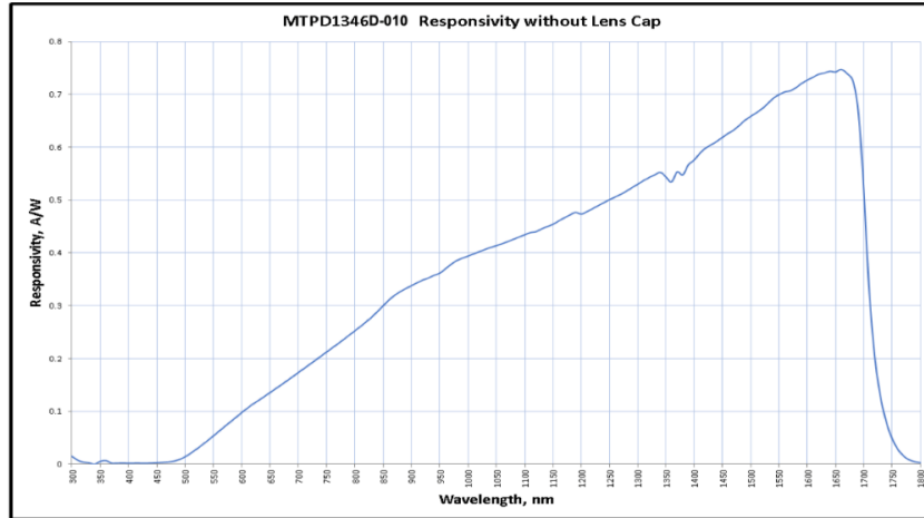
Figure 77 MTPD1346D-010 Responsivity Spectrum
