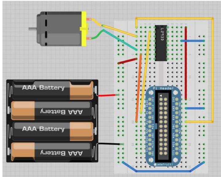
Figure 17 Motor Controlling Scheme
