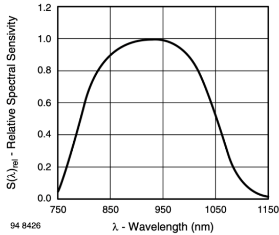
Figure 25 BPV23FL Spectral Sensitivity
