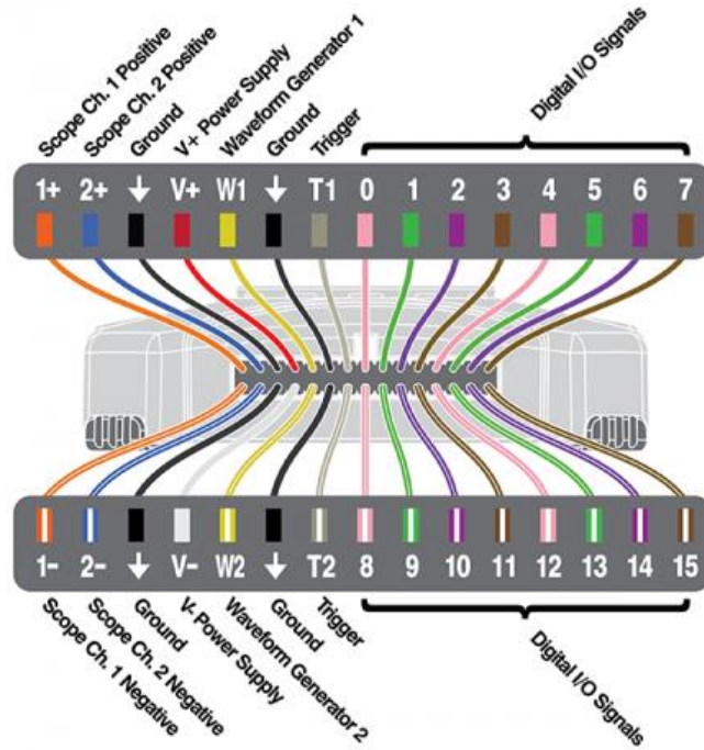
Figure 80 Analog Discovery Two Schematic
