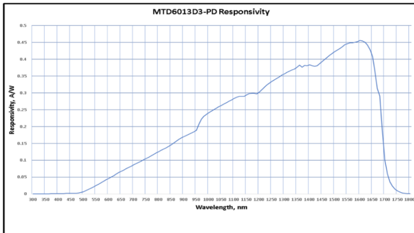
Figure 79 MTD6013D3-PD Responsivity
