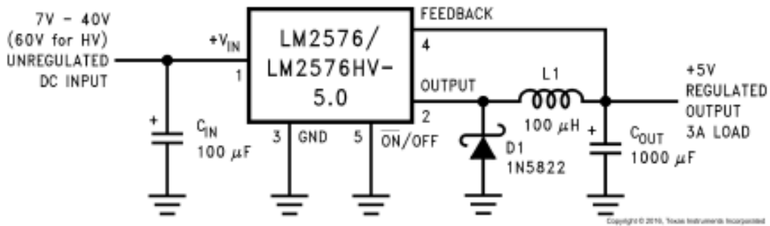
Figure 75 Voltage Regulator Circuit from LM 2576 Datasheet (Courtesy of Texas Instruments)
