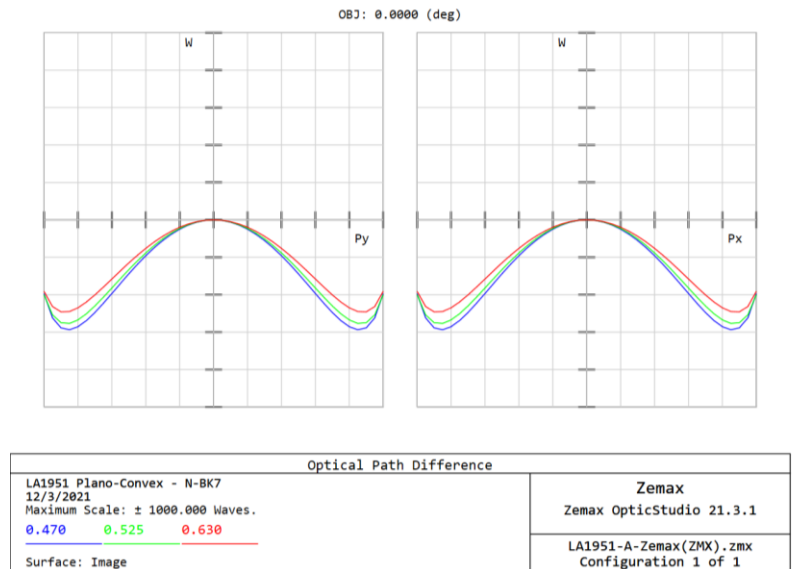
Figure 29 Optical path difference of the Planoconvex lens
