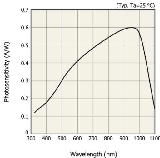
Figure 24 S2386-5K Spectral Response
