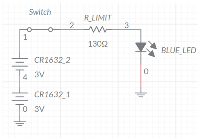
Figure 49 Circuit Schematic for Blue LED
