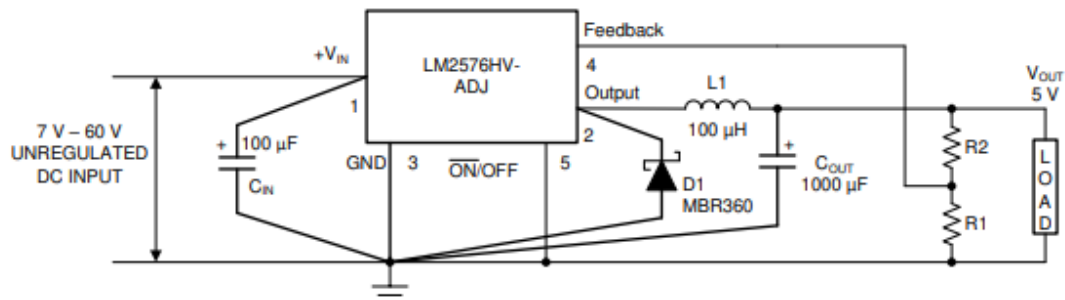
Figure 76 Adjustable Voltage Regulator Circuit from LM 2576 Datasheet (Courtesy of Texas Instruments)
