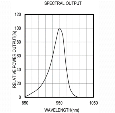
Figure 20 MTE9460N5 Spectral Output
