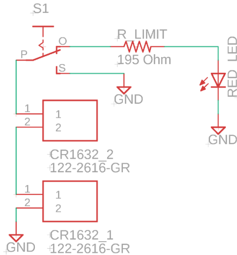
Figure 54 Collar PCB Schematic
