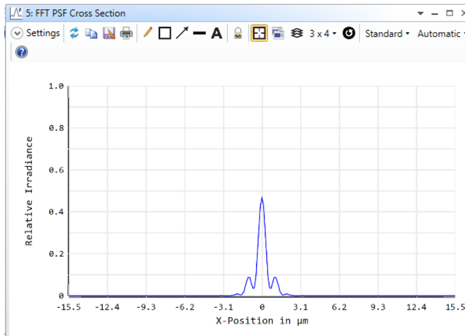
Figure 34 Point Spread Function
