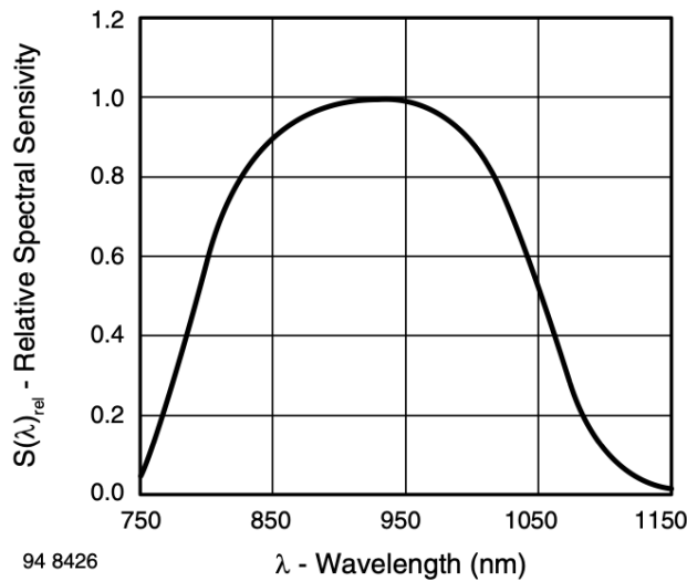
Figure 26 BPW82 Spectral Sensitivity
