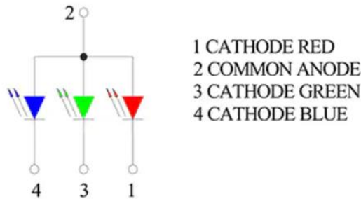
Figure 36 Pinout diagram for a Multi Color LED
