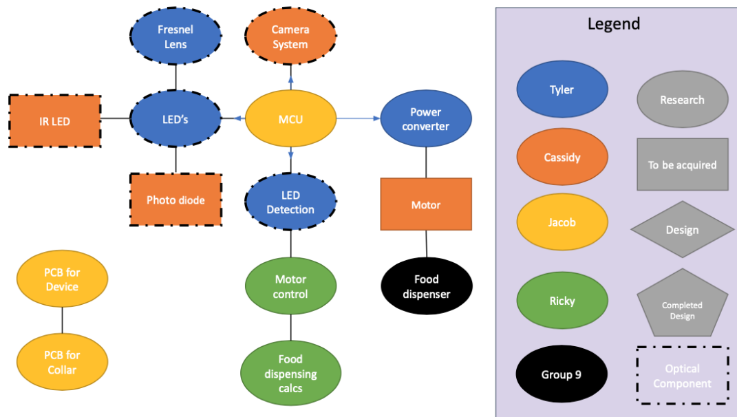
Figure 5 Opto-Smart Role Assignment Block Diagram
