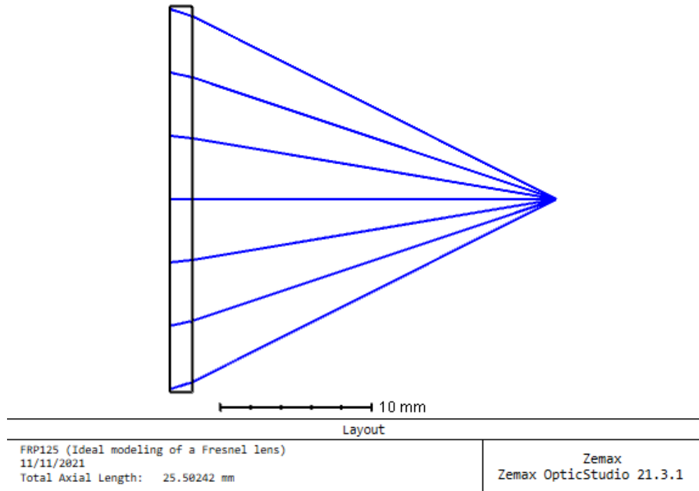
Figure 32 Layout of Fresnel Lens
