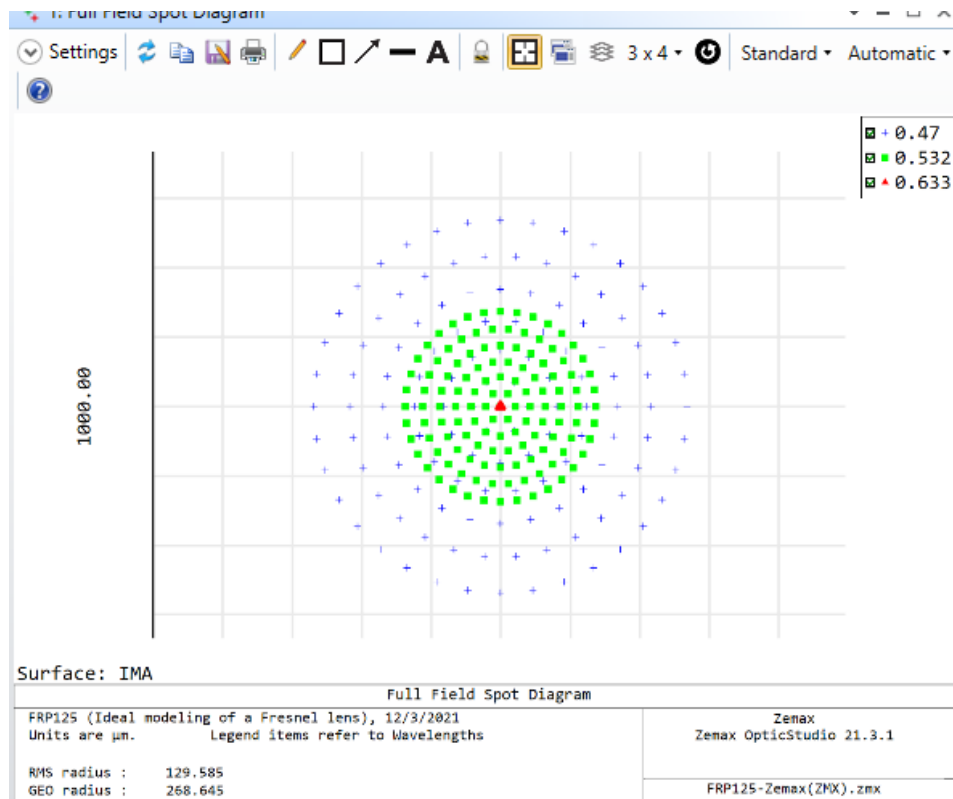
Figure 33 Spot Diagram of Fresnel Lens
