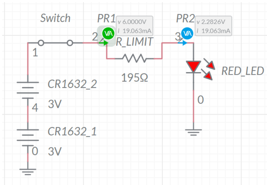
Figure 51 Circuit Schematic with Values for Red LED
