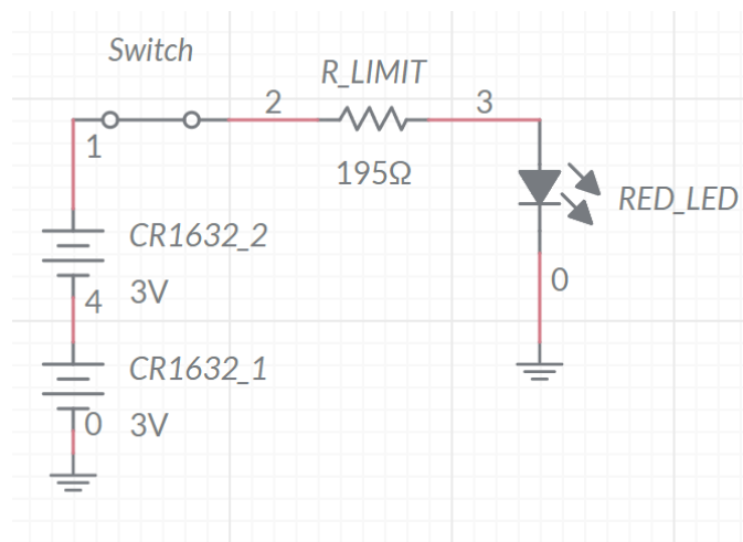
Figure 48 Circuit Schematic for Red LED
