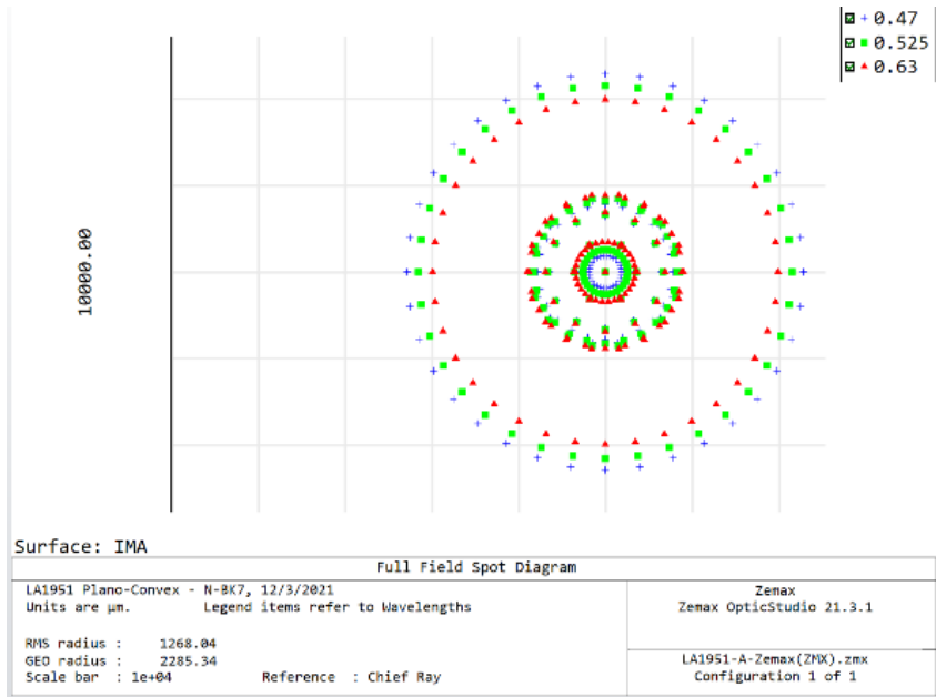
Figure 28 Spot diagram of plano-convex lens
