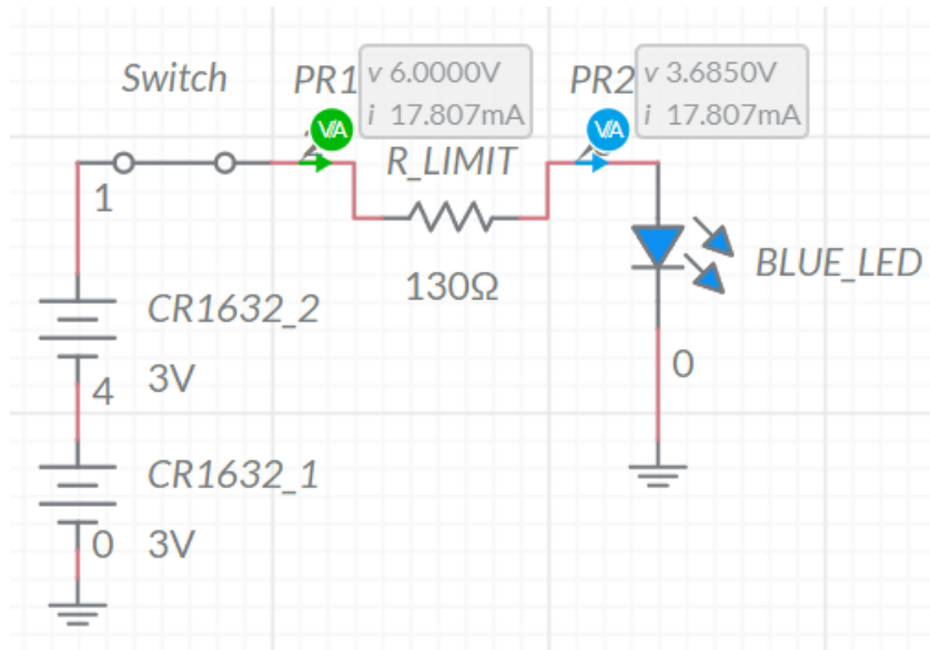
Figure 52 Circuit Schematic with Values for Blue LED
