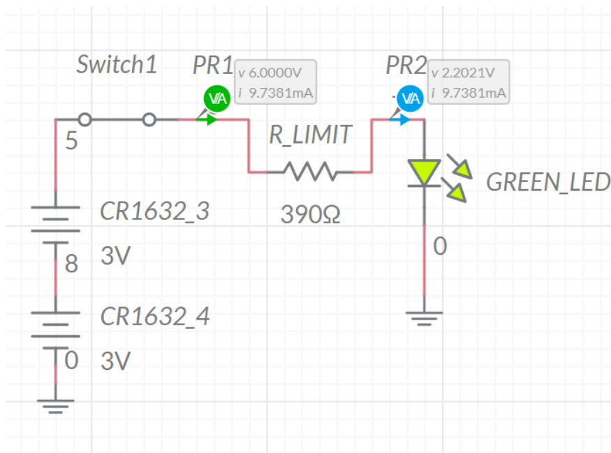
Figure 53 Circuit Schematic with Values for Green LED
