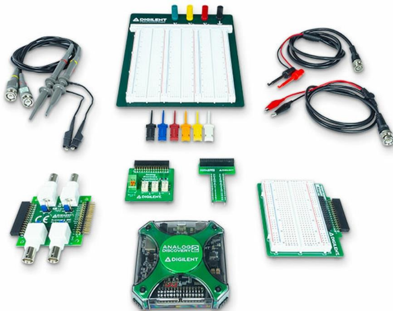
Figure 45 Analog Discovery 2
