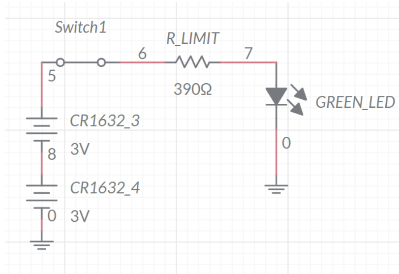
Figure 50 Circuit Schematic for Green LED
