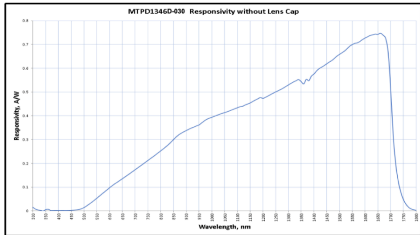
Figure 78 MTPD1346D-030 Responsivity Spectrum
