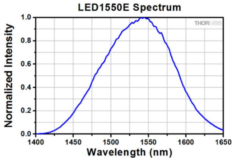
Figure 21 Ultra Bright NIR, Epoxy- Encased LED, 1550 nm Spectrum
