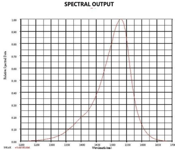
Figure 22 MTE5115D4 Spectrum
