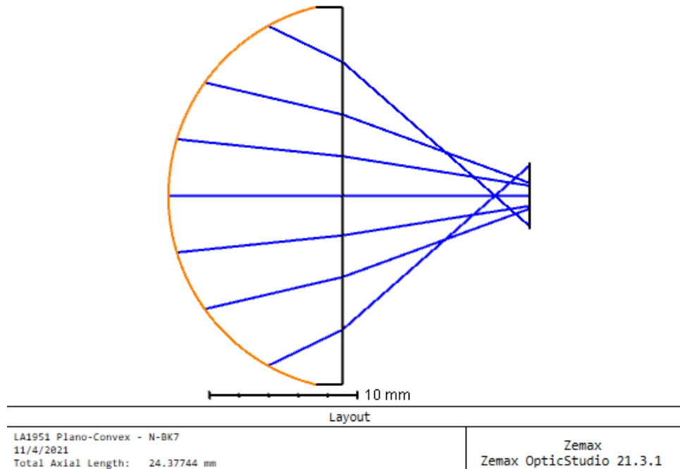
Figure 27: Layout of Plano-Convex Lens
