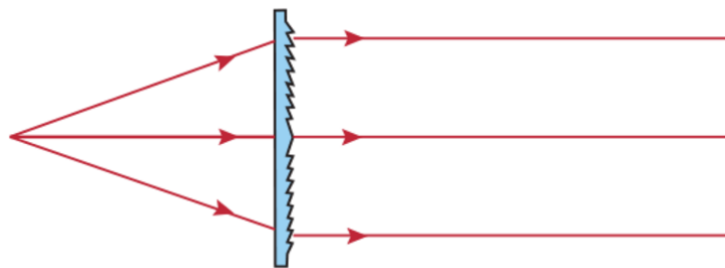
Figure 31 Fresnel Lens
