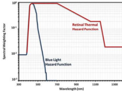
Figure 73 Retinal thermal and blue light hazard functions
