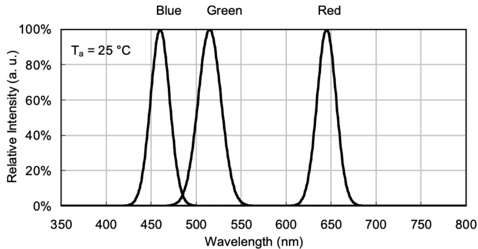
Figure 37: WP154A4SUREQBFZGC Intensity Spectrum
