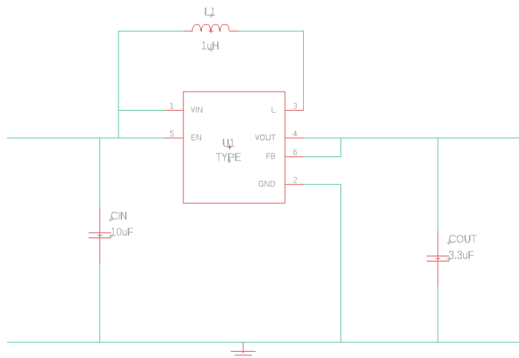
Figure 56 3.3V to 5V Converter Schematic
