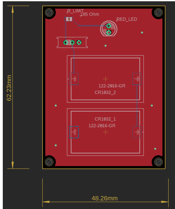
Figure 55 Collar PCB Board Layout
