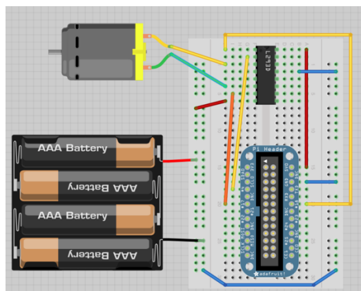
Figure 15 Motor Controlling Scheme
