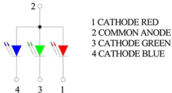
Figure 26 Pinout diagram for a Multi Color LED
