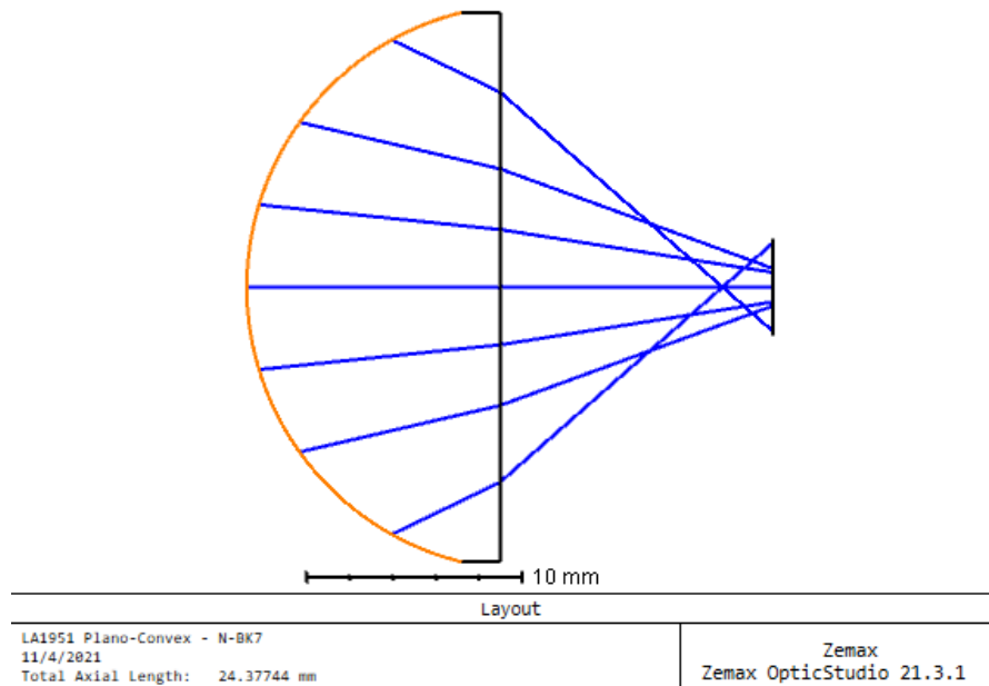
Figure 19: Layout of Plano-Convex Lens
