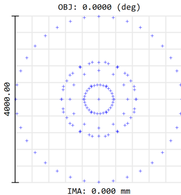
Figure 20 Spot diagram of plano-convex lens
