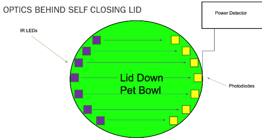
Figure 2 Opto-Smart Self Closing Lid Block Diagram
