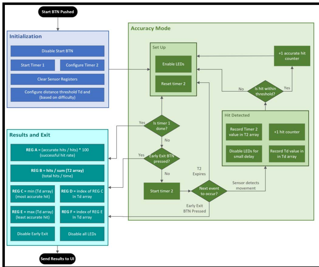
Figure 33: Software flow chart for the Accuracy Mode on Side B
