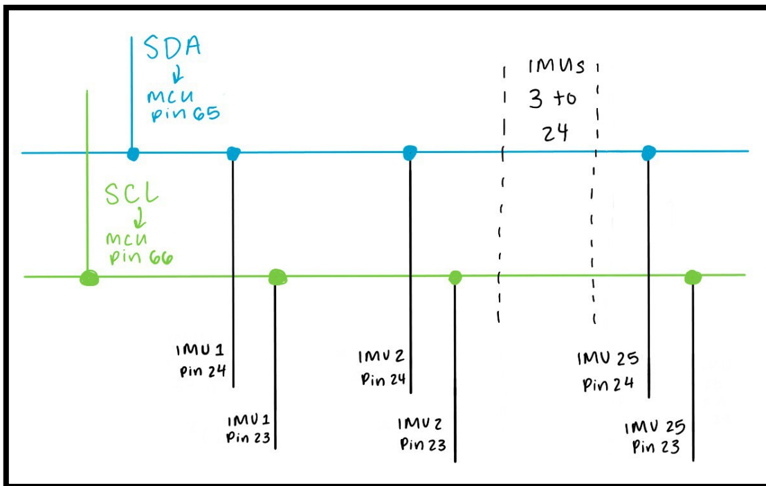
Figure 22: IMU Communication with I2C setup
