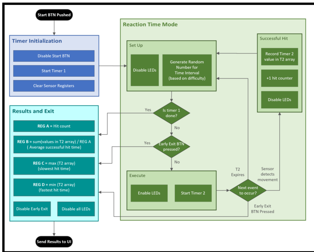
Figure 32: Software flow chart for the Reaction Time Mode on Side B
