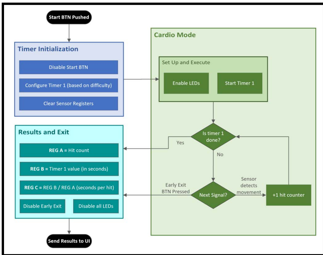
Figure 34: Software flow chart for the Cardio Mode on Side B
