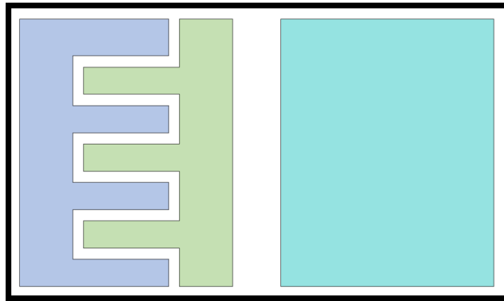
Figure 16: Visual representation of the two layers of the binary sensors for side A
