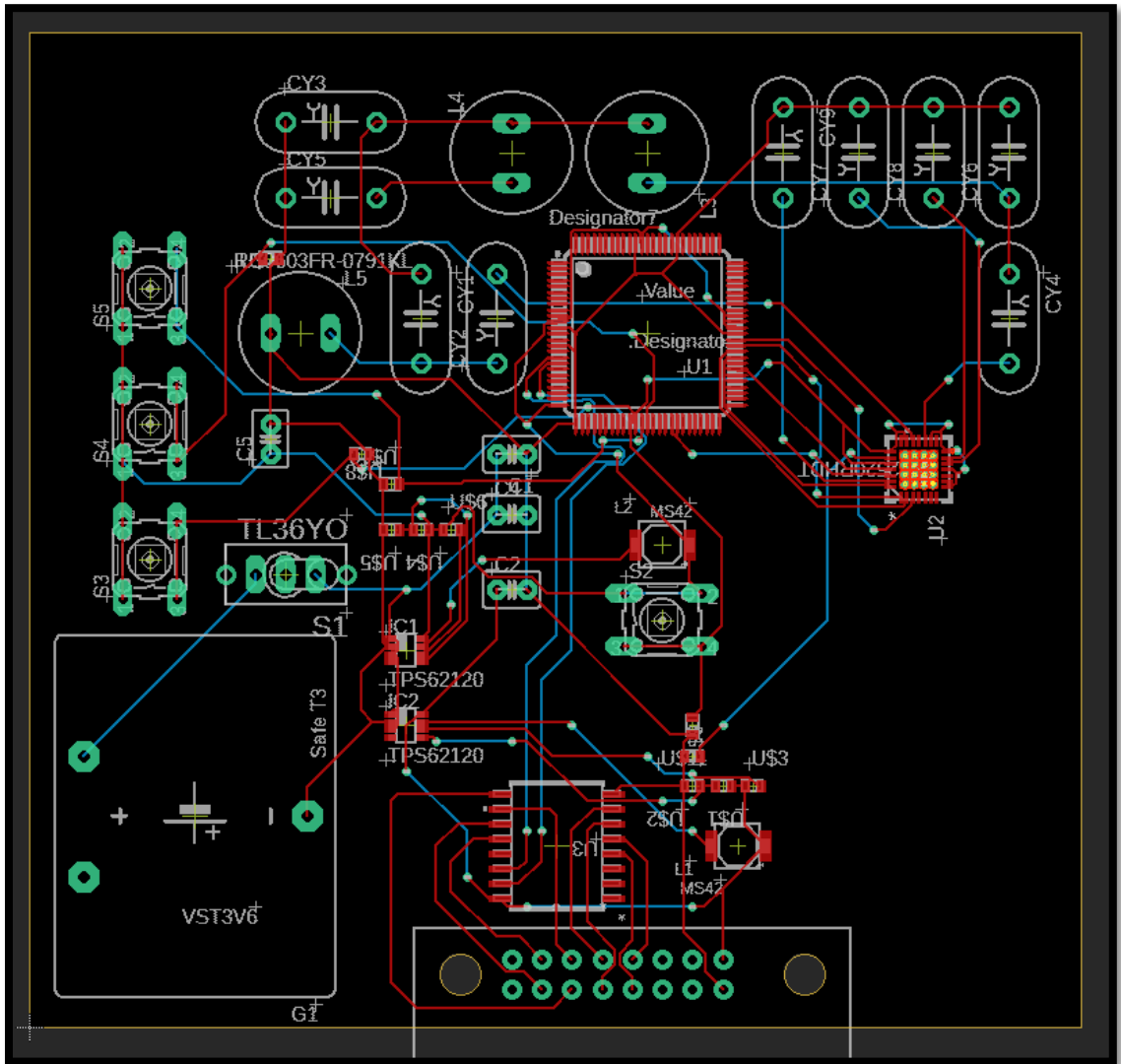
Figure 28: UI Handheld System Board Layout
