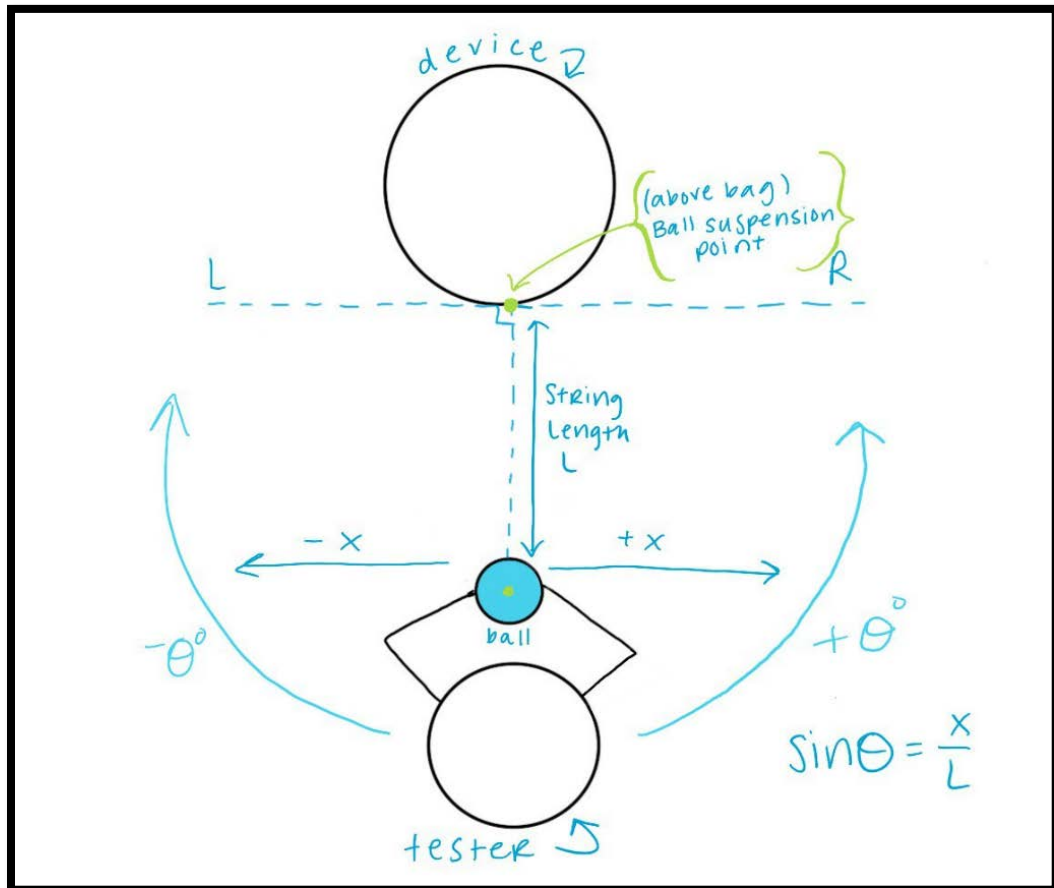
Figure 44: Visual Representation of the testing for side B (top view)
