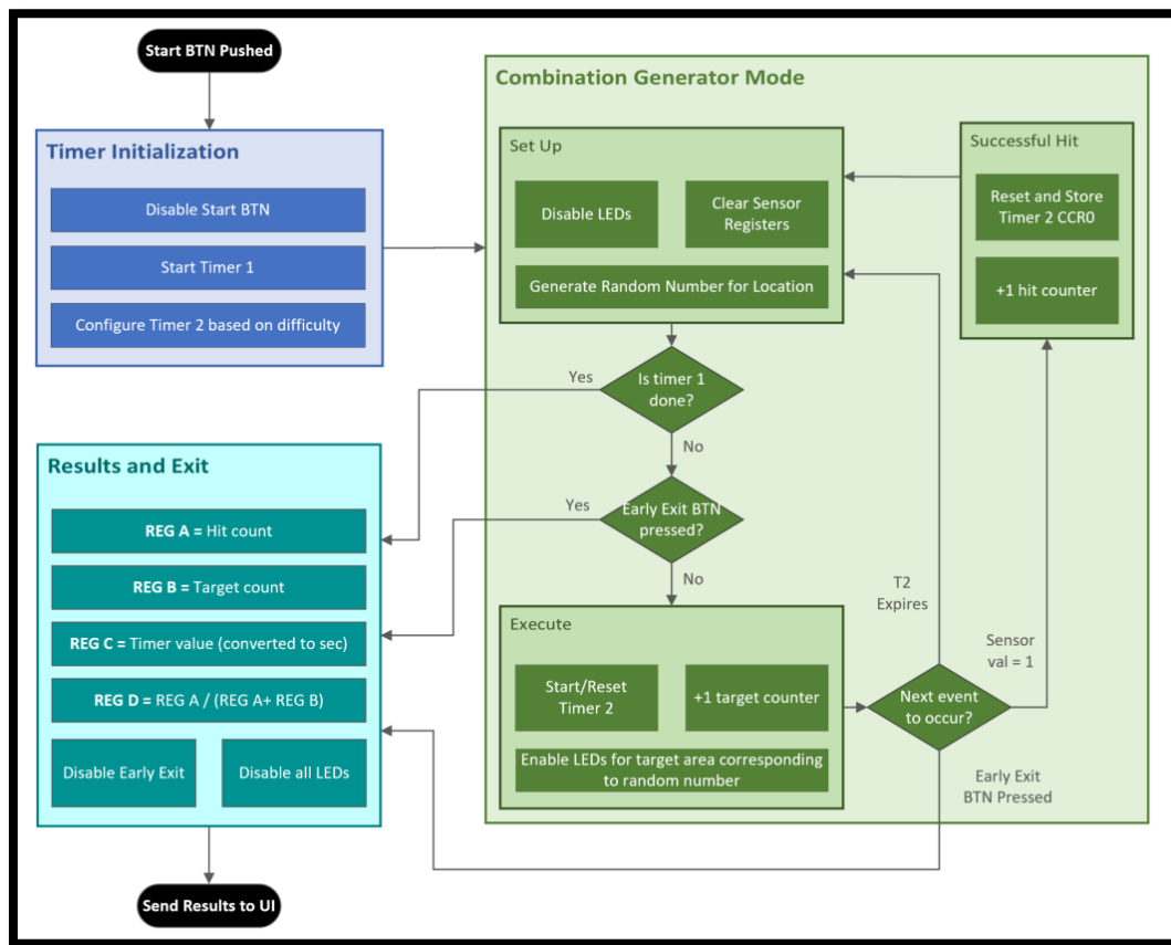
Figure 31: Software flow chart for the Combination Generator Mode on Side A
