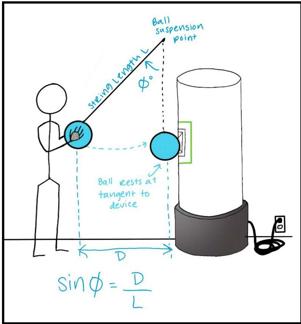
Figure 43: Visual Representation of the testing for side B (front view)
