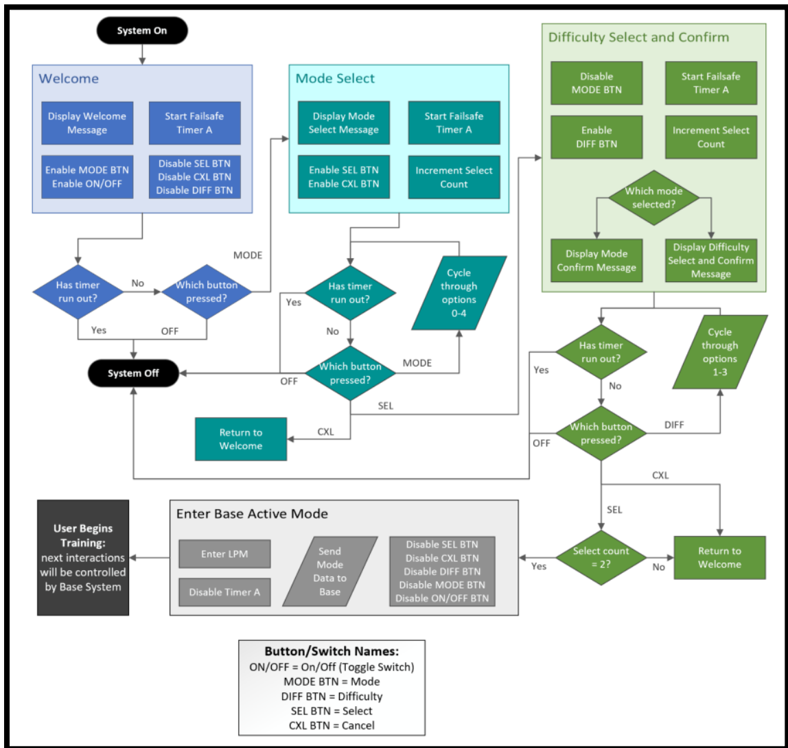
Figure 29: Software flow chart for UI and Initialization
