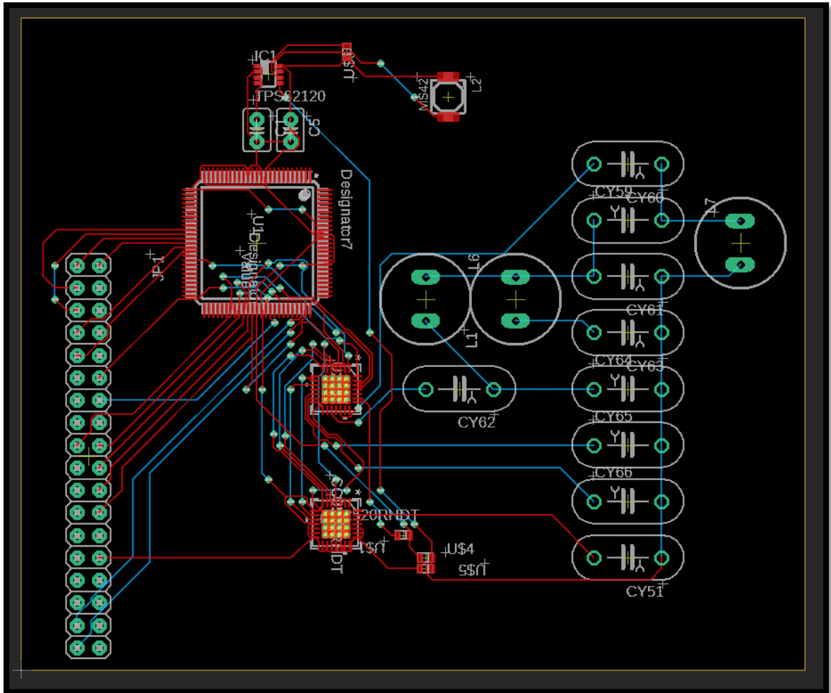
Figure 26: Base System PCB Layout
