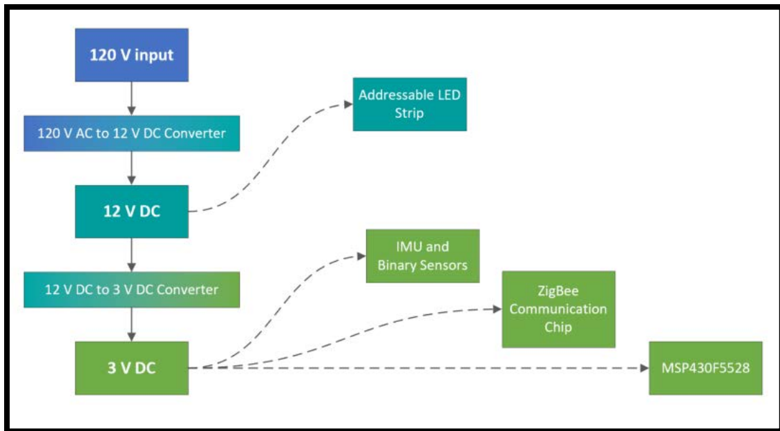
Figure 18: Flow chart for Power Supply in Base System
