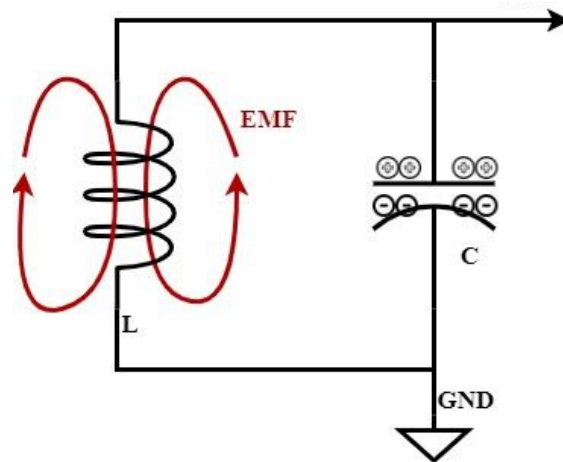
Figure 24: EMF Sensor
