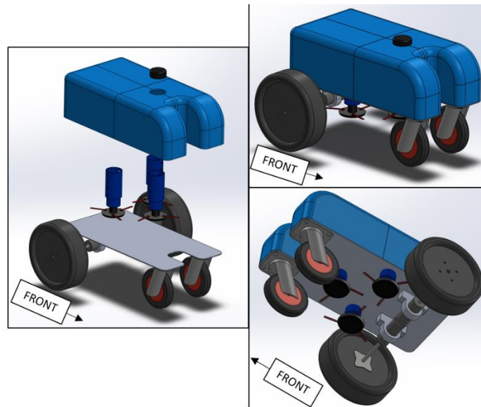
Figure 34: CAD rendering
