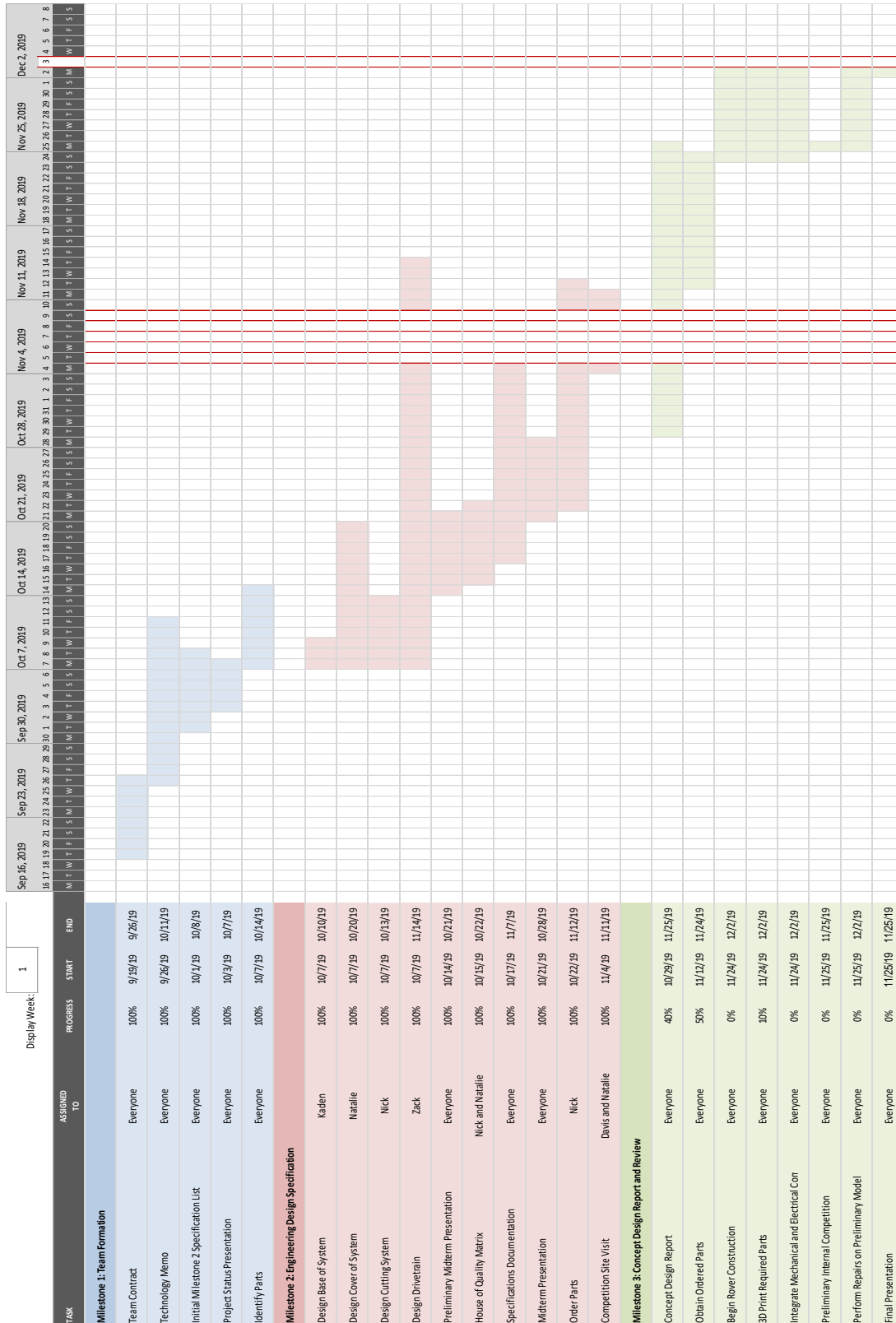
Figure 42: Gantt Chart 1
