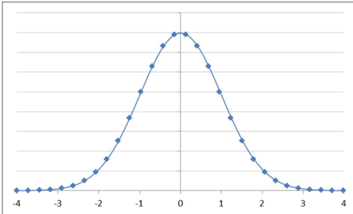
Figure 17: Gaussian Bell Curve
