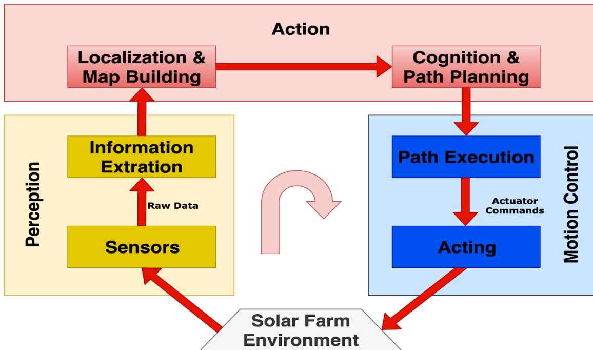
Figure 1: Control Scheme
