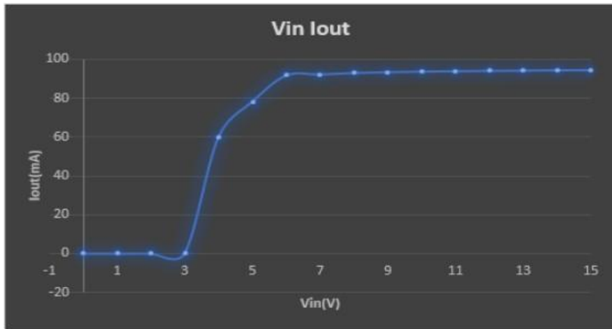
Figure 29 - Plot of the Input Voltage and Output Current.
