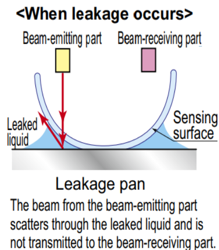
Figure 23 - Leak Sensor Mechanism Diagram 2 [15]
