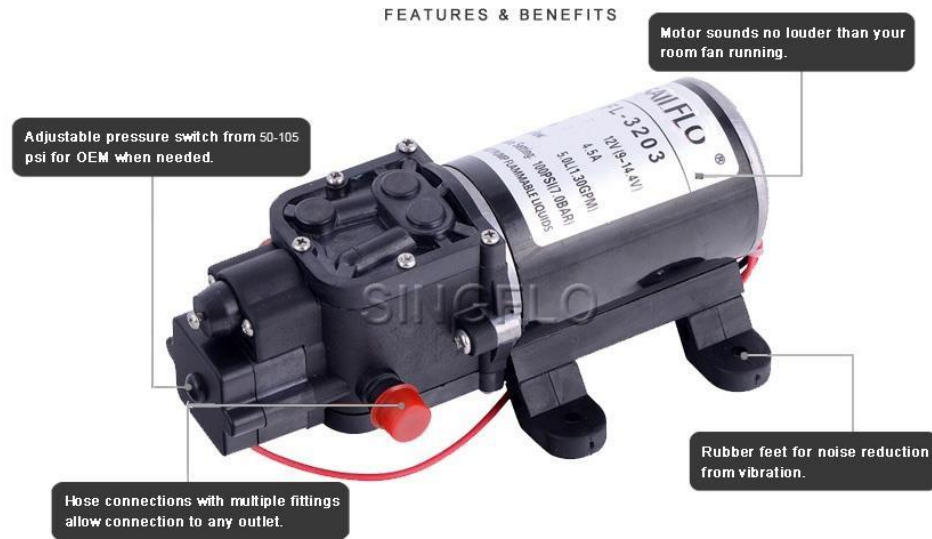
Figure 14 - Standard Transfer Pump [10]
