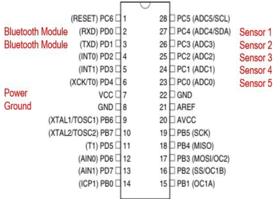
Figure 39 - Pin Mapping
