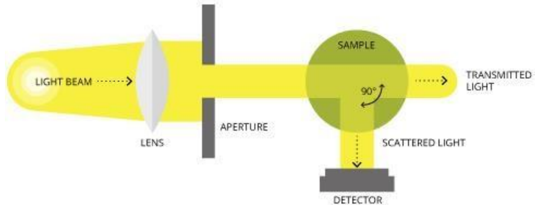
Figure 21 - Turbidity sensor mechanism diagram [14]
