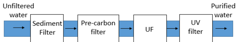
Figure 43 - Filters Order
