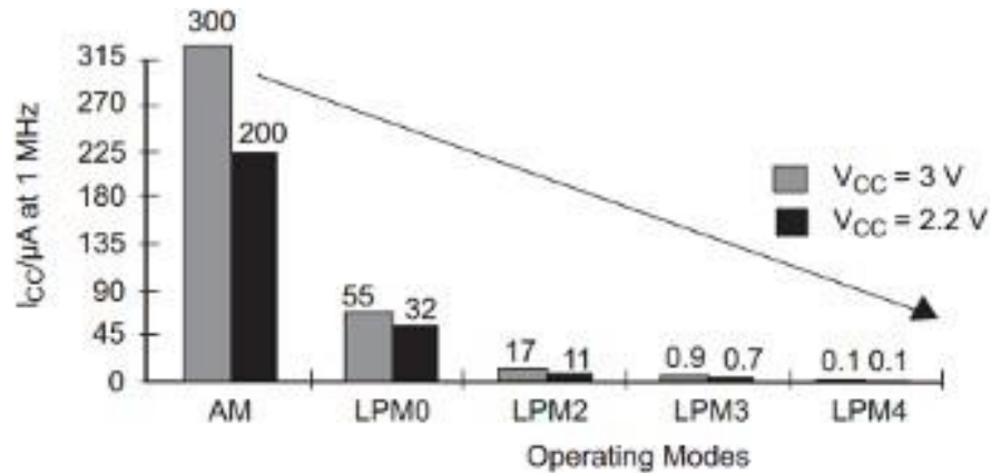
Figure 12 - Power Consumption Profile of LPM [8]
