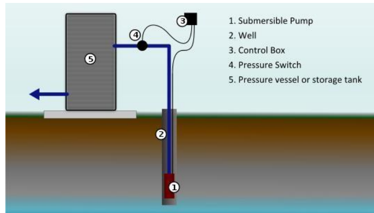
Figure 13 - Example of System Using Submersible Pump [9]
