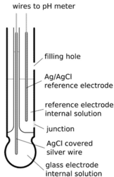
Figure 20 - pH probe diagram [13]
