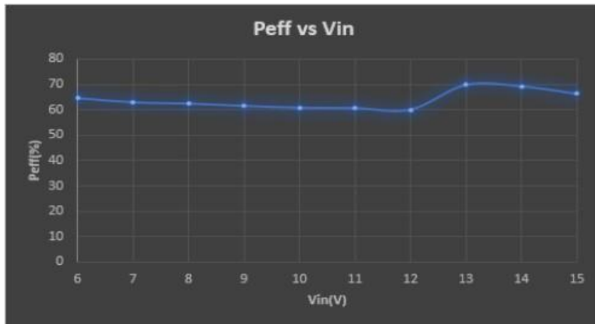
Figure 30 - Plot of the Output Efficiency P_{out}/P_{in} as a Function of V_{in}
