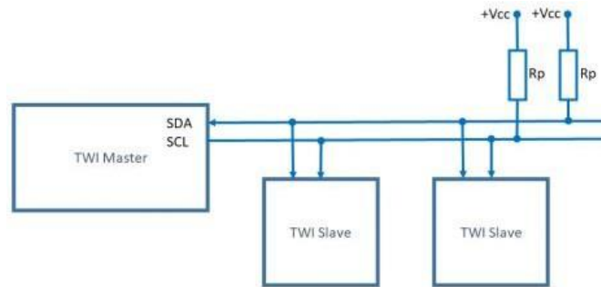
Figure 11 - I2C Connection Sample [7]
