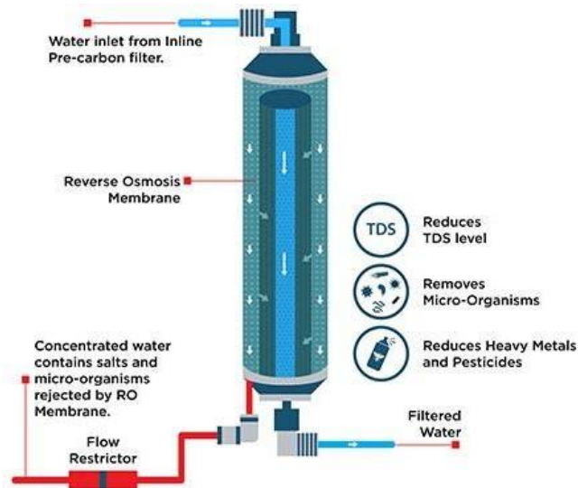
Figure 17 - Pre-carbon Filter System [12]
