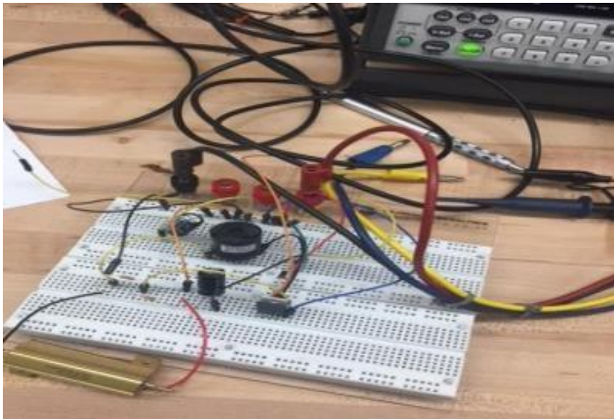
Figure 28 - Circuit for the LM2576 ADJ Voltage Regulator
