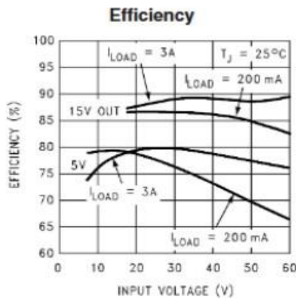
Figure 31 - Efficiency of LM2576 ADJ From its Datasheet[18]
