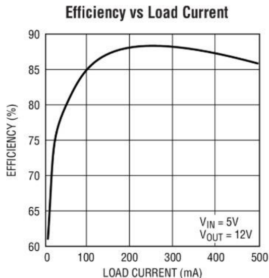
Figure 26 - Efficiency Vs Load Current [17]
