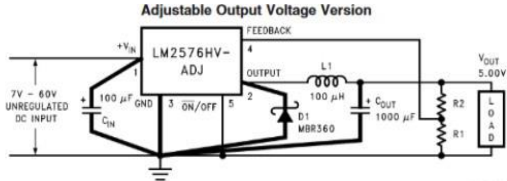
Figure 27 - Schematic of LM2576 ADJ Voltage Regulator (5V output) [18]
