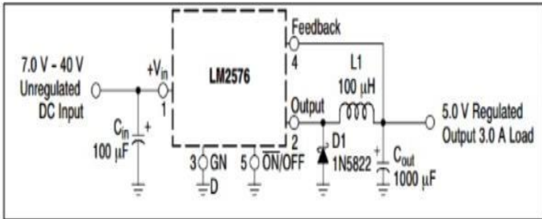
Figure 32 - Schematic of LM2576 Voltage Regulator (5V output)[18]
