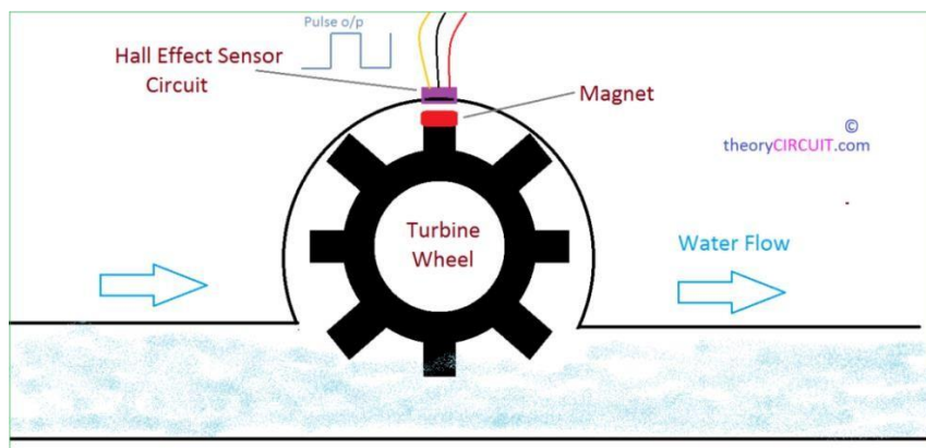
Figure 25 - Water flow sensor mechanism diagram [16]
