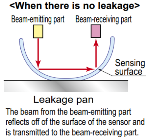
Figure 22 - Leak Sensor Mechanism Diagram 1 [15]
