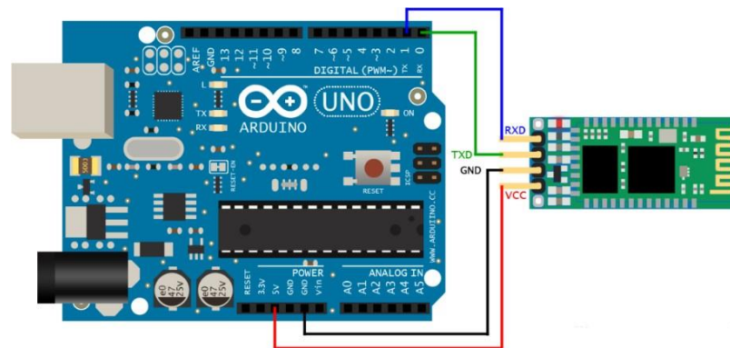
Figure 42 - Bluetooth Module Mapping [25]
