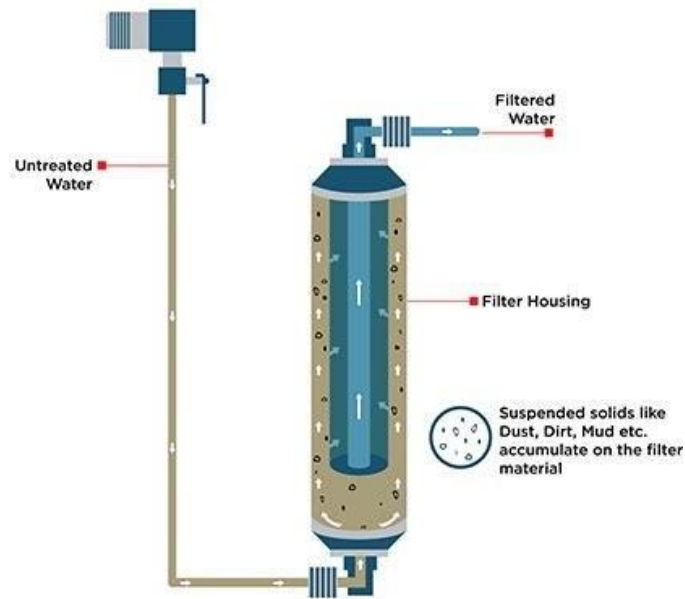
Figure 16 - Sediment Filter [12]
