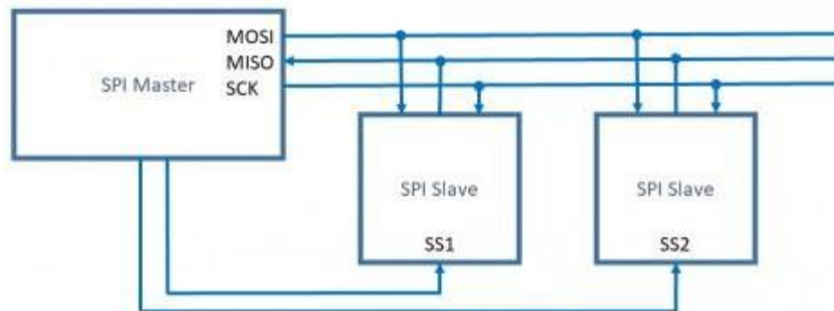
Figure 10 - SPI Connection Sample [7]
