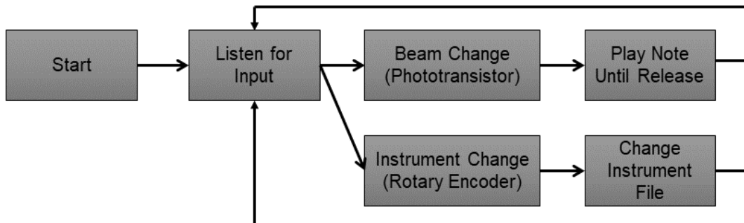
Figure 23 Software Flow
