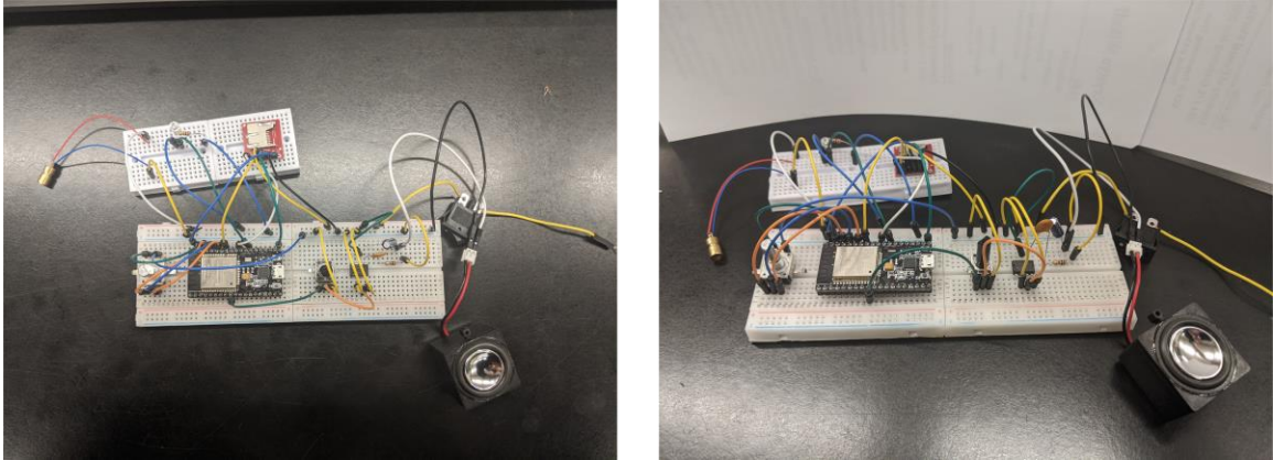
Figure 21 Example Layout on Breadboard
