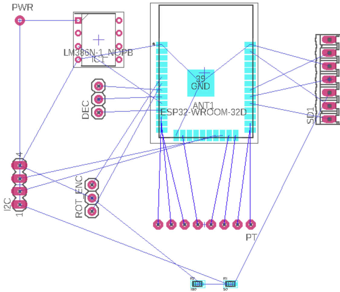
Figure 25 PCB Layout
