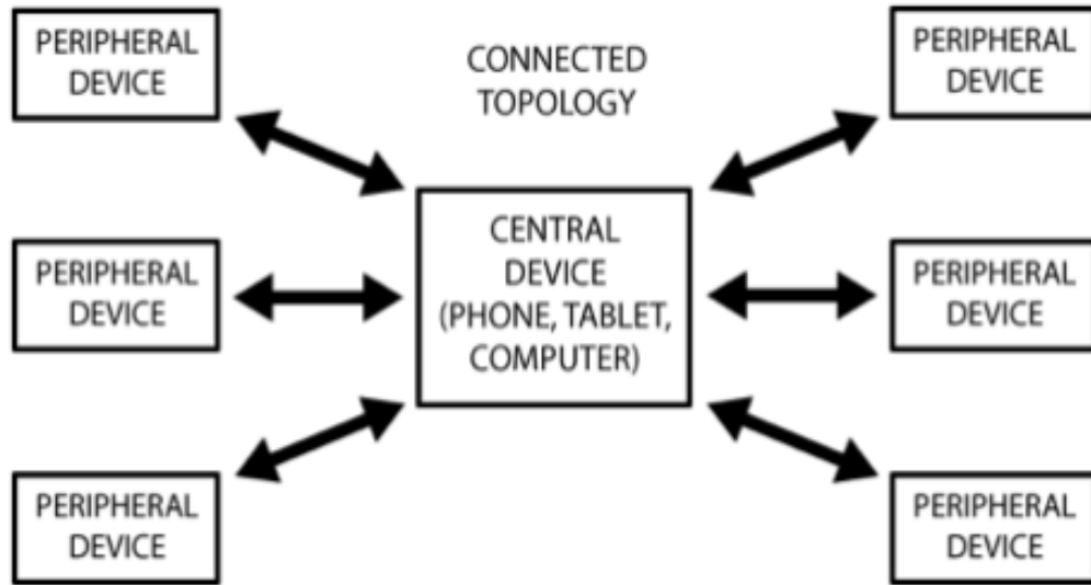
Figure 45. Topology of BLE connected devices
