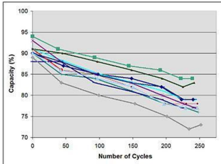
Figure 11. Lithium Ion Battery Capacity vs Cycles
