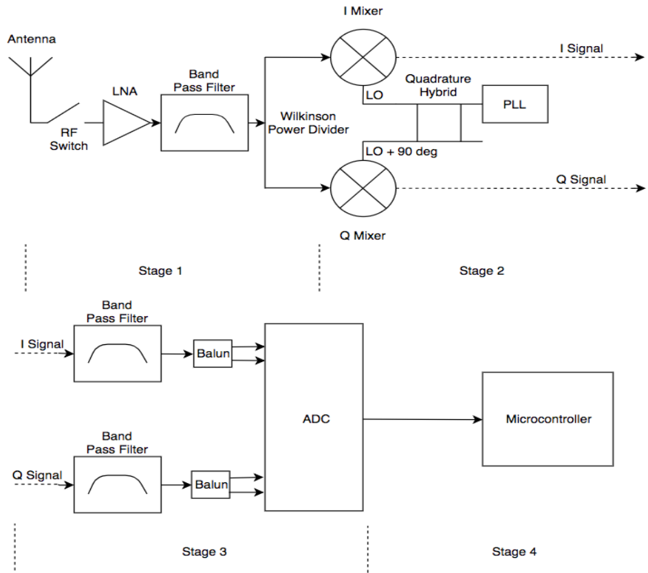
Figure 50. Receive Path of the Transceiver
