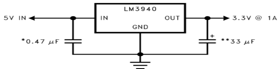
Figure 37. LM3940 5V to 3.3V LDO
