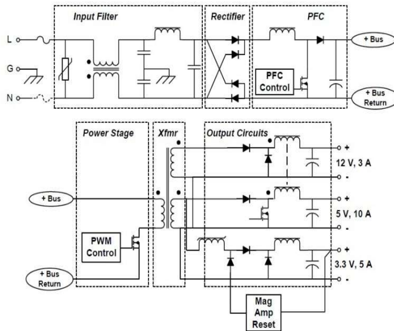
Figure 30. Forward Converter Circuit Diagram.
