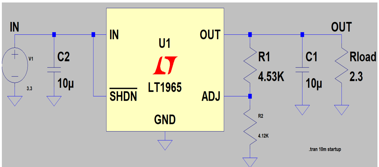
Figure 39. 3.3V to 2.5V LDO.
