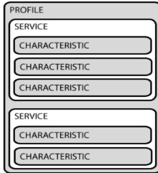
Figure 47. Nested object topology in BLE
