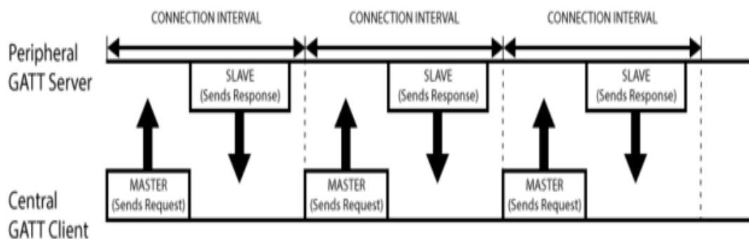
Figure 46. Typical data exchange between BLE devices
