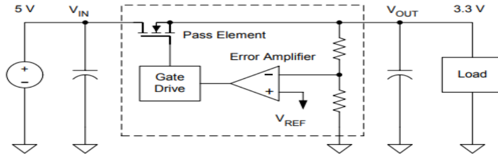
Figure 36. LDO Voltage Regulator Schematic.
