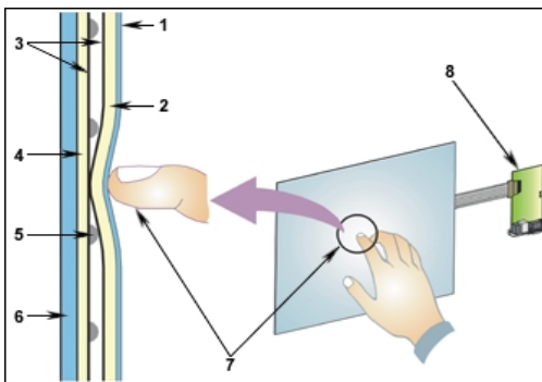
Figure 12. Operation of a Resistive Touchscreen
