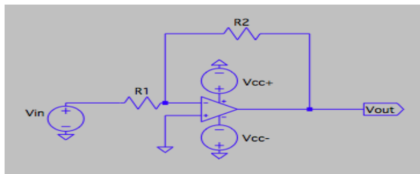
Figure 25. Op-Amp Buck-Boost Circuit
