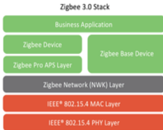
Figure 42. The Zigbee protocol stack
