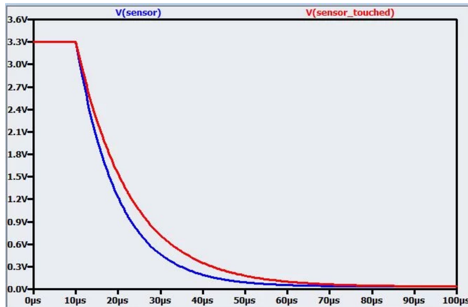
Figure 14. Touch screen time constant
