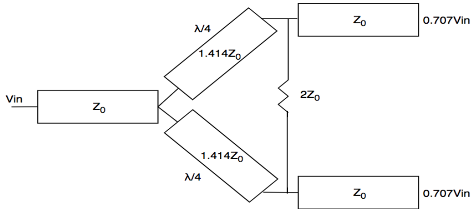
Figure 59. Wilkinson Power Divider/Combiner
