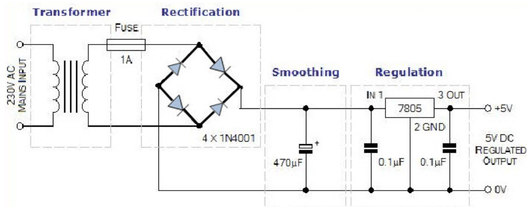
Figure 32. Bridge Rectifier AC/DC converter circuit.
