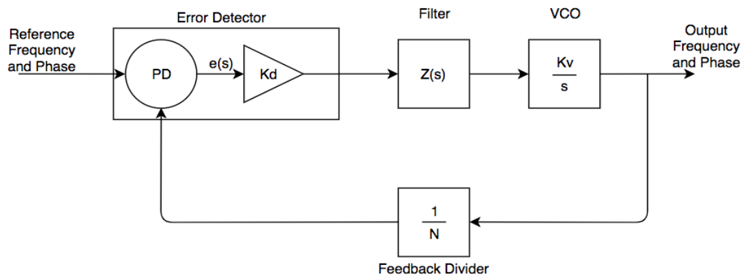
Figure 57. Typical Phase-Locked Loop Transfer Function Block Diagram
