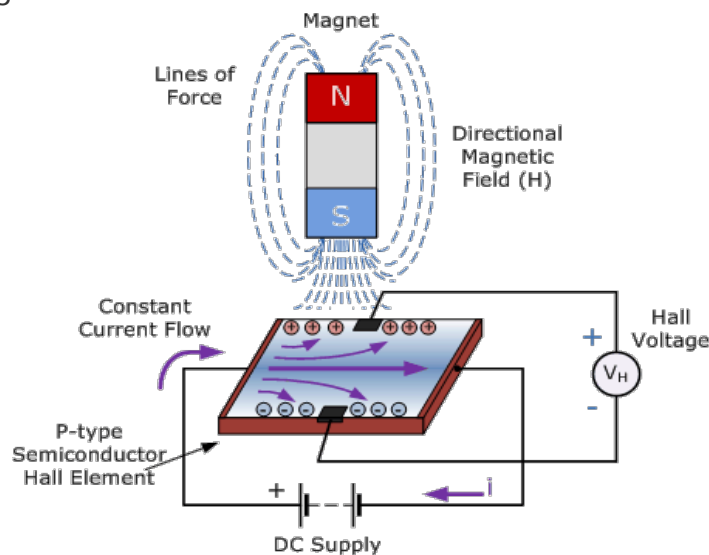
Figure 8. Operation of a Hall Effect Sensor
