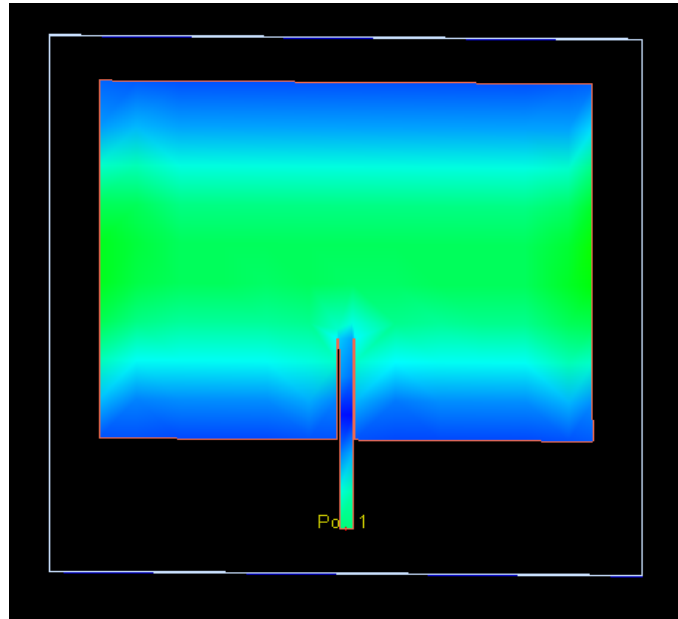
Figure 56. Advanced Design System E&M Representation of the Microstrip Patch Antenna
