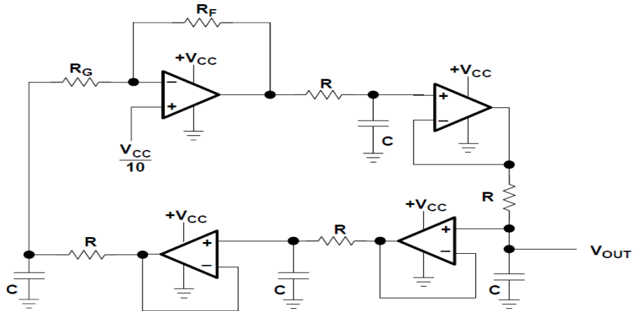
Figure 29. Bubba Oscillator Circuit Schematic
