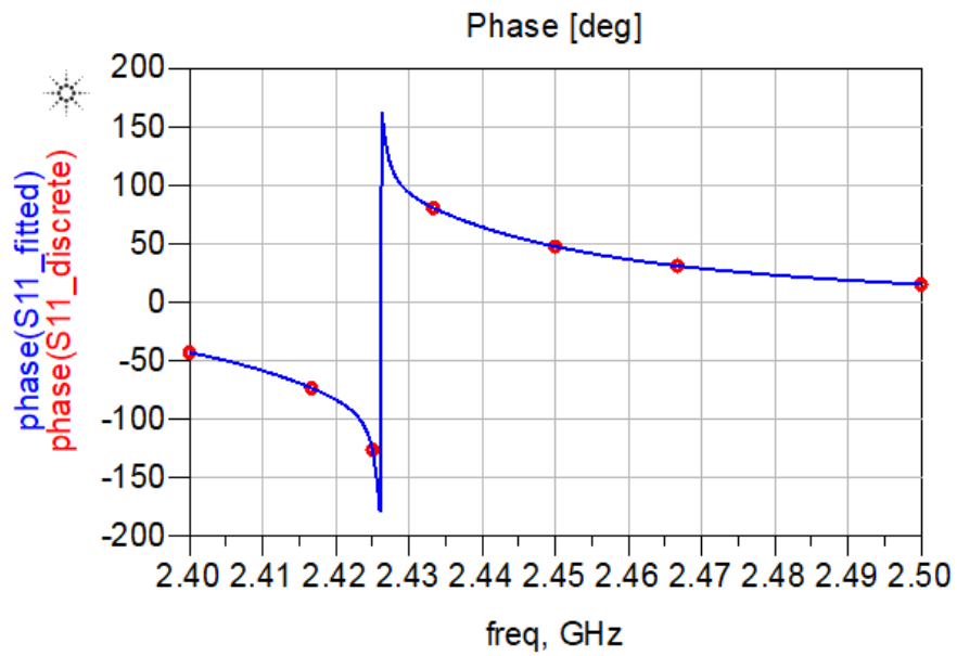
Figure 54. Microstrip Patch Antenna Port One Phase
