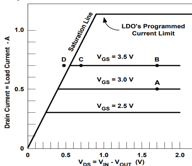
Figure 20. LDO Drain Current vs Voltage
