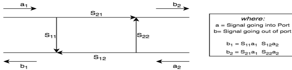
Figure 48. S-parameter Port Representation
