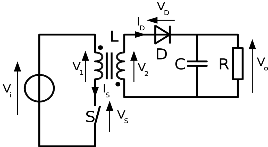
Figure 31. Flyback Converter Circuit Schematic.
