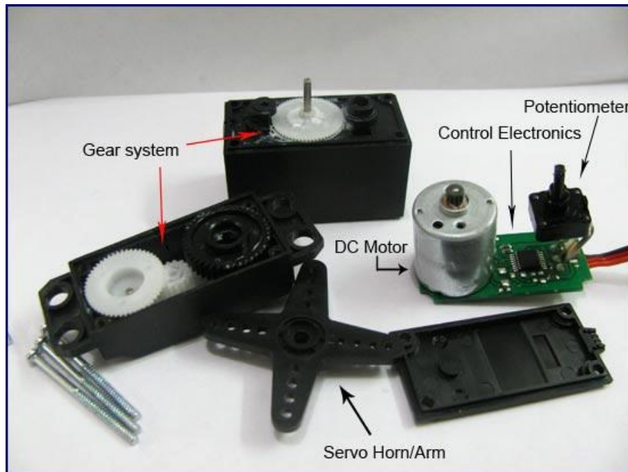
Figure 4. Inner Mechanism of a Servo
