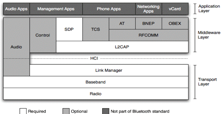
Figure 16. The Bluetooth Protocol Stack
