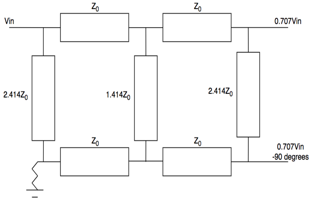
Figure 58. Broad bandwidth Quadrature Hybrid
