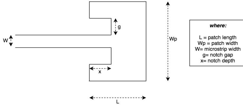
Figure 52. Microstrip Patch Antenna Parameters
