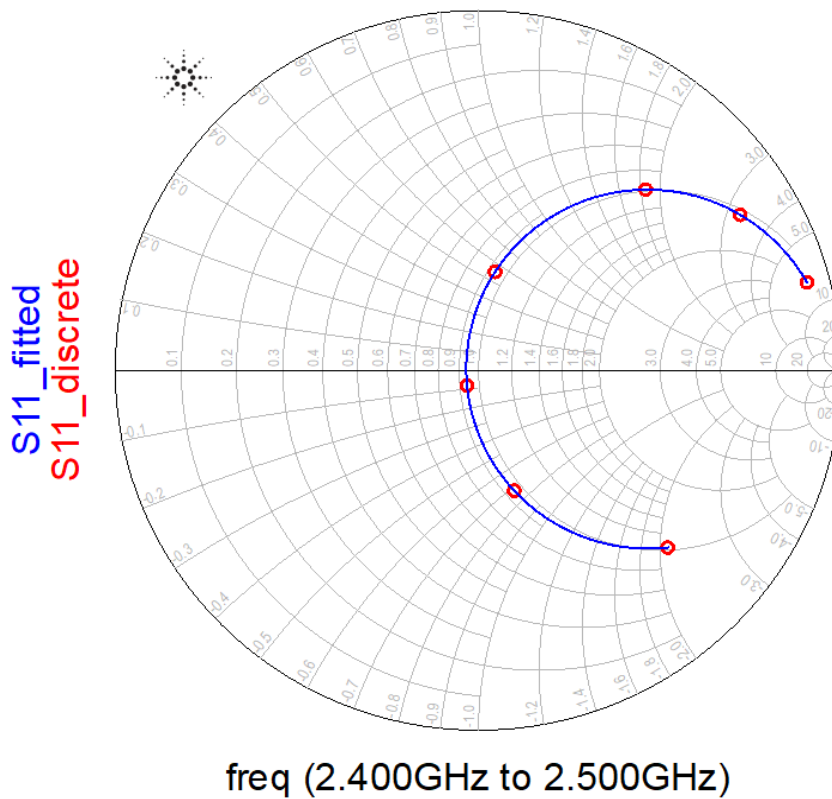
Figure 55. Microstrip Patch Antenna Smith Chart
