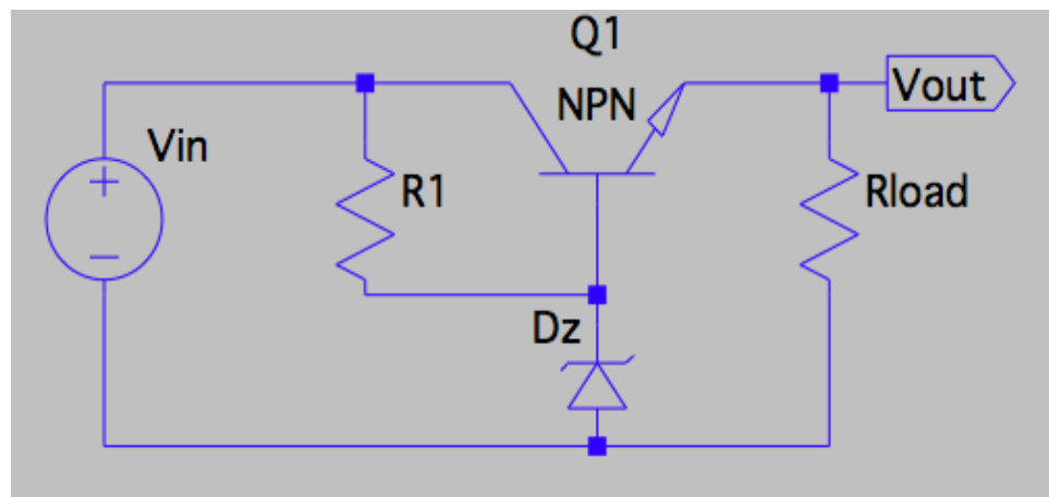
Figure 18. Transistor Regulator Circuit
