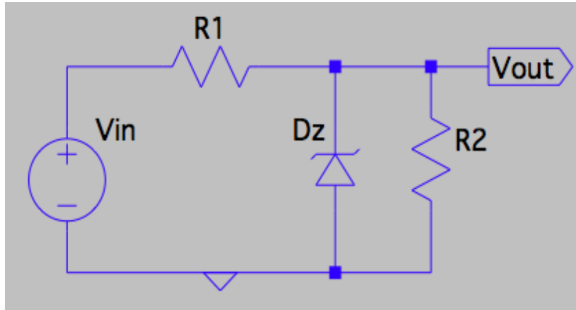
Figure 17. Shunt Regulator Circuit
