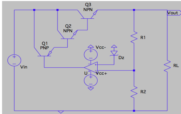
Figure 21. LDO Circuit
