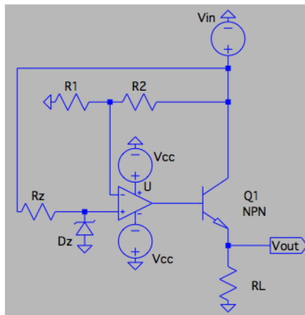
Figure 19. Op-Amp Regulator
