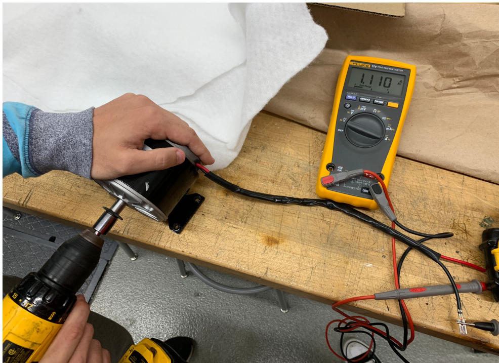
Figure 66. Amp Output of DC Generator
