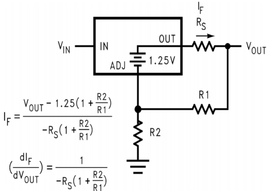
Figure 34. Voltage Regulator Battery Sense Circuit
