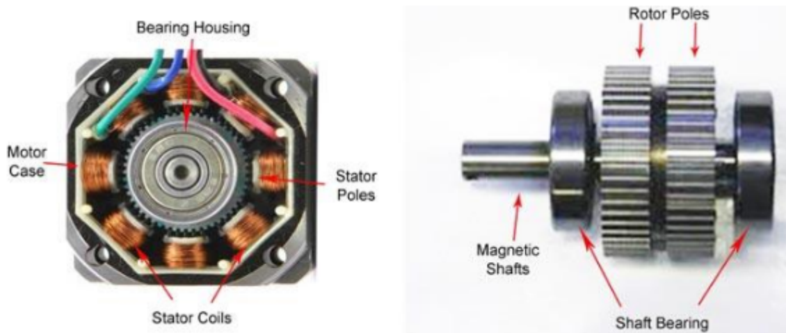
Figure 5. Inner Mechanism of a Stepper Motor
