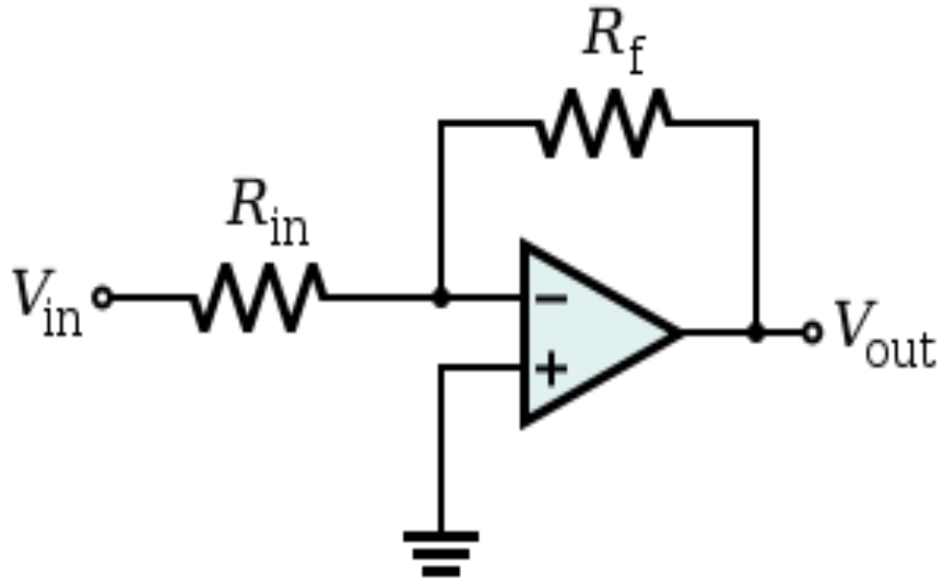
Figure 40. Op amp inverting circuit.
