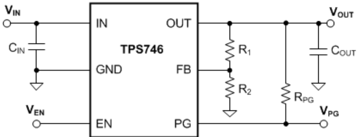
Figure 41. 2.5V to 1.8V LDO regulator schematic.
