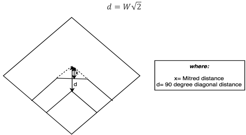
Figure 49. Mitred Bend
