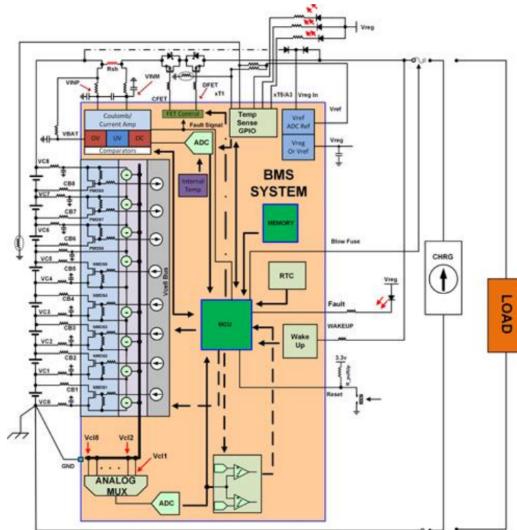
Figure 33. BMS Circuit Diagram.
