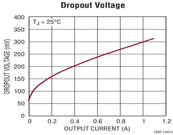
Figure 38. Current vs Dropout Voltage LDO.
