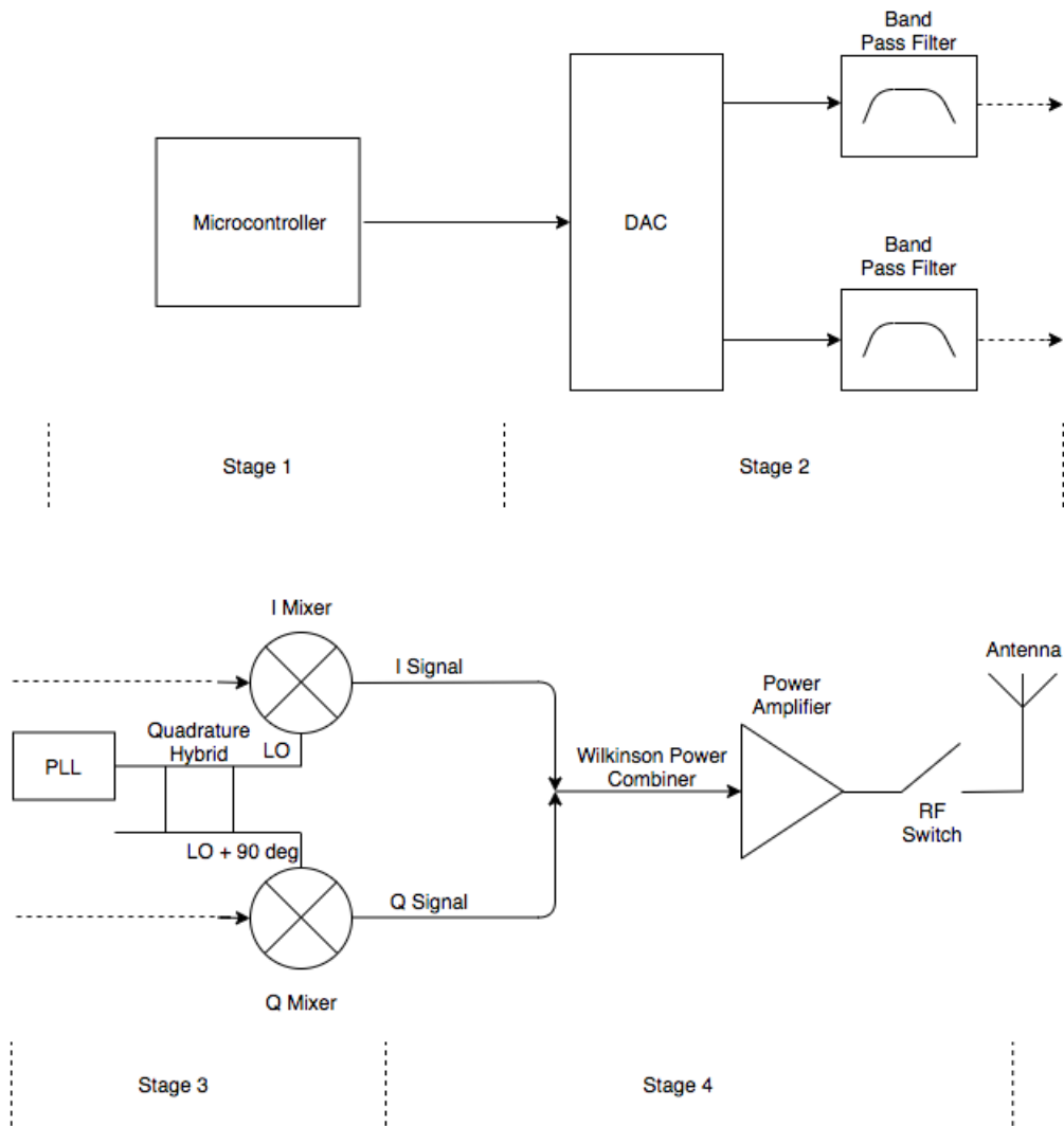
Figure 51. Transmit Path of the Transceiver
