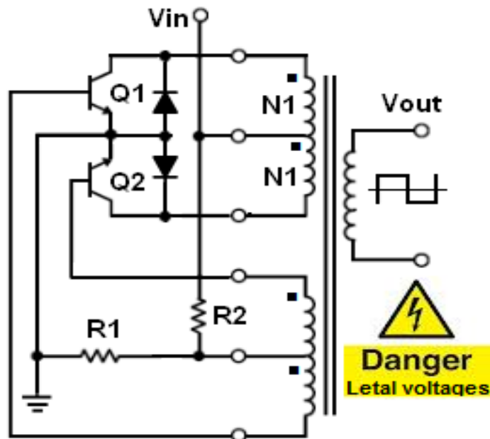
Figure 27. Push-Pull Converter Circuit.
