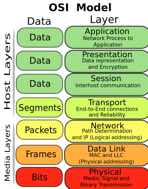
Figure 15. The OSI Model
