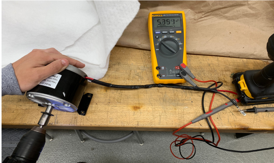
Figure 67. Voltage Output of DC Generator
