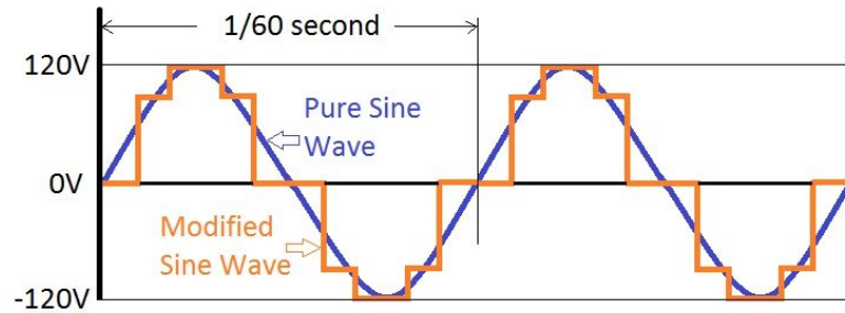
Figure 28. Pulse Width Modulation vs Pure Sine Wave
