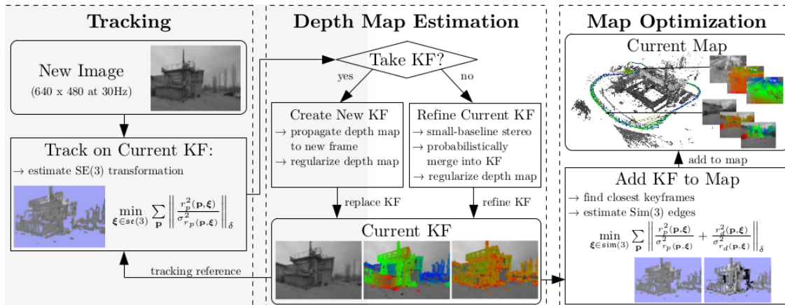
Figure 9: Overview of How LSD-SLAM Works used with reference from medium.com [7]
