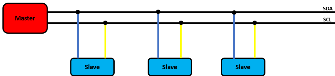
Figure 14: I 2 C Bus Configuration made by Mario Mcclelland
