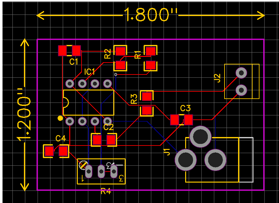
Figure 59: Perimeter Wire Generator Circuit PCB made by Brandei Dieter
