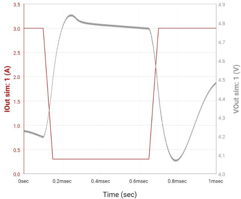
Figure 44: Load Transient Plot from TI Webench Power Design Simulator
