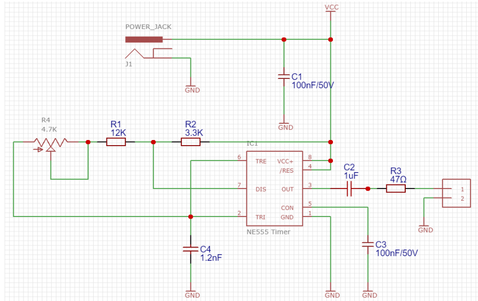
Figure 58: Perimeter Wire Generator Circuit Schematic made by Brandei Dieter
