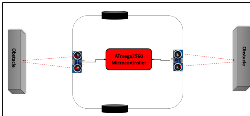
Figure 38: Sensors Subsystem 1 Design made by Brandei Dieter
