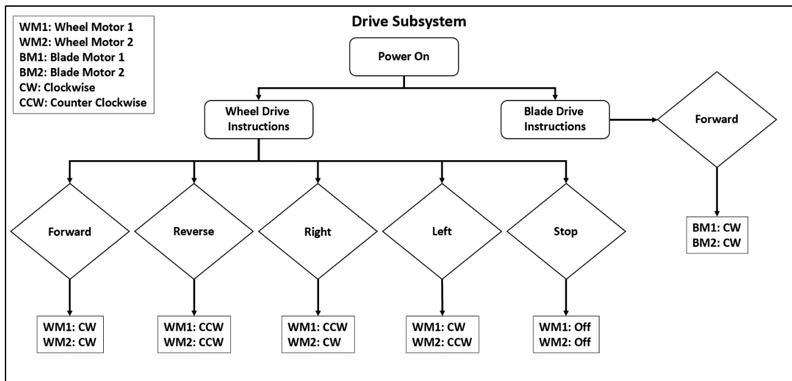
Figure 46: Drive Subsystem Flowchart made by Brandei Dieter
