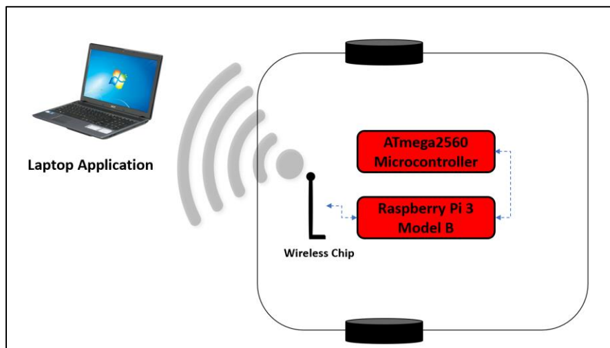
Figure 48: Wireless Communications Diagram made by Brandei Dieter
