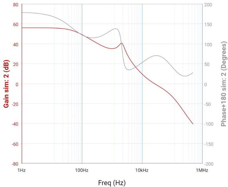
Figure 45: Bode Plot from TI Webench Power Design Simulator
