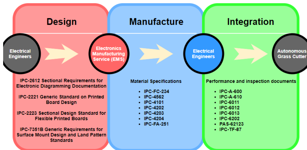
Figure 35: Flow of PCB Design and Implementation made by Christopher Entwistle
