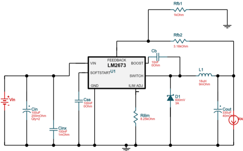
Figure 42: LM2673 Circuit Design from TI Webench Power Design Simulator
