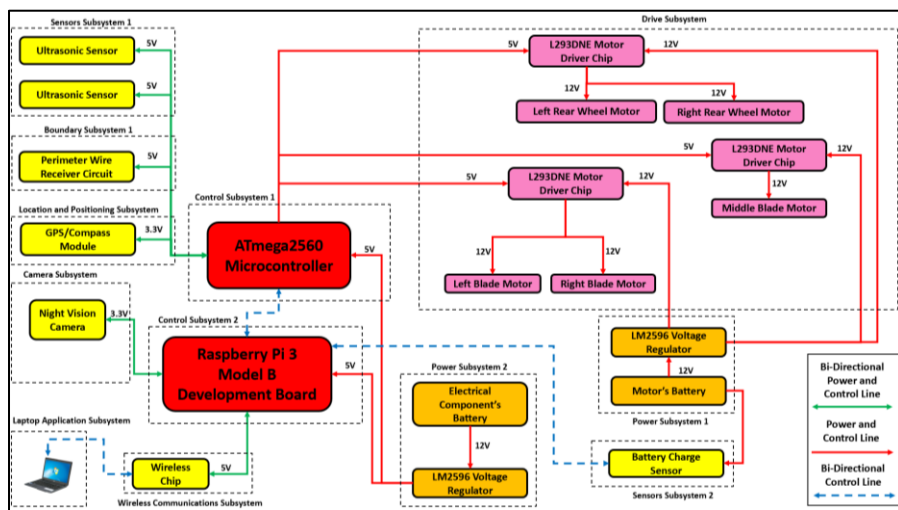
Figure 36: Updated Hardware Block Diagram of the Grass Cutter System made by Brandei Dieter
