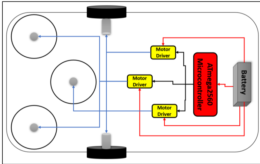
Figure 47: Drive Subsystem Diagram made by Brandei Dieter
