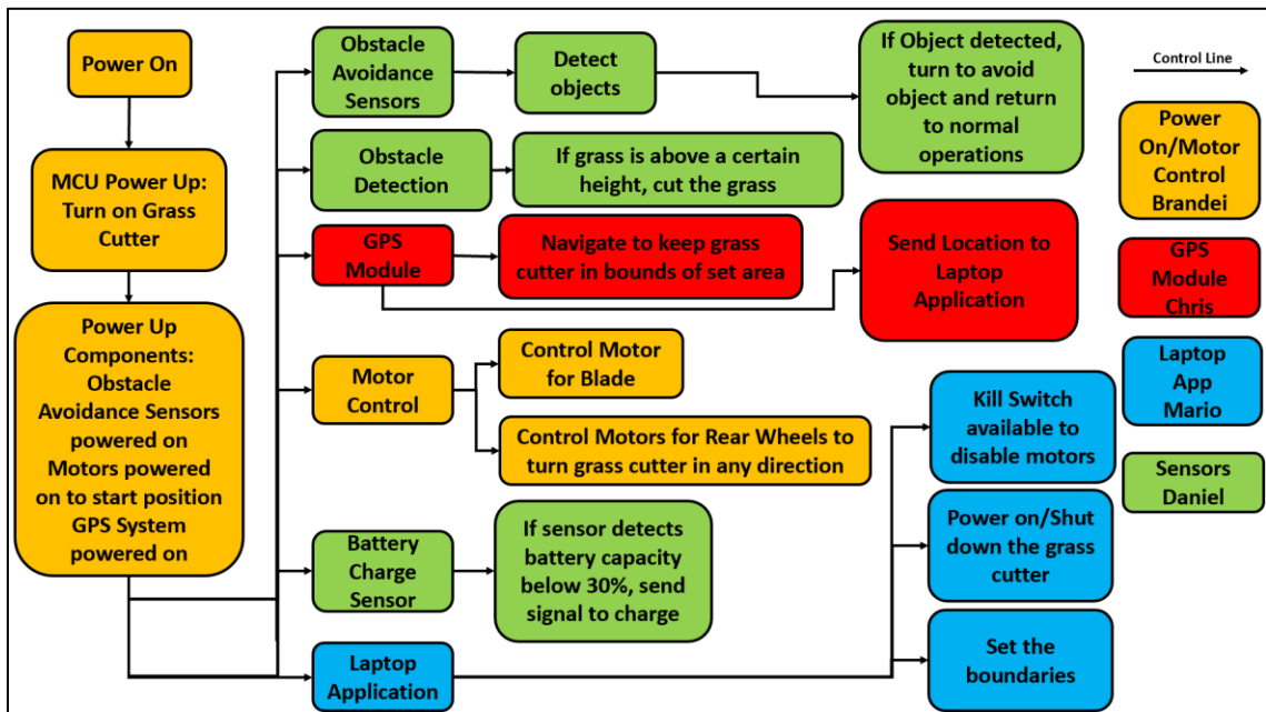
Figure 4: Possible Software Block Diagram made by Brandei Dieter
