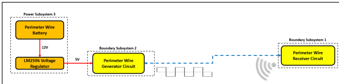
Figure 37: Updated Hardware Block Diagram of the Boundary System made by Brandei Dieter
