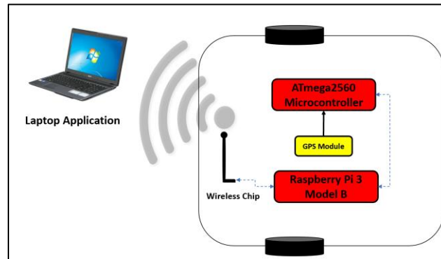
Figure 39: Location and Positioning Subsystem Diagram made by Brandei Dieter
