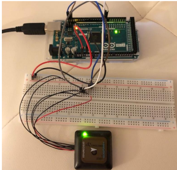
Figure 66: GPS Tested picture taken by Mario McClelland
