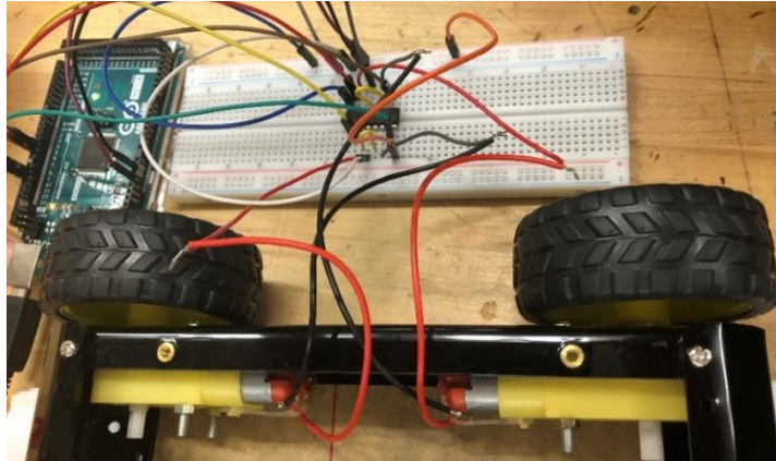
Figure 60: Motor Driver Chip and DC Motors Tested picture taken by Brandei Dieter
