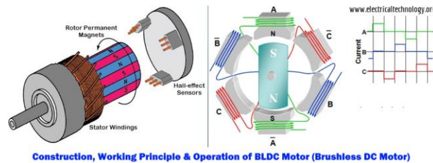
Figure 11: Brushless Motors Diagram used with reference from electricaltechnology.com [15]
