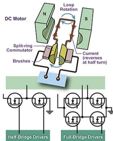
Figure 10: Brush DC Motors Diagram used with reference from Allegro Micro Systems [14]
