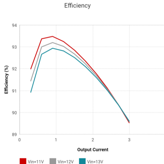
Figure 43: Efficiency Versus Output Current Plot from TI Webench Power Design Simulator
