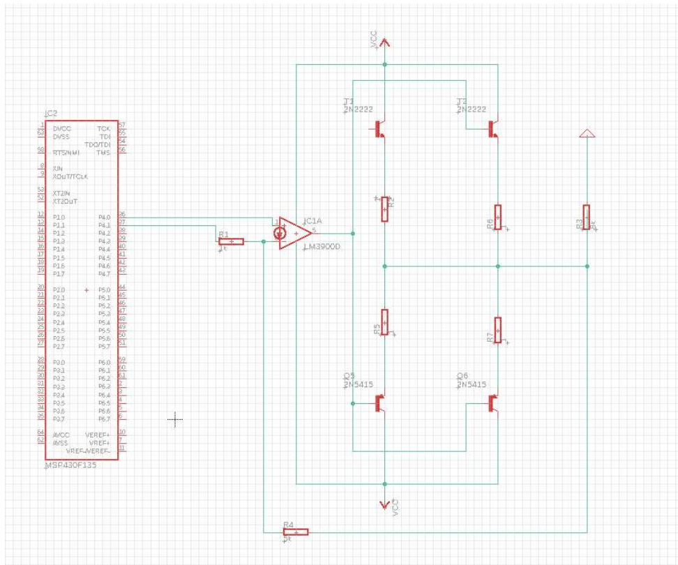
Figure: Schematic of Initial Custom PCB Design
