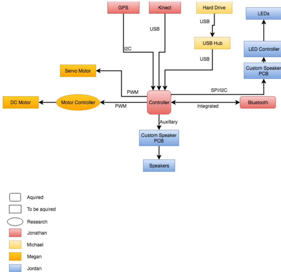
Figure: Hardware Block Diagram
