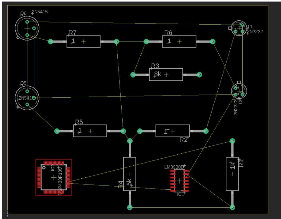
Figure: PCB Board Design from EagleCAD
