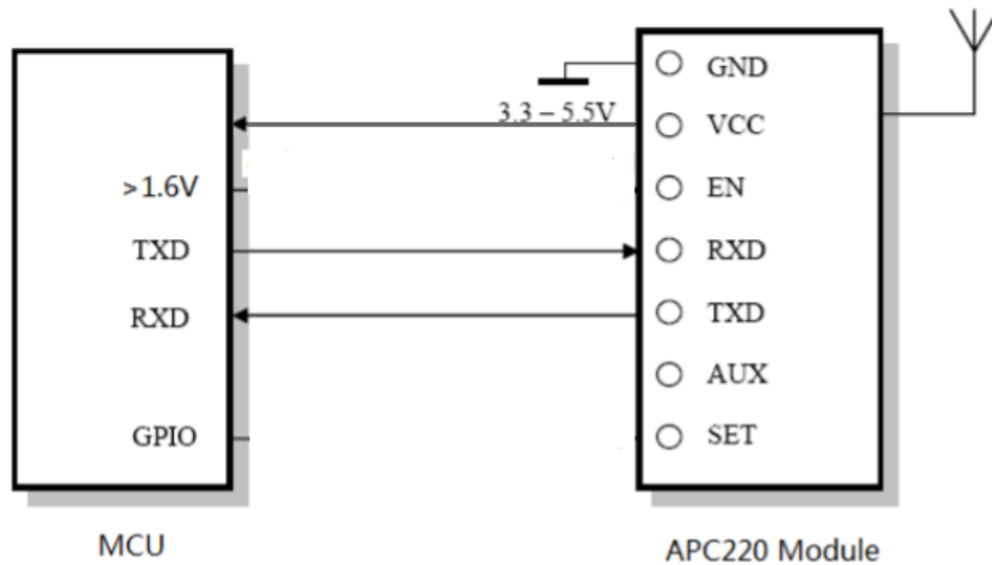
Figure 75: RF Setup
