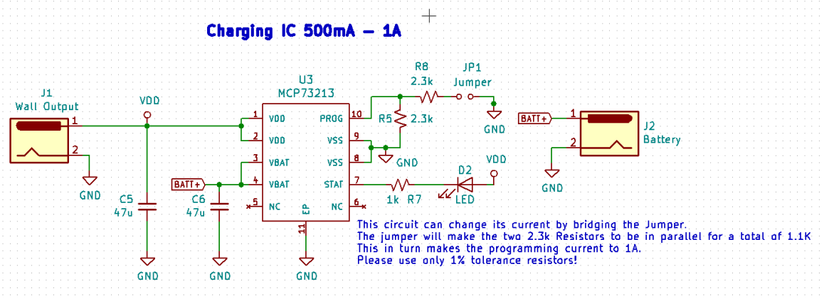
Figure 68: Charging Circuit Schematic
