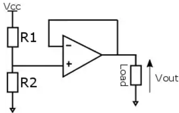
Figure 55: Operational Amplifier
