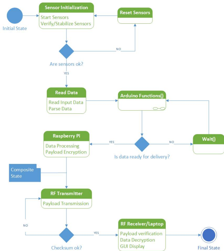
Figure 73: State Machine Diagram
