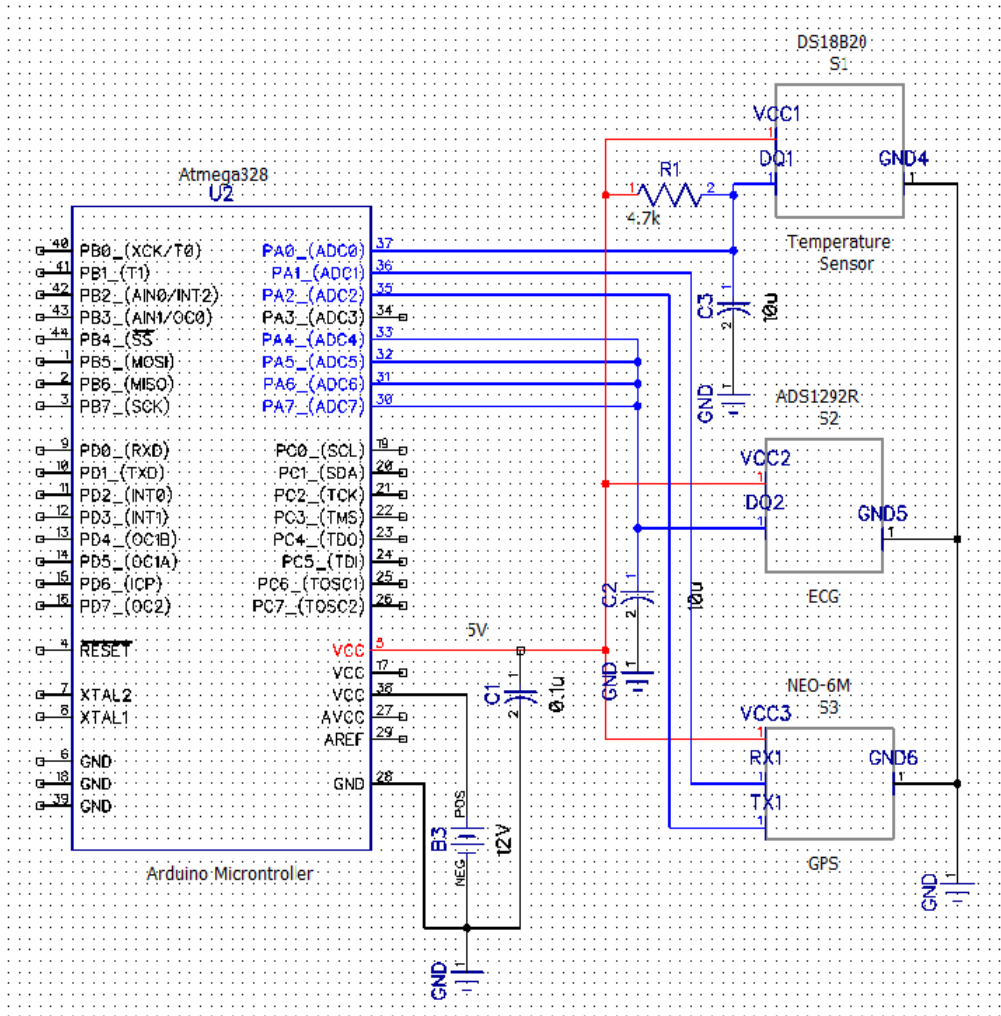
Figure 63: Arduino Circuit
