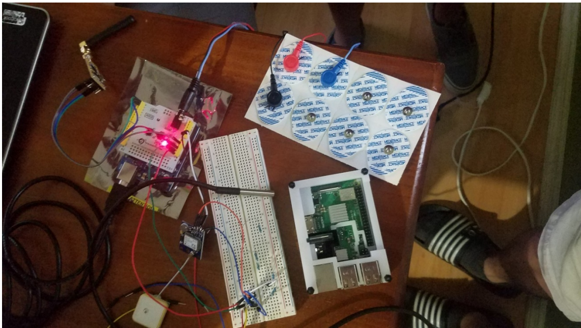
Figure 76: Breadboard Testing
