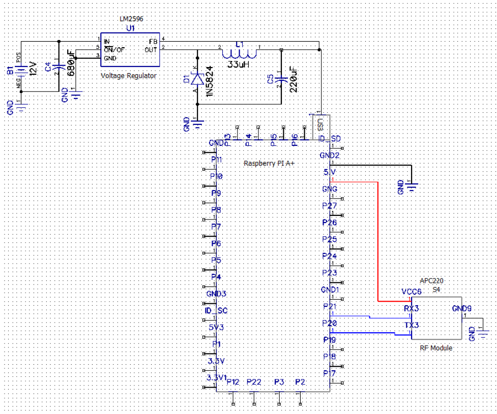
Figure 64: Raspberry Pi Circuit
