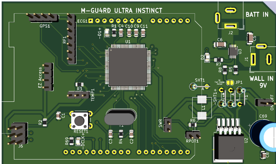
Figure 53: Finalized PCB Design
