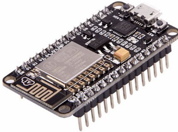
Figure 12: NodeMCU
