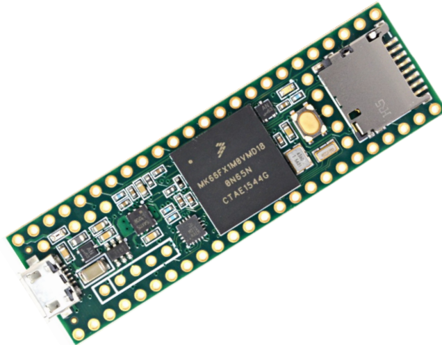
Figure 13: Teensy 3.6
