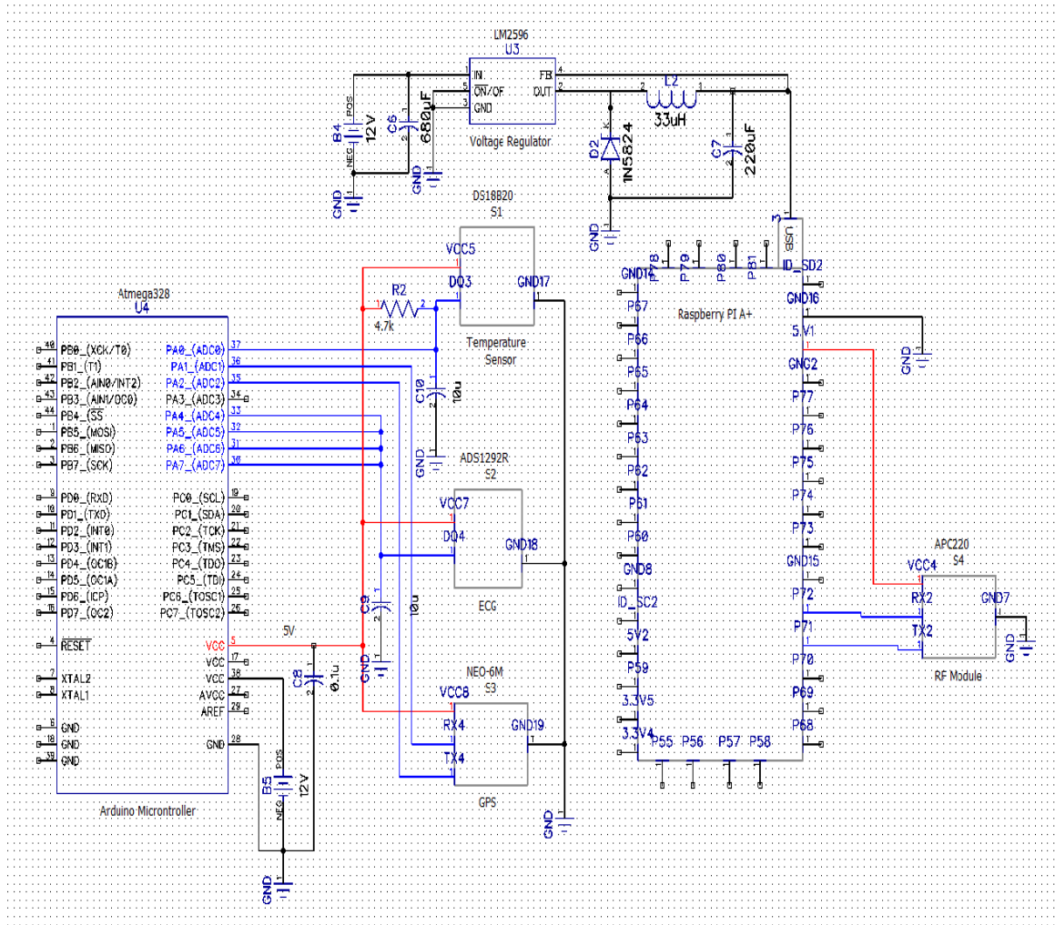
Figure 66: Overall Schematic
