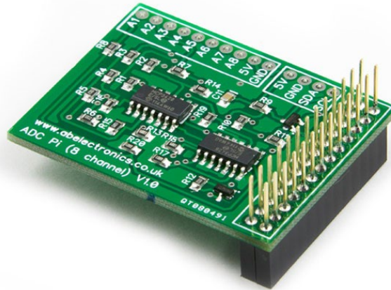
Figure 46: Raspberry Pi ADC Chip
