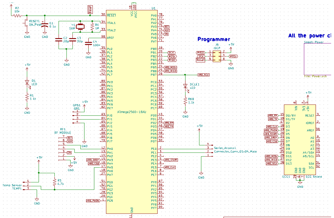
Figure 67: Finalized Overall Schematic
