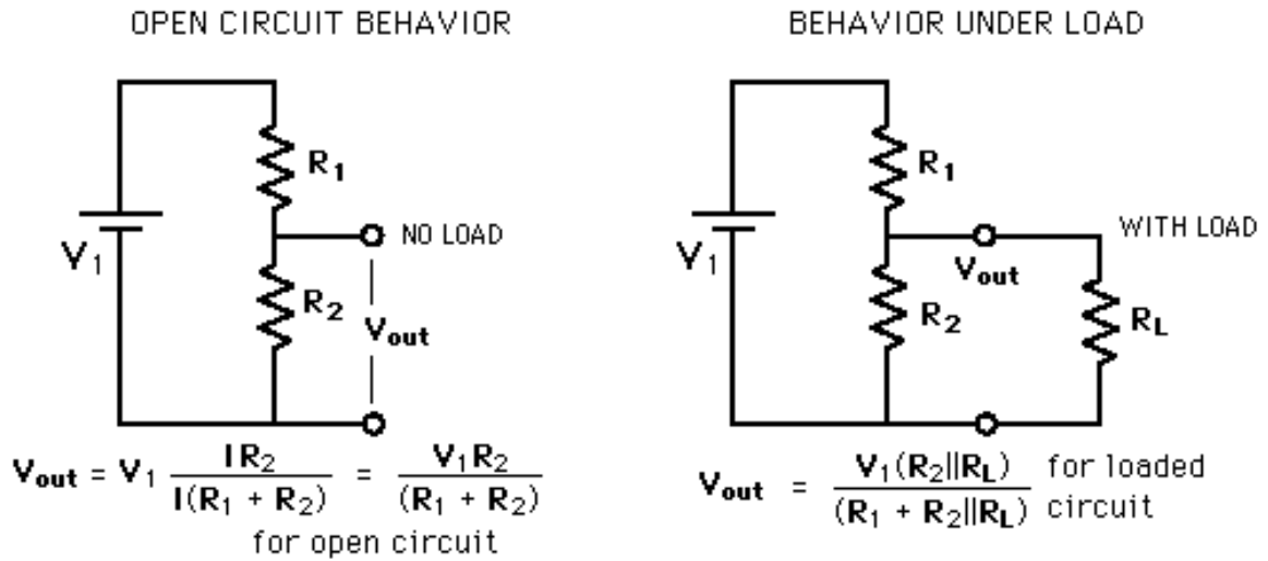
Figure 54: Voltage Divider
