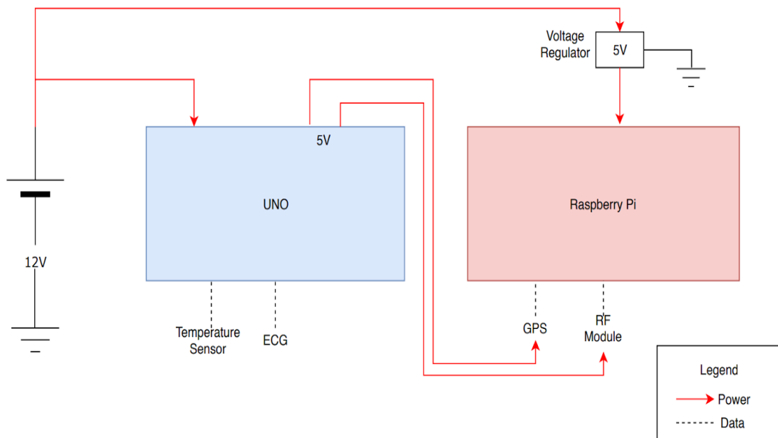
Figure 60: Tx High Level Diagram
