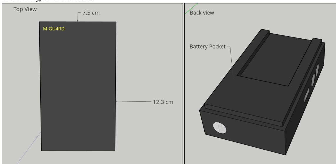
Figure 70: Casing Dimensions
