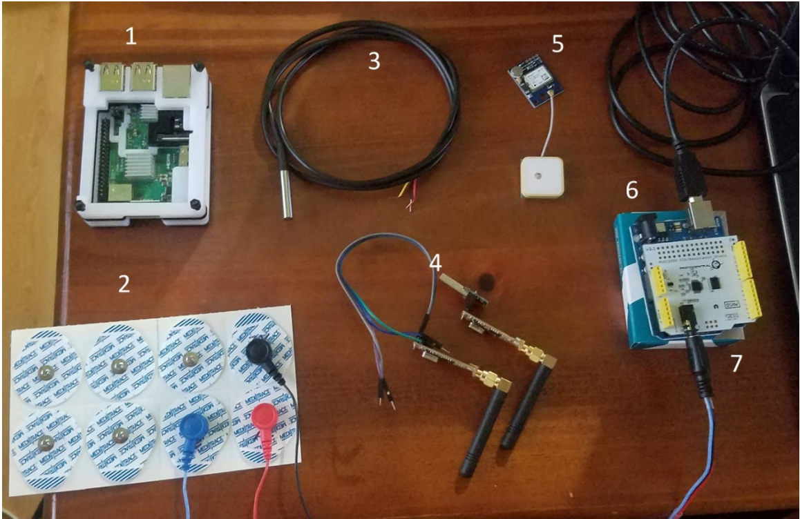
Figure 50: Core Components of M-GU4RD
