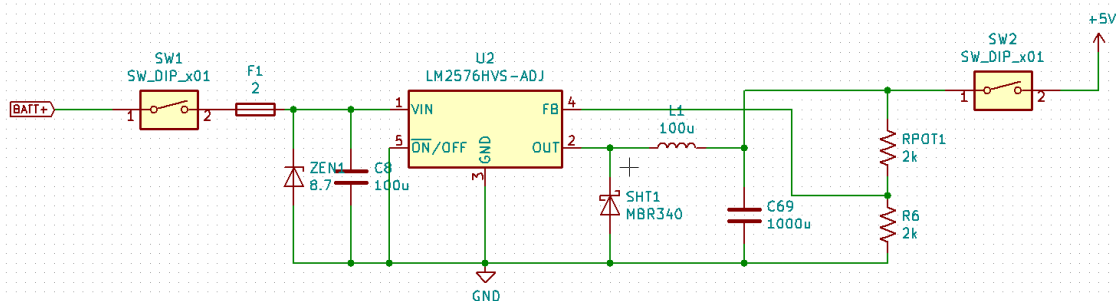
Figure 69: Buck Converter Circuit Schematic
