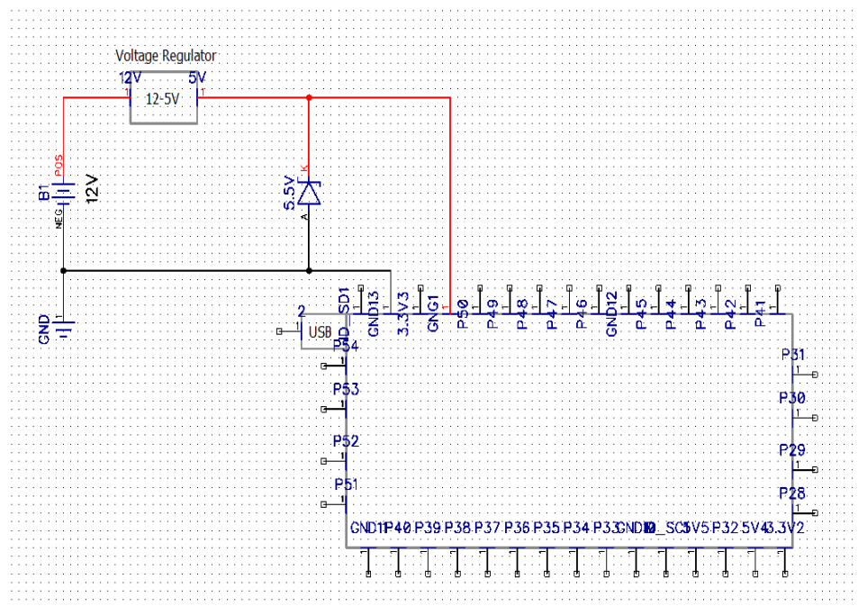
Figure 65: Safety Circuit
