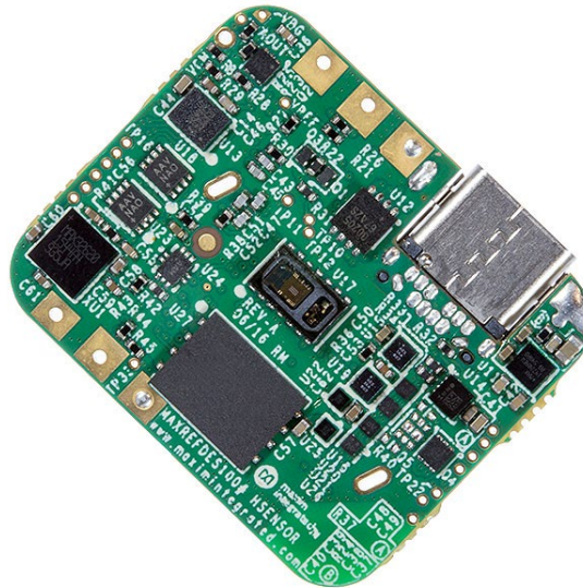
Figure 22: MAXREFDES100
