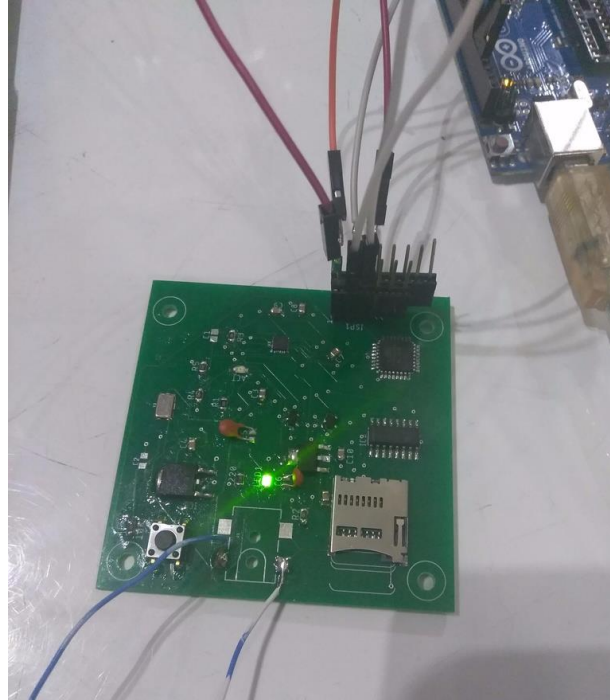
Figure 13: Printed Circuit Board Final, Using In-System Programming
