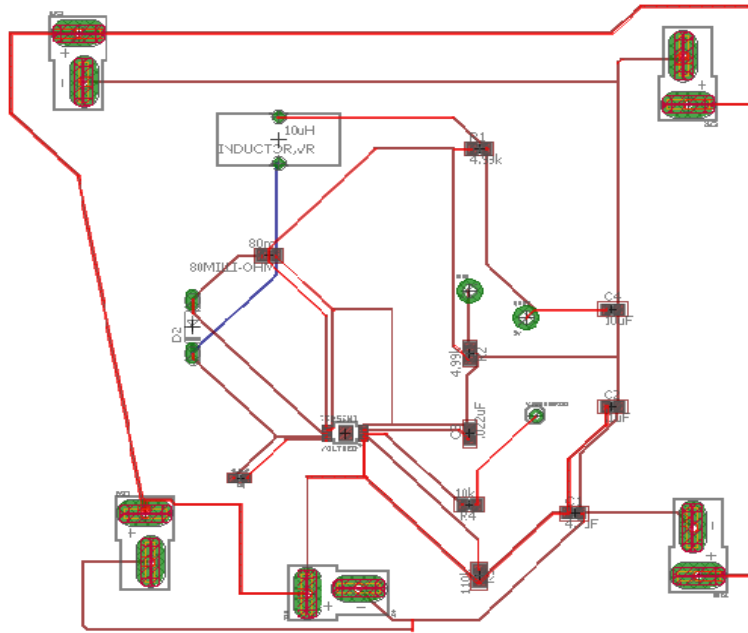
Figure 18 : Power Distribution Board Layout
