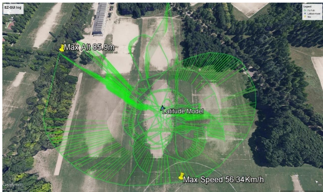
Figure 24: EZ-GUI KML converter flight path [17]
