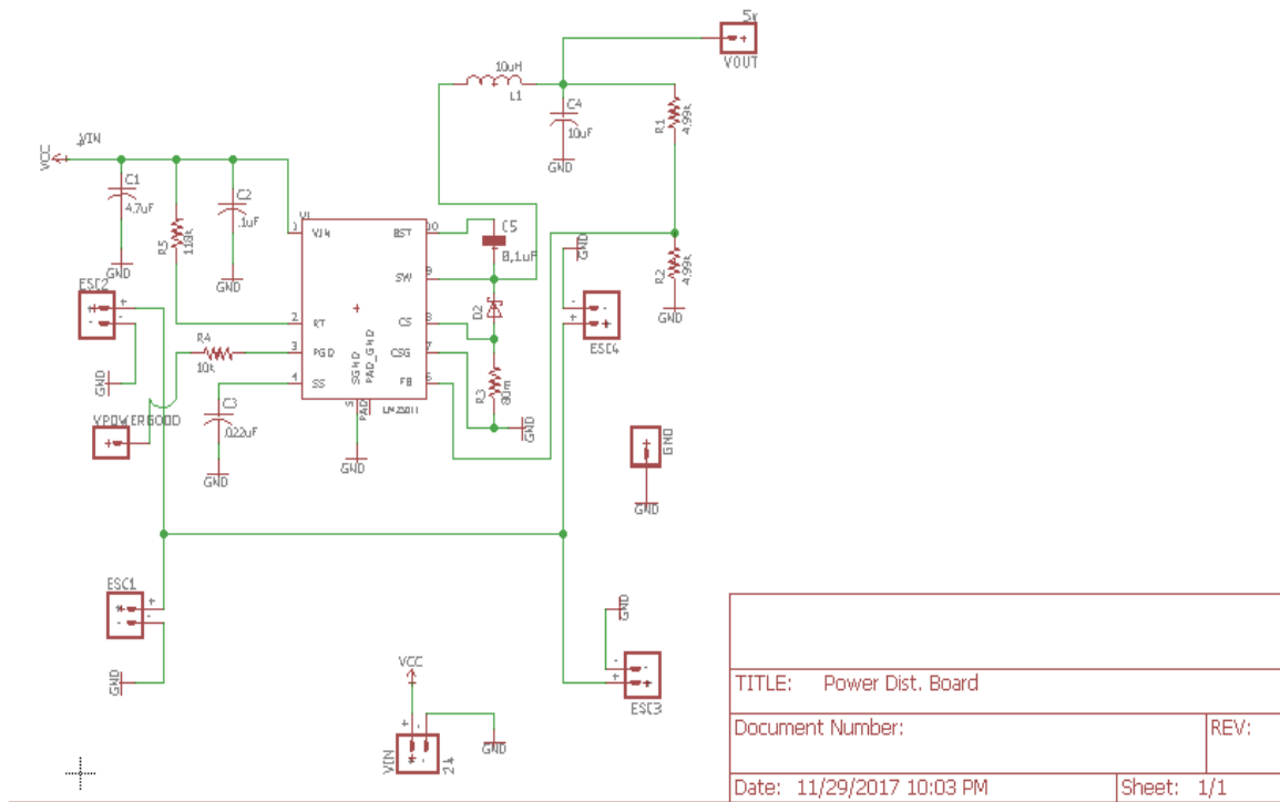
Figure 17: Power Distribution Board– Custom Fabricated-Switching Voltage Reg. Rev01
