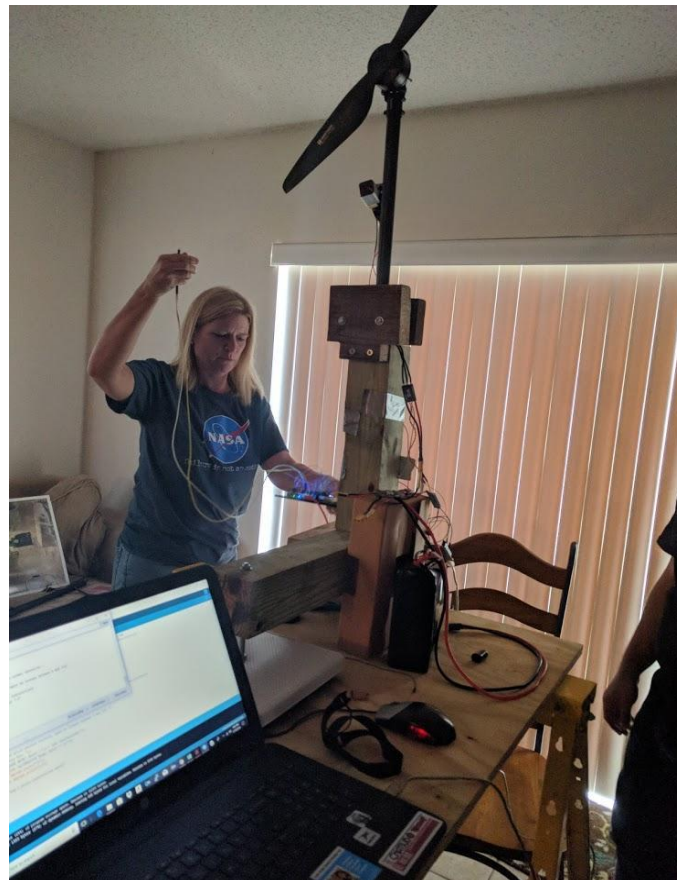
Figure 26: Thrust Testing Rig
