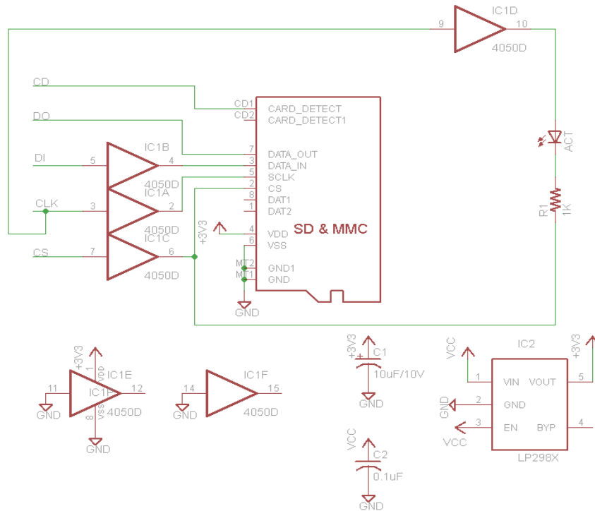
Figure 11: Eagle CAD electrical schematic diagram, black box storage
