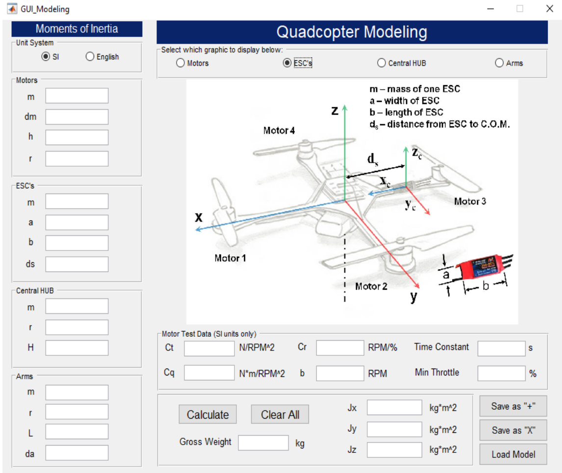
Figure 8: Quad Sim Modeling- Moments of Inertia
