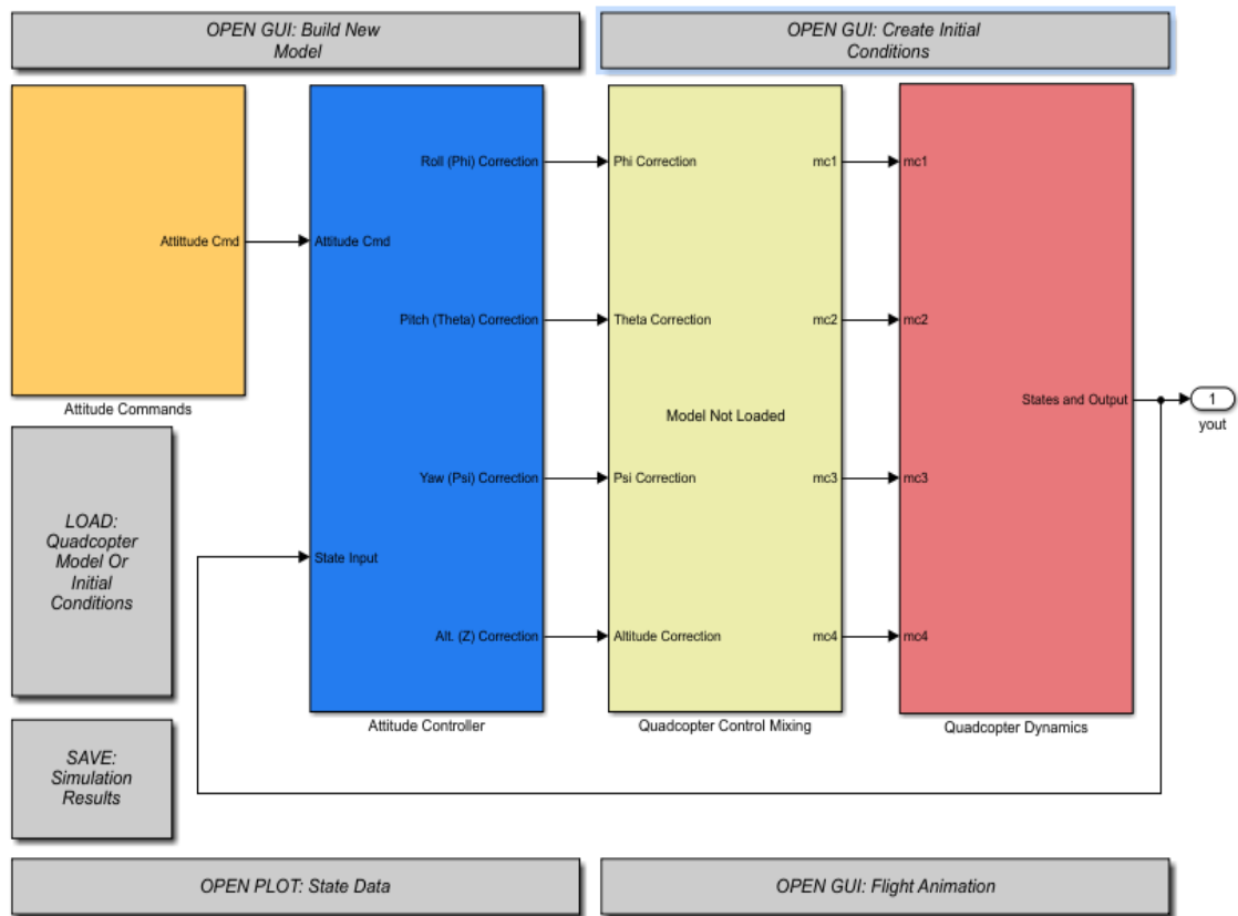
Figure 9: Quad Sim Attitude Control Blocks
