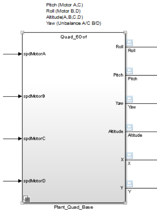
Figure 25: MIMO block
