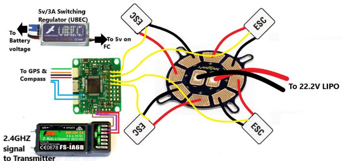
Figure 16: Power distribution Wiring Diagram
