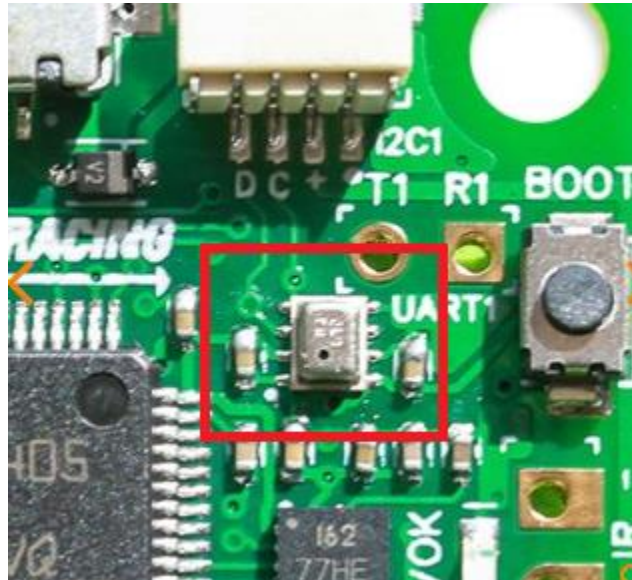
Figure 15: BMP280 barometer sensor mounted to flight control
