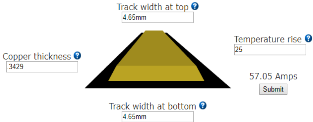
Figure 19: Trace Width Calculation for 57 A Carrying Capacity [14]
