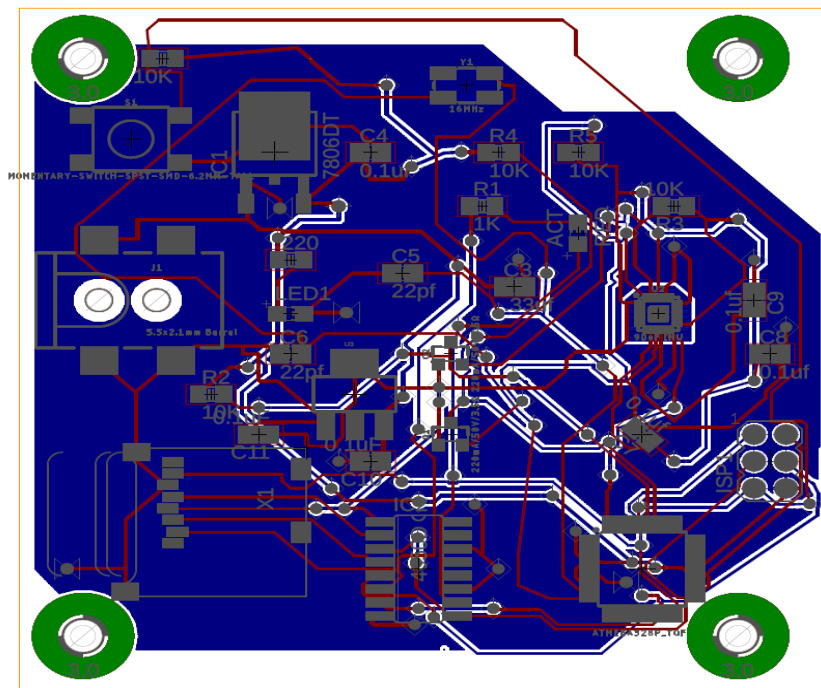
Figure 12: Printed Circuit Board Layout, Black Box Rev. 03
