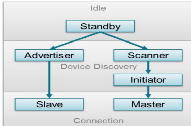
Figure 28: GAP State Diagram [39, reprinted with permission from TI]
