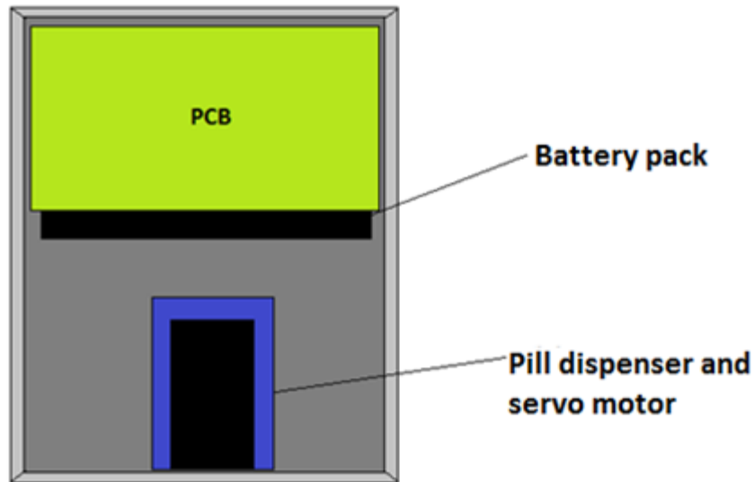
Figure 35: Inside of Casing
