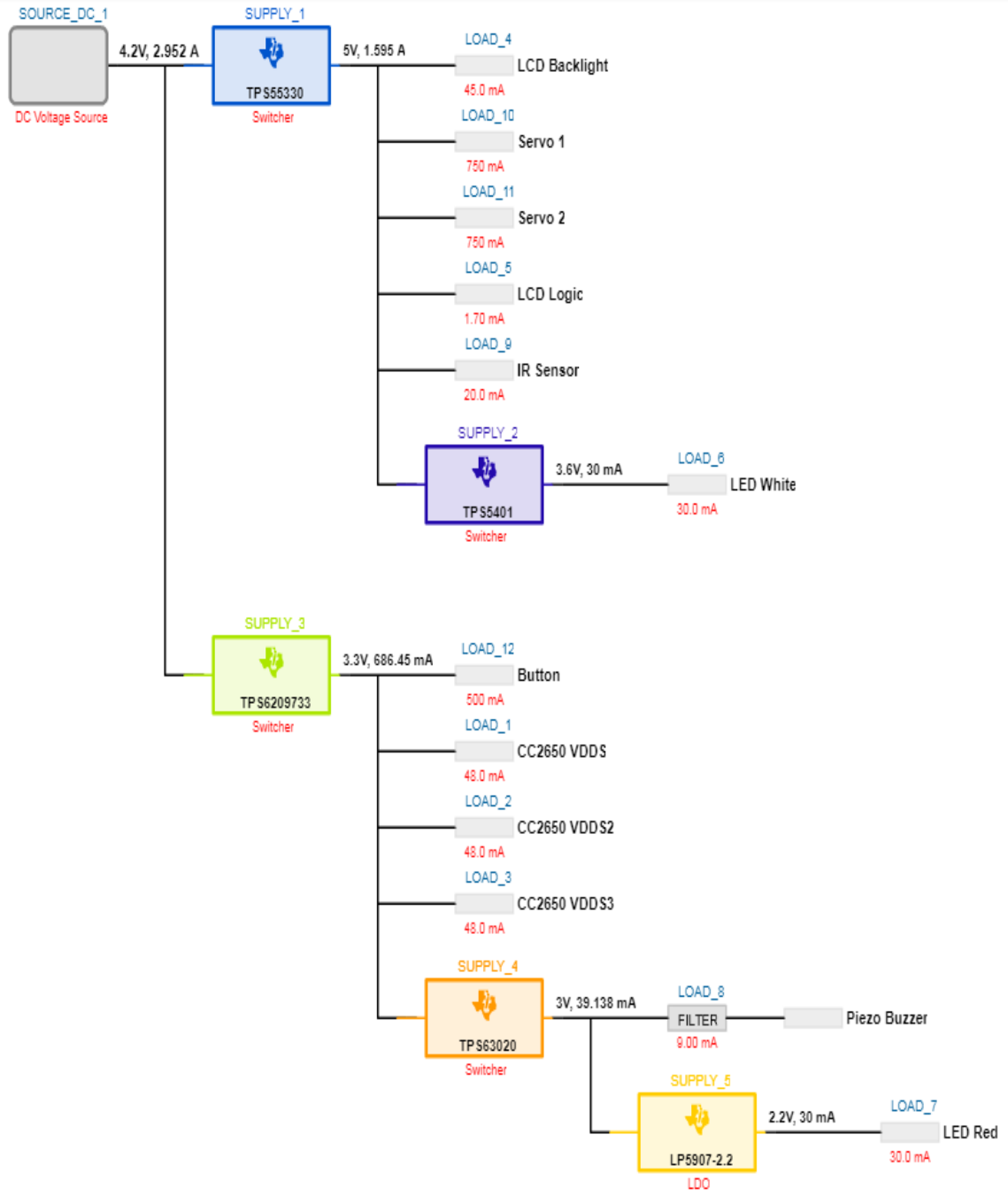
Figure 25: Overview of Power Distribution [Custom design via TI Webench]
