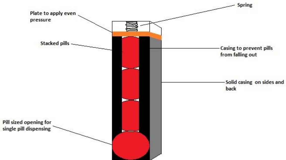
Figure 10: Pill Dispenser
