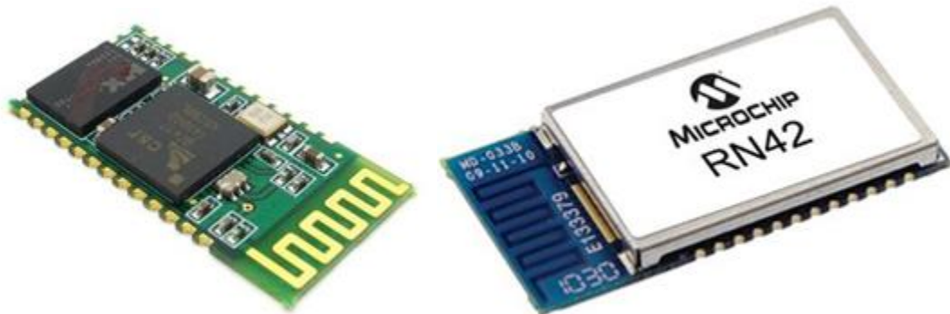
Figure 9: HC-05 Bluetooth Module (left), RN42 Bluetooth Module (right) [reprinted with permission from Microchip.com]
