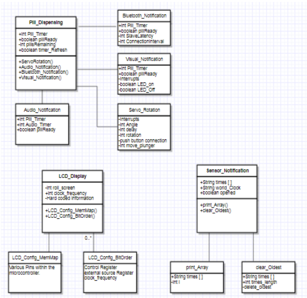
Figure 31: Software Class Diagram
