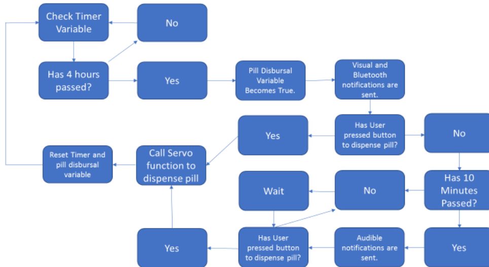
Figure 30: Pill Disbursal Flow Chart
