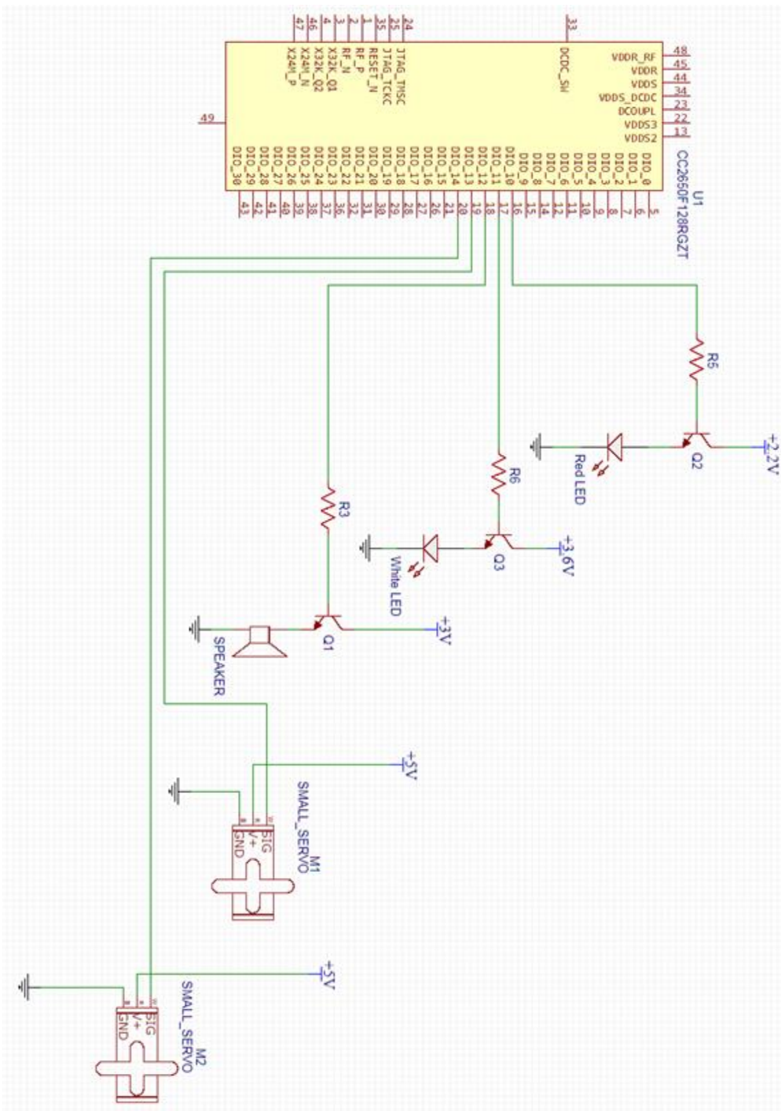
Figure 27: MCU to LEDs, Buzzer, and Servo Motor Units [Custom design created in EasyEDA]
