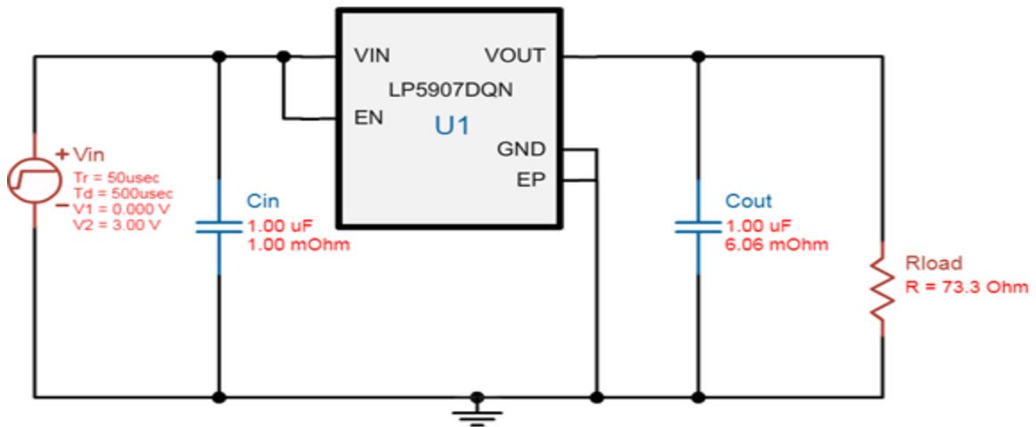
Figure 24: Fifth voltage regulator [Custom design via TI Webench]
