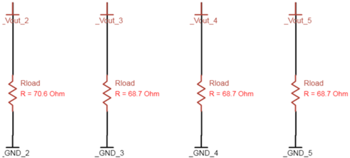
Figure 22: Top: Regulator setup with values Bottom: Loads attached to regulator output [Custom design via TI Webench]
