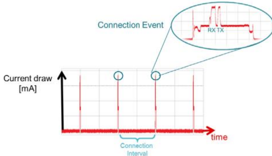
Figure 29: Connection Event and Interval [39, reprinted with permission from TI]
