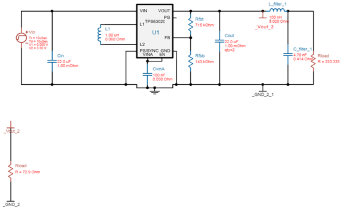
Figure 23: Fourth voltage regulator [Custom design via TI Webench]
