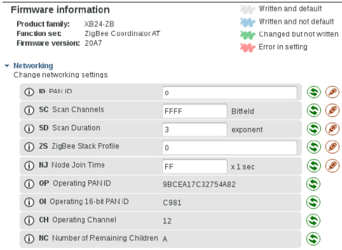
Figure 52 – XCTU Configuration Window
