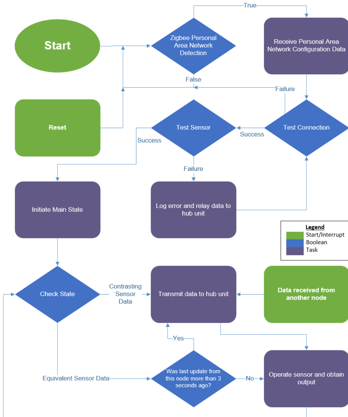
Figure 45 – Software Flowchart: Sensor Unit
