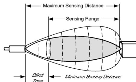
Figure 16 – Blind zone of an ultrasound sensor
