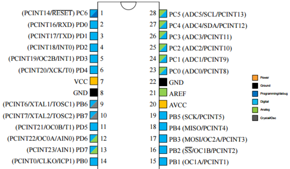
Figure 68 – Atmega328P Pin Out Diagram (used with permission from Atmel)
