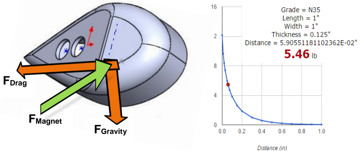
Figure 58 – Peripheral Sensor Force Diagram
