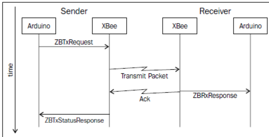
Figure 50 – Network Flow Diagram (used with Permission from Packet)
