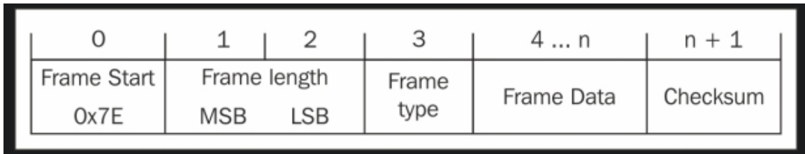
Figure 51 – Layout of a frame using the API module (used with permission from Packt)
