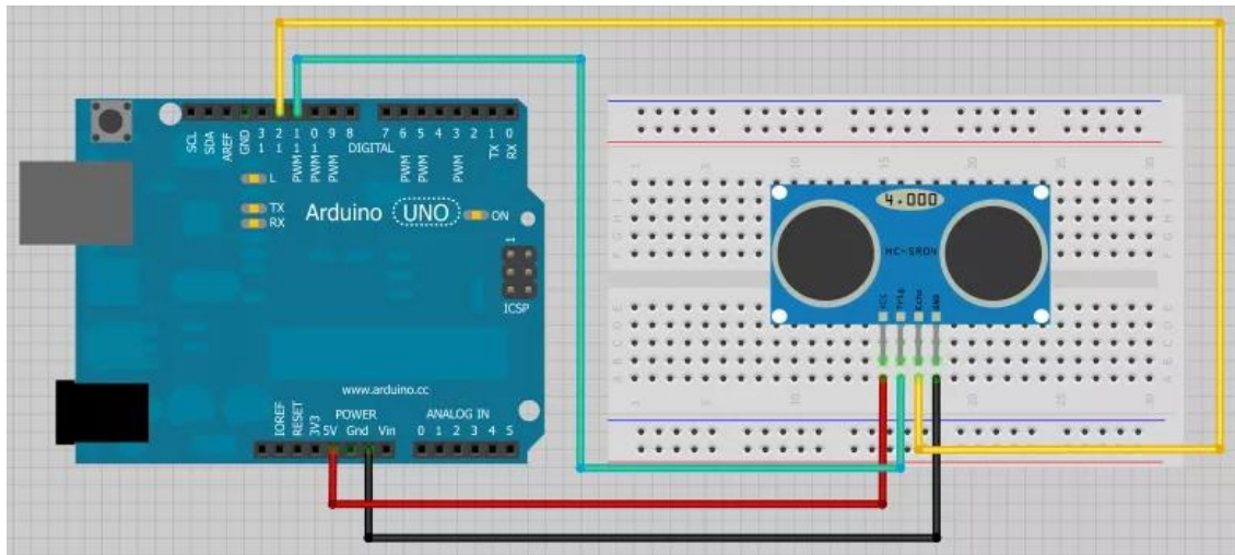
Figure 54 – Sensor's Layout and Integration with the System
