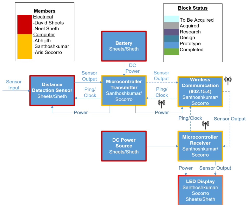
Figure 30 – Hardware Block Diagrams
