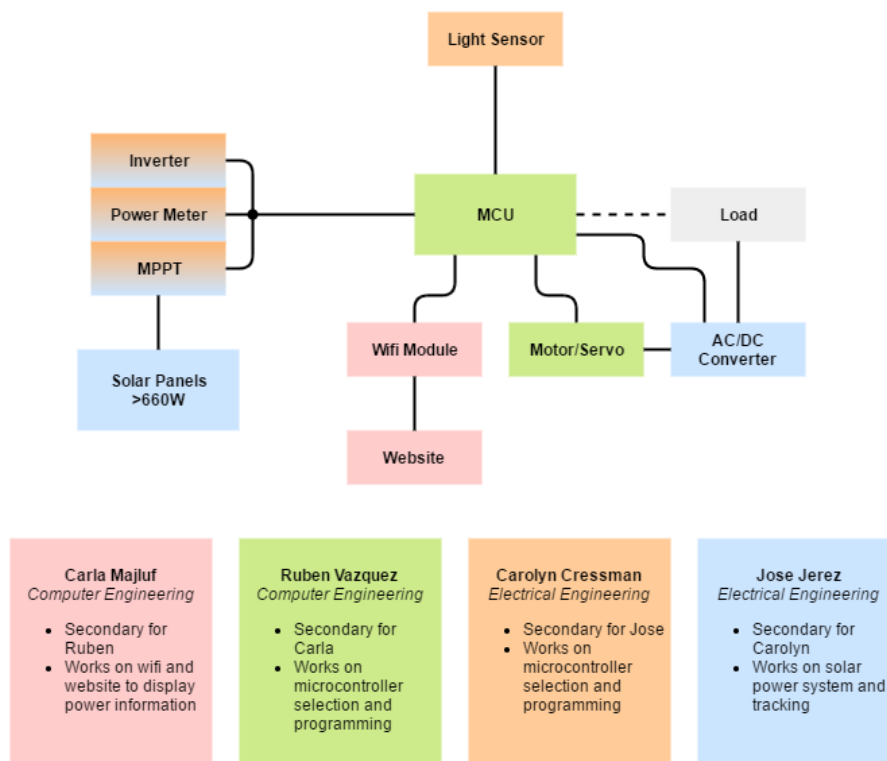
Figure 5.1.1 – Full-scale Diagram
