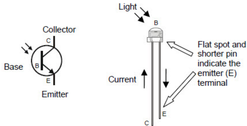
Figure 5.3.3 – Circuit Symbol and Figure of an NPN Phototransistor
