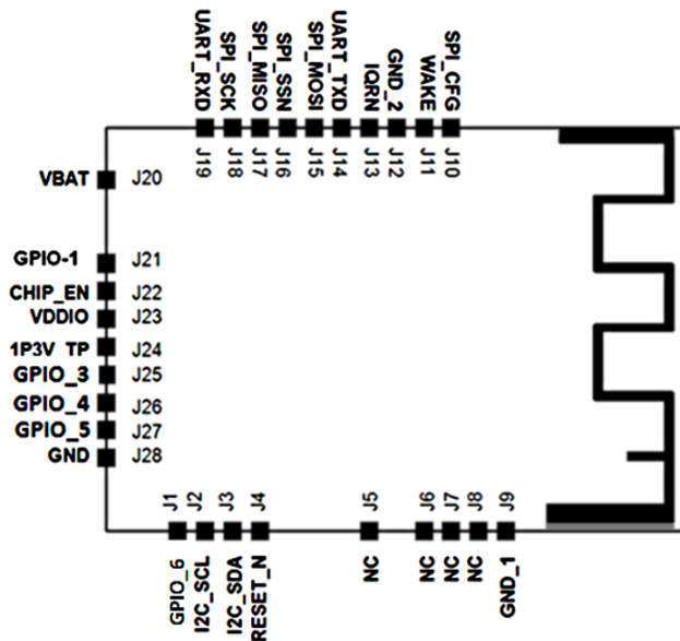
Figure 5.4.6 – WiFi Module Pin Assignments
