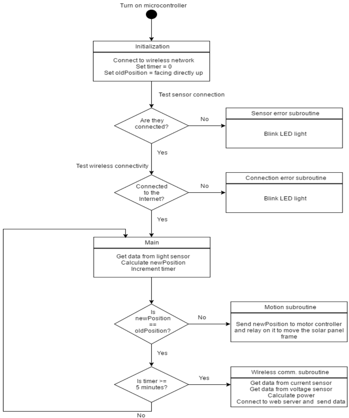
Figure 6.3.1 – Microcontroller's Code State Diagram
