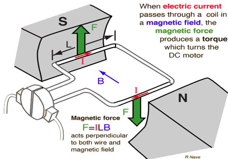
Figure 4.9.1 – Electromagnetism Principle of DC Motors
