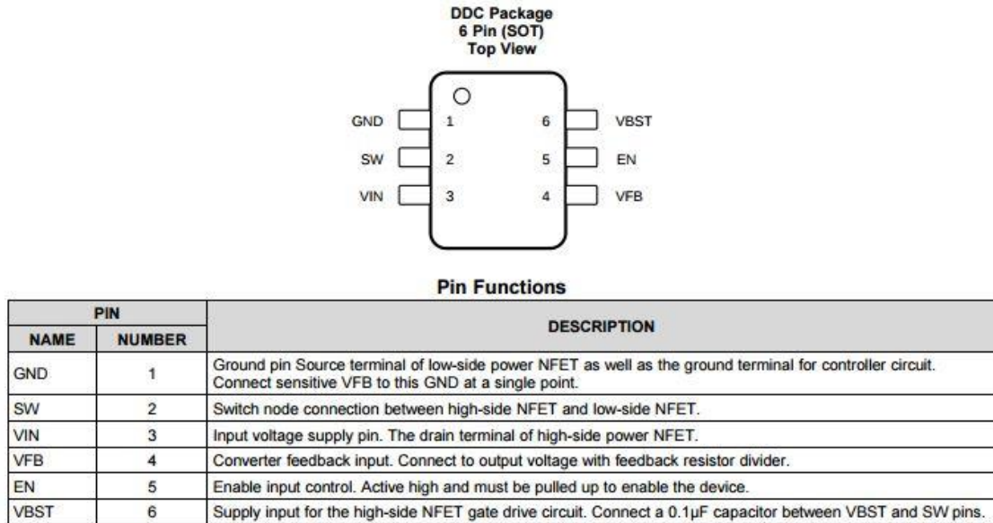
Figure 5.2.10 – Pin/Out Diagram from Datasheet
