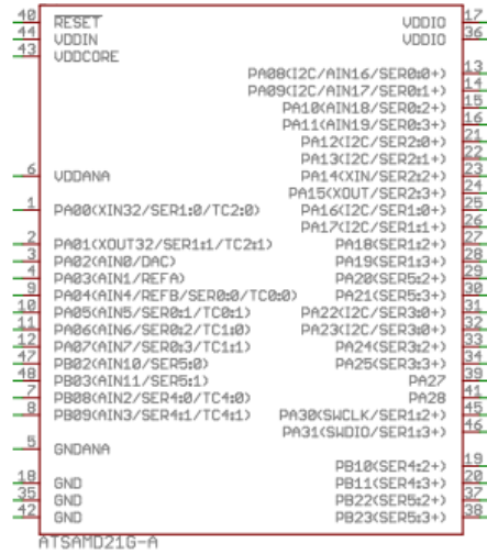
Figure 5.3.12 – Schematic of the ATSAM D21G18 MCU
