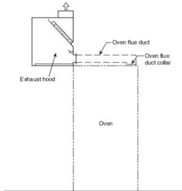
FIGURE 5.1.8.1 Typical Section of Eyebrow-Type Hood.
