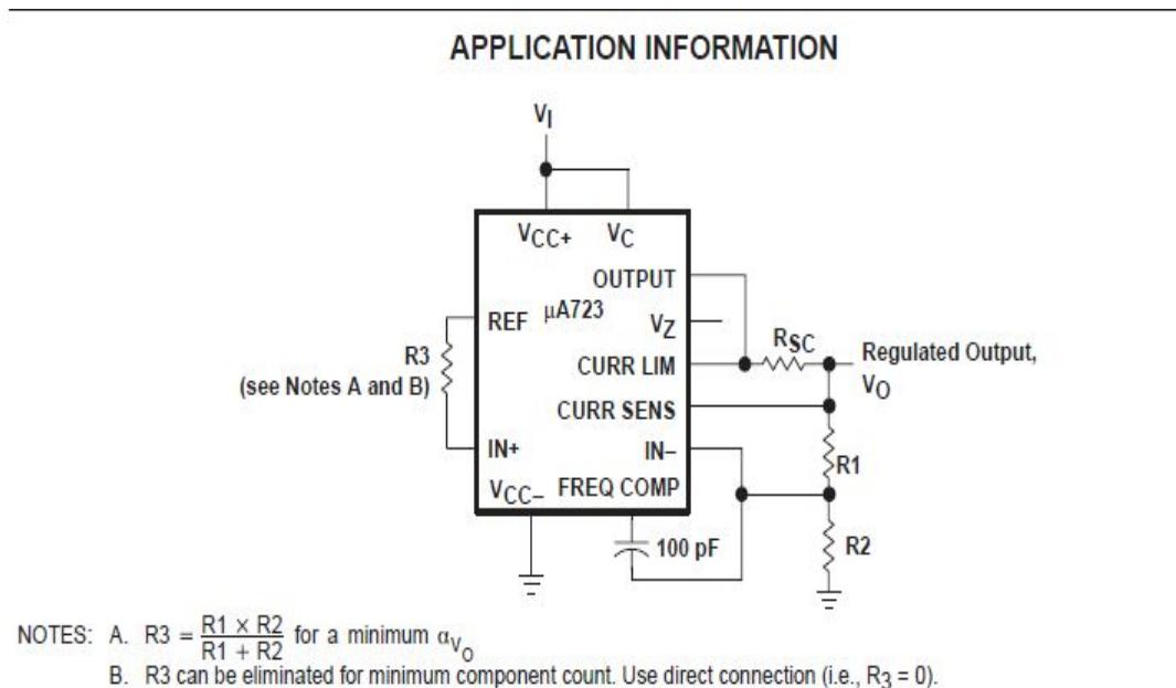
Figure 2. Basic High-Voltage Regulator ( V_O = 7\text{ V to }37\text{ V} )
