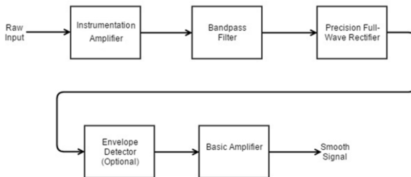
Figure 39: EMG Sensor General Circuit
