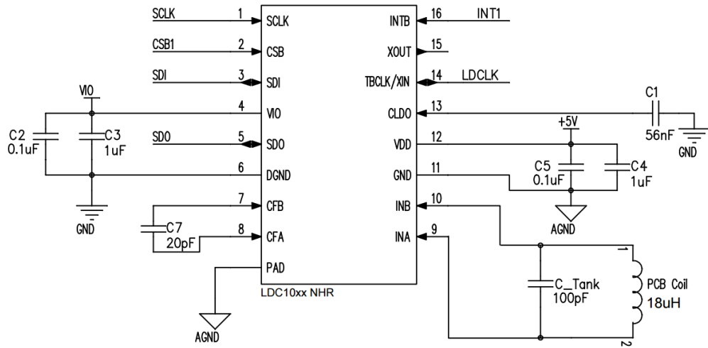
Figure 17: General Usage Schematic for LDC1000*
