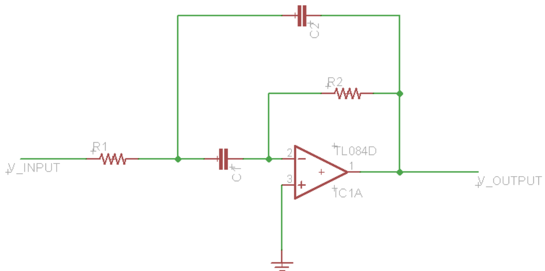
Figure 38: Active Bandpass Filter Schematic
