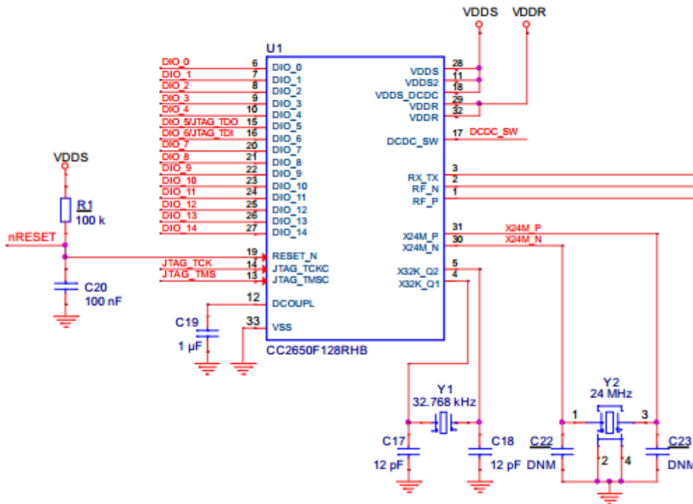
Figure 28: CC2650 Clocks and Power Schematics *
