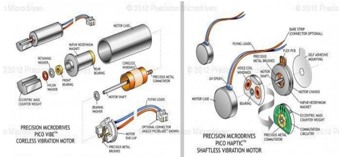
Figure 21: Inside of the Eccentric Rotation Mass Actuator*
