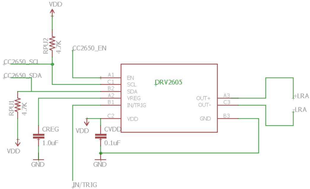
Figure 22: DRV2605 Eagle Schematic
