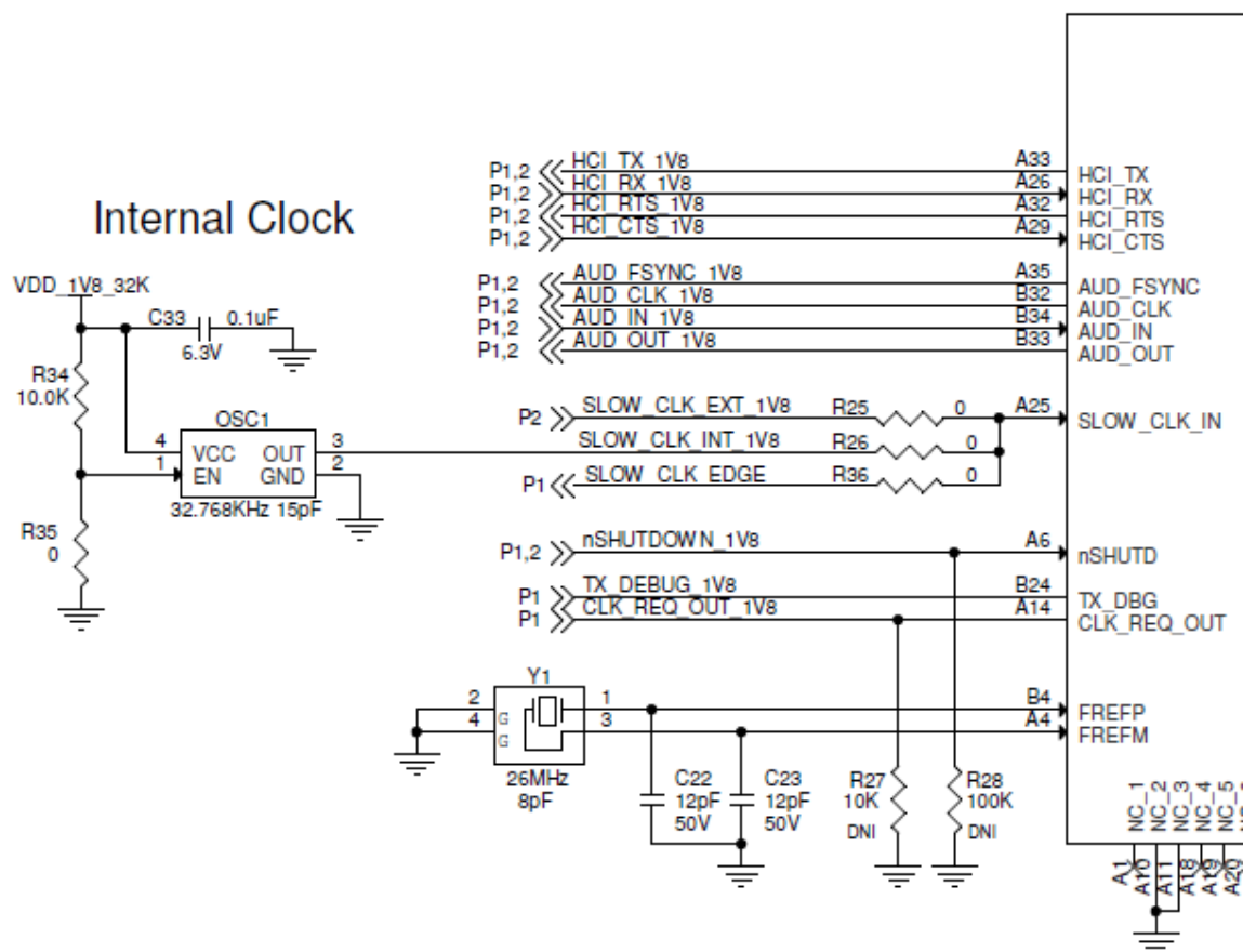
Figure 24: TI's CC2560 Reference Design*
