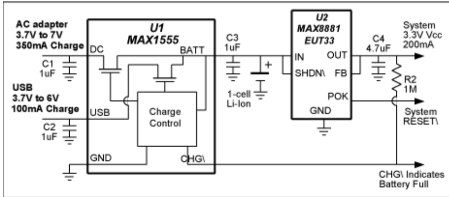
Figure 52: Charge Controller Schematic 8
