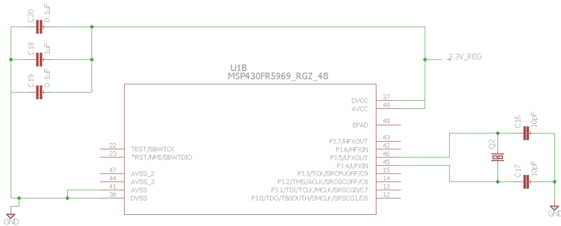
Figure 35: MSP430 Power Schematic
