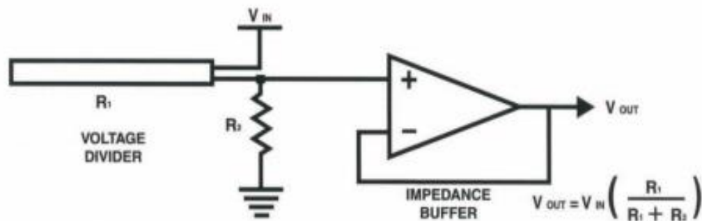
Figure 16: Schematic of Flex22 Sensor®
