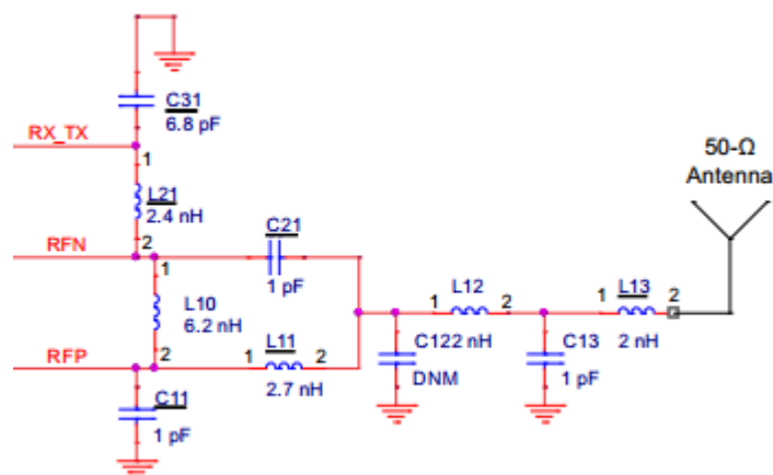
Figure 27: BT Passive Filter Antenna Schematic
