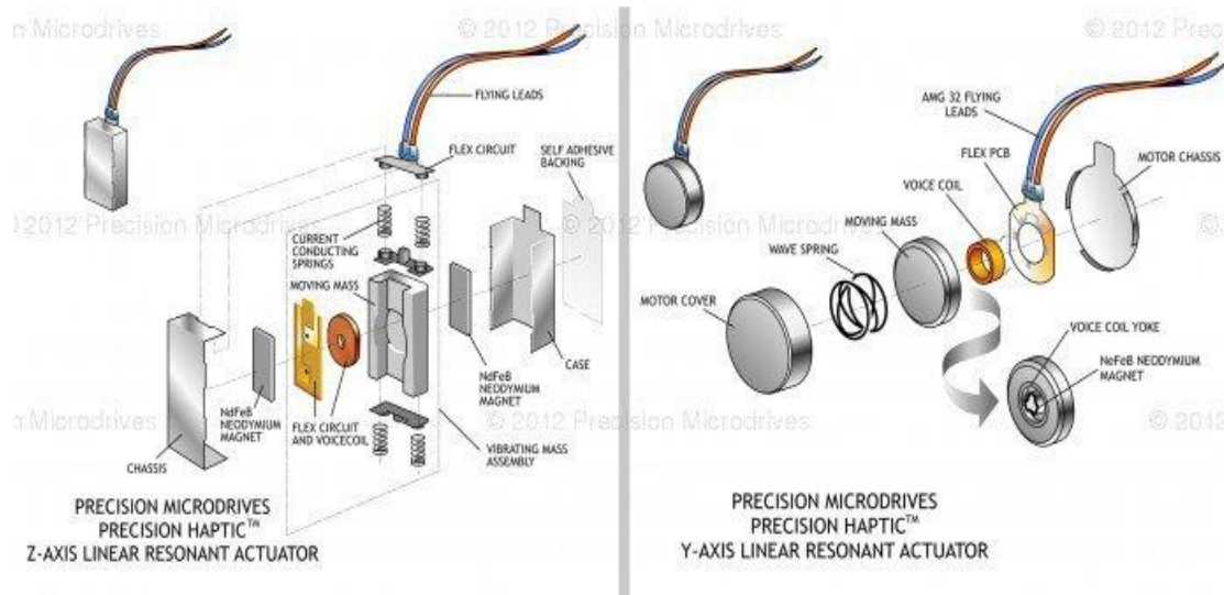
Figure 20: Inside of the LRA+
