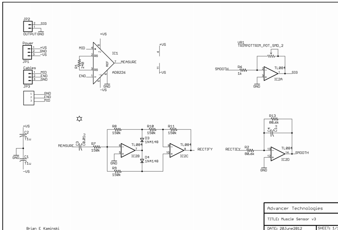
Figure 7: Advancer EMG Schematic#
