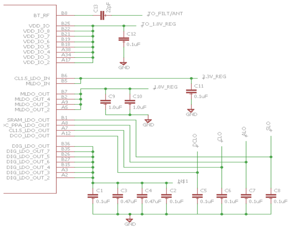
Figure 33: CC2560 IO Schematic
