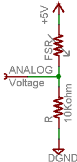
Figure 15: Schematic of FSR~
