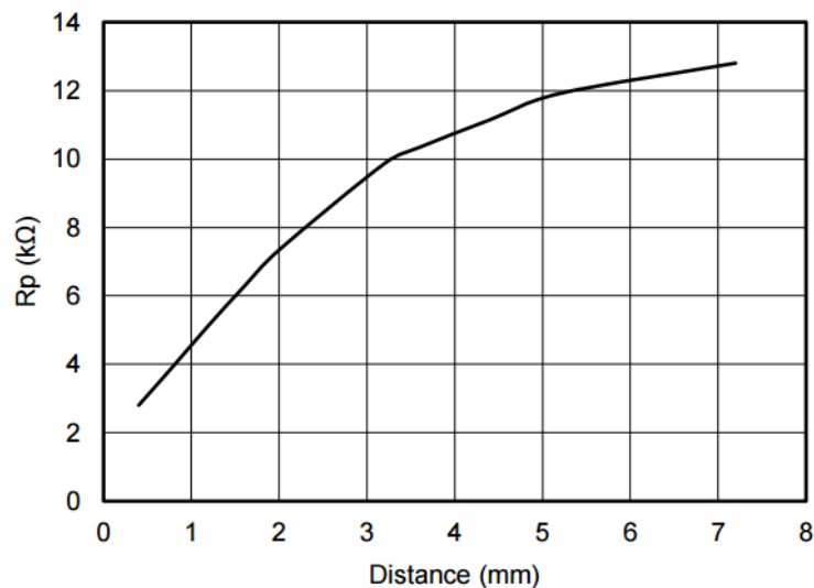
Figure 14: LDC1000 Characteristics*
