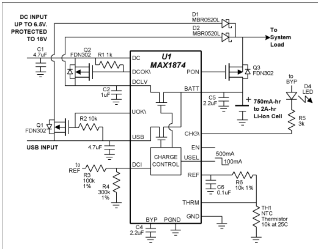
Figure 53: MOSFET Integrated Charge Controller Design 8
