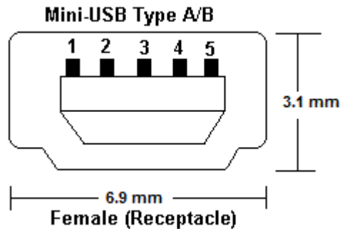
Figure 51: Mini-USB Connector &
