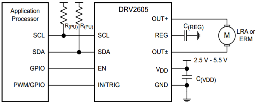
Figure 19: Typical Usage Schematic for DRV2605*
