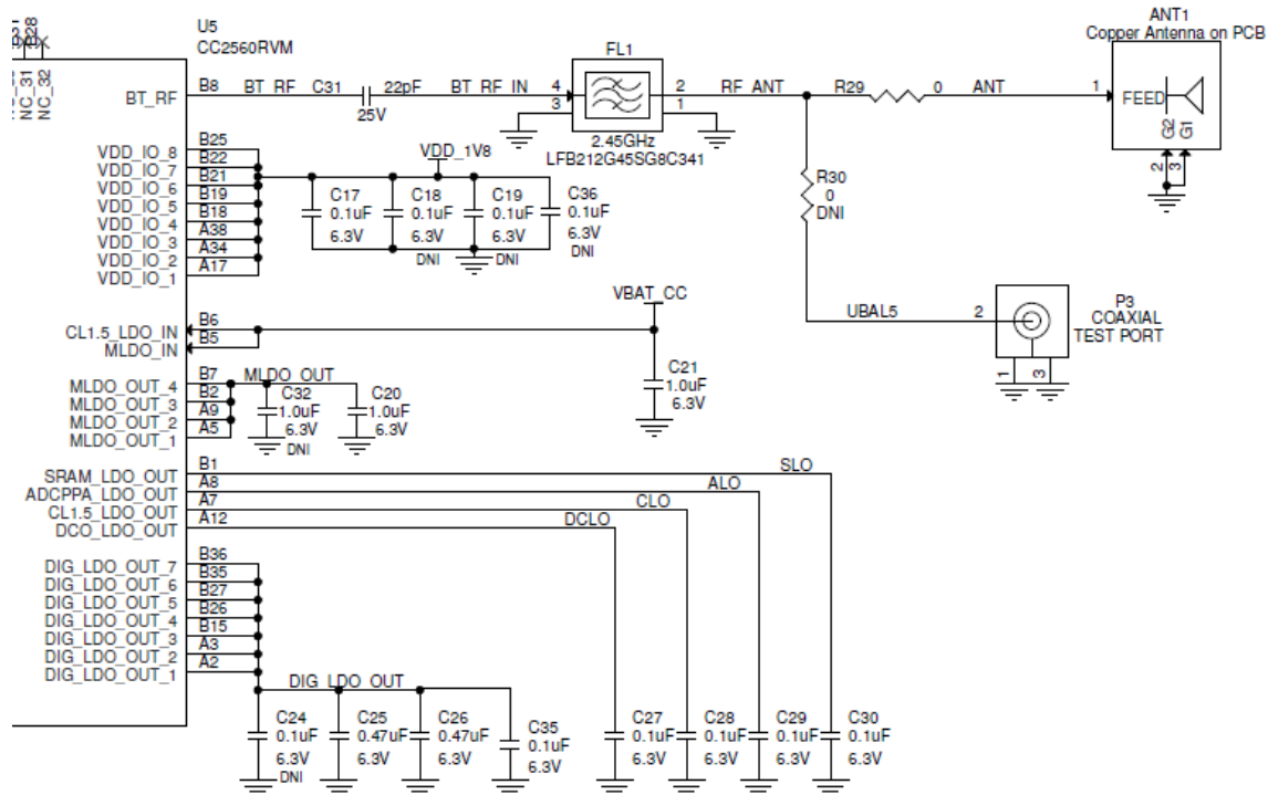
Figure 25: TI's CC2560 Reference Design Continued*
