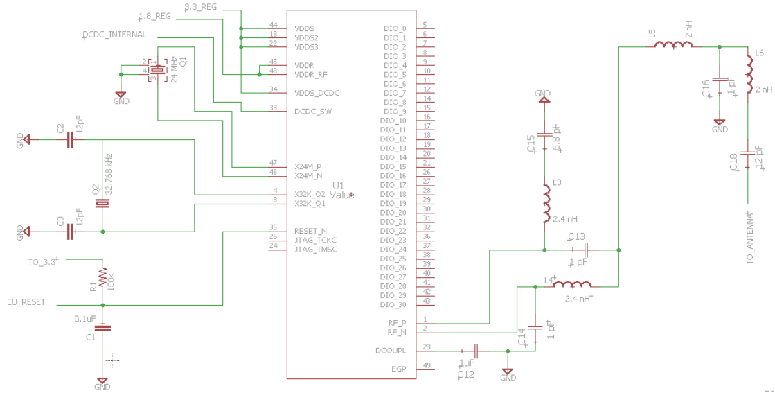
Figure 29: CC2650 Final Schematic
