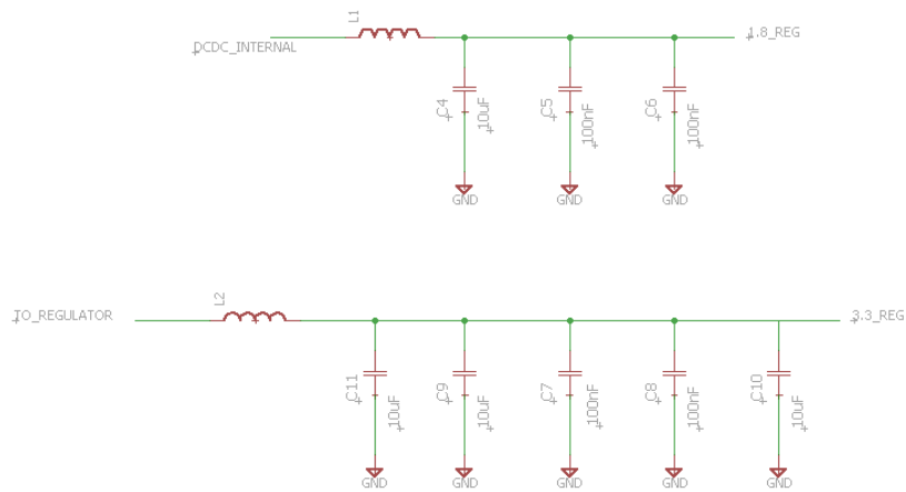
Figure 30: CC2650 Bypass Capacitors
