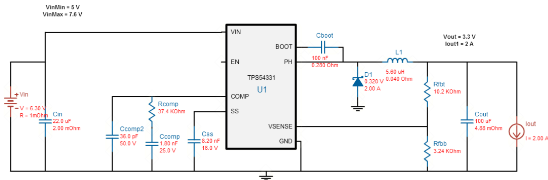
Figure 32: Switching Buck Converter*
