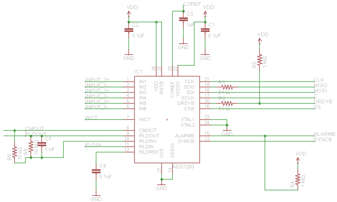
Figure 41: ADS1293 Schematic
