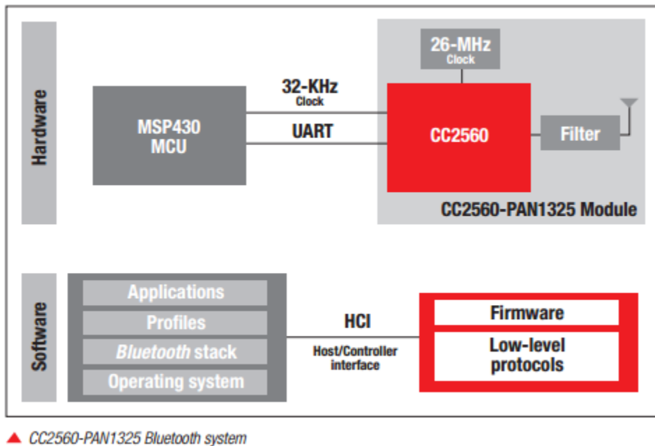
Figure 55: CC2560 EVM Block Diagram*
