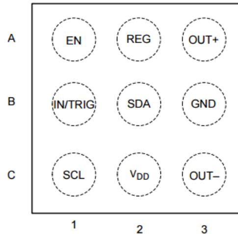
Figure 18: DRV260 Pin Configuration*
