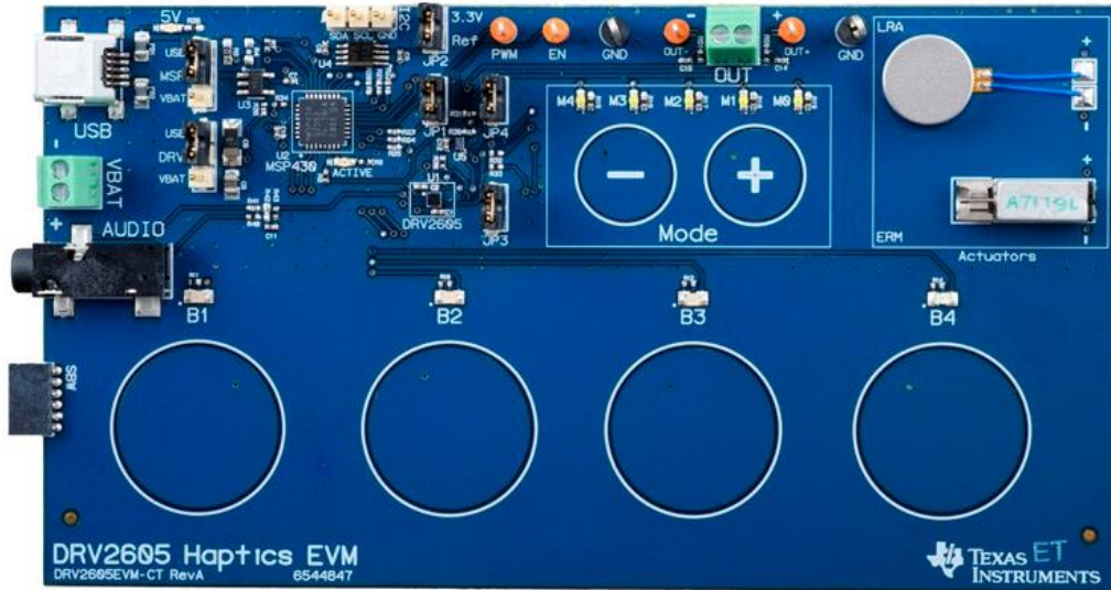
Figure 56: DRV 2605 EVM
