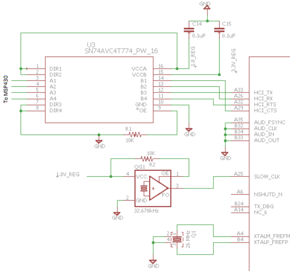
Figure 34: MSP430 Connection to CC2560
