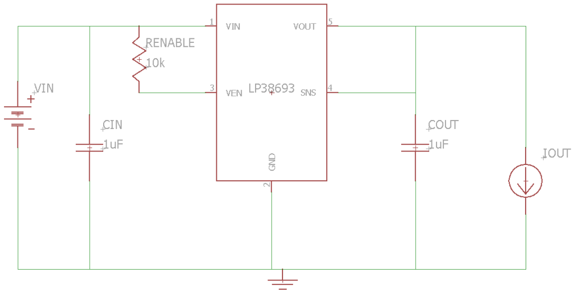
Figure 31: 3.3 V LDO Regulator
