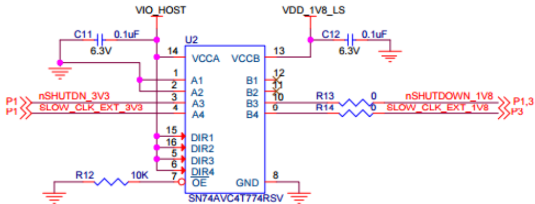
Figure 26: Logic Level Shifter Schematic
