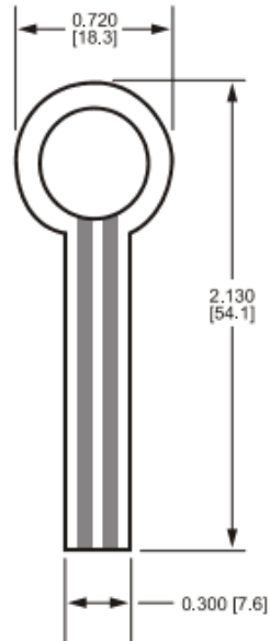
Figure 12: Layout of Rounded FSR~
