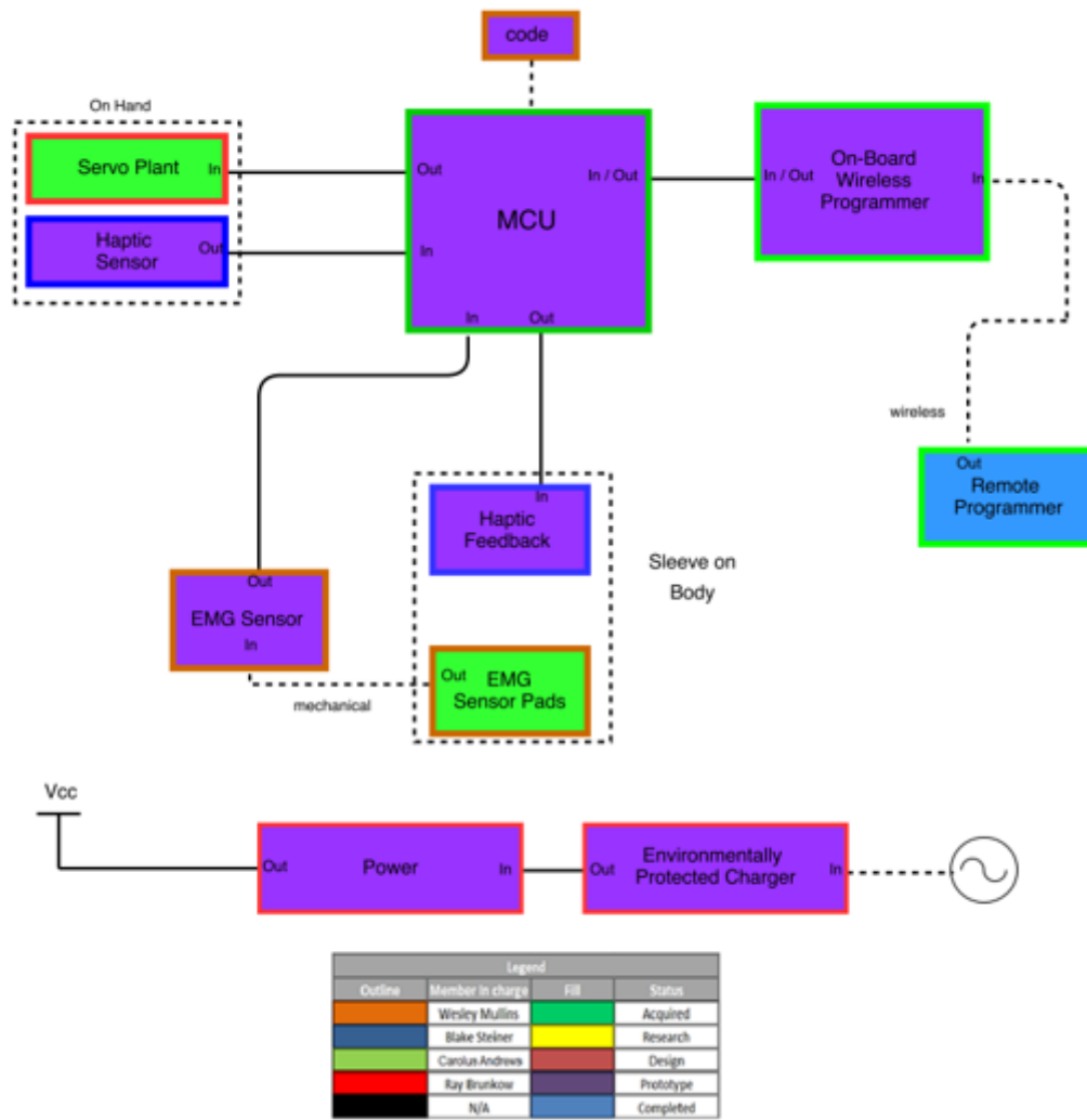
Figure 1: Block Diagram
